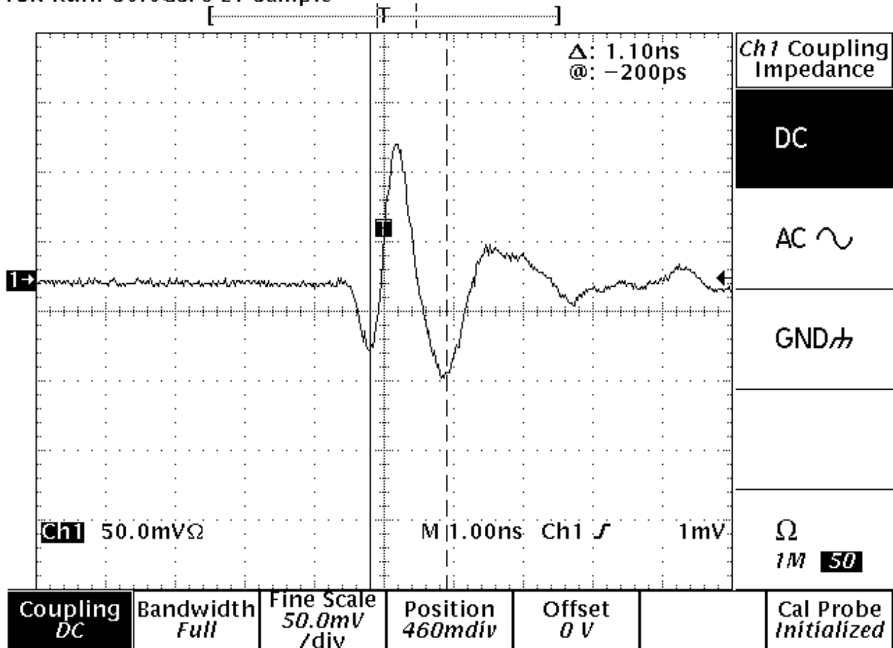
Figure 1. Pulse characteristic of a 800 UWB-unit.
