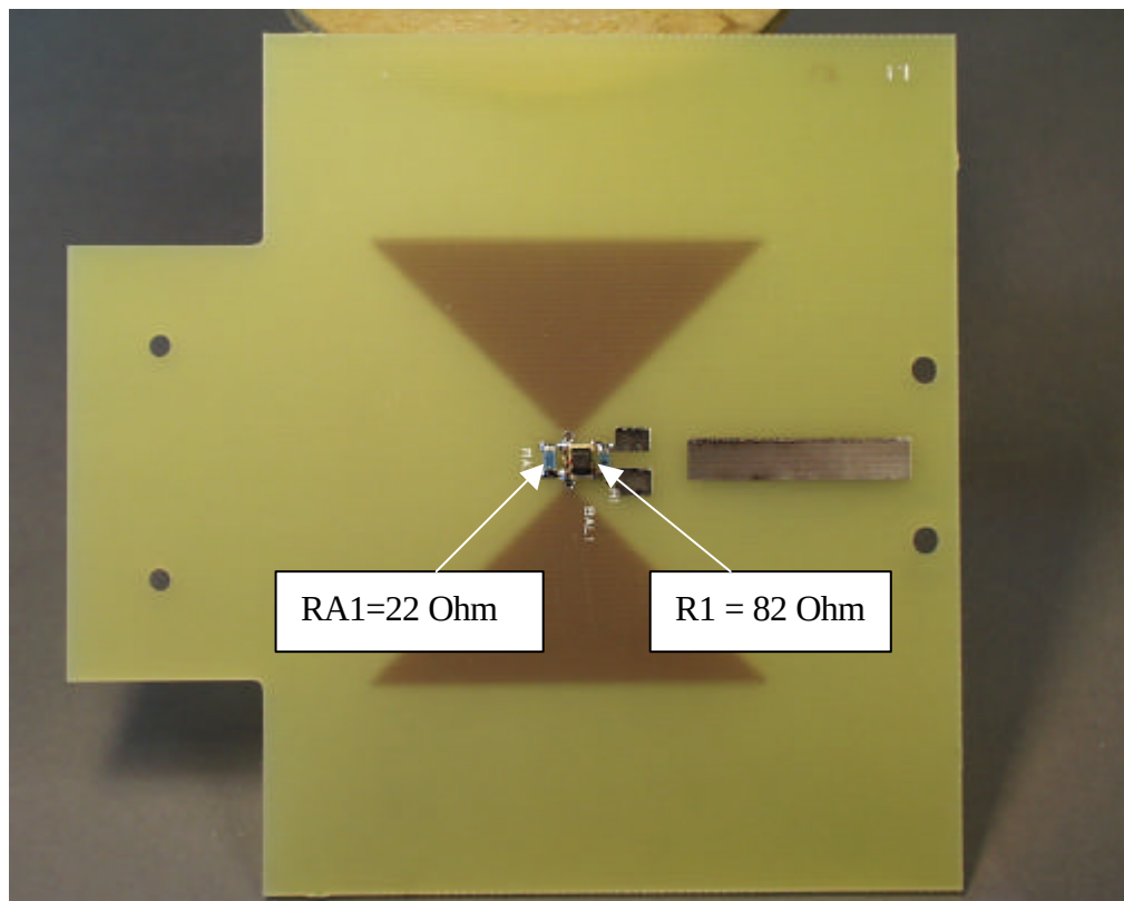
Picture 8. Transmitter antenna board with required modifications according to section 4.5 in testreport.
