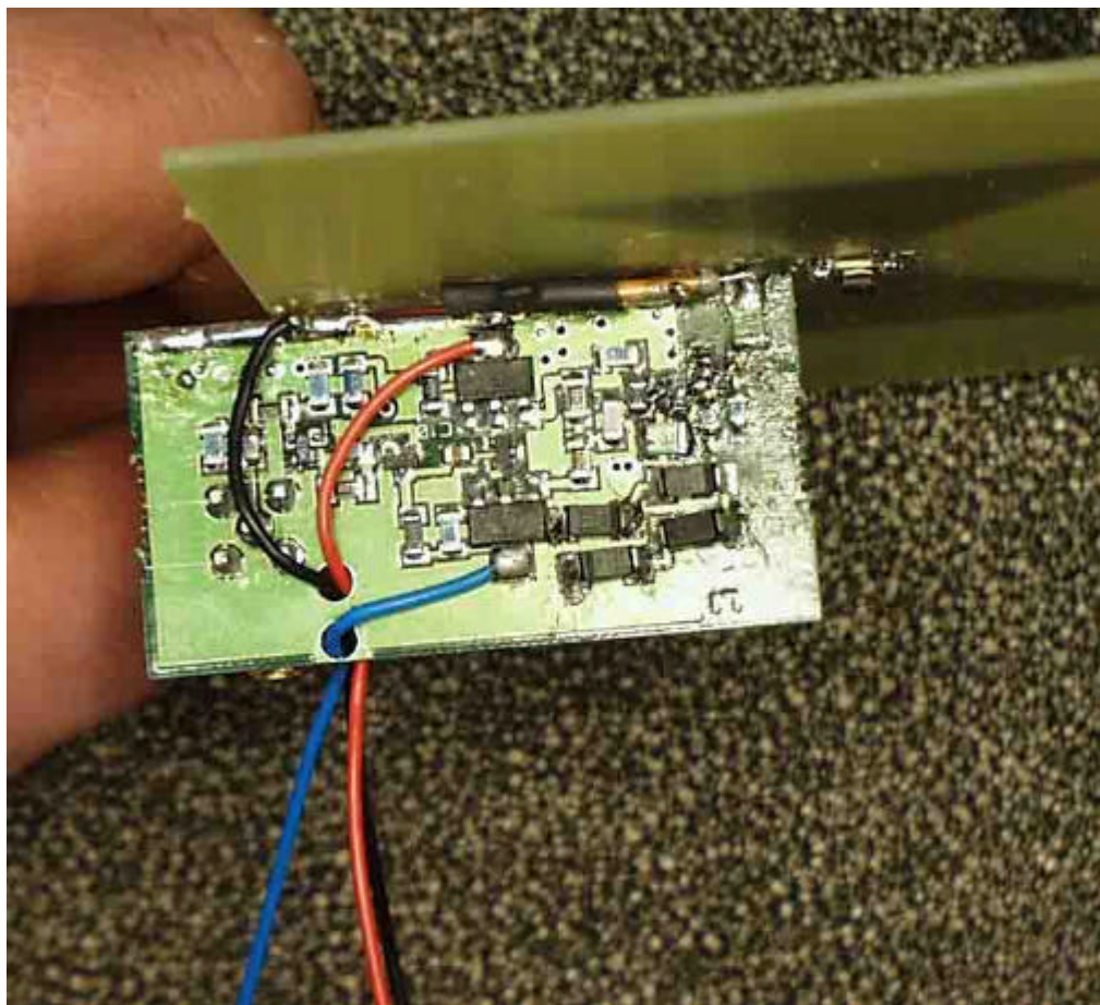
Picture 9. Antenna board with impulse generator.
