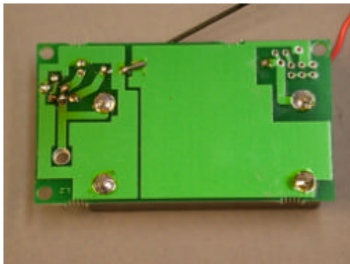
Picture 6. Backside of High voltage PCB
