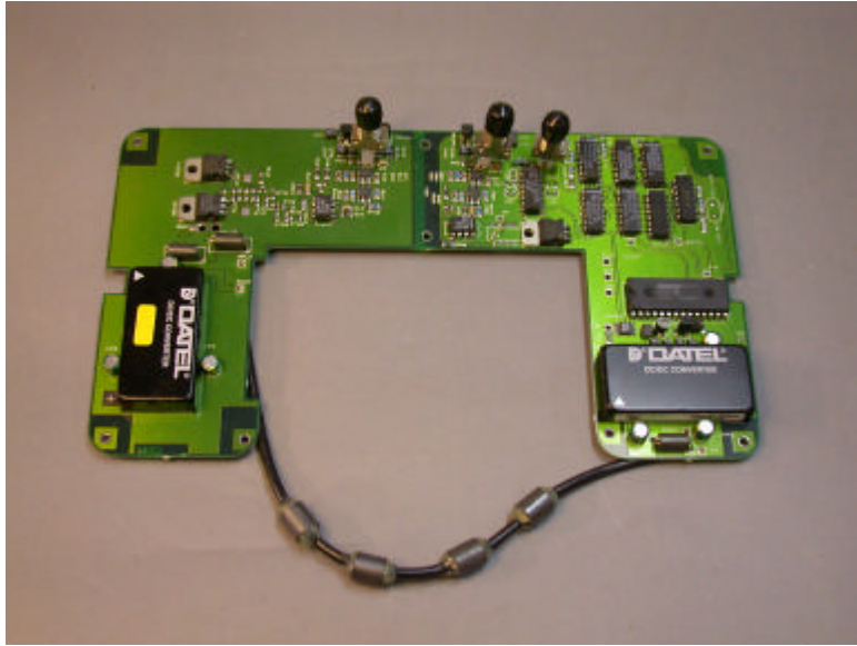
Picture 5. Backside of main board
