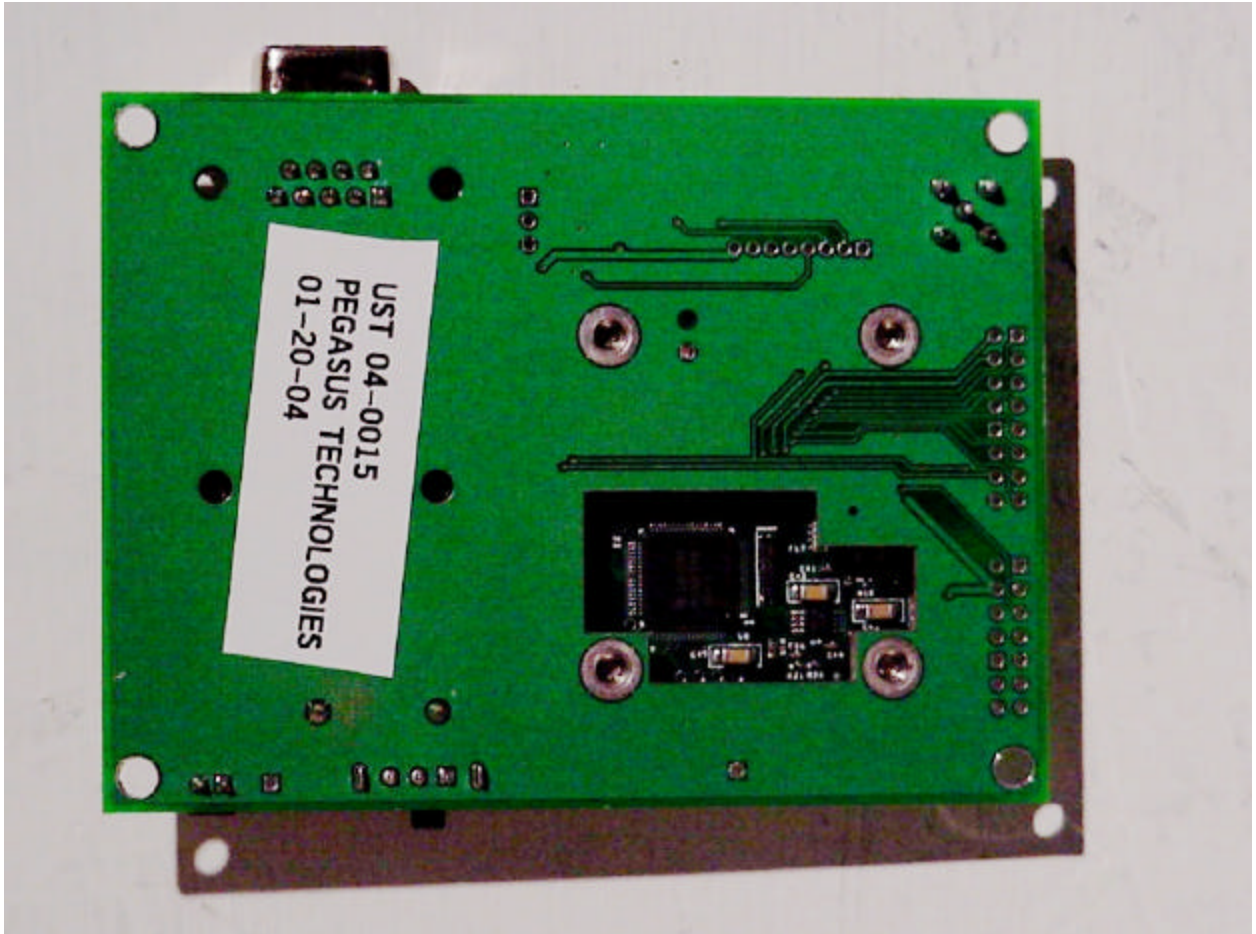
Photo 2. (EUT) Bottom View
