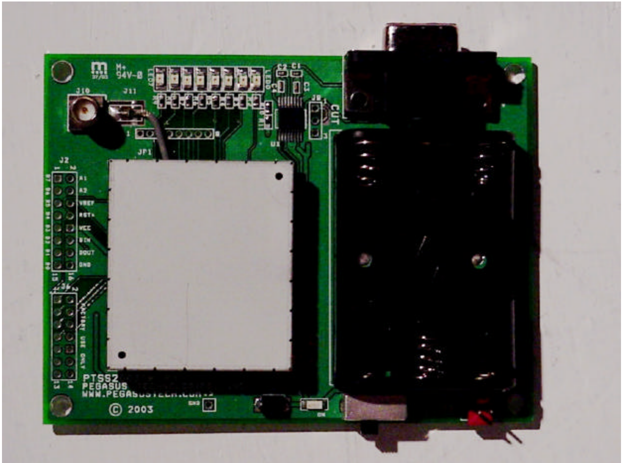
Photo 1. (EUT) Top View
