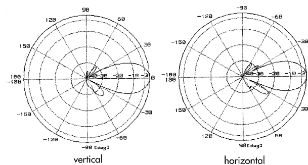
Figure B.7: VLA 2418 CP-R Antenna Polarization
