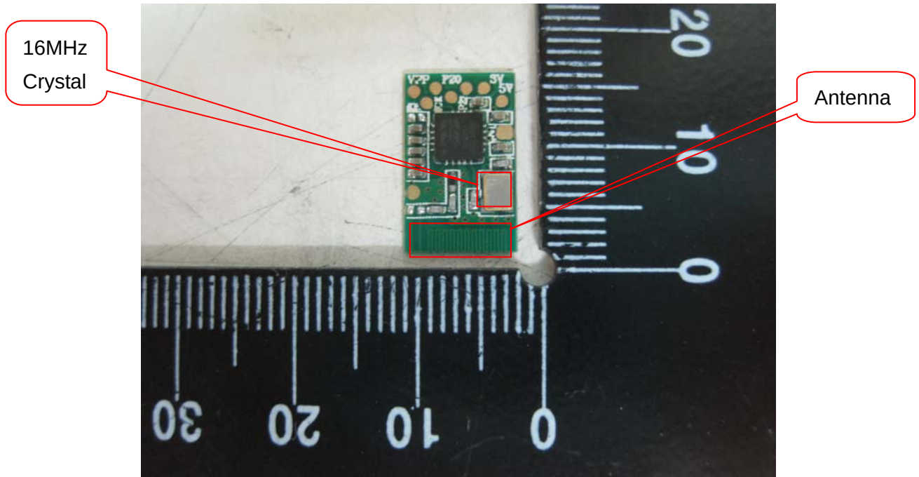
Front View of the RF module
