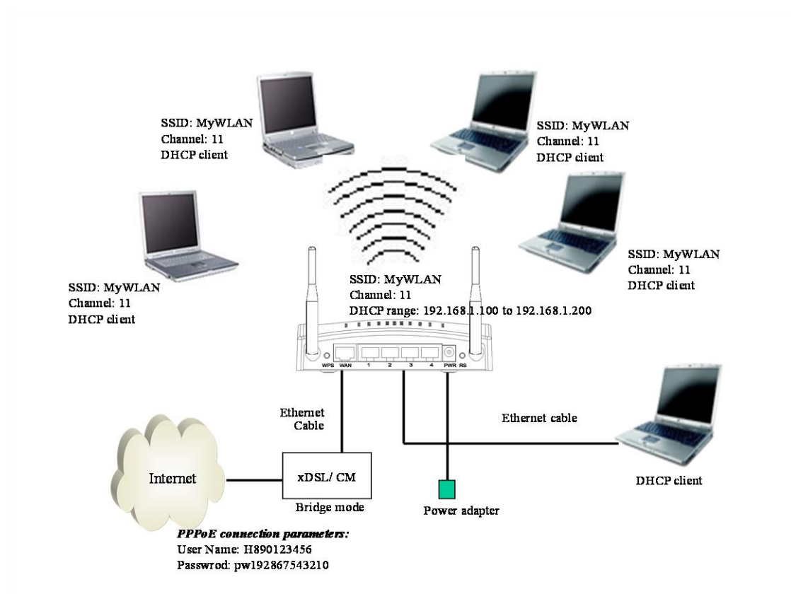
Figure 3 – Configuration Example One – PPPoE on the WAN
