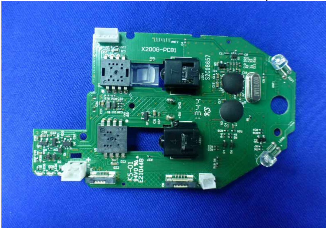
Figure 9 Component Side of the PCB
