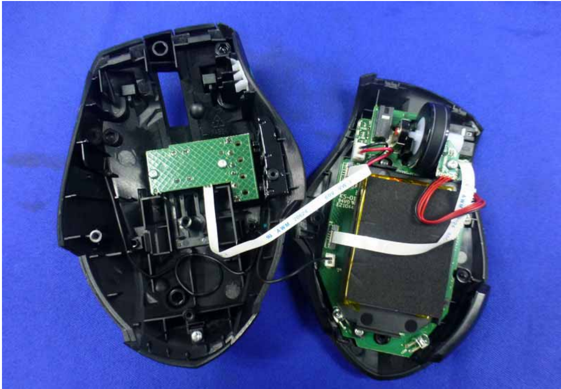
Figure 5 Inside of the EUT
