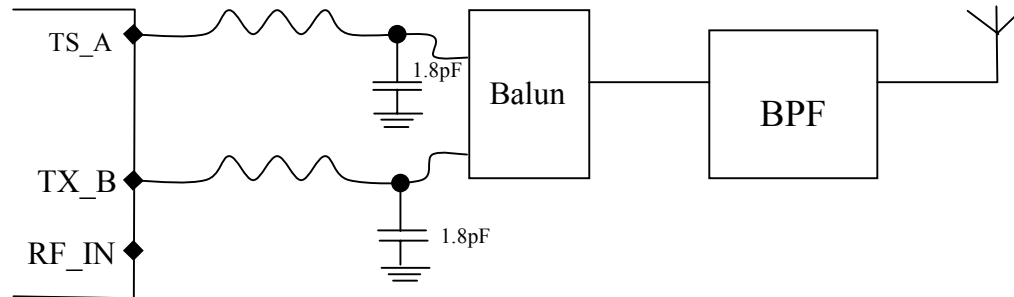
Figure 3.1: RF Parts (Class2)
