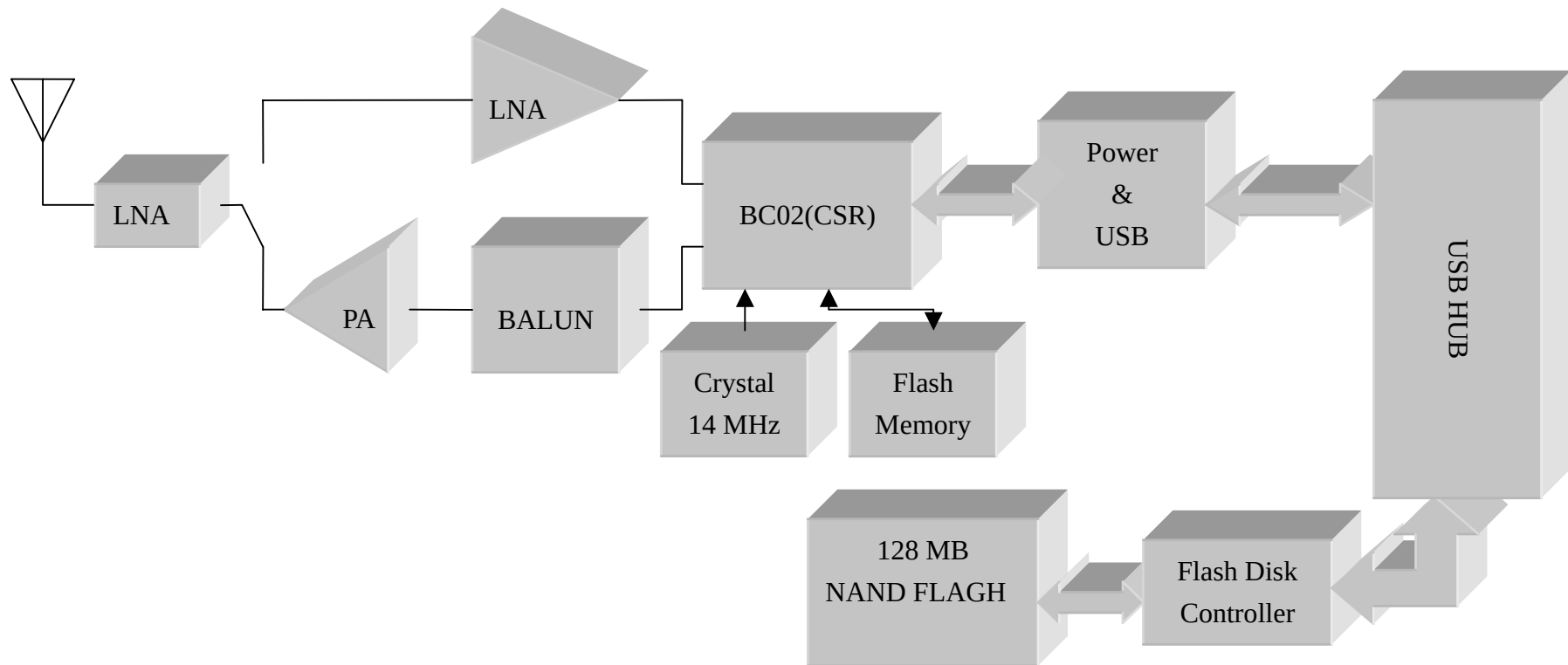
Block Diagram of BT-DG04A
