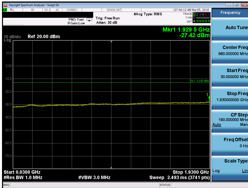
Plot 7-205. Conducted Spurious Plot (Band 2 - 1.4MHz QPSK – Mid Channel)
