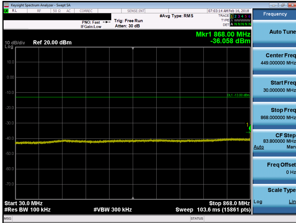
Plot 7-138. Conducted Spurious Plot (Band 5 - 1.4MHz QPSK – Low Channel)
