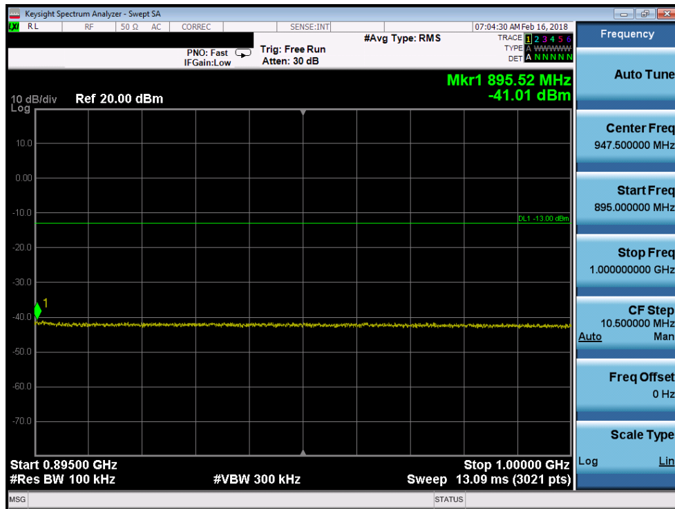
Plot 7-139. Conducted Spurious Plot (Band 5 - 1.4MHz QPSK – Low Channel)
