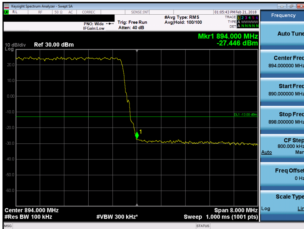
Plot 7-194. Upper Band Edge Plot (Band 5 - 10.0MHz 256-QAM)
