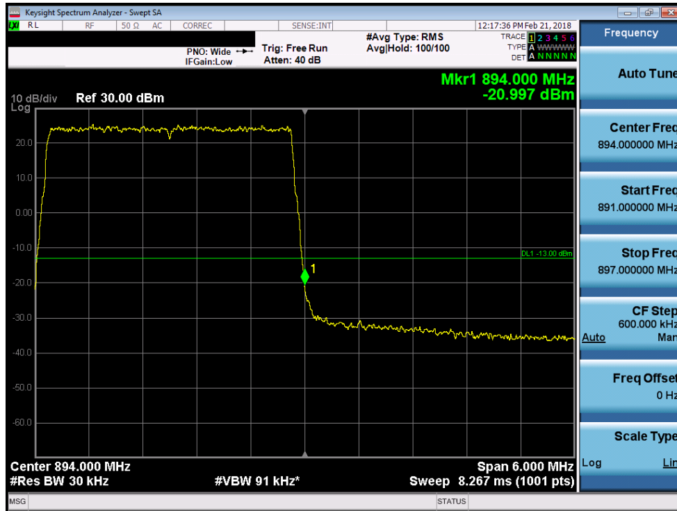
Plot 7-173. Upper Band Edge Plot (Band 5 - 3.0MHz 64-QAM)
