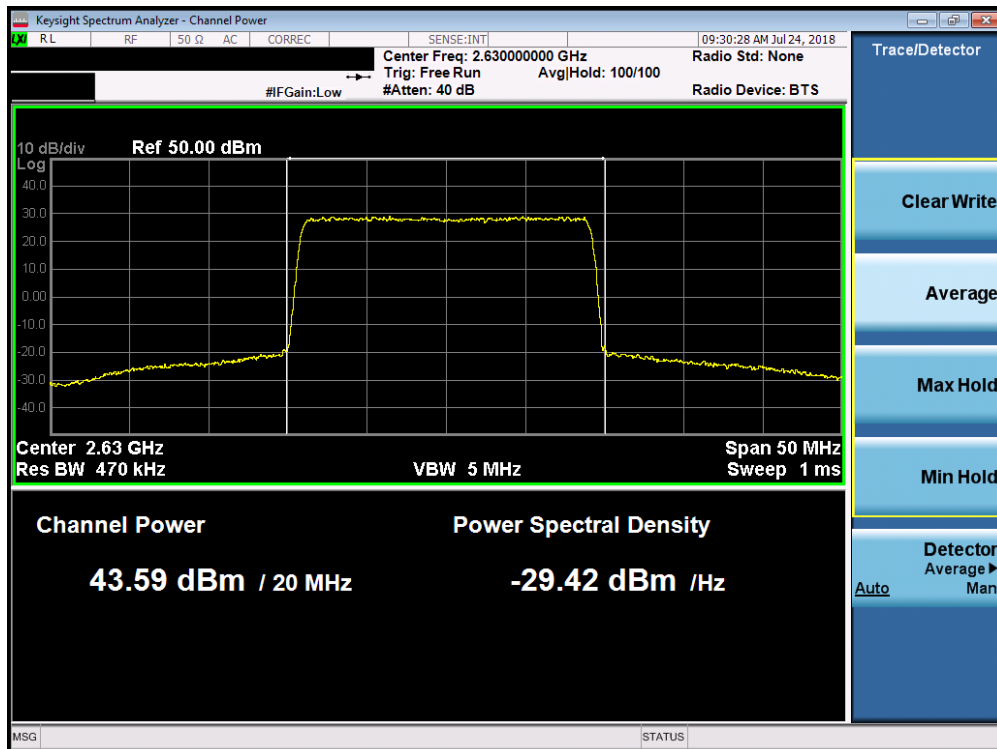
Plot 7-85. Maximum Conducted Power (Band 7 - 20.0MHz QPSK - Low Channel)
