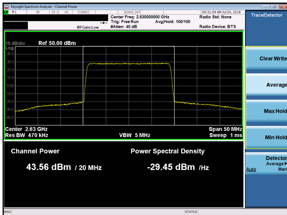
Plot 7-88. Maximum Conducted Power (Band 7 - 20.0MHz 16-QAM - Low Channel)
