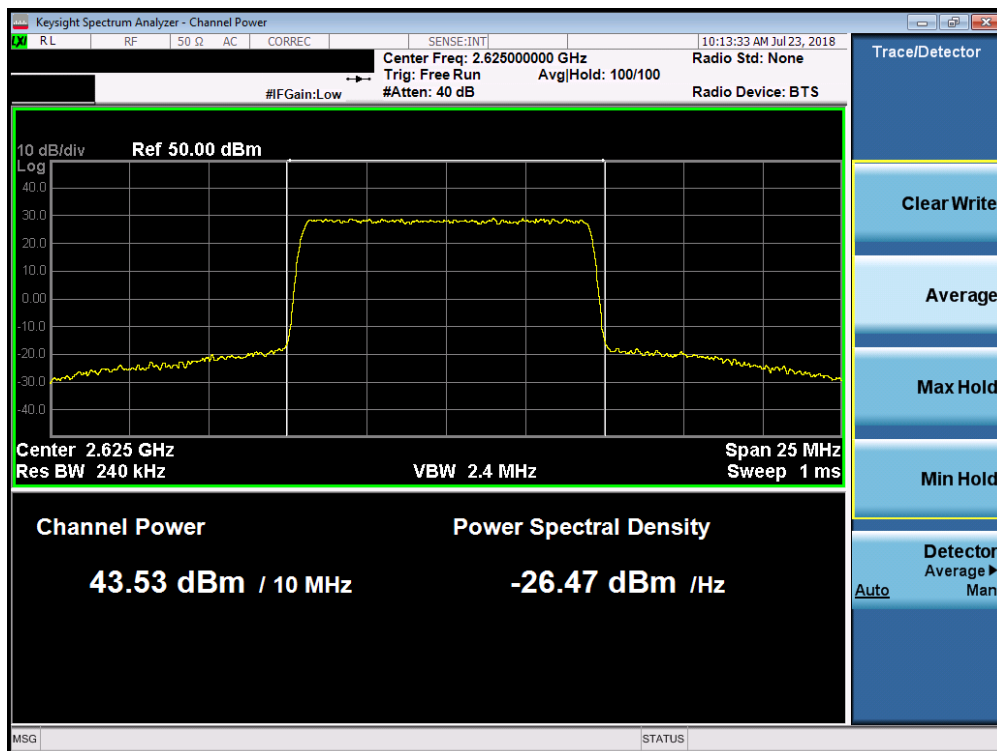
Plot 7-19. Maximum Conducted Power (Band 7 - 10.0MHz 64-QAM – Low Channel)
