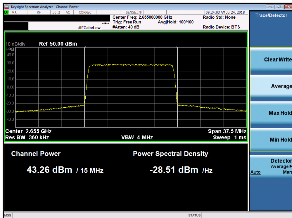
Plot 7-80. Maximum Conducted Power (Band 7 - 15.0MHz 64-QAM - Mid Channel)
