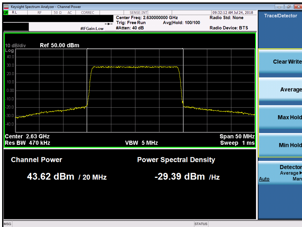
Plot 7-91. Maximum Conducted Power (Band 7 - 20.0MHz 64-QAM - Low Channel)
