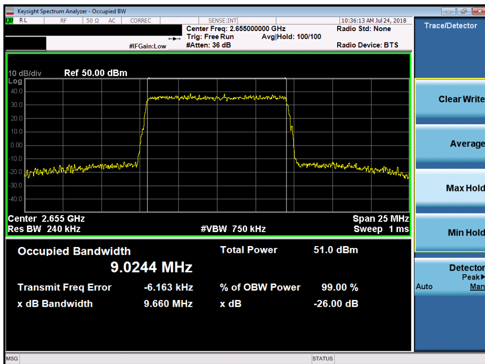
Plot 7-120. Occupied Bandwidth Plot (Band 7 - 10.0MHz 256-QAM)
