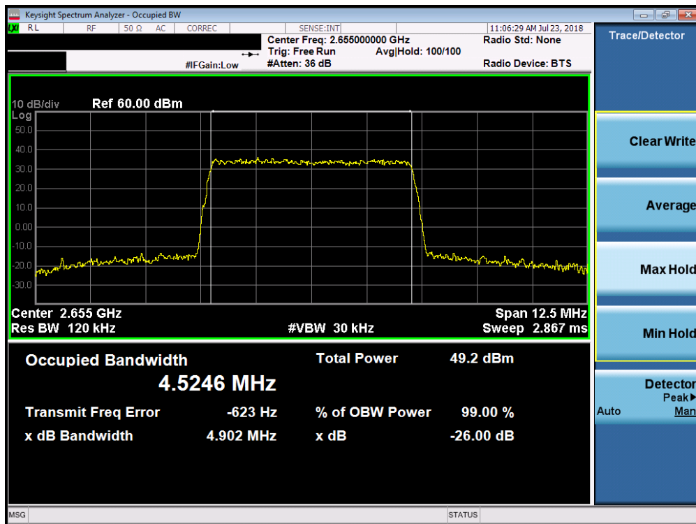
Plot 7-100. Occupied Bandwidth Plot (Band 7 - 5.0MHz 256-QAM)
