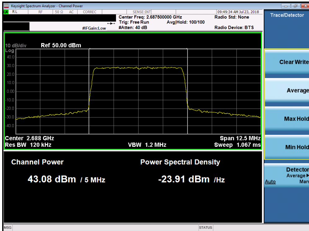
Plot 7-6. Maximum Conducted Power (Band 7 - 5.0MHz 16-QAM – High Channel)
