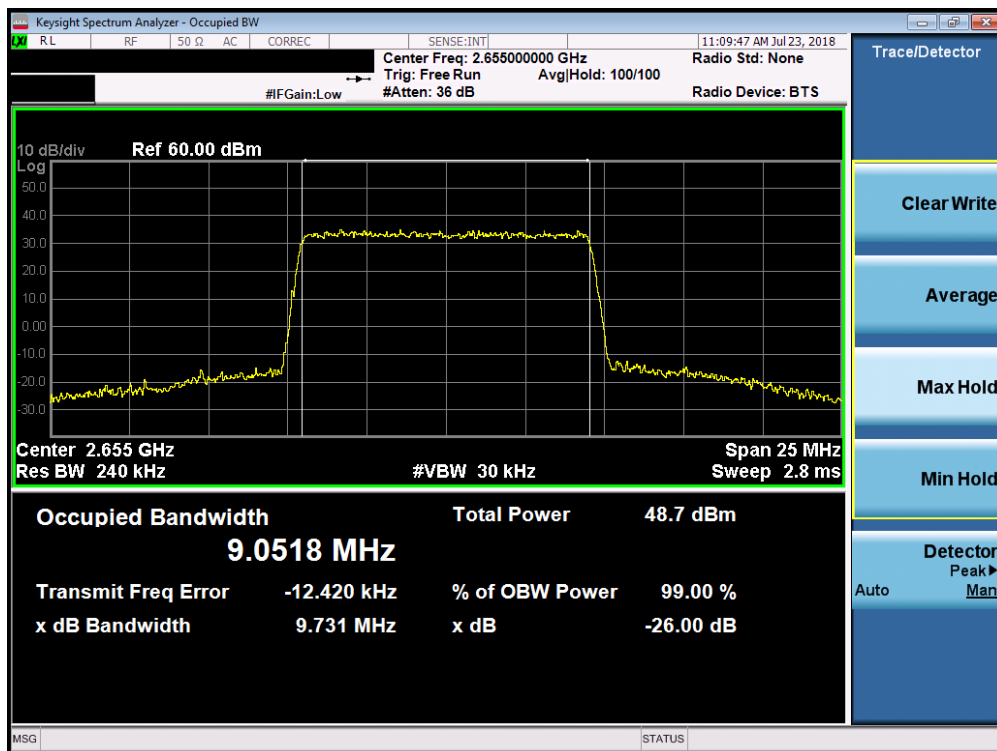
Plot 7-103. Occupied Bandwidth Plot (Band 7 - 10.0MHz 64-QAM)
