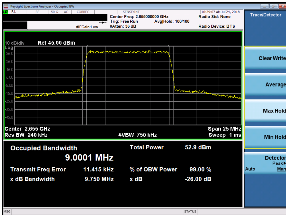
Plot 7-119. Occupied Bandwidth Plot (Band 7 - 10.0MHz 64-QAM)
