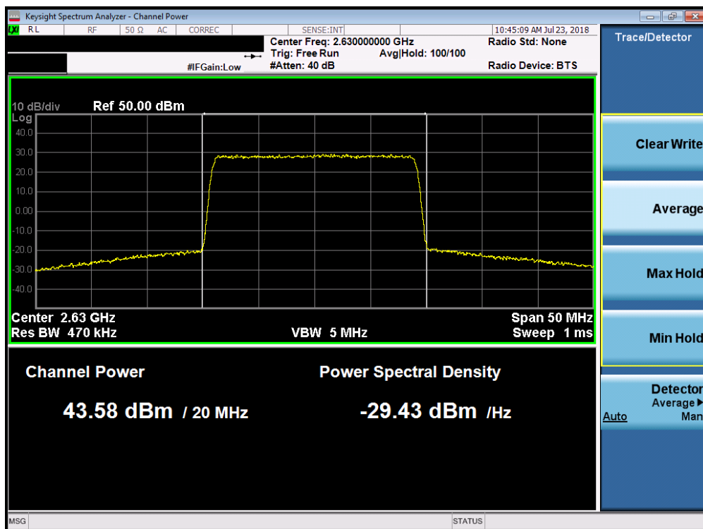
Plot 7-46. Maximum Conducted Power (Band 7 - 20.0MHz 256-QAM – Low Channel)
