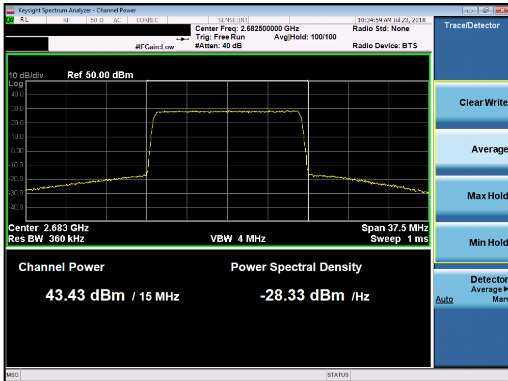
Plot 7-27. Maximum Conducted Power (Band 7 - 15.0MHz QPSK – High Channel)
