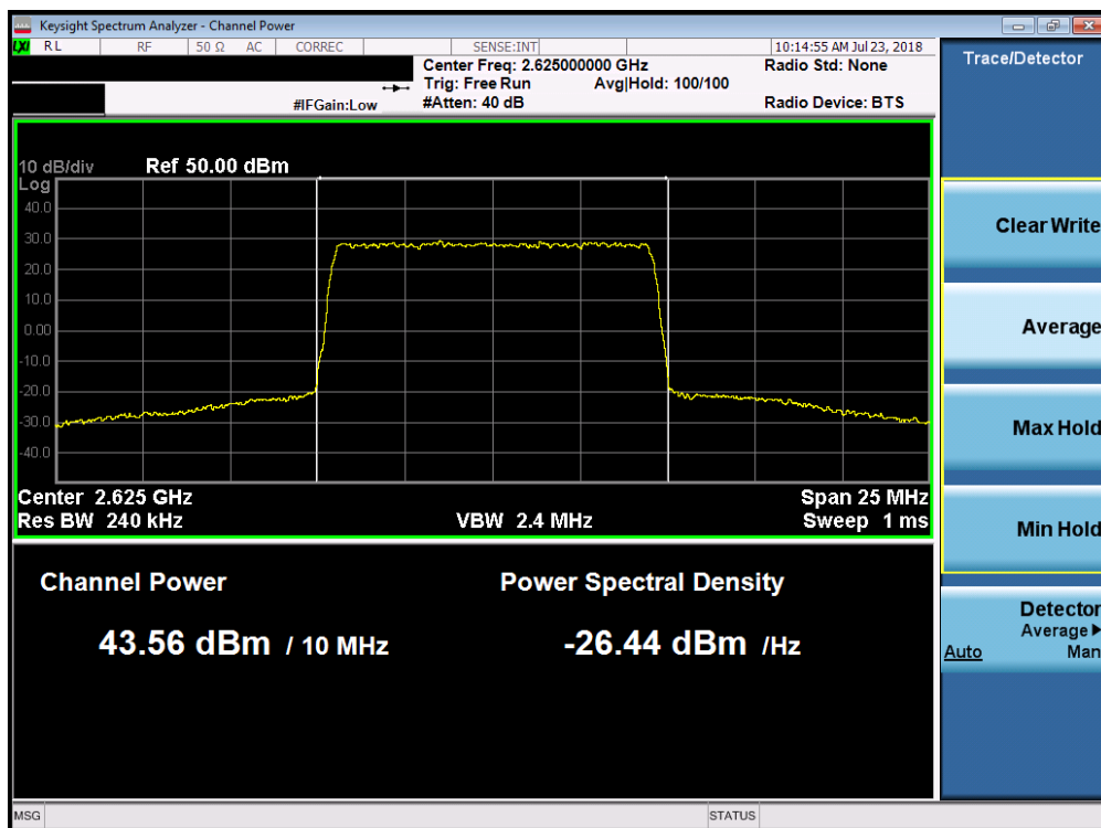
Plot 7-22. Maximum Conducted Power (Band 7 - 10.0MHz 256-QAM – Low Channel)
