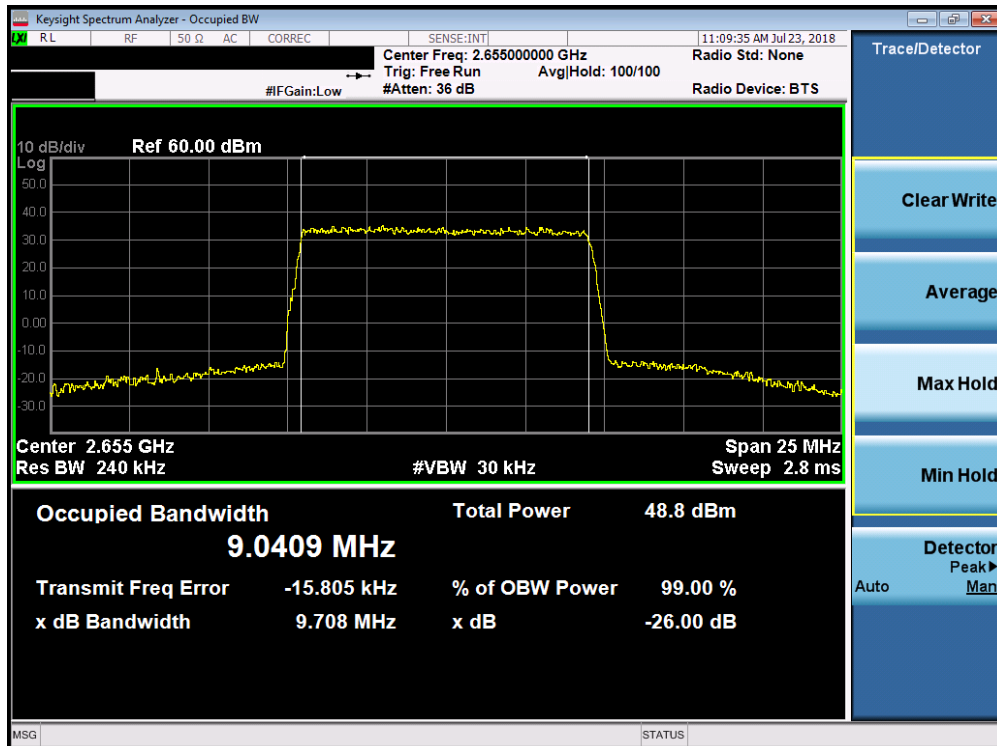
Plot 7-102. Occupied Bandwidth Plot (Band 7 - 10.0MHz 16-QAM)
