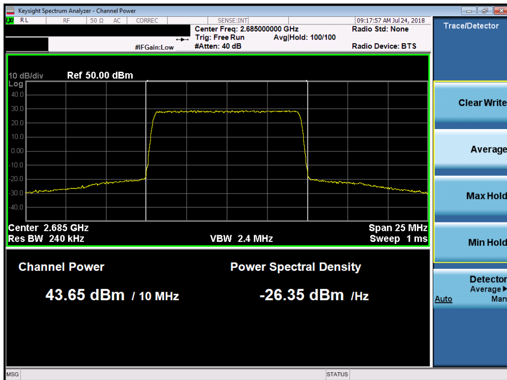
Plot 7-66. Maximum Conducted Power (Band 7 - 10.0MHz 16-QAM – High Channel)
