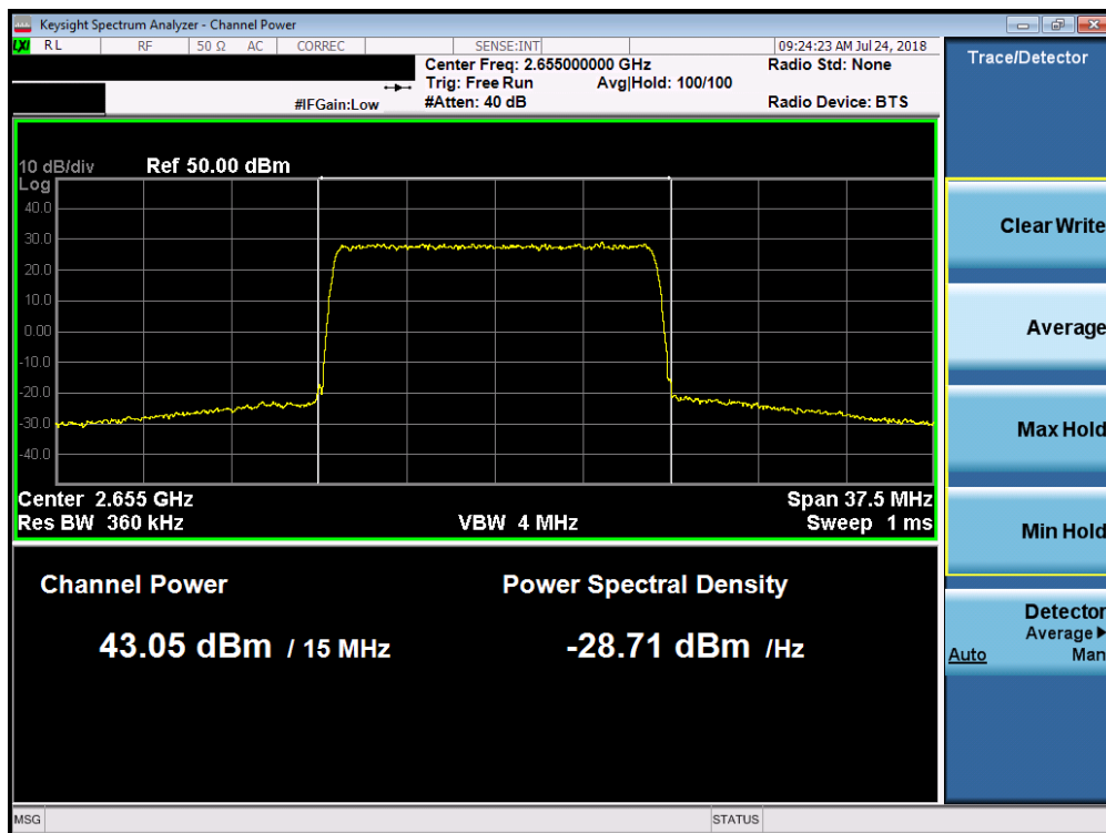
Plot 7-83. Maximum Conducted Power (Band 7 - 15.0MHz 256-QAM – Mid Channel)
