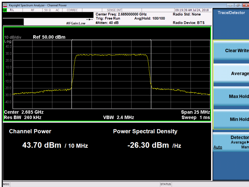
Plot 7-72. Maximum Conducted Power (Band 7 - 10.0MHz 256-QAM – High Channel)
