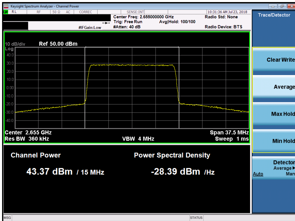
Plot 7-32. Maximum Conducted Power (Band 7 - 15.0MHz 64-QAM – Mid Channel)
