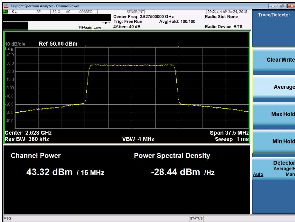
Plot 7-73. Maximum Conducted Power (Band 7 - 15.0MHz QPSK - Low Channel)
