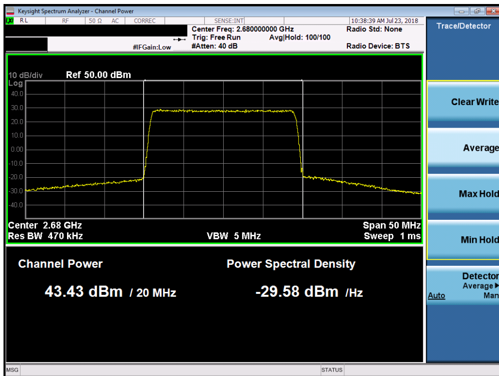
Plot 7-45. Maximum Conducted Power (Band 7 - 20.0MHz 64-QAM – High Channel)
