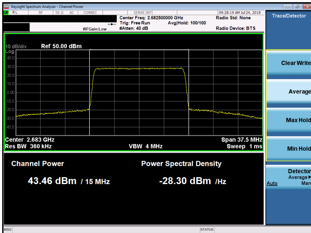
Plot 7-84. Maximum Conducted Power (Band 7 - 15.0MHz 256-QAM – High Channel)
