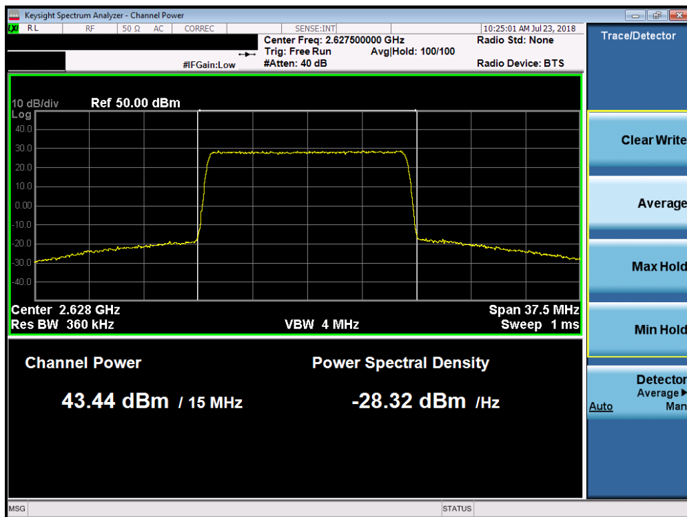
Plot 7-25. Maximum Conducted Power (Band 7 - 15.0MHz QPSK – Low Channel)
