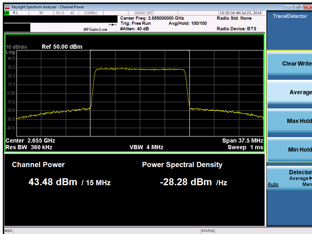
Plot 7-29. Maximum Conducted Power (Band 7 - 15.0MHz 16-QAM – Mid Channel)
