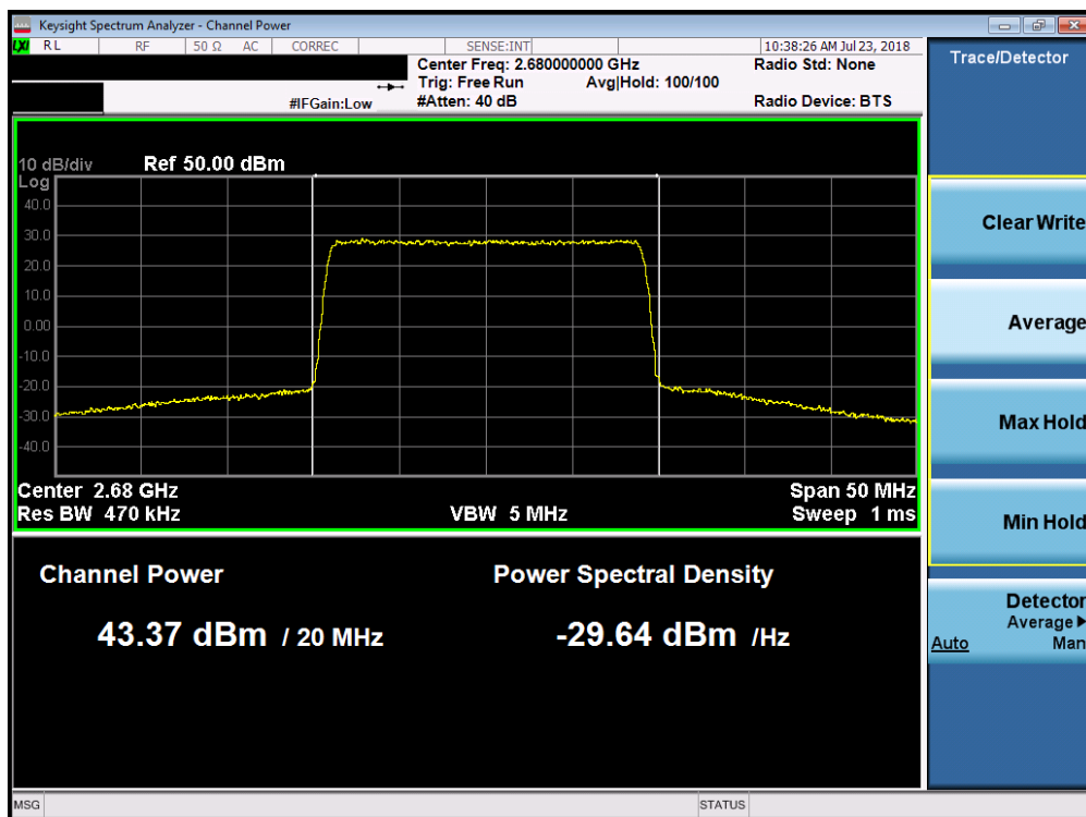
Plot 7-42. Maximum Conducted Power (Band 7 - 20.0MHz 16-QAM – High Channel)
