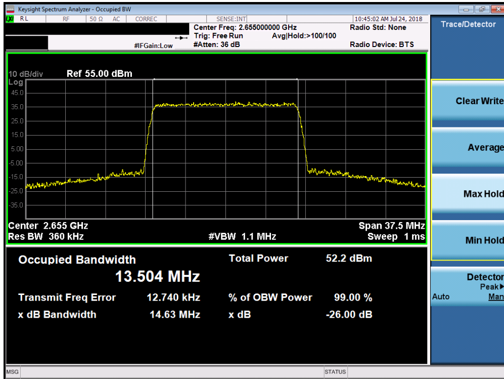
Plot 7-123. Occupied Bandwidth Plot (Band 7 - 15.0MHz 64-QAM)
