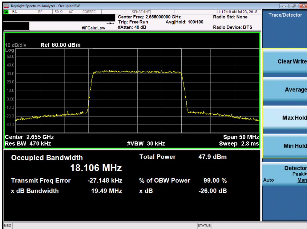
Plot 7-112. Occupied Bandwidth Plot (Band 7 - 20.0MHz 256-QAM)
