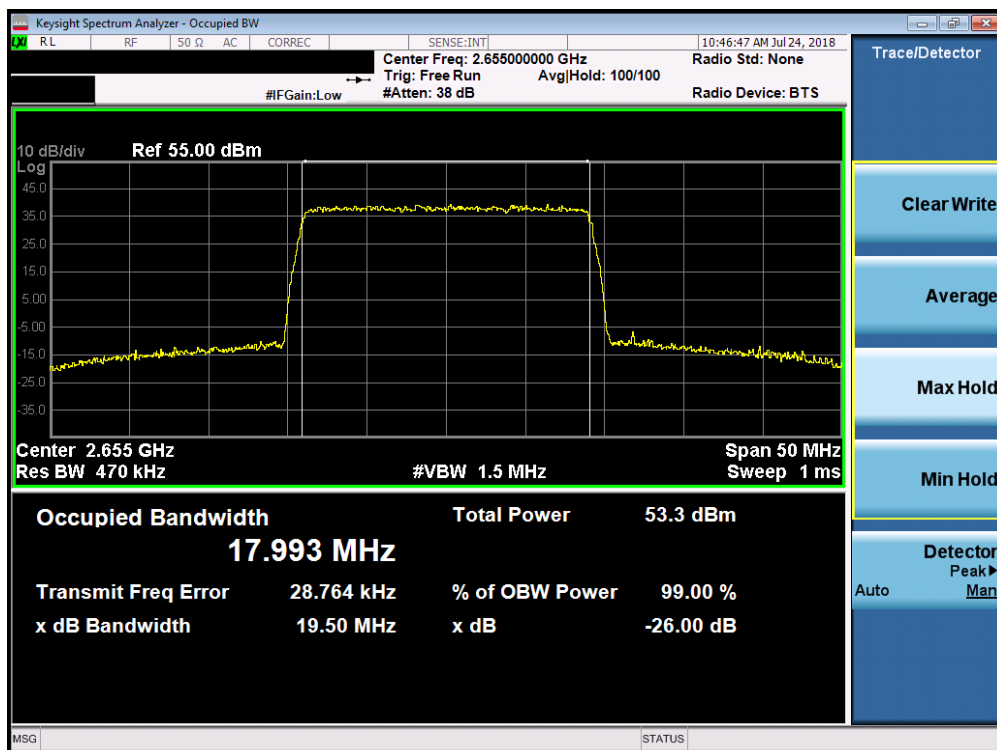
Plot 7-128. Occupied Bandwidth Plot (Band 7 - 20.0MHz 256-QAM)
