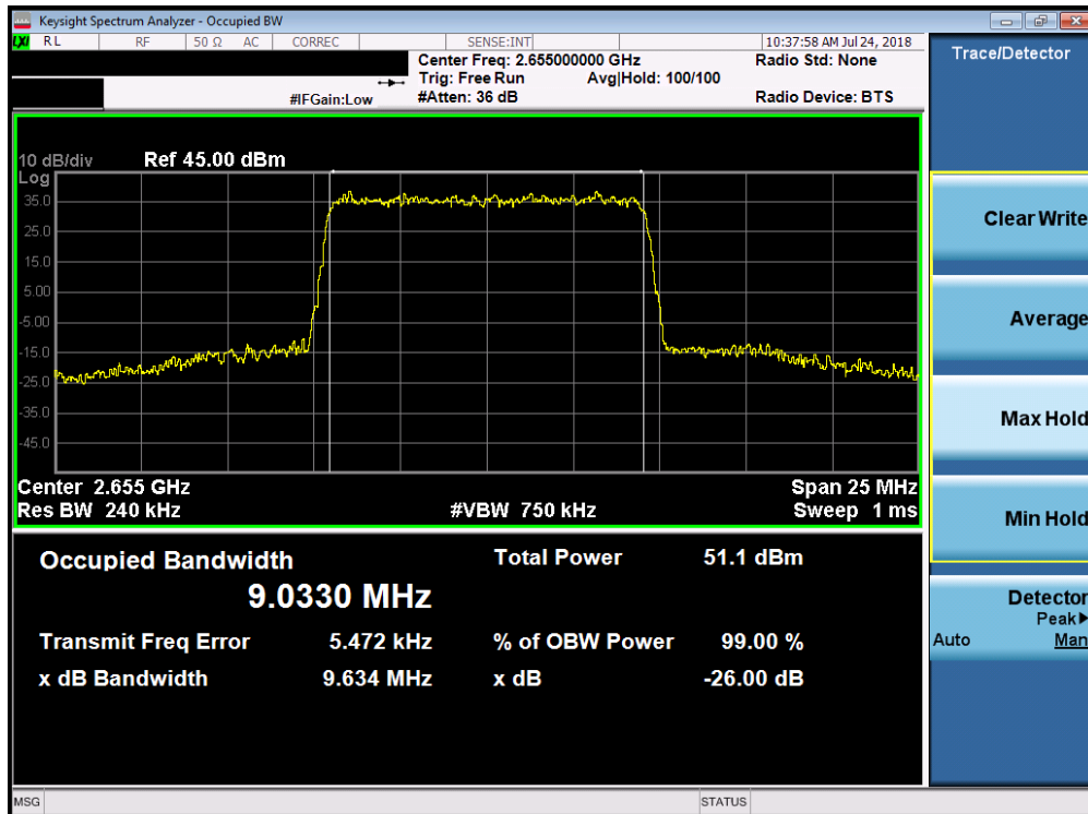
Plot 7-118. Occupied Bandwidth Plot (Band 7 - 10.0MHz 16-QAM)
