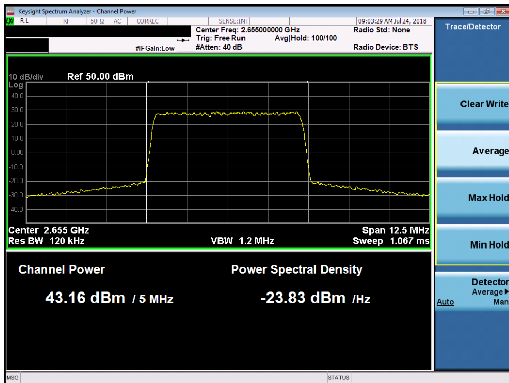
Plot 7-53. Maximum Conducted Power (Band 7 - 5.0MHz 16-QAM – Mid Channel)
