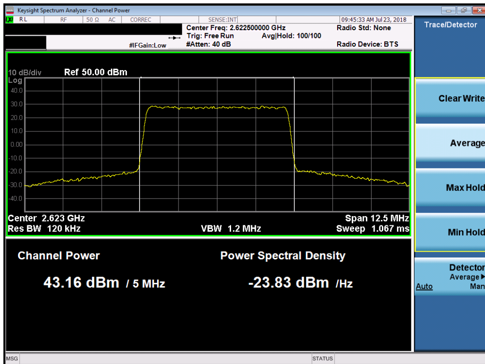
Plot 7-4. Maximum Conducted Power (Band 7 - 5.0MHz 16-QAM – Low Channel)
