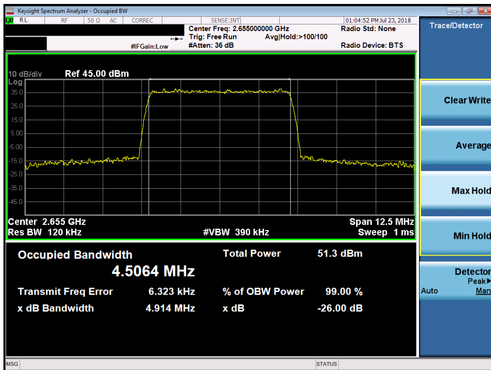
Plot 7-115. Occupied Bandwidth Plot (Band 7 - 5.0MHz 64-QAM)
