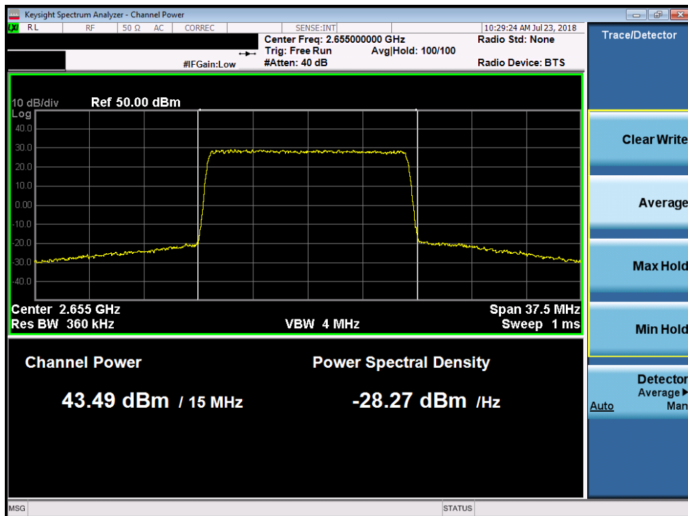
Plot 7-26. Maximum Conducted Power (Band 7 - 15.0MHz QPSK – Mid Channel)
