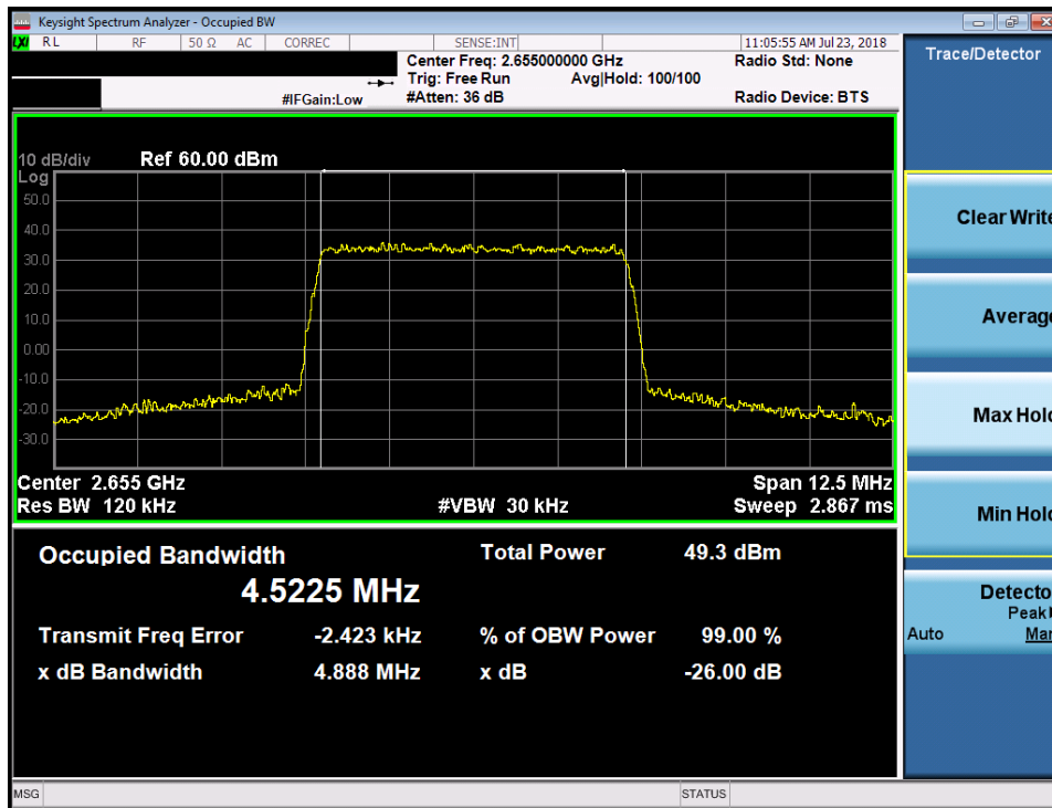
Plot 7-98. Occupied Bandwidth Plot (Band 7 - 5.0MHz 16-QAM)
