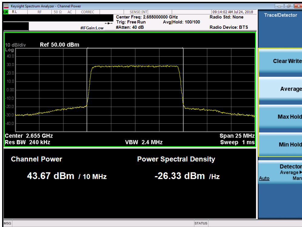
Plot 7-65. Maximum Conducted Power (Band 7 - 10.0MHz 16-QAM – Mid Channel)
