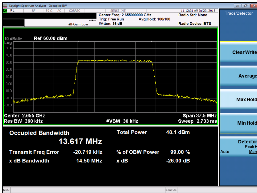
Plot 7-107. Occupied Bandwidth Plot (Band 7 - 15.0MHz 64-QAM)
