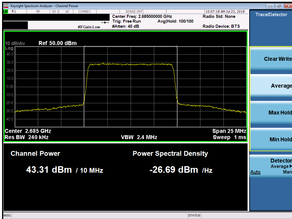
Plot 7-15. Maximum Conducted Power (Band 7 - 10.0MHz QPSK – High Channel)
