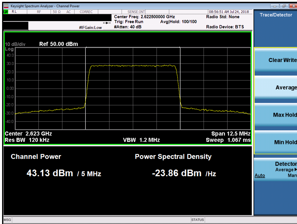
Plot 7-49. Maximum Conducted Power (Band 7 - 5.0MHz QPSK - Low Channel)
