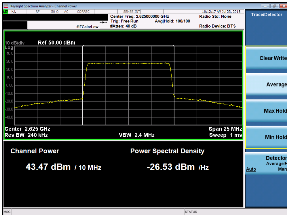
Plot 7-16. Maximum Conducted Power (Band 7 - 10.0MHz 16-QAM – Low Channel)
