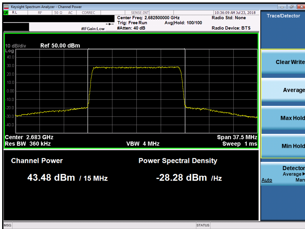
Plot 7-33. Maximum Conducted Power (Band 7 - 15.0MHz 64-QAM – High Channel)
