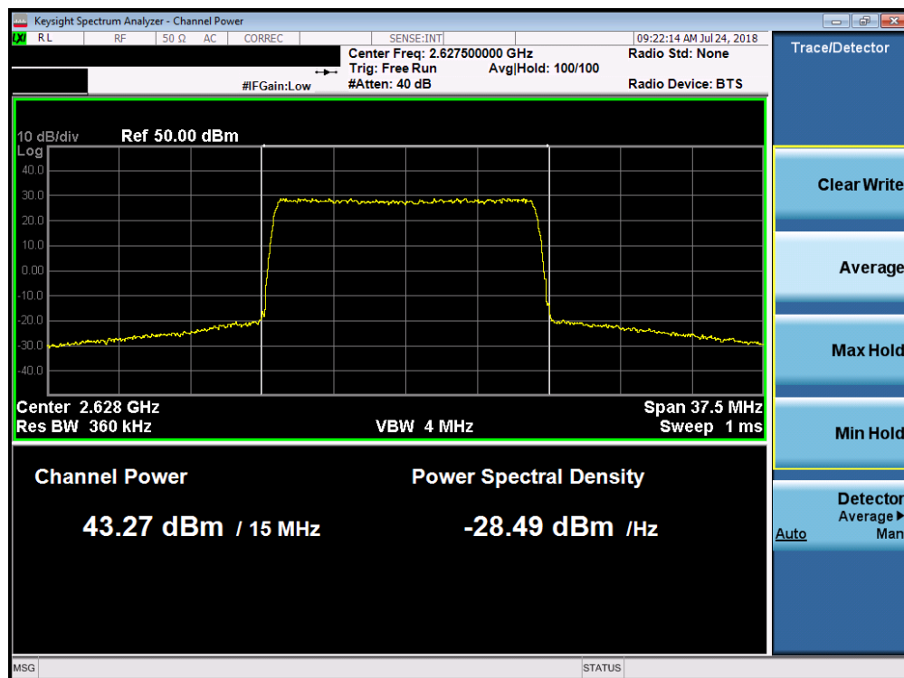
Plot 7-82. Maximum Conducted Power (Band 7 - 15.0MHz 256-QAM - Low Channel)
