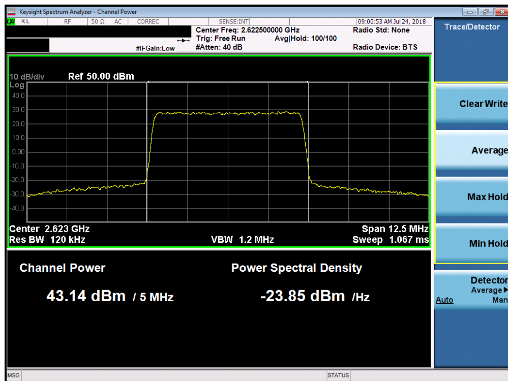
Plot 7-58. Maximum Conducted Power (Band 7 - 5.0MHz 256-QAM - Low Channel)
