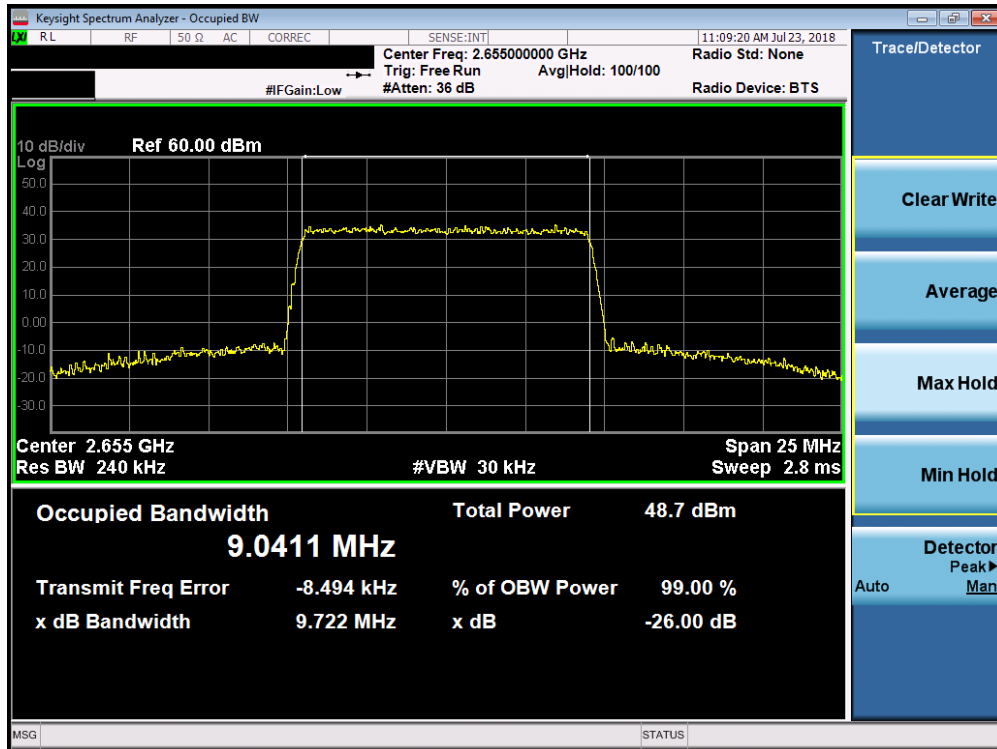
Plot 7-101. Occupied Bandwidth Plot (Band 7 - 10.0MHz QPSK)
