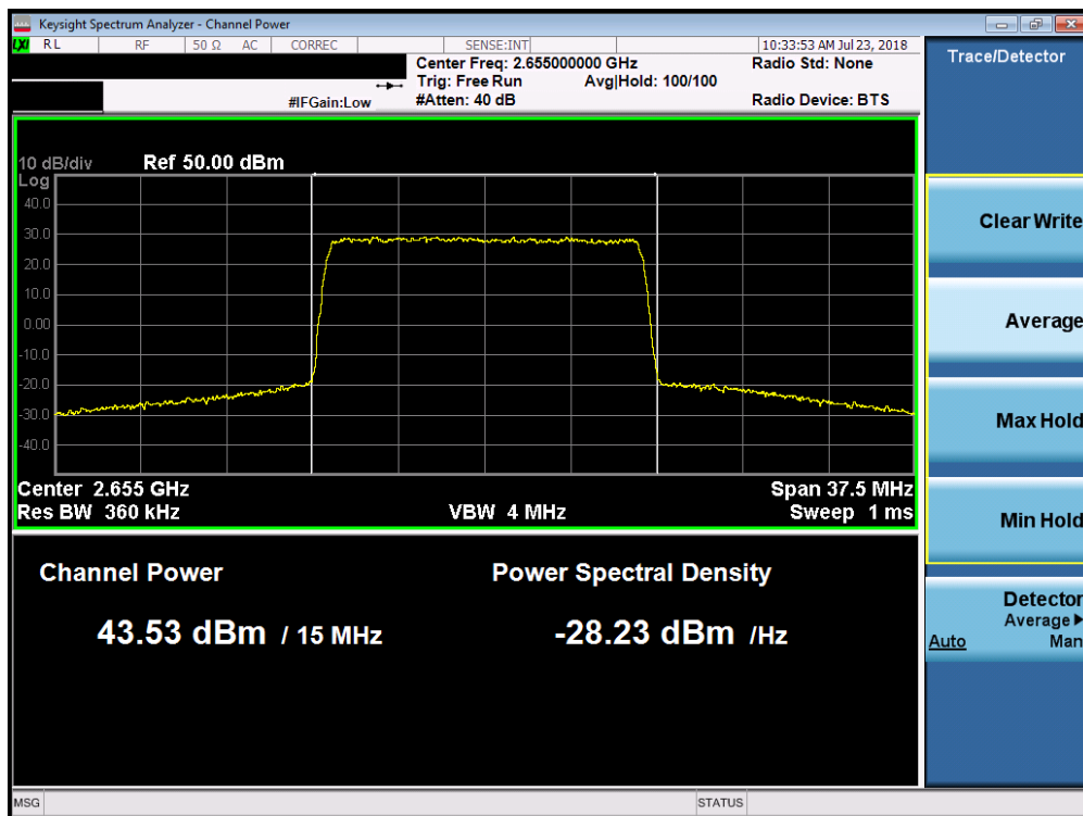
Plot 7-35. Maximum Conducted Power (Band 7 - 15.0MHz 256-QAM – Mid Channel)
