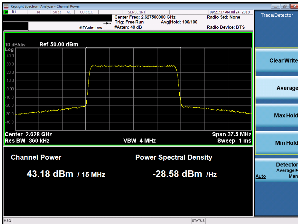
Plot 7-76. Maximum Conducted Power (Band 7 - 15.0MHz 16-QAM - Low Channel)
