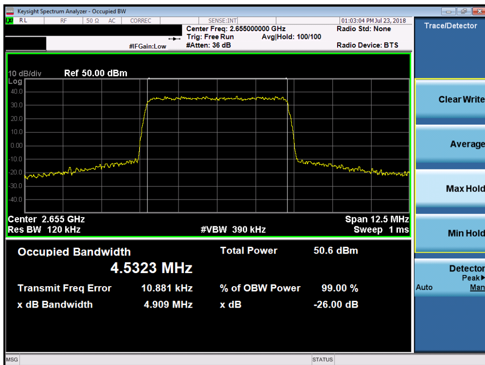
Plot 7-116. Occupied Bandwidth Plot (Band 7 - 5.0MHz 256-QAM)
