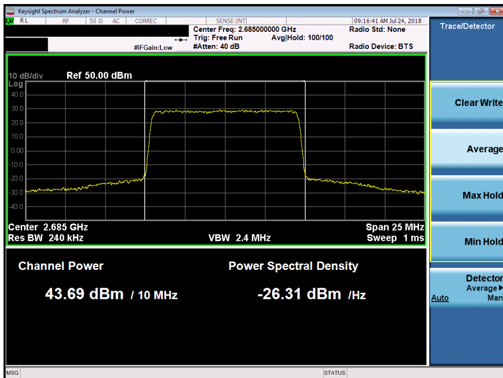
Plot 7-63. Maximum Conducted Power (Band 7 - 10.0MHz QPSK – High Channel)
