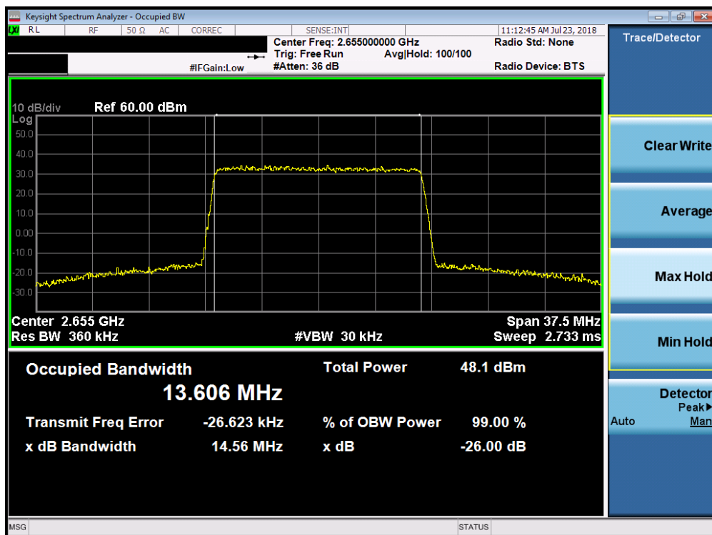
Plot 7-108. Occupied Bandwidth Plot (Band 7 - 15.0MHz 256-QAM)
