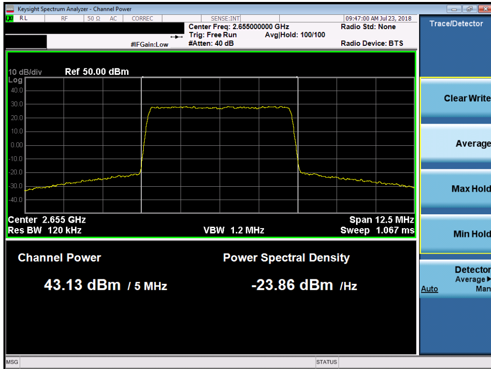
Plot 7-5. Maximum Conducted Power (Band 7 - 5.0MHz 16-QAM – Mid Channel)
