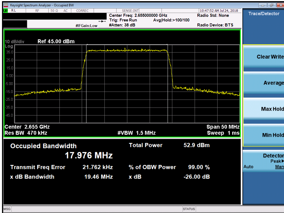
Plot 7-125. Occupied Bandwidth Plot (Band 7 - 20.0MHz QPSK)
