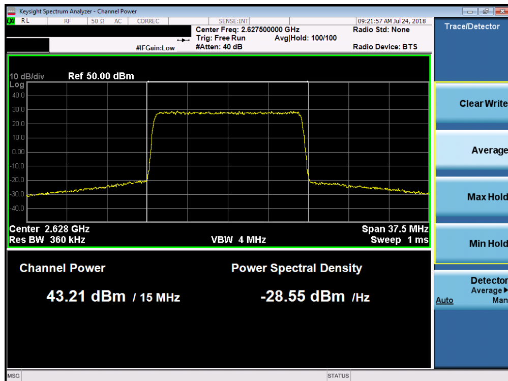
Plot 7-79. Maximum Conducted Power (Band 7 - 15.0MHz 64-QAM - Low Channel)
