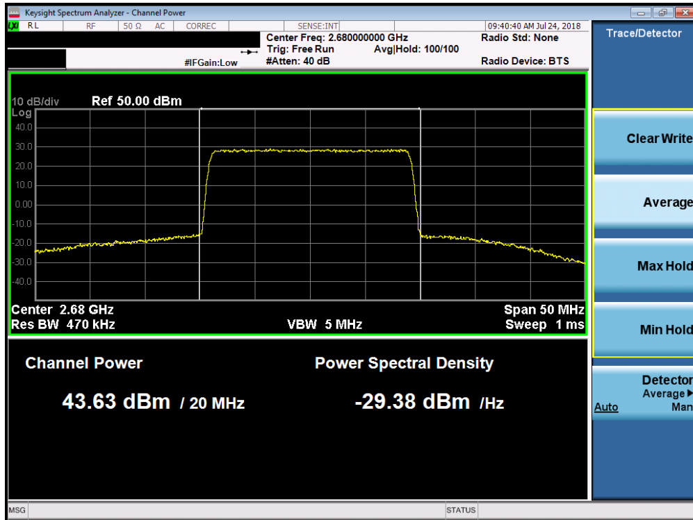
Plot 7-93. Maximum Conducted Power (Band 7 - 20.0MHz 64-QAM – High Channel)
