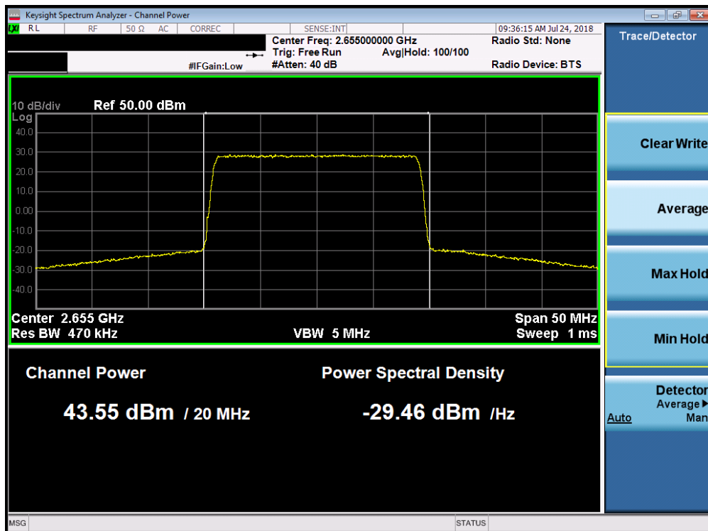
Plot 7-86. Maximum Conducted Power (Band 7 - 20.0MHz QPSK - Mid Channel)
