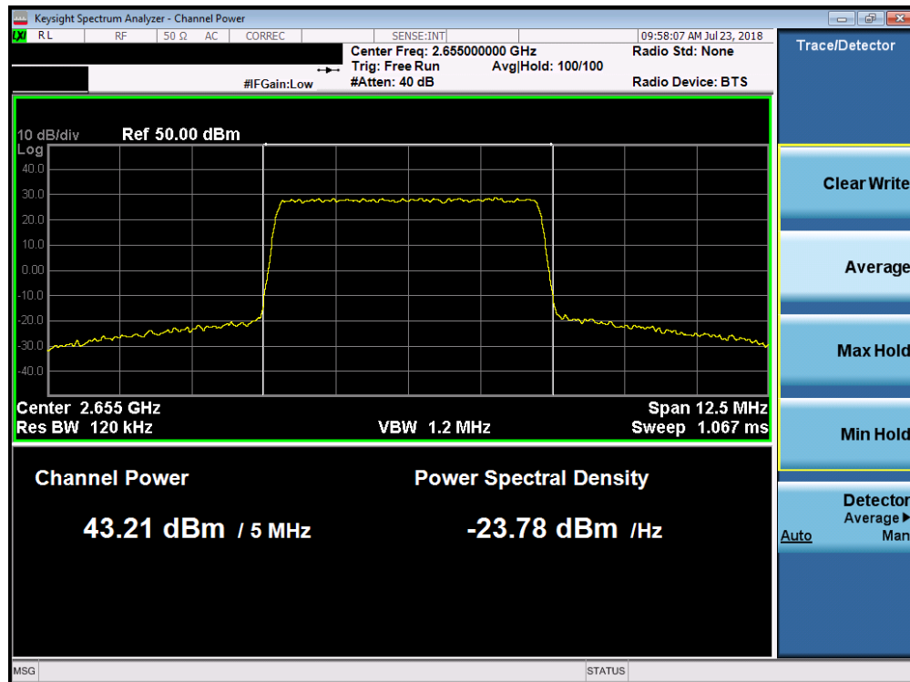
Plot 7-11. Maximum Conducted Power (Band 7 - 5.0MHz 256-QAM – Mid Channel)
