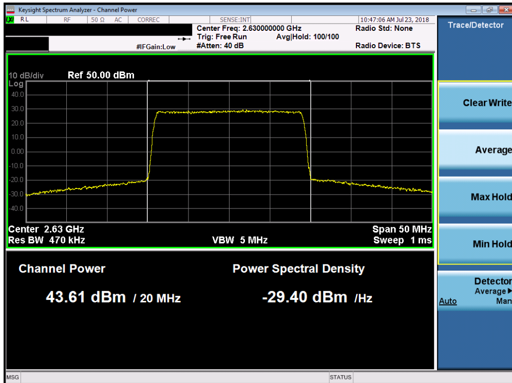
Plot 7-40. Maximum Conducted Power (Band 7 - 20.0MHz 16-QAM – Low Channel)
