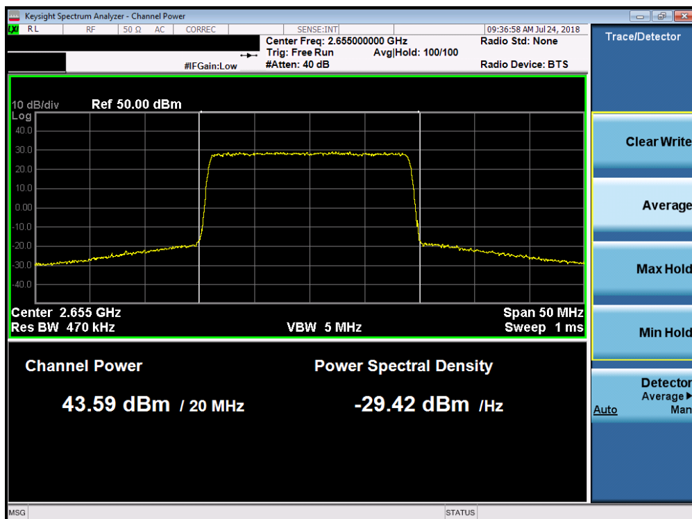
Plot 7-92. Maximum Conducted Power (Band 7 - 20.0MHz 64-QAM - Mid Channel)
