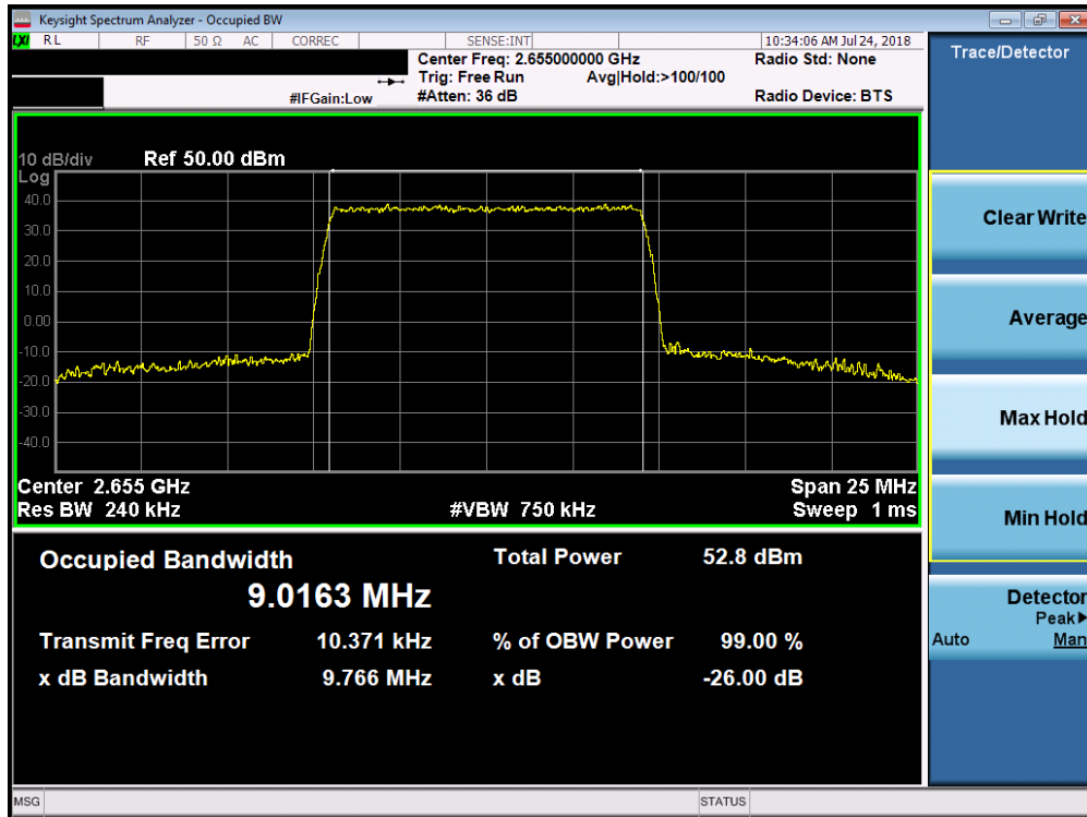
Plot 7-117. Occupied Bandwidth Plot (Band 7 - 10.0MHz QPSK)
