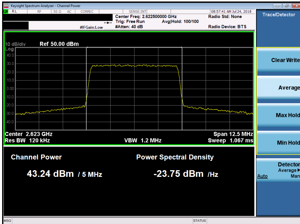
Plot 7-52. Maximum Conducted Power (Band 7 - 5.0MHz 16-QAM - Low Channel)
