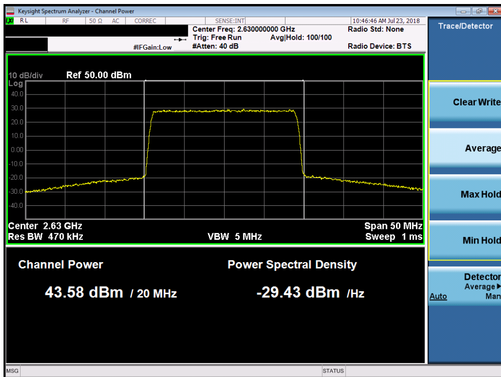
Plot 7-43. Maximum Conducted Power (Band 7 - 20.0MHz 64-QAM – Low Channel)
