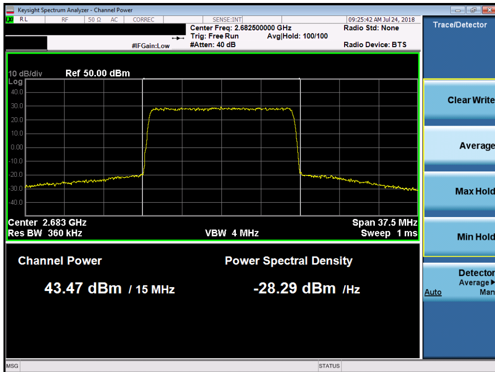
Plot 7-75. Maximum Conducted Power (Band 7 - 15.0MHz QPSK – High Channel)
