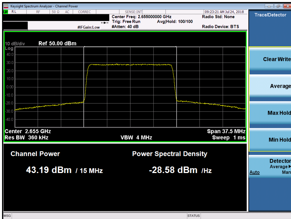
Plot 7-74. Maximum Conducted Power (Band 7 - 15.0MHz QPSK - Mid Channel)
