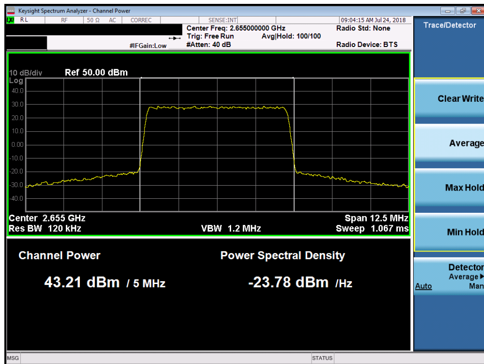
Plot 7-59. Maximum Conducted Power (Band 7 - 5.0MHz 256-QAM – Mid Channel)
