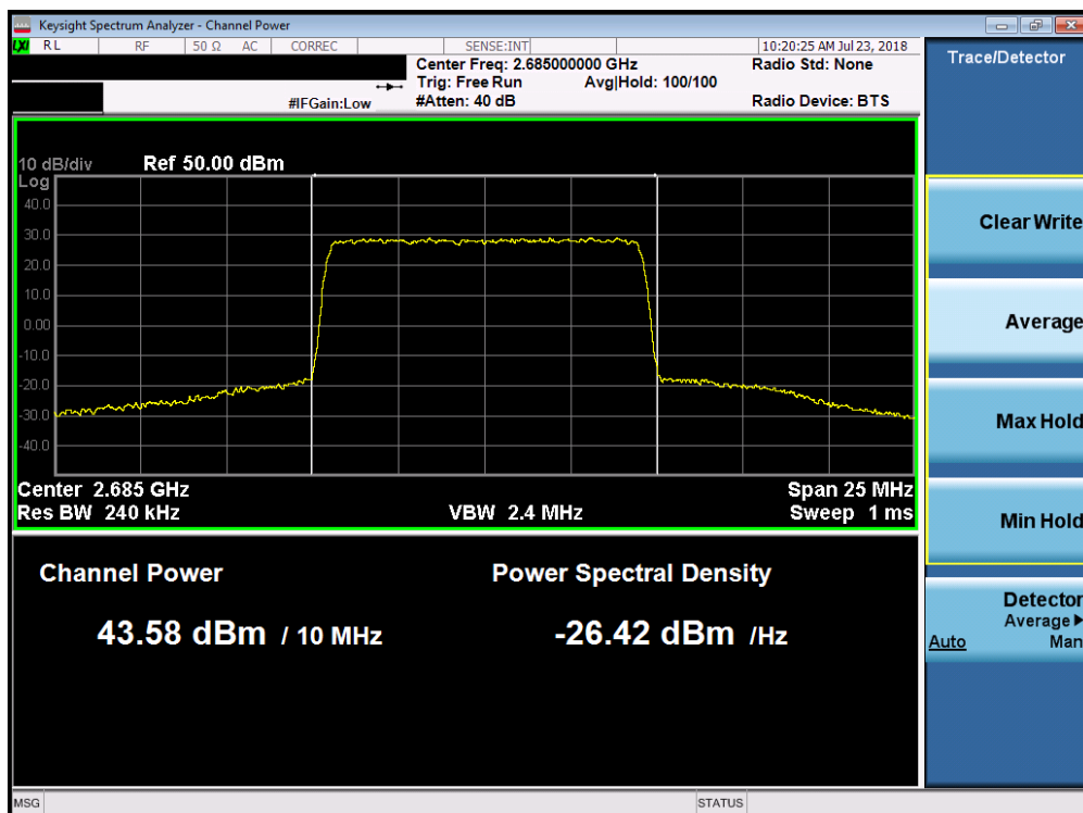
Plot 7-18. Maximum Conducted Power (Band 7 - 10.0MHz 16-QAM – High Channel)
