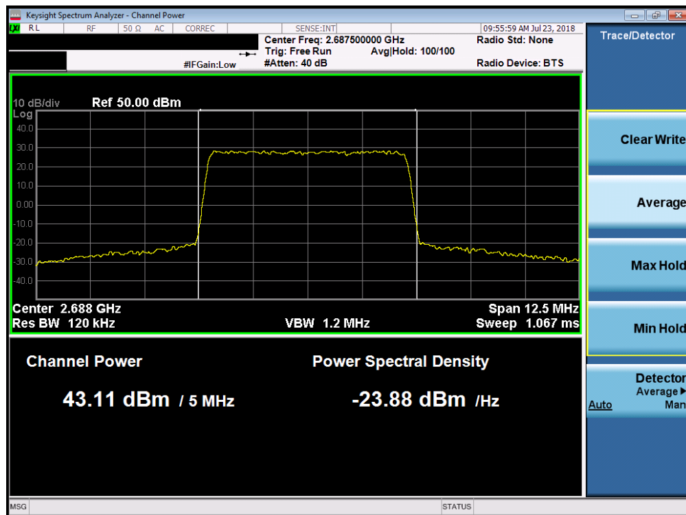
Plot 7-9. Maximum Conducted Power (Band 7 - 5.0MHz 64-QAM – High Channel)
