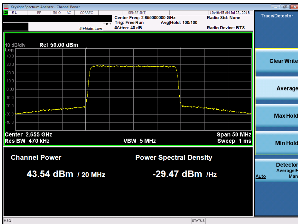
Plot 7-44. Maximum Conducted Power (Band 7 - 20.0MHz 64-QAM – Mid Channel)
