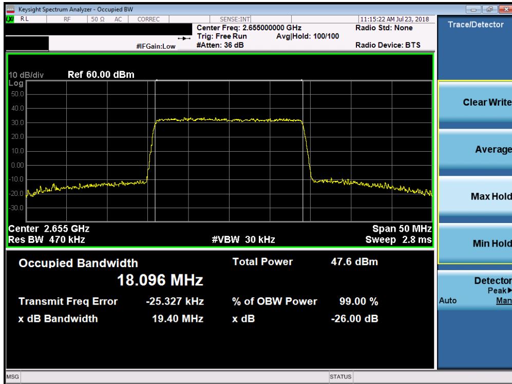
Plot 7-109. Occupied Bandwidth Plot (Band 7 - 20.0MHz QPSK)
