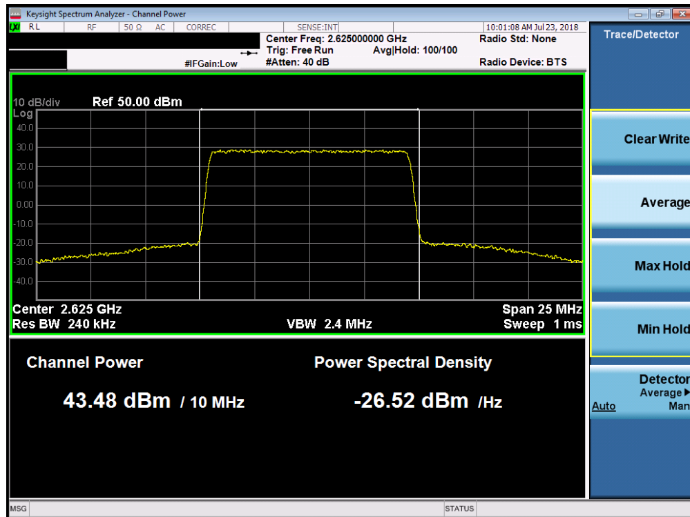
Plot 7-13. Maximum Conducted Power (Band 7 - 10.0MHz QPSK – Low Channel)
