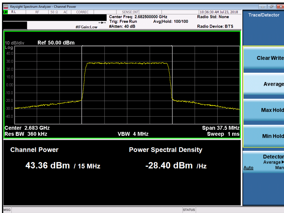
Plot 7-36. Maximum Conducted Power (Band 7 - 15.0MHz 256-QAM – High Channel)
