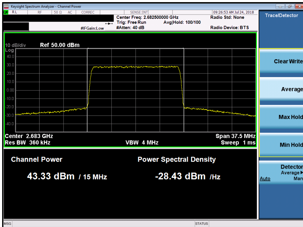
Plot 7-78. Maximum Conducted Power (Band 7 - 15.0MHz 16-QAM – High Channel)
