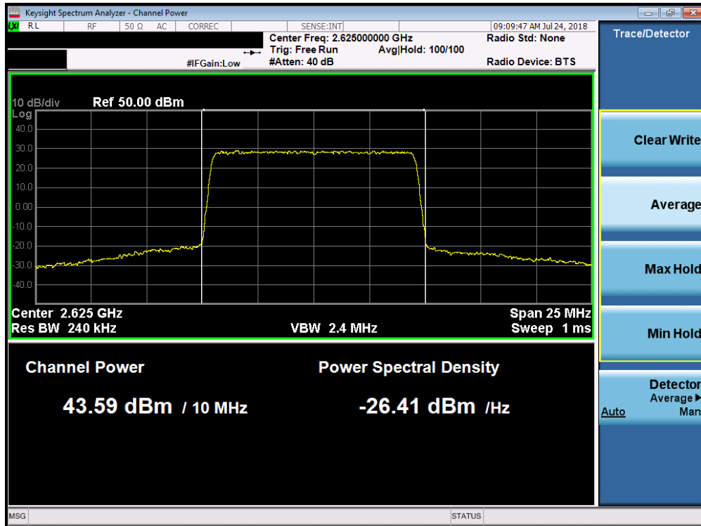
Plot 7-61. Maximum Conducted Power (Band 7 - 10.0MHz QPSK - Low Channel)
