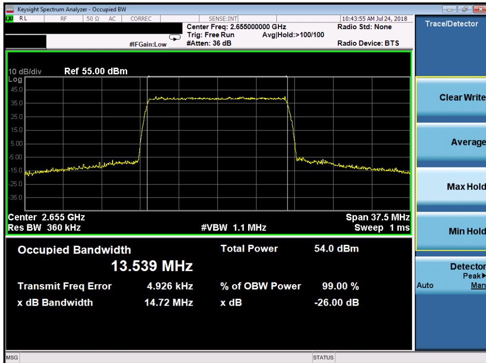
Plot 7-124. Occupied Bandwidth Plot (Band 7 - 15.0MHz 256-QAM)
