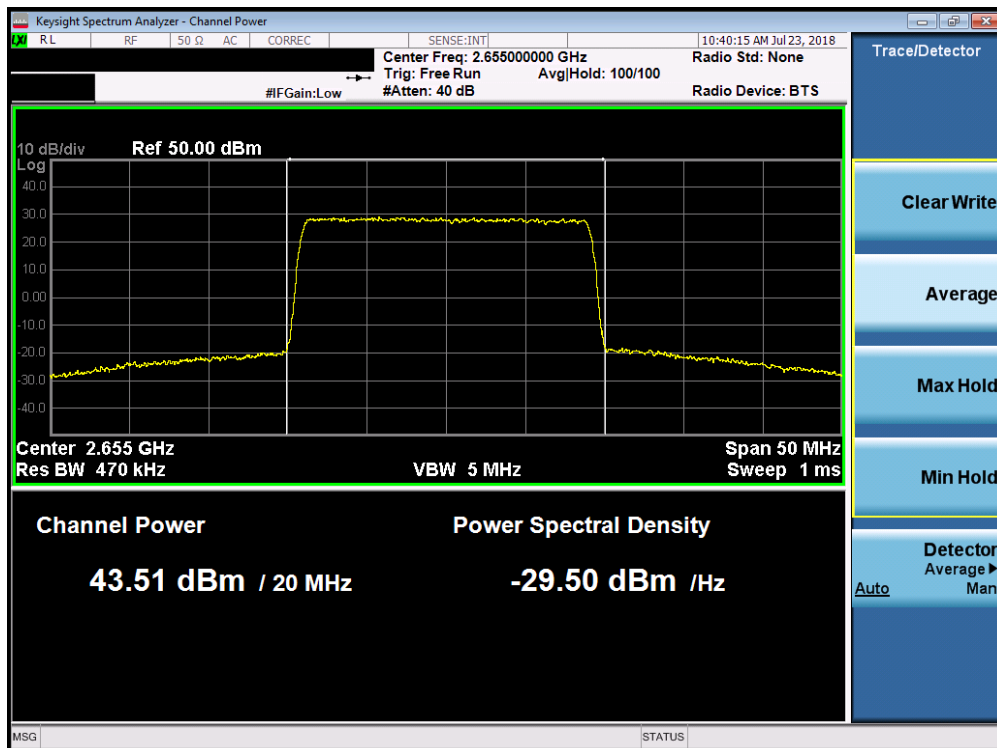
Plot 7-38. Maximum Conducted Power (Band 7 - 20.0MHz QPSK – Mid Channel)
