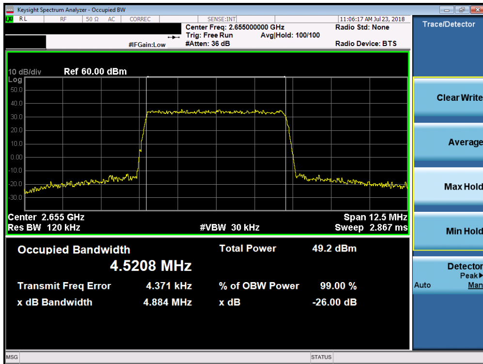
Plot 7-99. Occupied Bandwidth Plot (Band 7 - 5.0MHz 64-QAM)
