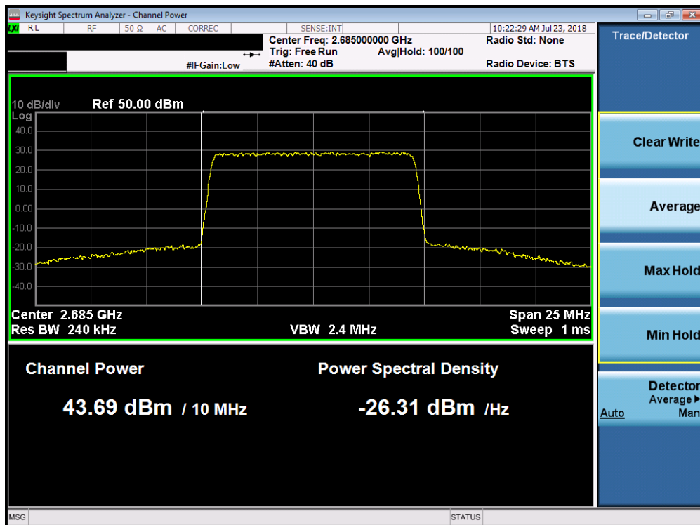
Plot 7-24. Maximum Conducted Power (Band 7 - 10.0MHz 256-QAM – High Channel)
