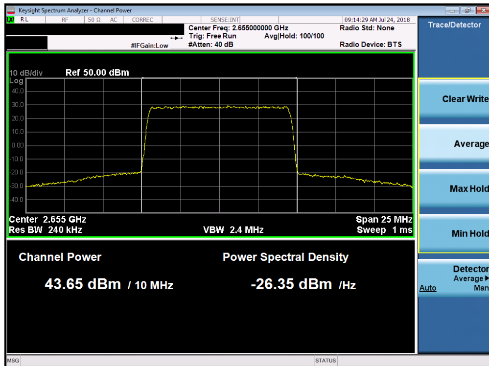
Plot 7-68. Maximum Conducted Power (Band 7 - 10.0MHz 64-QAM - Mid Channel)
