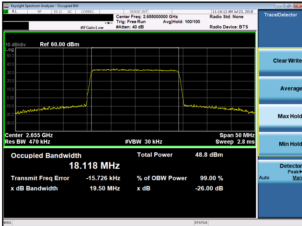
Plot 7-110. Occupied Bandwidth Plot (Band 7 - 20.0MHz 16-QAM)
