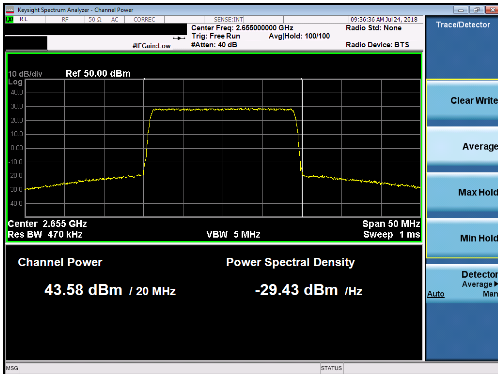
Plot 7-89. Maximum Conducted Power (Band 7 - 20.0MHz 16-QAM – Mid Channel)
