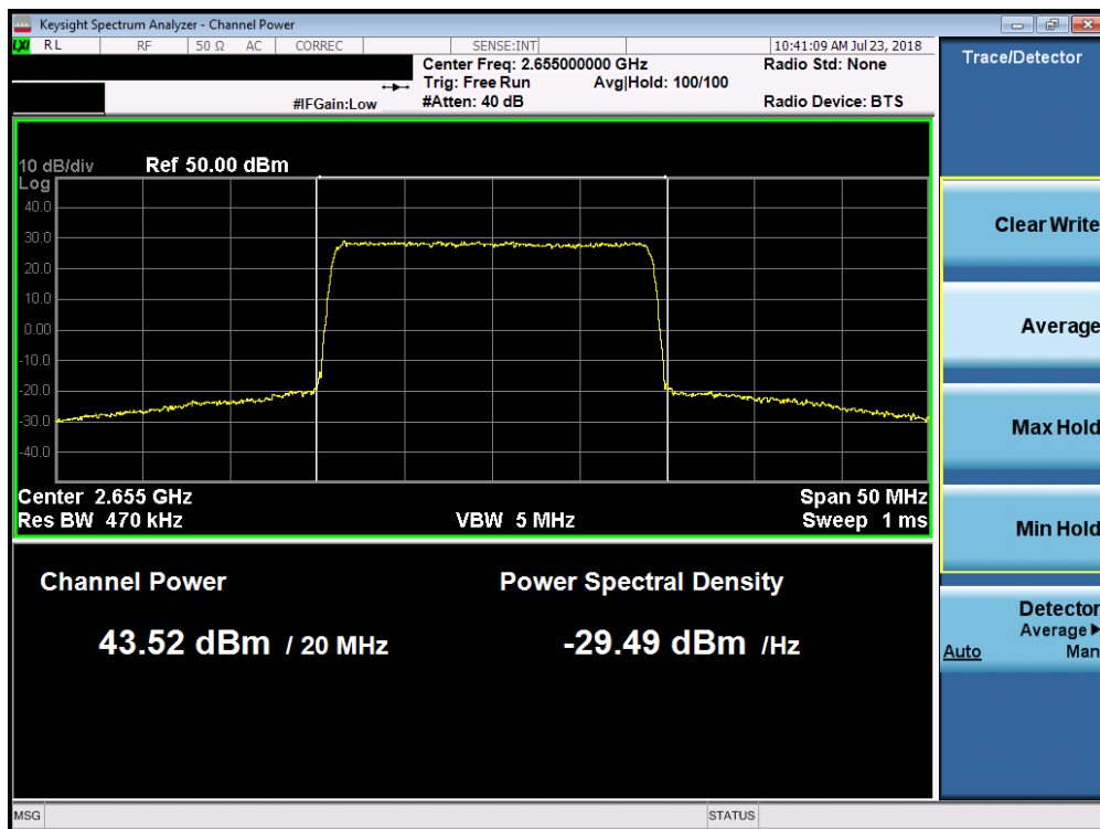
Plot 7-47. Maximum Conducted Power (Band 7 - 20.0MHz 256-QAM – Mid Channel)
