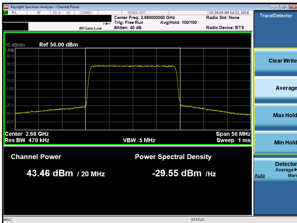
Plot 7-48. Maximum Conducted Power (Band 7 - 20.0MHz 256-QAM – High Channel)
