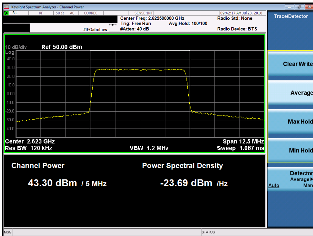
Plot 7-1. Maximum Conducted Power (Band 7 - 5.0MHz QPSK – Low Channel)
