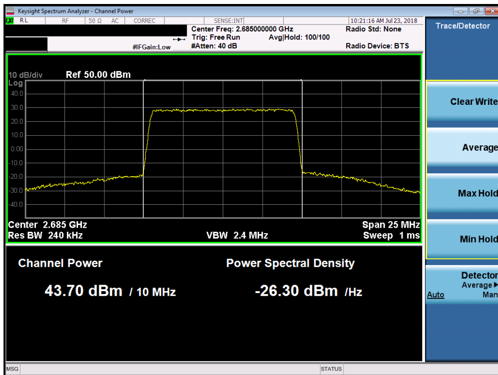
Plot 7-21. Maximum Conducted Power (Band 7 - 10.0MHz 64-QAM – High Channel)
