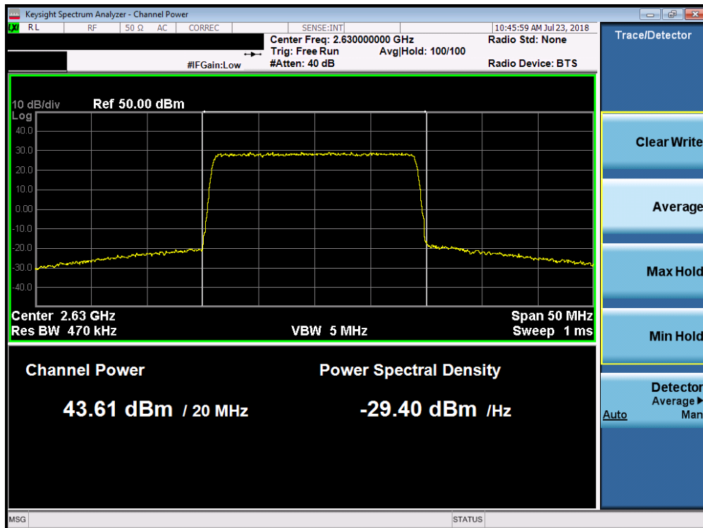
Plot 7-37. Maximum Conducted Power (Band 7 - 20.0MHz QPSK – Low Channel)
