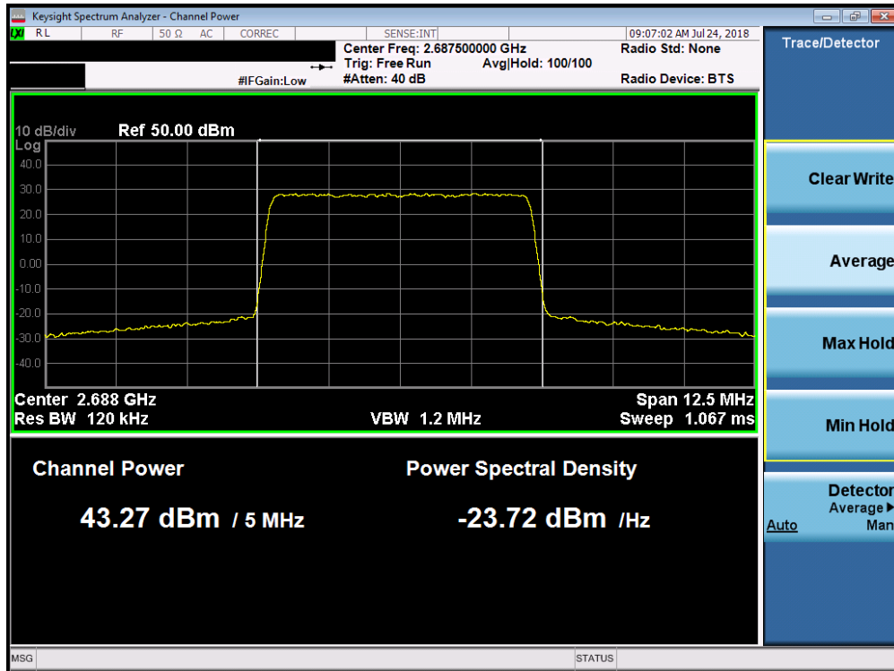
Plot 7-51. Maximum Conducted Power (Band 7 - 5.0MHz QPSK – High Channel)
