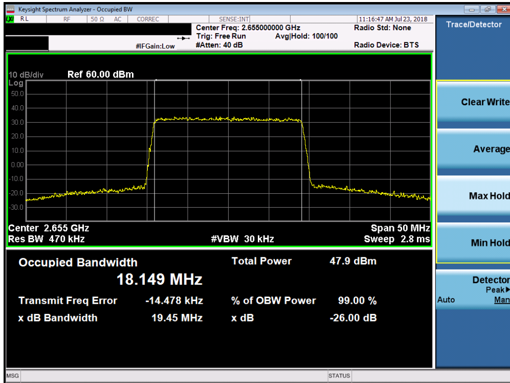
Plot 7-111. Occupied Bandwidth Plot (Band 7 - 20.0MHz 64-QAM)
