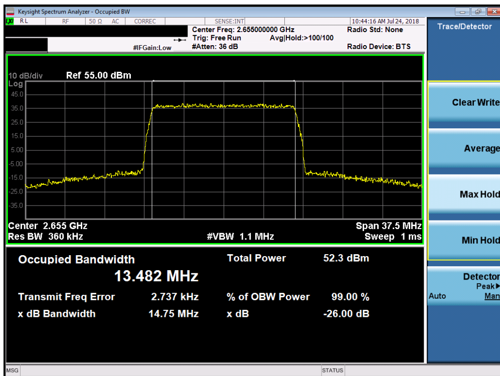
Plot 7-122. Occupied Bandwidth Plot (Band 7 - 15.0MHz 16-QAM)
