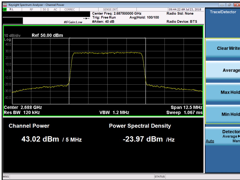
Plot 7-3. Maximum Conducted Power (Band 7 - 5.0MHz QPSK – High Channel)
