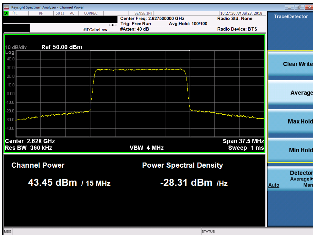
Plot 7-34. Maximum Conducted Power (Band 7 - 15.0MHz 256-QAM – Low Channel)
