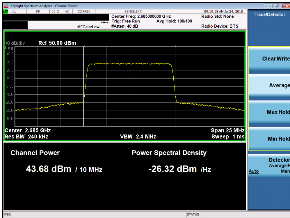
Plot 7-69. Maximum Conducted Power (Band 7 - 10.0MHz 64-QAM – High Channel)
