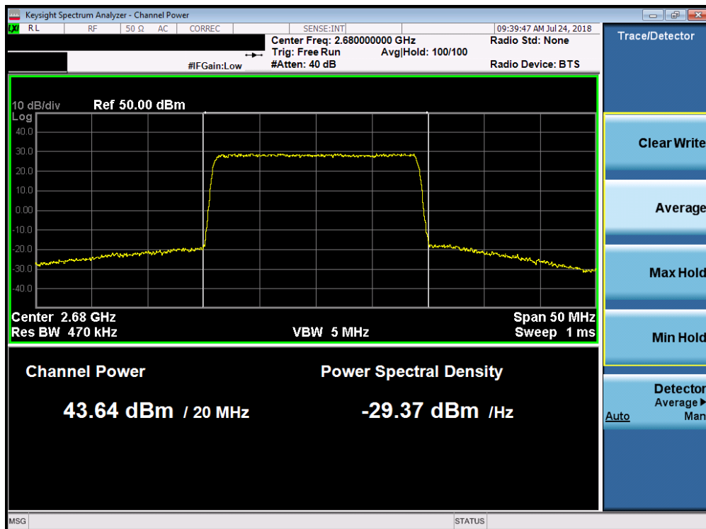
Plot 7-90. Maximum Conducted Power (Band 7 - 20.0MHz 16-QAM – High Channel)
