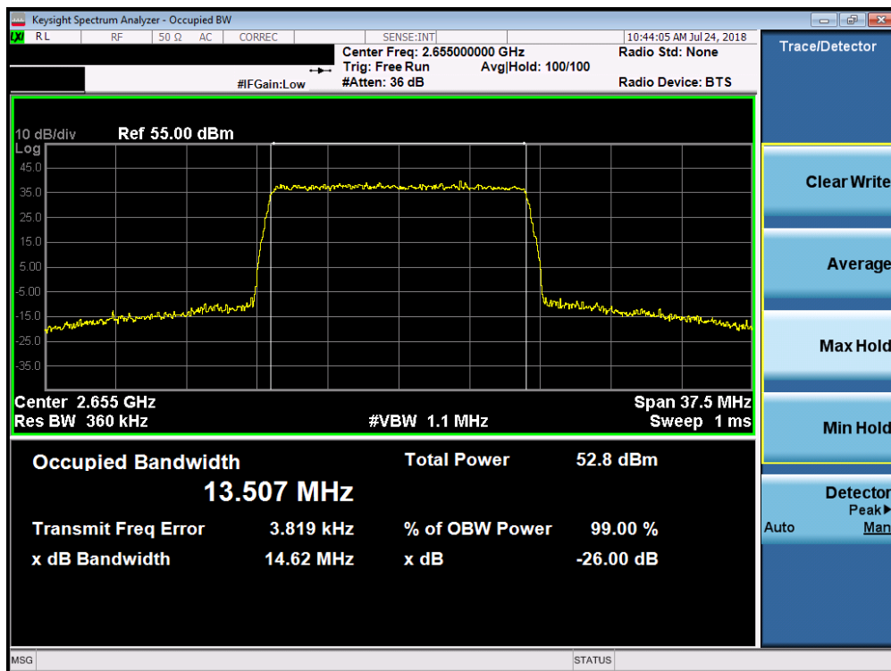
Plot 7-121. Occupied Bandwidth Plot (Band 7 - 15.0MHz QPSK)
