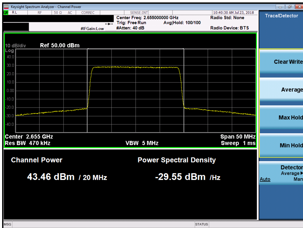
Plot 7-41. Maximum Conducted Power (Band 7 - 20.0MHz 16-QAM – Mid Channel)
