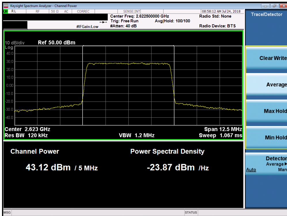
Plot 7-55. Maximum Conducted Power (Band 7 - 5.0MHz 64-QAM - Low Channel)
