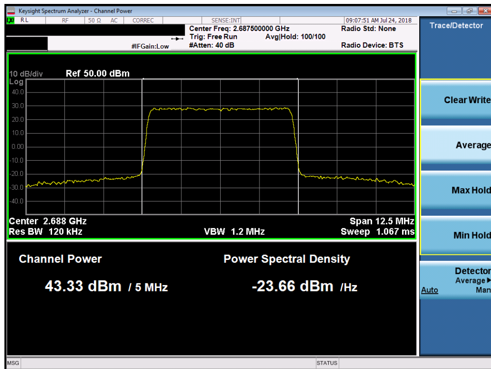
Plot 7-57. Maximum Conducted Power (Band 7 - 5.0MHz 64-QAM – High Channel)
