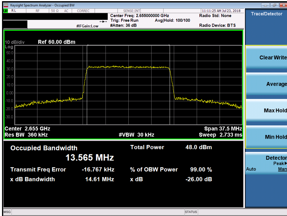
Plot 7-105. Occupied Bandwidth Plot (Band 7 - 15.0MHz QPSK)
