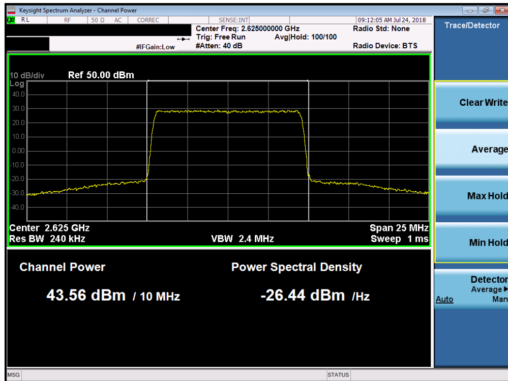
Plot 7-67. Maximum Conducted Power (Band 7 - 10.0MHz 64-QAM - Low Channel)
