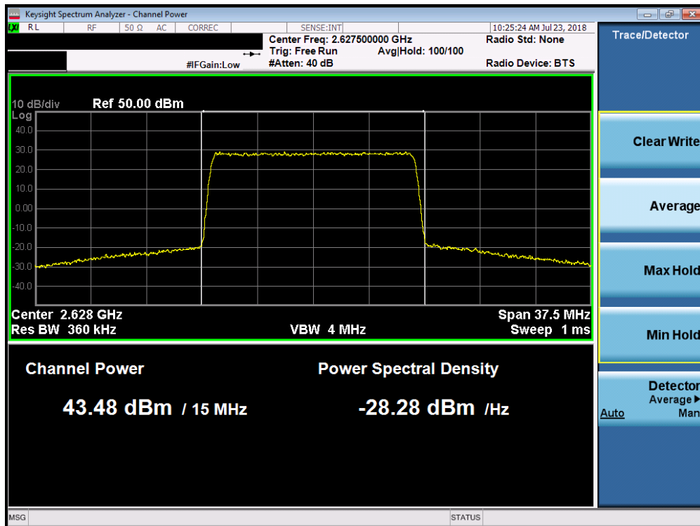
Plot 7-31. Maximum Conducted Power (Band 7 - 15.0MHz 64-QAM – Low Channel)
