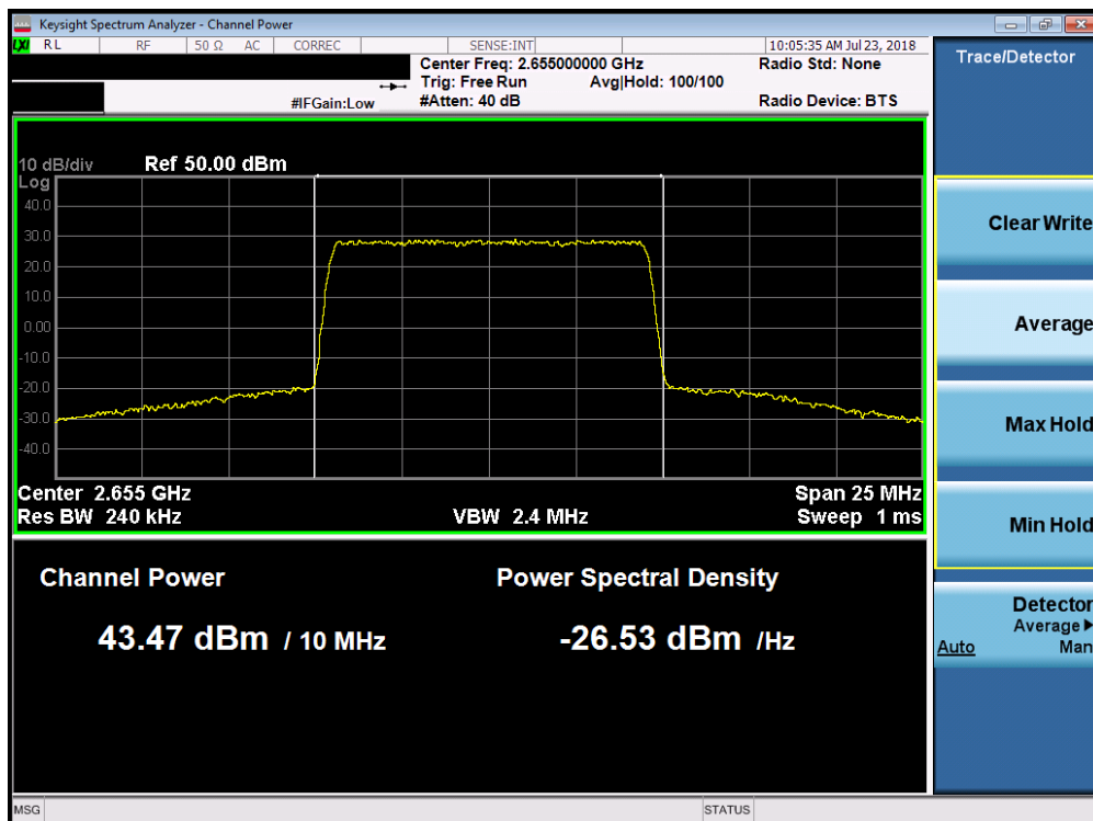
Plot 7-17. Maximum Conducted Power (Band 7 - 10.0MHz 16-QAM – Mid Channel)
