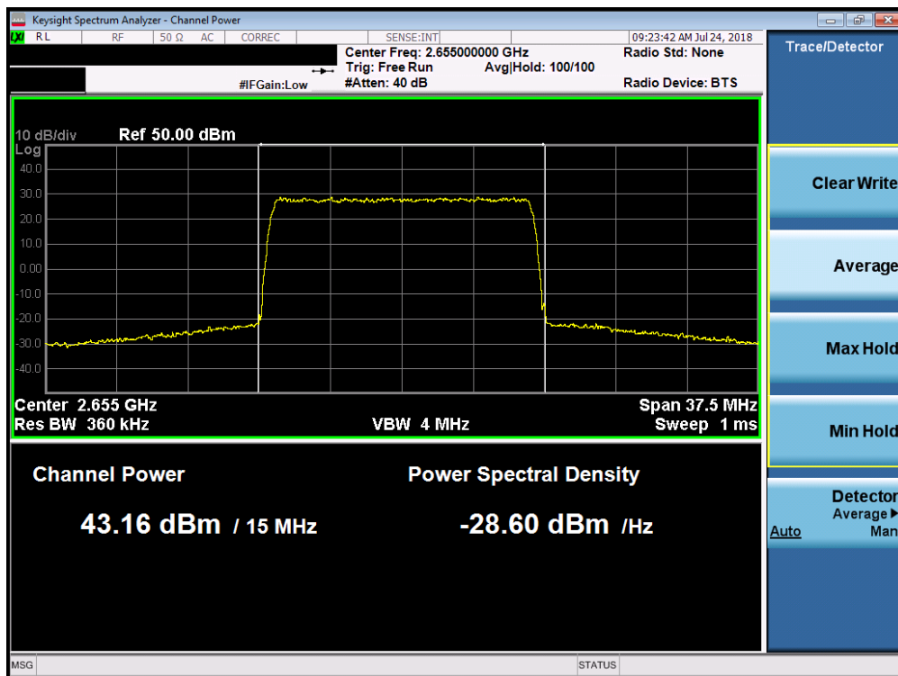
Plot 7-77. Maximum Conducted Power (Band 7 - 15.0MHz 16-QAM – Mid Channel)
