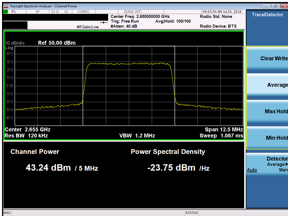
Plot 7-56. Maximum Conducted Power (Band 7 - 5.0MHz 64-QAM – Mid Channel)
