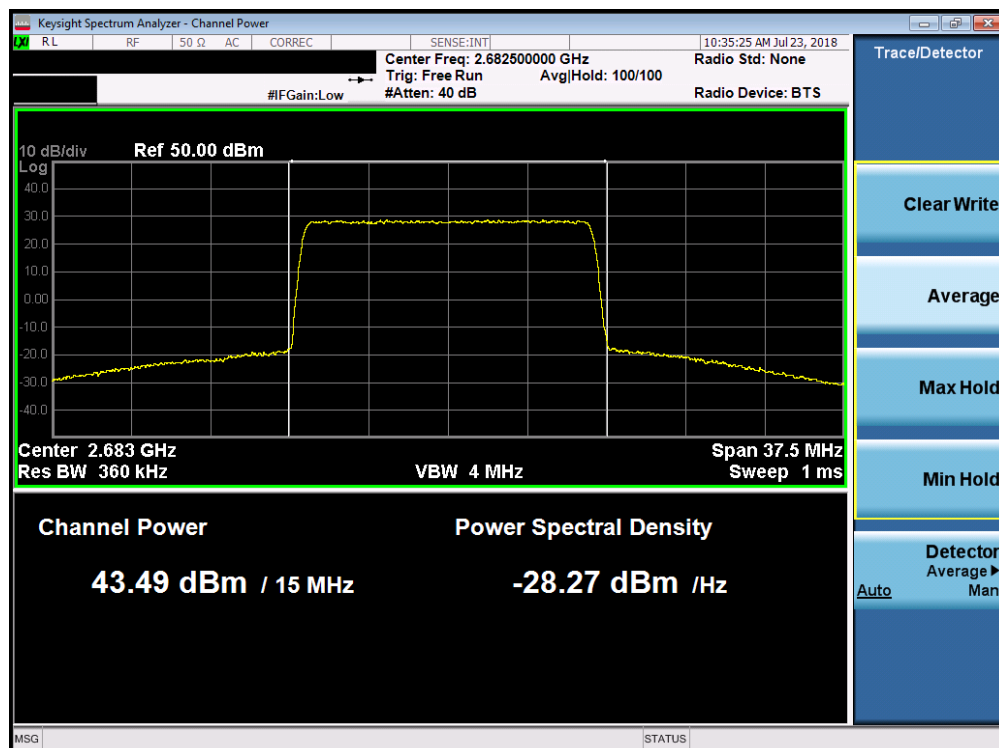
Plot 7-30. Maximum Conducted Power (Band 7 - 15.0MHz 16-QAM – High Channel)
