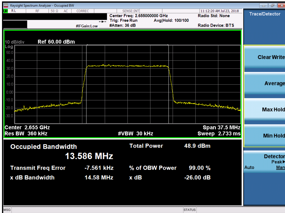
Plot 7-106. Occupied Bandwidth Plot (Band 7 - 15.0MHz 16-QAM)
