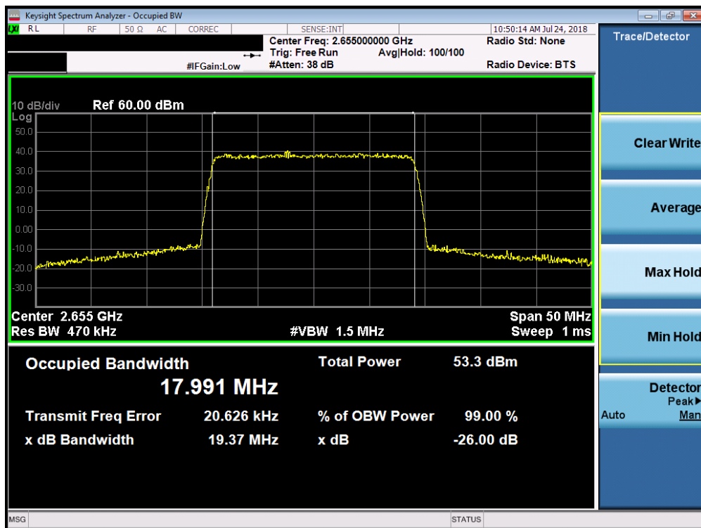
Plot 7-127. Occupied Bandwidth Plot (Band 7 - 20.0MHz 64-QAM)
