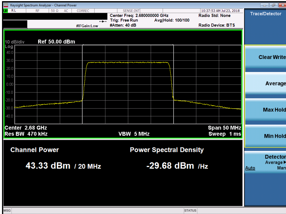
Plot 7-39. Maximum Conducted Power (Band 7 - 20.0MHz QPSK – High Channel)
