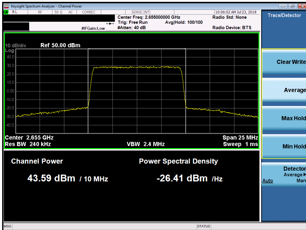
Plot 7-23. Maximum Conducted Power (Band 7 - 10.0MHz 256-QAM – Mid Channel)
