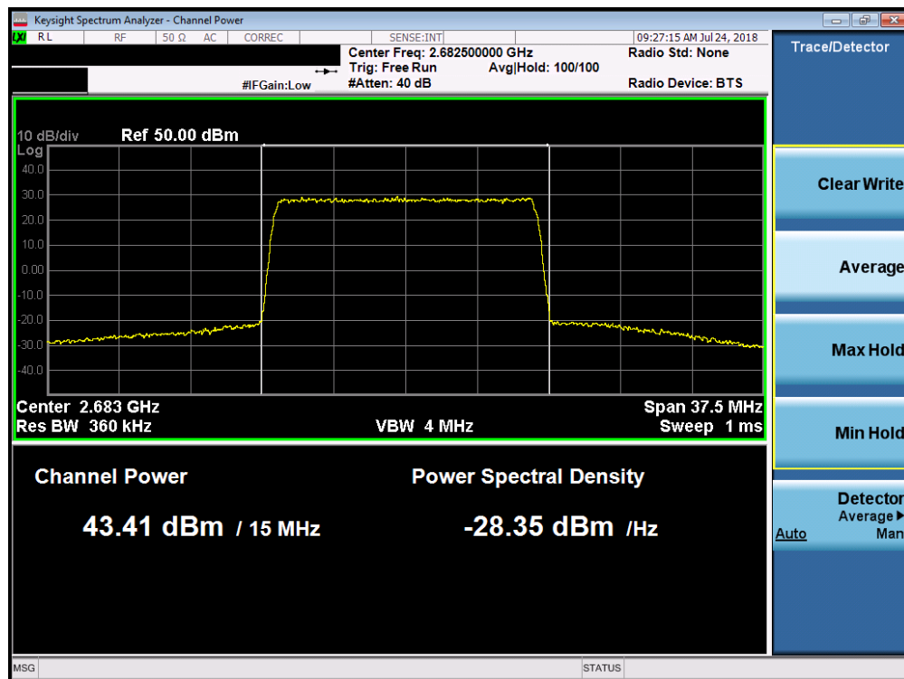
Plot 7-81. Maximum Conducted Power (Band 7 - 15.0MHz 64-QAM – High Channel)
