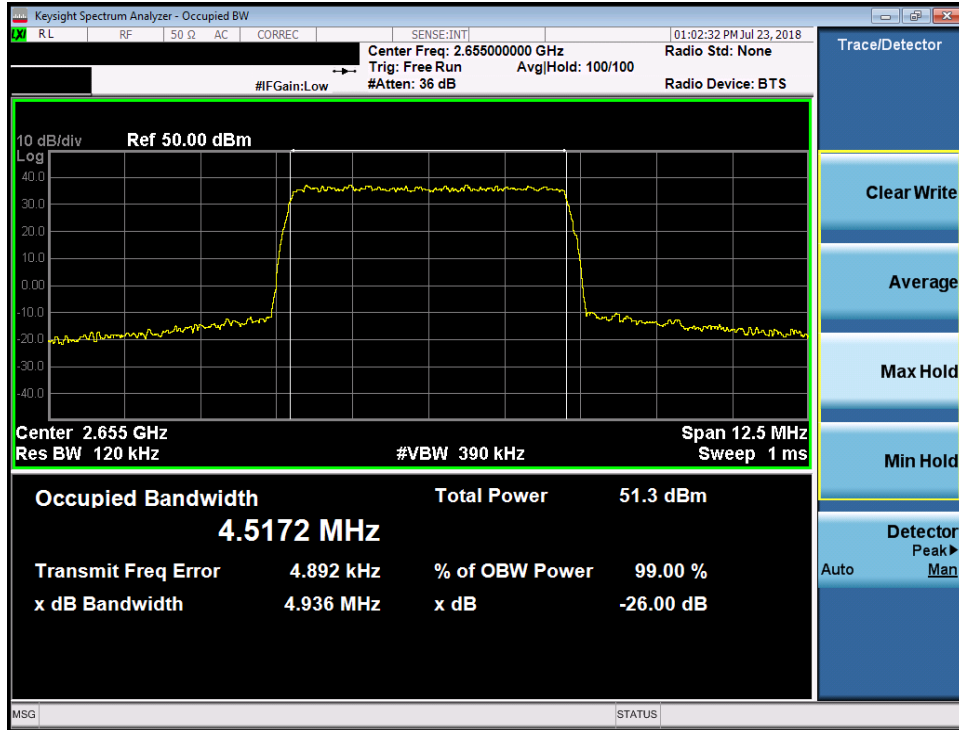
Plot 7-113. Occupied Bandwidth Plot (Band 7 - 5.0MHz QPSK)
