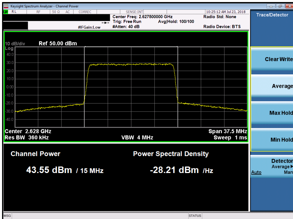
Plot 7-28. Maximum Conducted Power (Band 7 - 15.0MHz 16-QAM – Low Channel)
