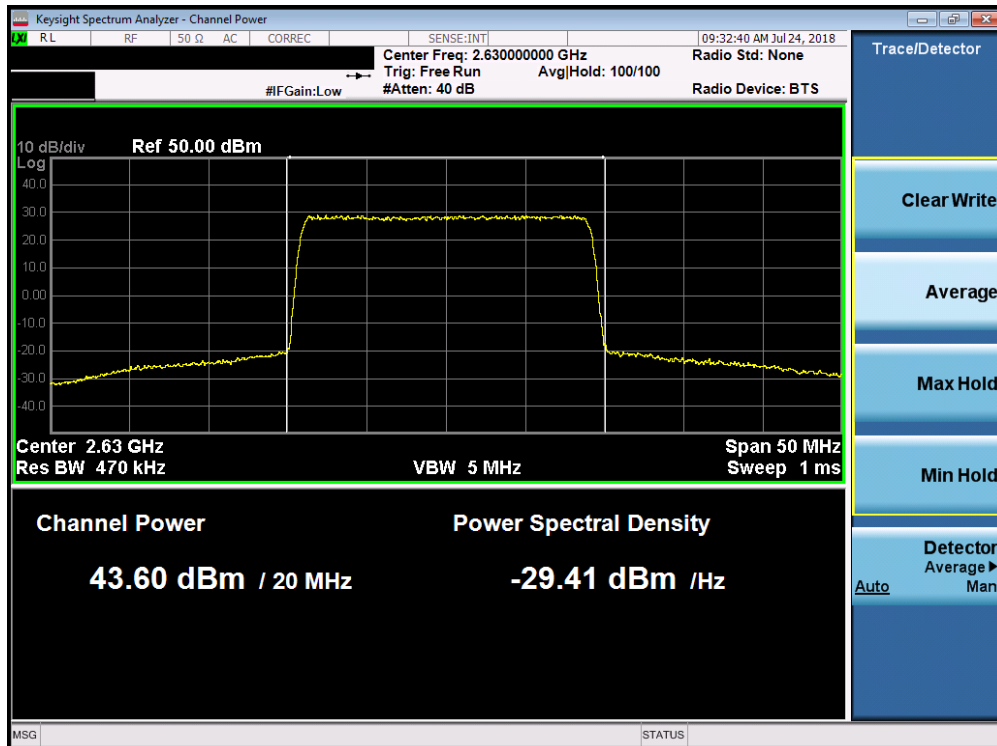
Plot 7-94. Maximum Conducted Power (Band 7 - 20.0MHz 256-QAM - Low Channel)
