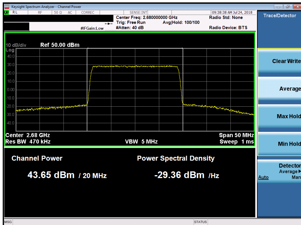
Plot 7-87. Maximum Conducted Power (Band 7 - 20.0MHz QPSK – High Channel)
