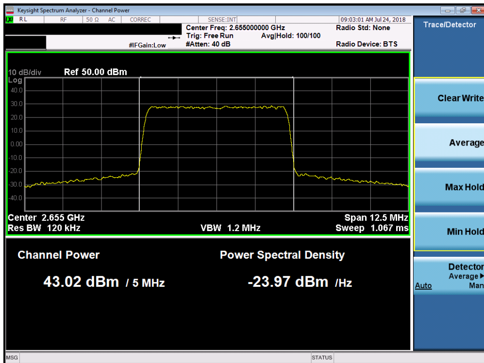
Plot 7-50. Maximum Conducted Power (Band 7 - 5.0MHz QPSK - Mid Channel)
