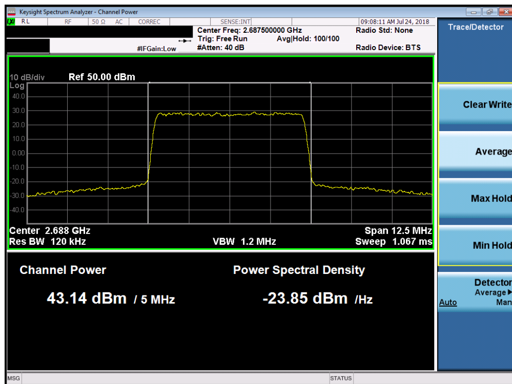
Plot 7-60. Maximum Conducted Power (Band 7 - 5.0MHz 256-QAM – High Channel)
