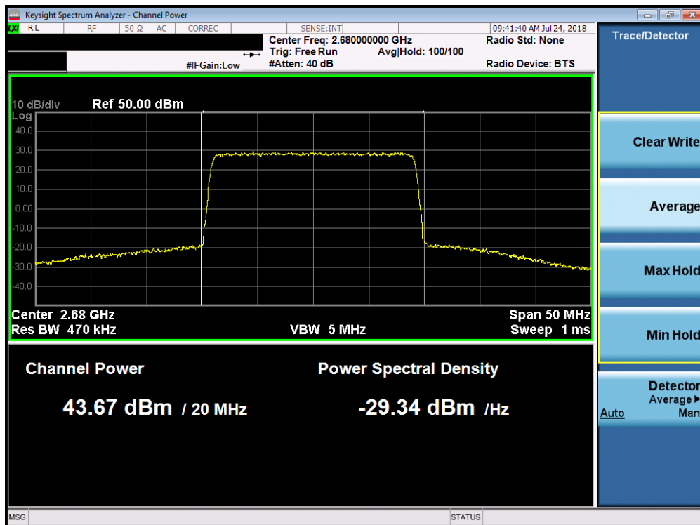
Plot 7-96. Maximum Conducted Power (Band 7 - 20.0MHz 256-QAM – High Channel)
