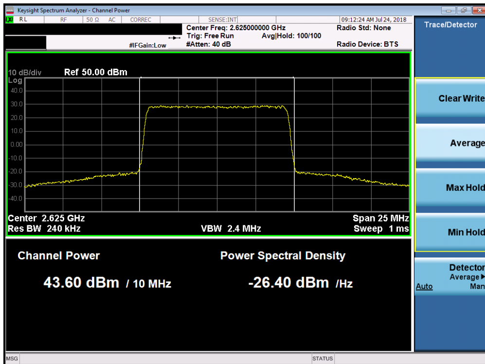
Plot 7-70. Maximum Conducted Power (Band 7 - 10.0MHz 256-QAM - Low Channel)
