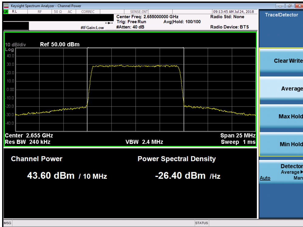
Plot 7-62. Maximum Conducted Power (Band 7 - 10.0MHz QPSK - Mid Channel)
