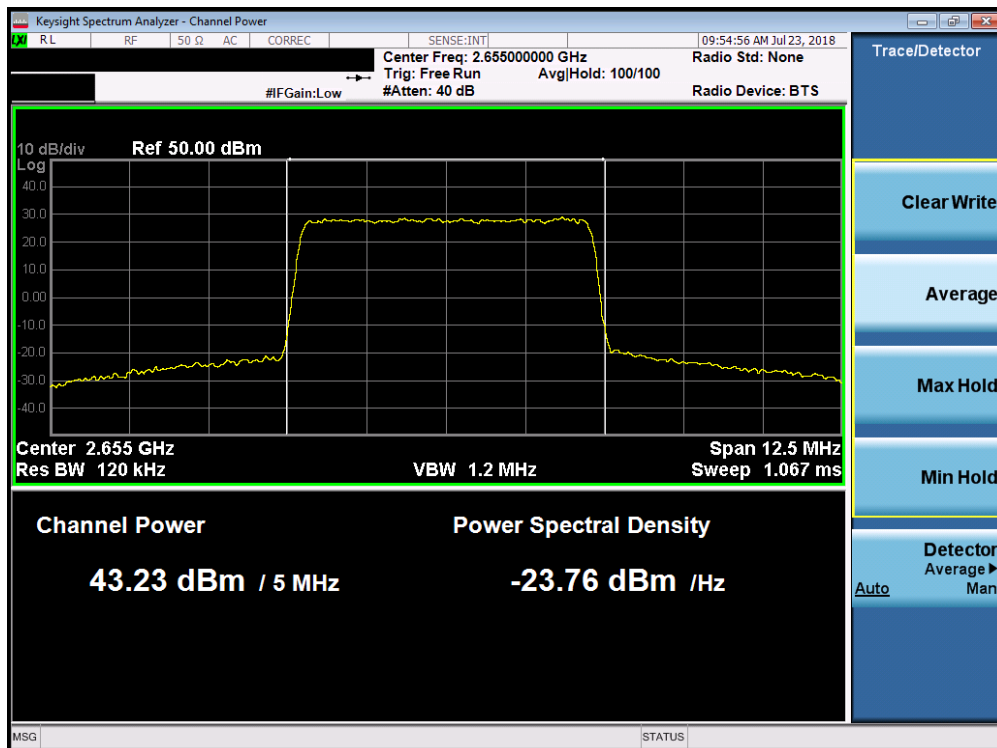
Plot 7-8. Maximum Conducted Power (Band 7 - 5.0MHz 64-QAM – Mid Channel)
