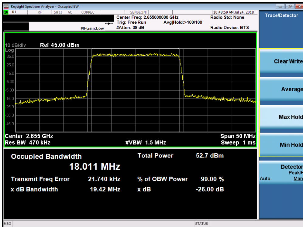
Plot 7-126. Occupied Bandwidth Plot (Band 7 - 20.0MHz 16-QAM)
