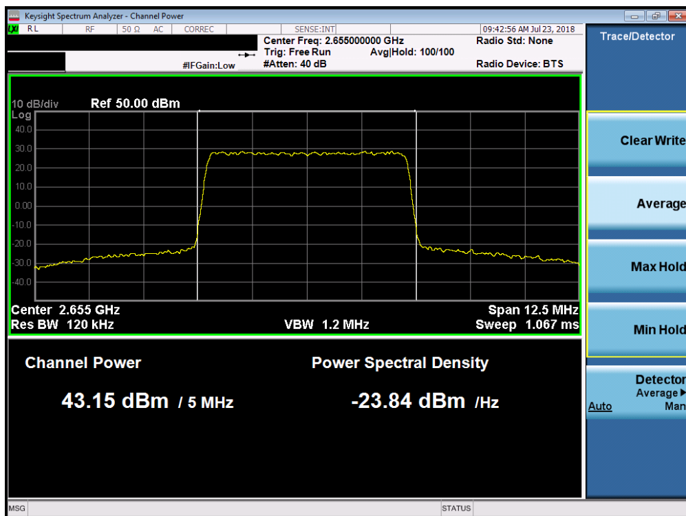
Plot 7-2. Maximum Conducted Power (Band 7 - 5.0MHz QPSK – Mid Channel)
