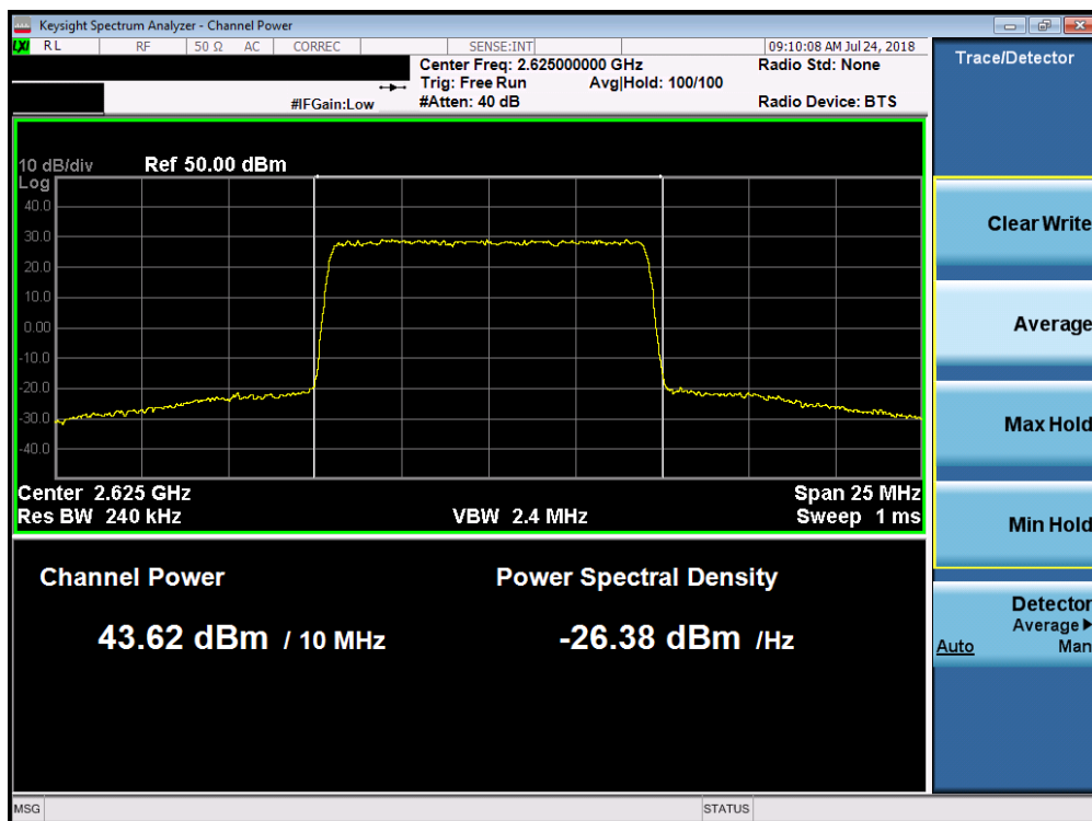
Plot 7-64. Maximum Conducted Power (Band 7 - 10.0MHz 16-QAM - Low Channel)
