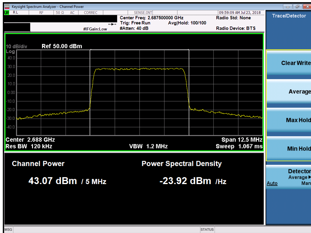
Plot 7-12. Maximum Conducted Power (Band 7 - 5.0MHz 256-QAM – High Channel)
