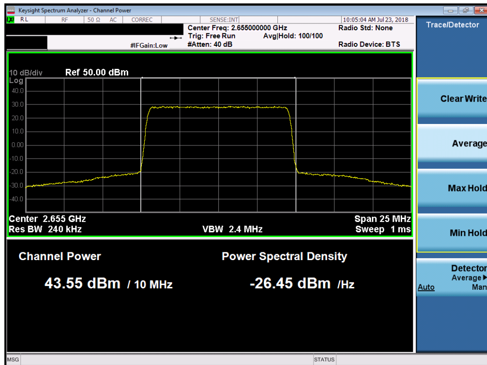
Plot 7-14. Maximum Conducted Power (Band 7 - 10.0MHz QPSK – Mid Channel)
