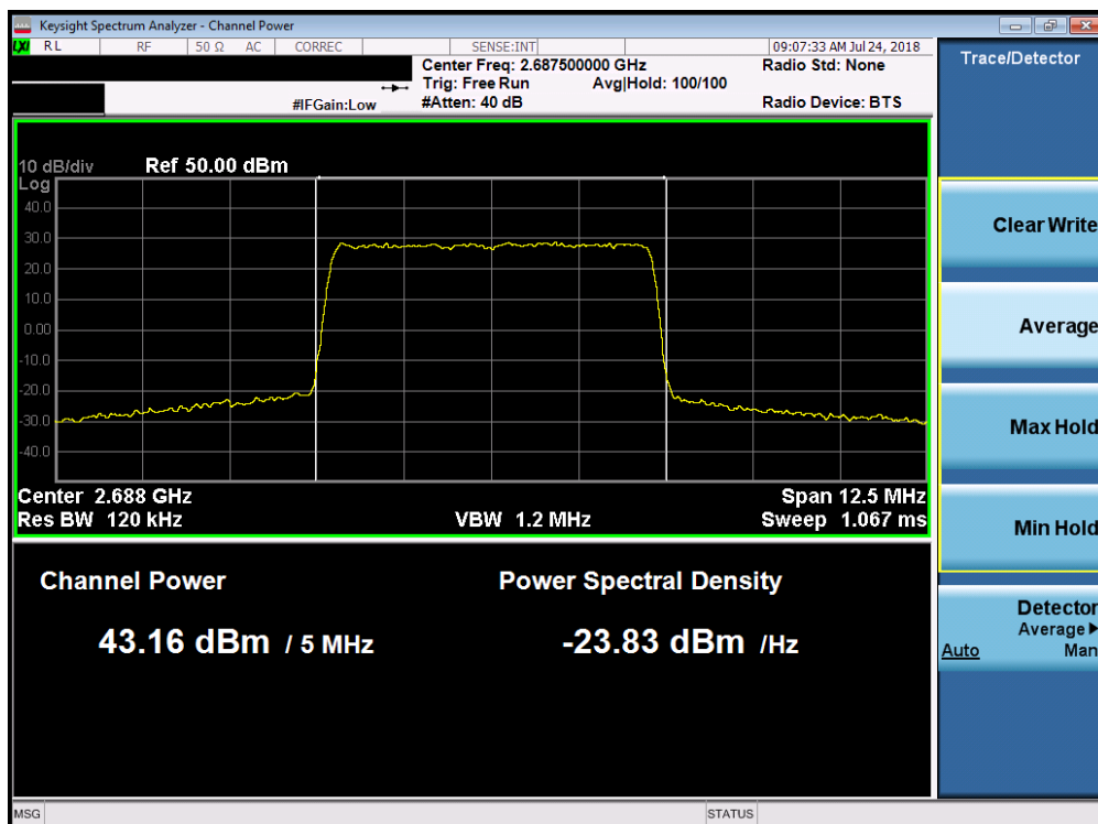
Plot 7-54. Maximum Conducted Power (Band 7 - 5.0MHz 16-QAM – High Channel)
