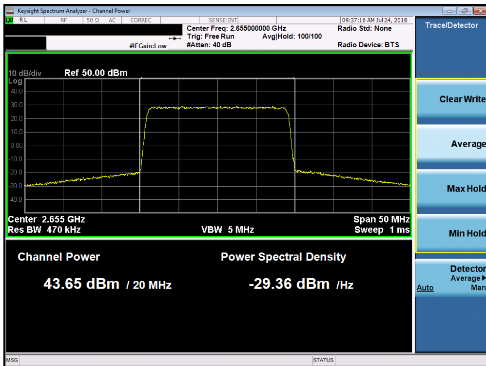
Plot 7-95. Maximum Conducted Power (Band 7 - 20.0MHz 256-QAM – Mid Channel)
