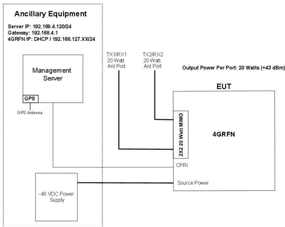
Figure 2-1. Test Setup
