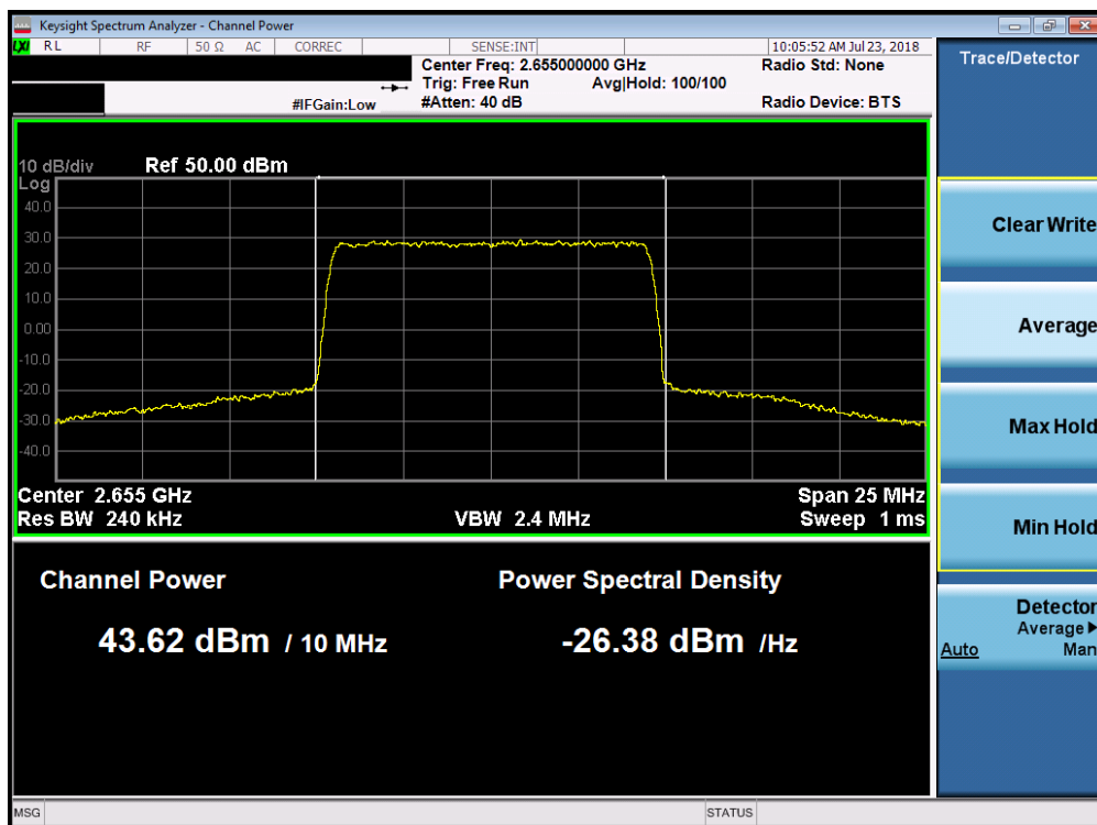
Plot 7-20. Maximum Conducted Power (Band 7 - 10.0MHz 64-QAM – Mid Channel)
