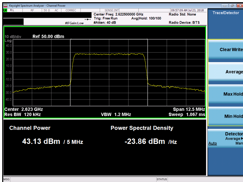
Plot 7-10. Maximum Conducted Power (Band 7 - 5.0MHz 256-QAM – Low Channel)
