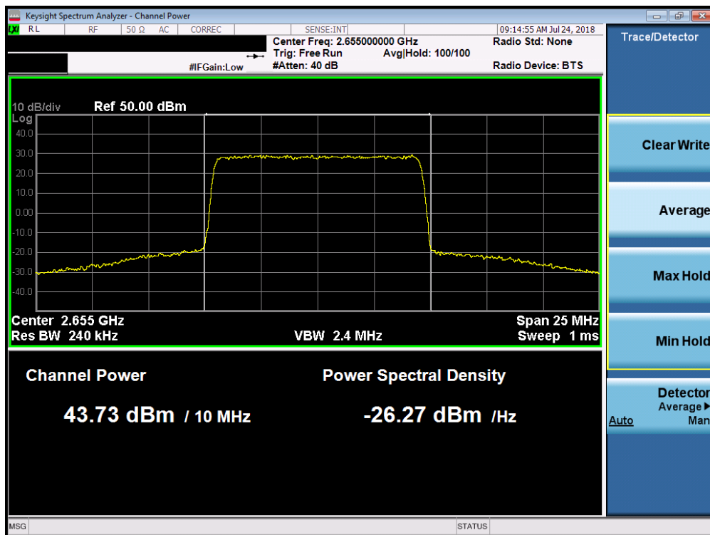
Plot 7-71. Maximum Conducted Power (Band 7 - 10.0MHz 256-QAM – Mid Channel)
