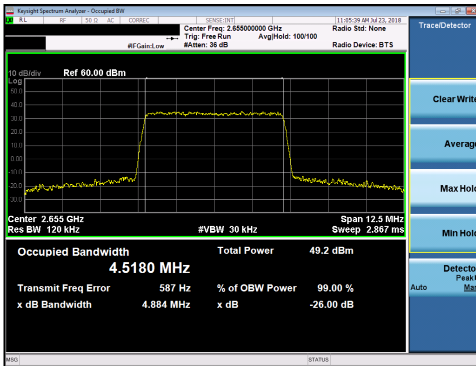
Plot 7-97. Occupied Bandwidth Plot (Band 7 - 5.0MHz QPSK)
