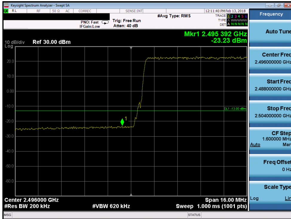
Plot 7-207. Lower Band Edge Plot (Band 41 - 20.0MHz 256-QAM)
