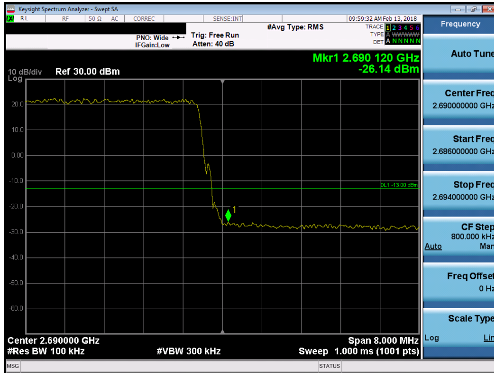
Plot 7-165. Upper Band Edge Plot (Band 41 - 10.0MHz QPSK)
