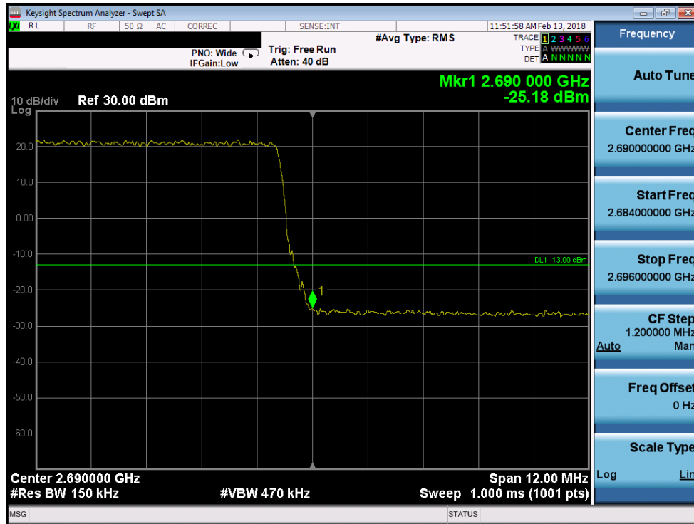
Plot 7-189. Upper Band Edge Plot (Band 41 - 15.0MHz 64-QAM)
