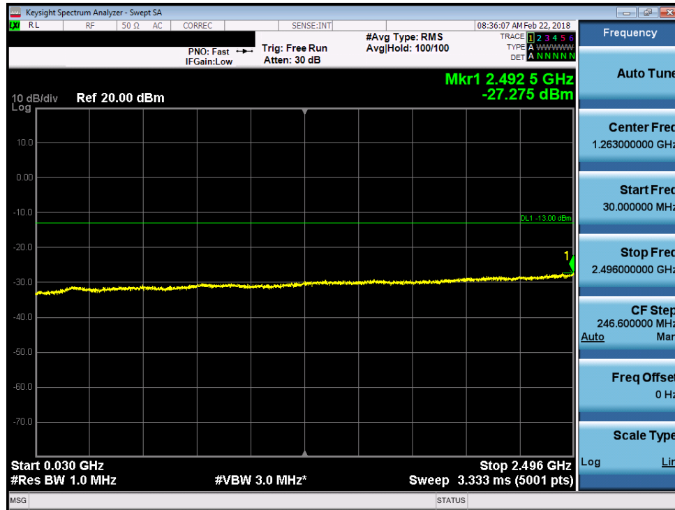
Plot 7-144. Conducted Spurious Plot (Band 41 - 5.0MHz QPSK – High Channel)
