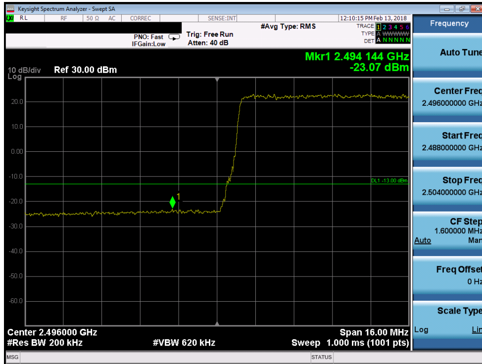
Plot 7-203. Lower Band Edge Plot (Band 41 - 20.0MHz 64-QAM)
