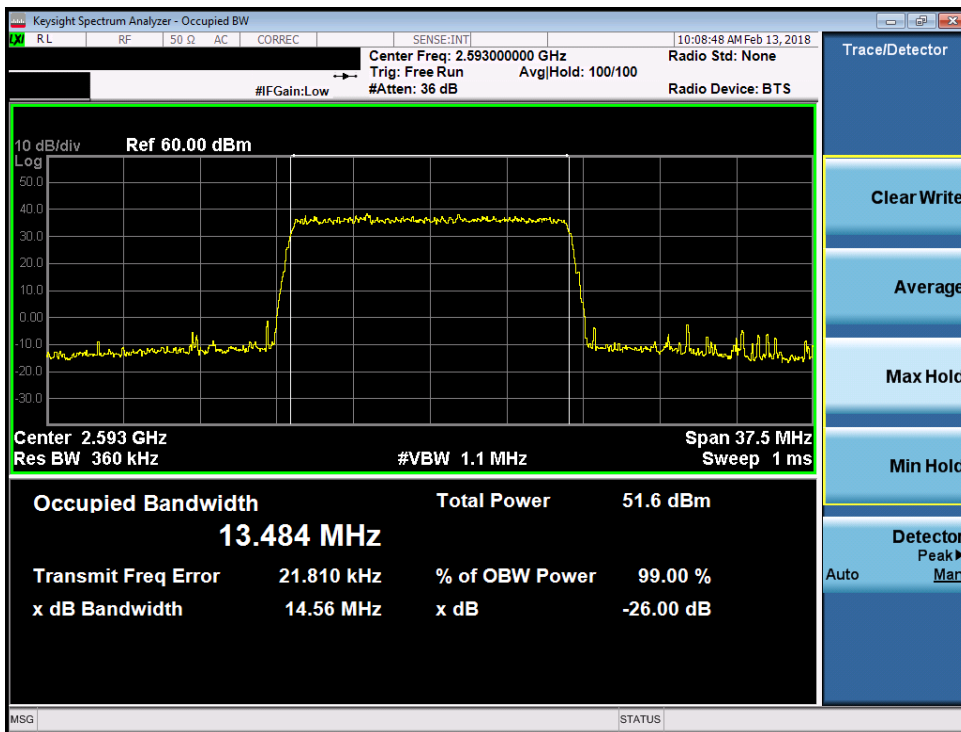
Plot 7-106. Occupied Bandwidth Plot (Band 41 - 15.0MHz 16-QAM)
