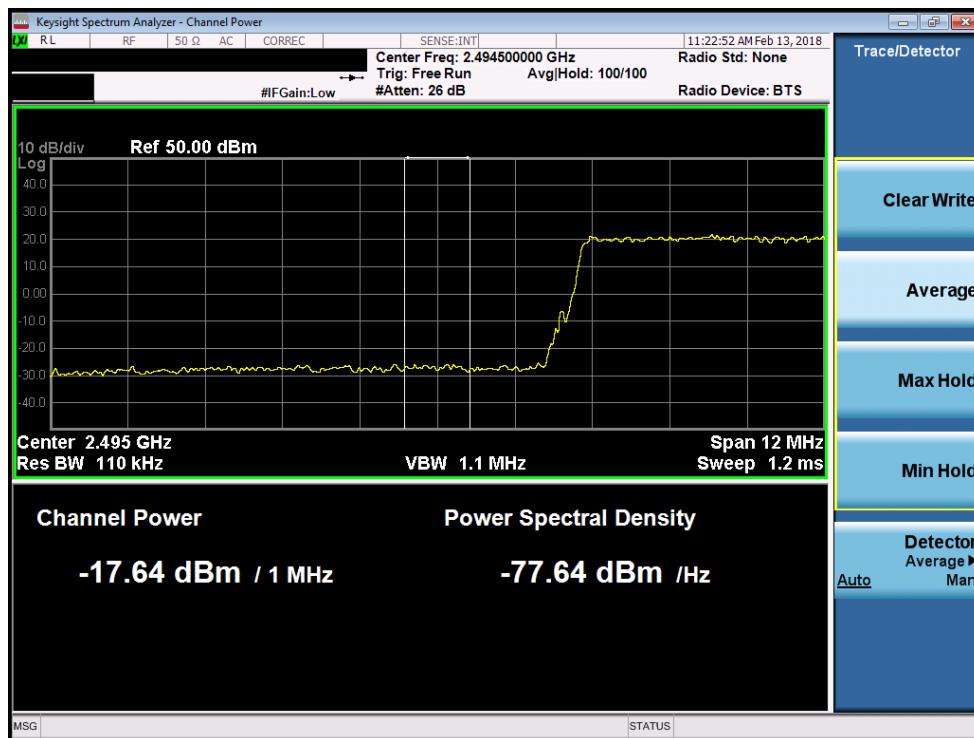
Plot 7-180. Lower Extended Band Edge Plot (Band 41 - 15.0MHz QPSK)
