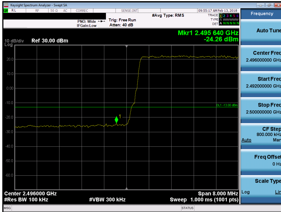
Plot 7-171. Lower Band Edge Plot (Band 41 - 10.0MHz 64-QAM)
