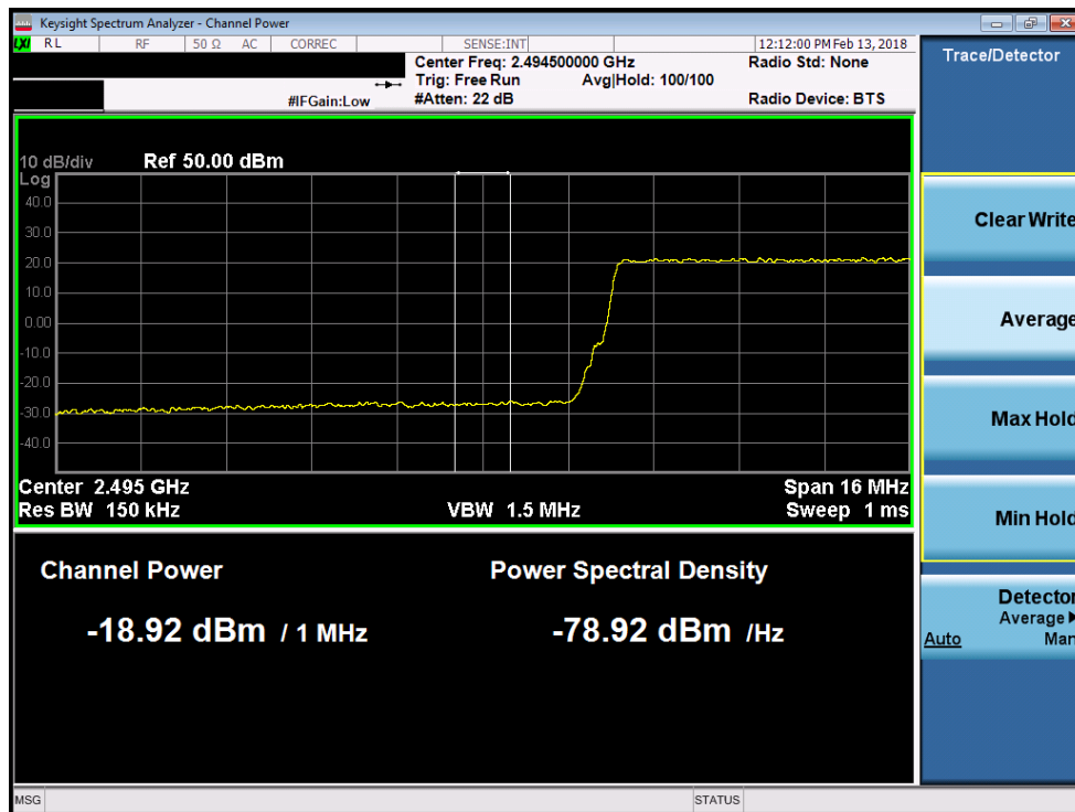
Plot 7-208. Lower Extended Band Edge Plot (Band 41 - 20.0MHz 256-QAM)
