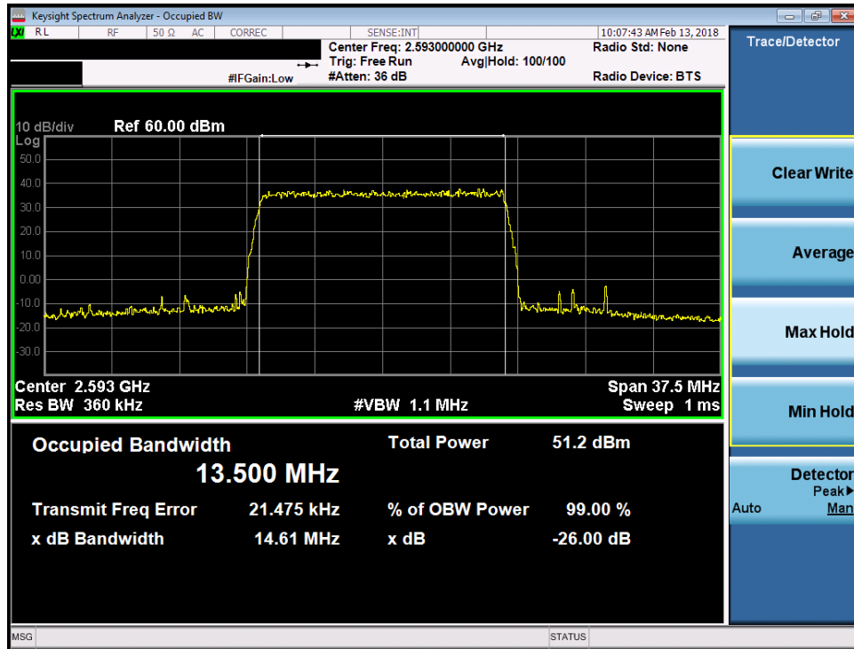
Plot 7-105. Occupied Bandwidth Plot (Band 41 - 15.0MHz QPSK)
