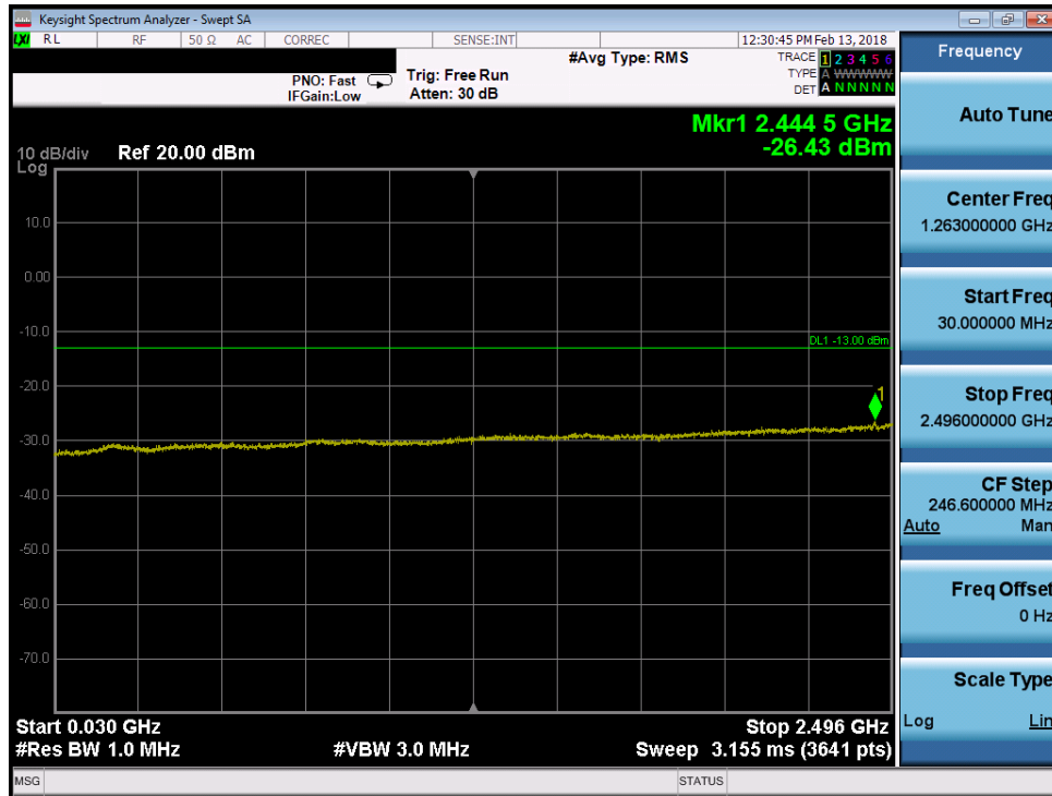
Plot 7-135. Conducted Spurious Plot (Band 41 - 5.0MHz QPSK – High Channel)
