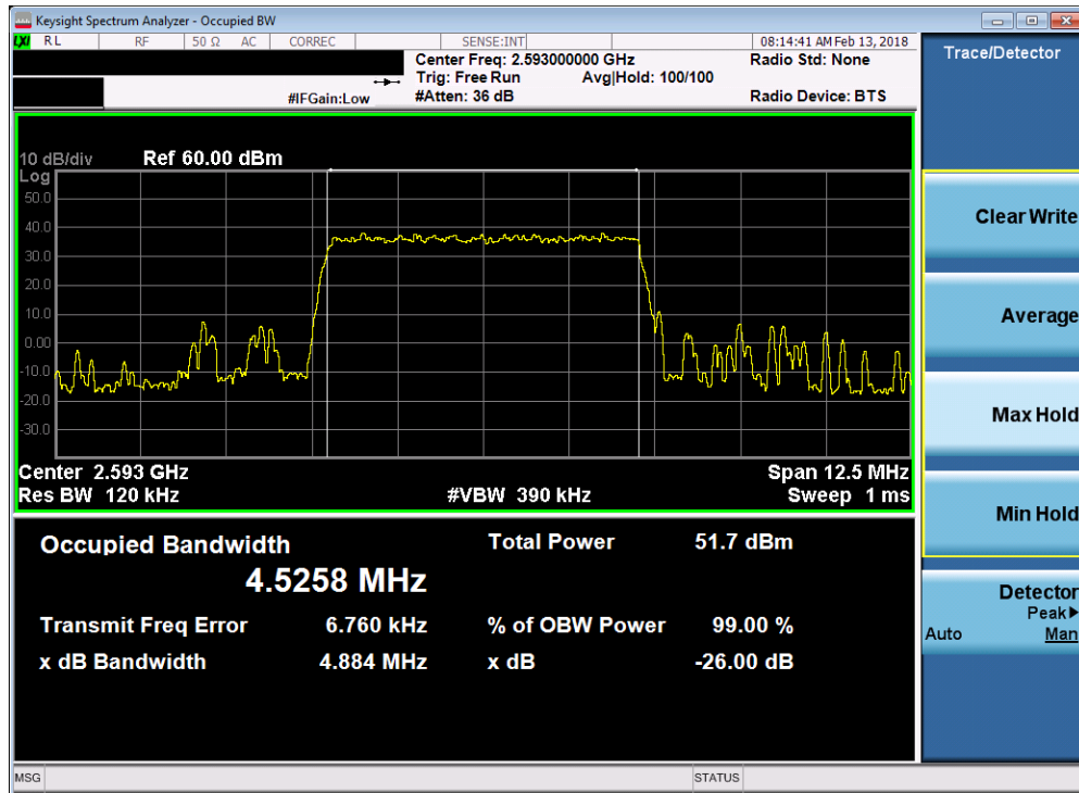
Plot 7-99. Occupied Bandwidth Plot (Band 41 - 5.0MHz 64-QAM)
