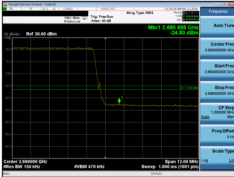
Plot 7-181. Upper Band Edge Plot (Band 41 - 15.0MHz QPSK)
