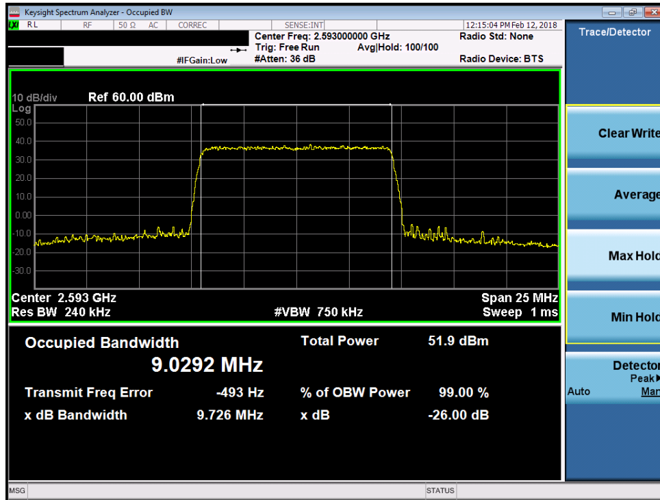
Plot 7-117. Occupied Bandwidth Plot (Band 41 - 10.0MHz QPSK)
