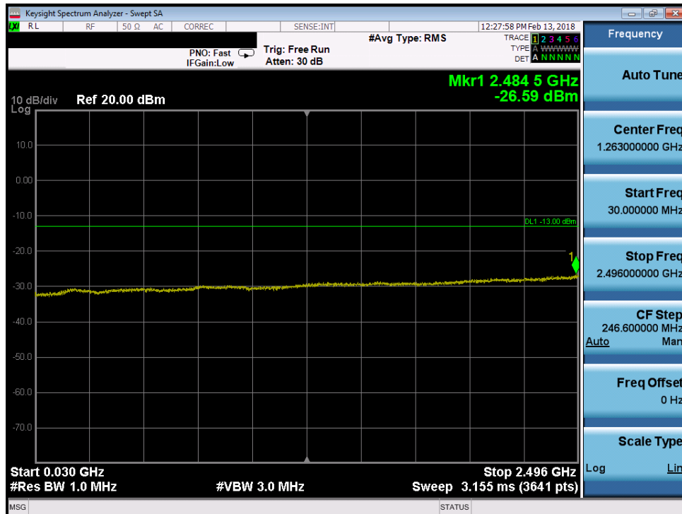
Plot 7-132. Conducted Spurious Plot (Band 41 - 5.0MHz QPSK – Mid Channel)
