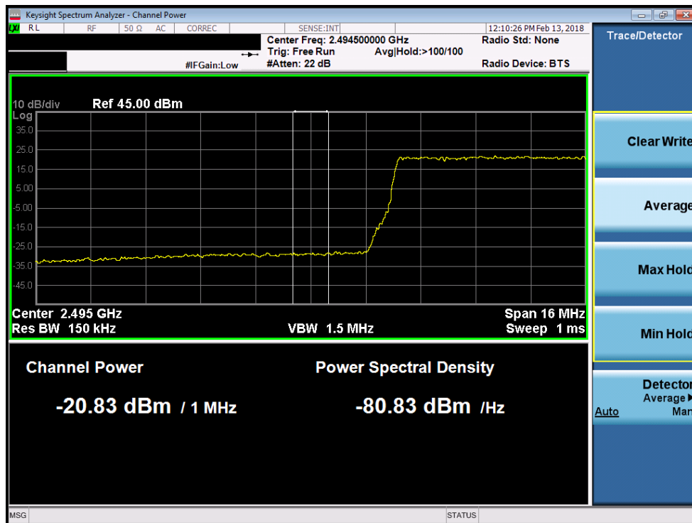
Plot 7-204. Lower Extended Band Edge Plot (Band 41 - 20.0MHz 64-QAM)
