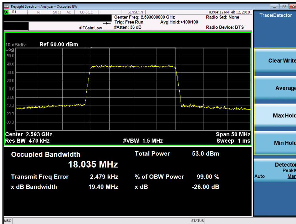
Plot 7-126. Occupied Bandwidth Plot (Band 41 - 20.0MHz 16-QAM)
