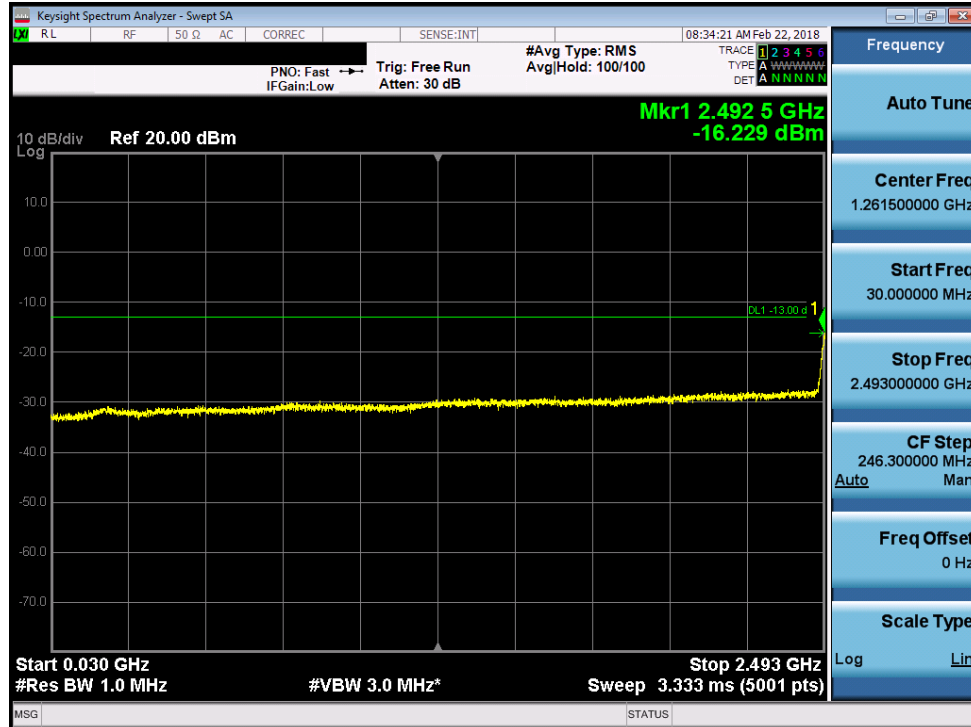
Plot 7-138. Conducted Spurious Plot (Band 41 - 5.0MHz QPSK – Low Channel)
