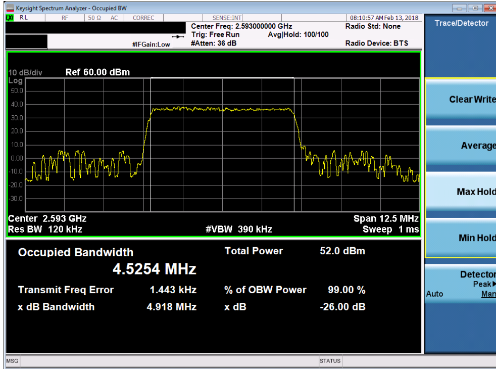
Plot 7-97. Occupied Bandwidth Plot (Band 41 - 5.0MHz QPSK)
