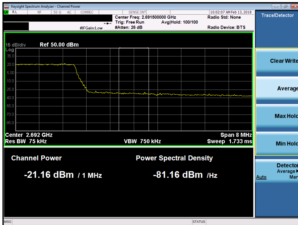
Plot 7-170. Upper Extended Band Edge Plot (Band 41 - 10.0MHz 16-QAM)
