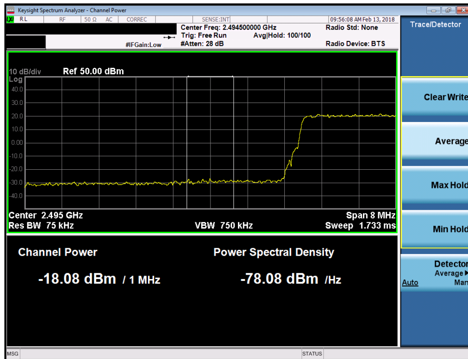
Plot 7-172. Lower Extended Band Edge Plot (Band 41 - 10.0MHz 64-QAM)
