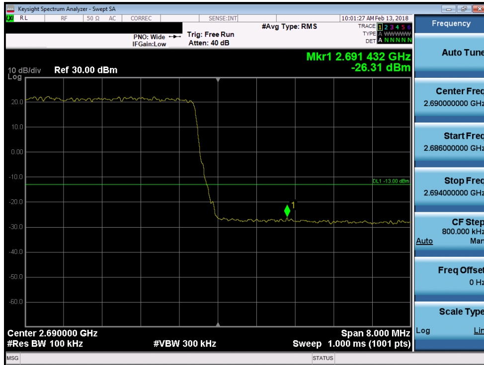
Plot 7-169. Upper Band Edge Plot (Band 41 - 10.0MHz 16-QAM)
