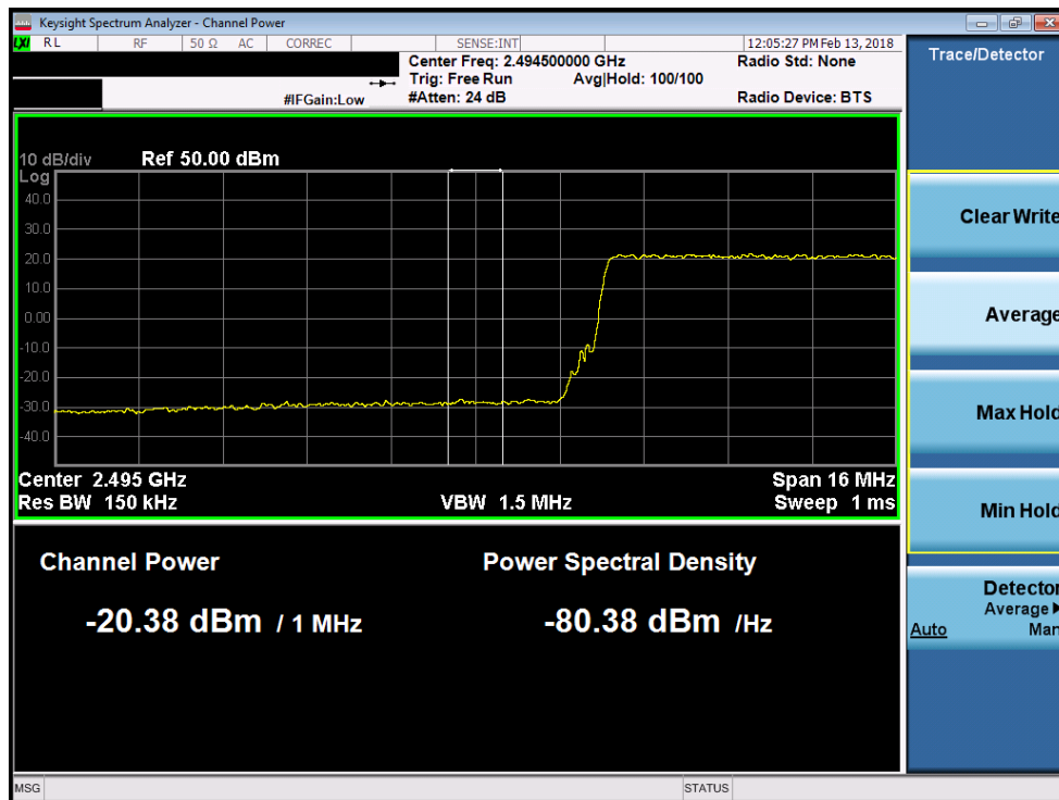
Plot 7-196. Lower Extended Band Edge Plot (Band 41 - 20.0MHz QPSK)
