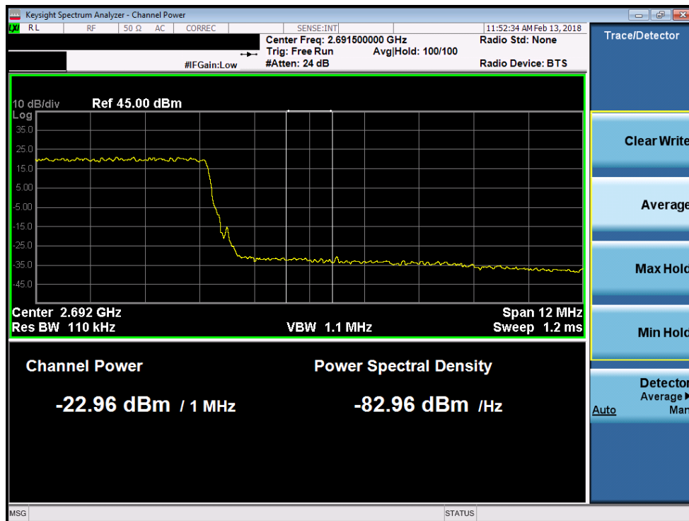
Plot 7-190. Upper Extended Band Edge Plot (Band 41 - 15.0MHz 64-QAM)
