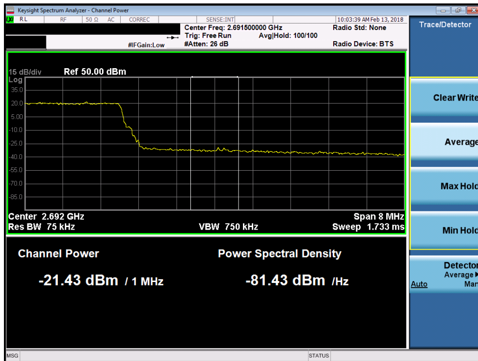
Plot 7-174. Upper Extended Band Edge Plot (Band 41 - 10.0MHz 64-QAM)
