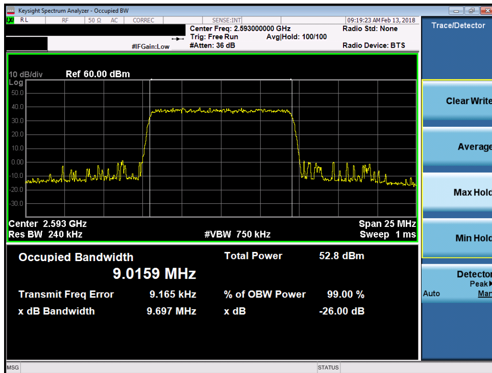
Plot 7-104. Occupied Bandwidth Plot (Band 41 - 10.0MHz 256-QAM)
