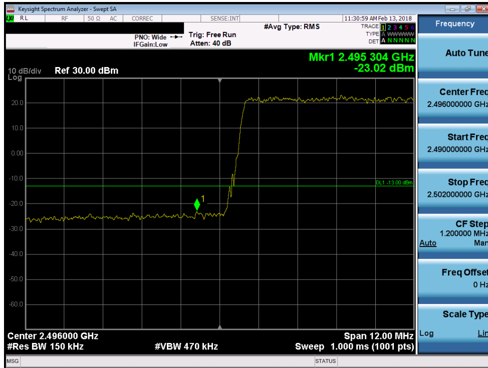
Plot 7-191. Lower Band Edge Plot (Band 41 - 15.0MHz 256-QAM)
