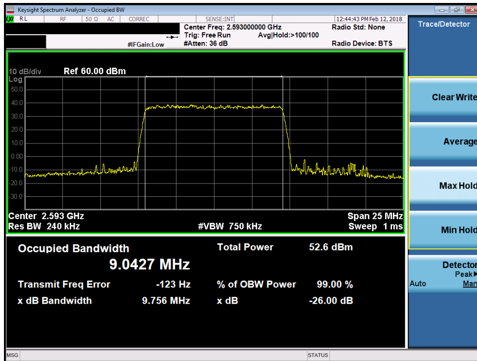
Plot 7-120. Occupied Bandwidth Plot (Band 41 - 10.0MHz 256-QAM)
