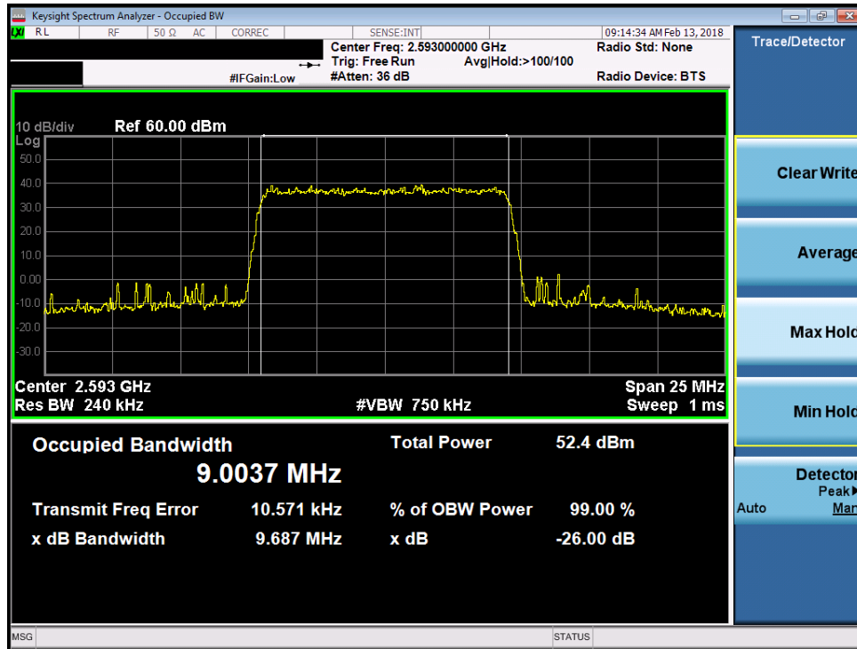
Plot 7-103. Occupied Bandwidth Plot (Band 41 - 10.0MHz 64-QAM)
