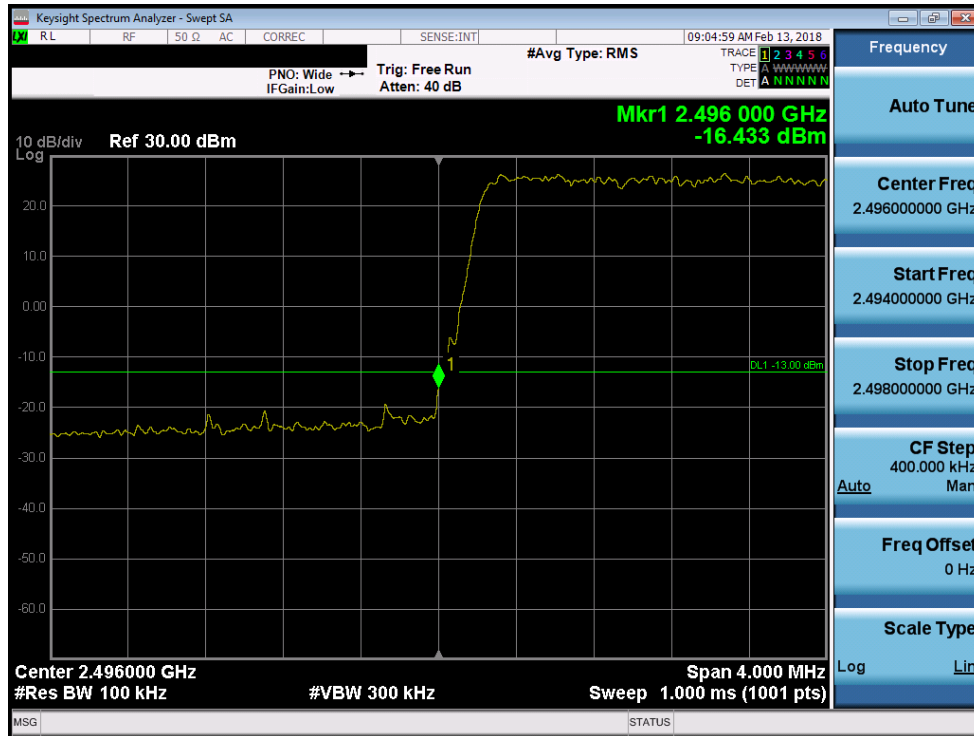
Plot 7-155. Lower Band Edge Plot (Band 41 - 5.0MHz 64-QAM)
