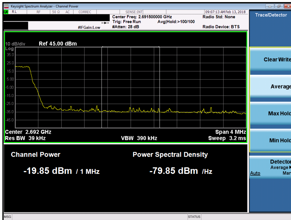
Plot 7-150. Upper Extended Band Edge Plot (Band 41 - 5.0MHz QPSK)
