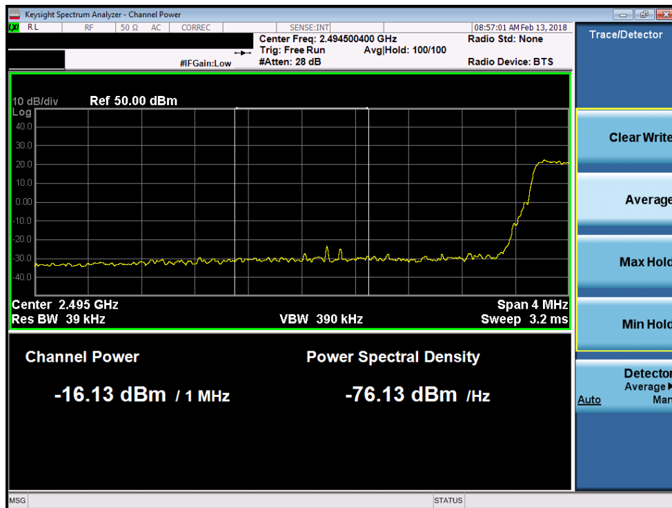
Plot 7-160. Lower Extended Band Edge Plot (Band 41 - 5.0MHz 256-QAM)
