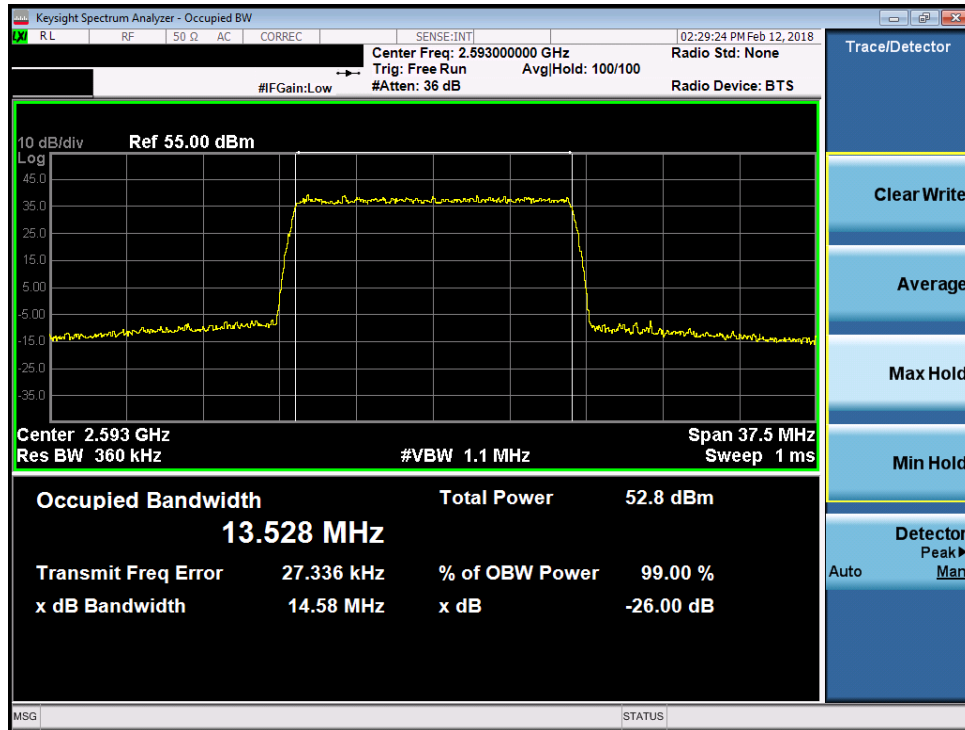
Plot 7-123. Occupied Bandwidth Plot (Band 41 - 15.0MHz 64-QAM)
