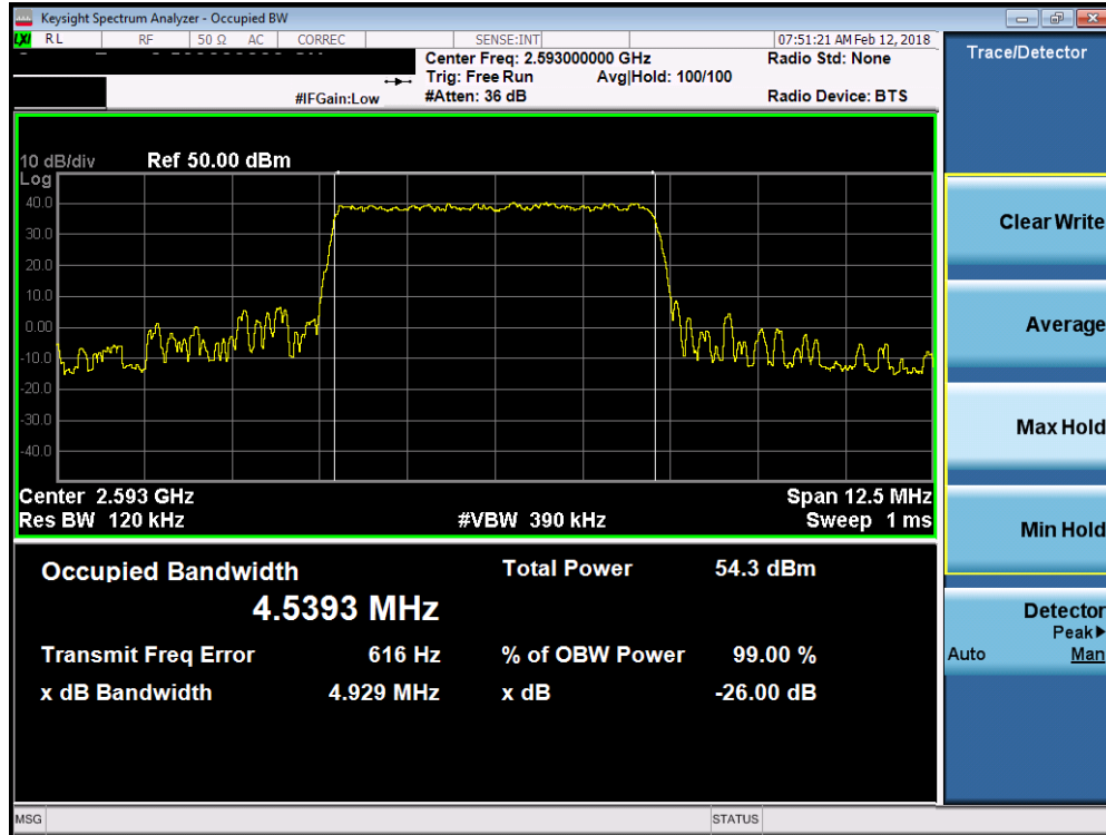
Plot 7-115. Occupied Bandwidth Plot (Band 41 - 5.0MHz 64-QAM)
