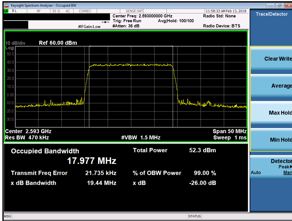
Plot 7-111. Occupied Bandwidth Plot (Band 41 - 20.0MHz 64-QAM)
