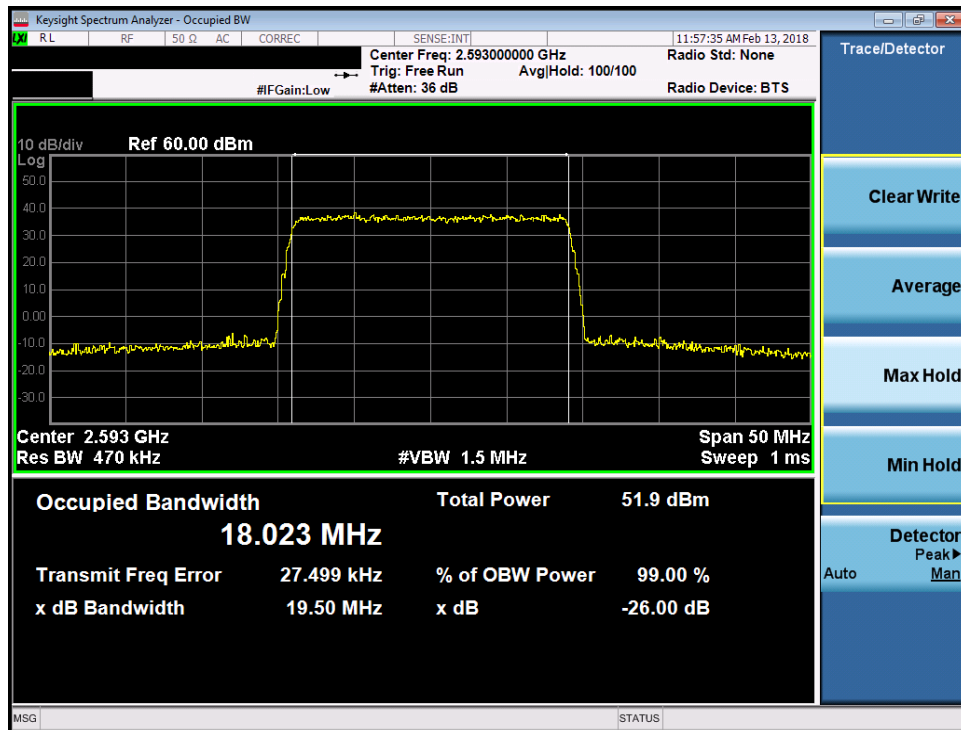
Plot 7-110. Occupied Bandwidth Plot (Band 41 - 20.0MHz 16-QAM)
