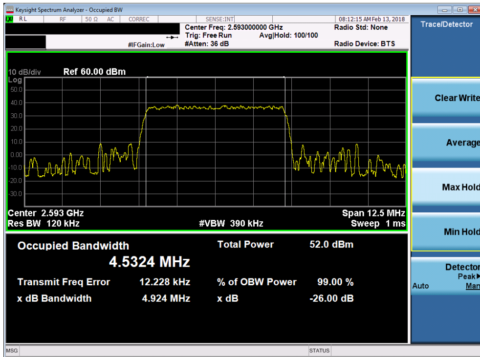
Plot 7-98. Occupied Bandwidth Plot (Band 41 - 5.0MHz 16-QAM)
