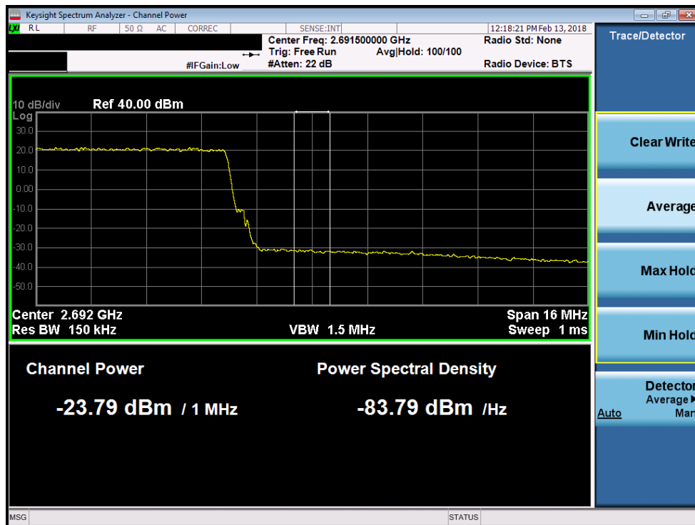
Plot 7-210. Upper Extended Band Edge Plot (Band 41 - 20.0MHz 256-QAM)
