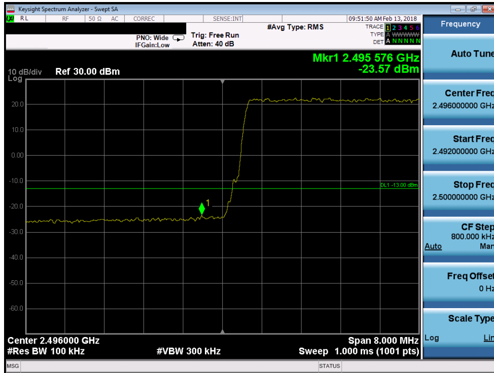
Plot 7-163. Lower Band Edge Plot (Band 41 - 10.0MHz QPSK)
