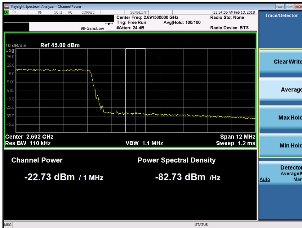
Plot 7-194. Upper Extended Band Edge Plot (Band 41 - 15.0MHz 256-QAM)
