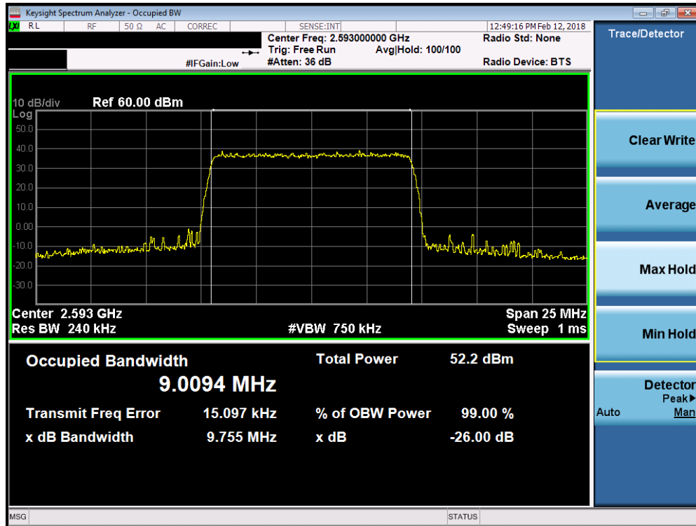
Plot 7-119. Occupied Bandwidth Plot (Band 41 - 10.0MHz 64-QAM)
