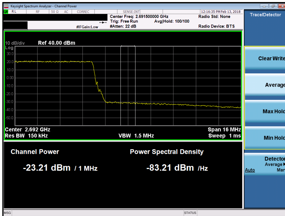
Plot 7-206. Upper Extended Band Edge Plot (Band 41 - 20.0MHz 64-QAM)
