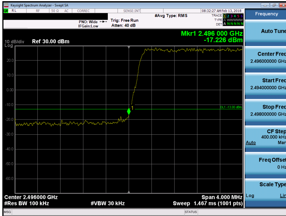
Plot 7-151. Lower Band Edge Plot (Band 41 - 5.0MHz 16-QAM)
