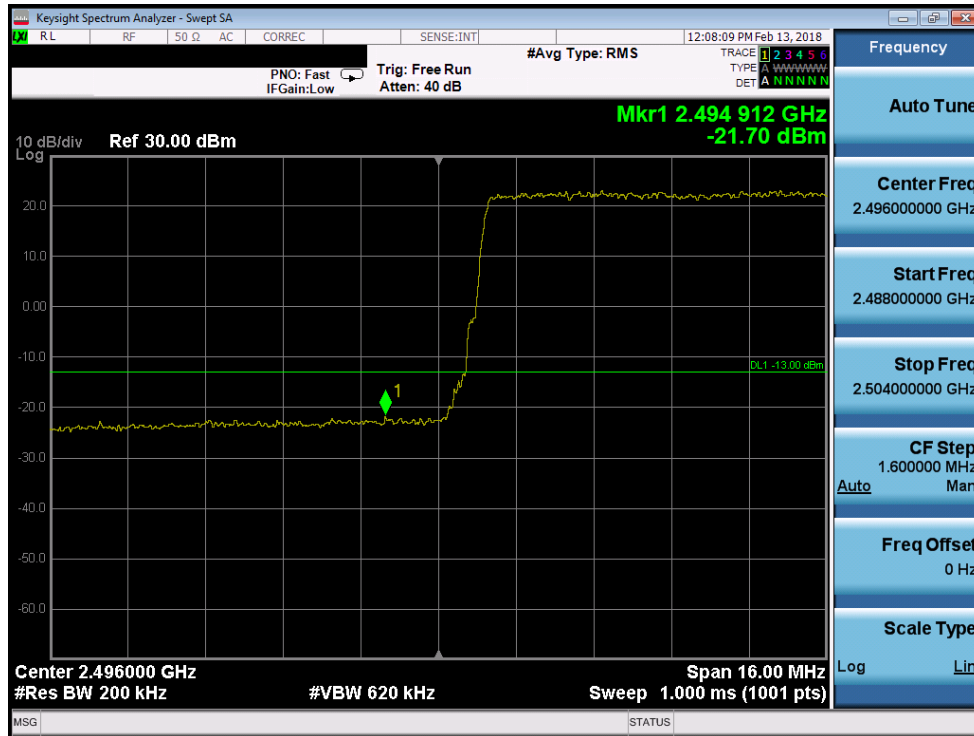
Plot 7-199. Lower Band Edge Plot (Band 41 - 20.0MHz 16-QAM)
