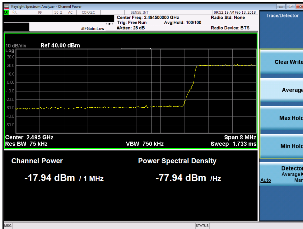
Plot 7-164. Lower Extended Band Edge Plot (Band 41 - 10.0MHz QPSK)
