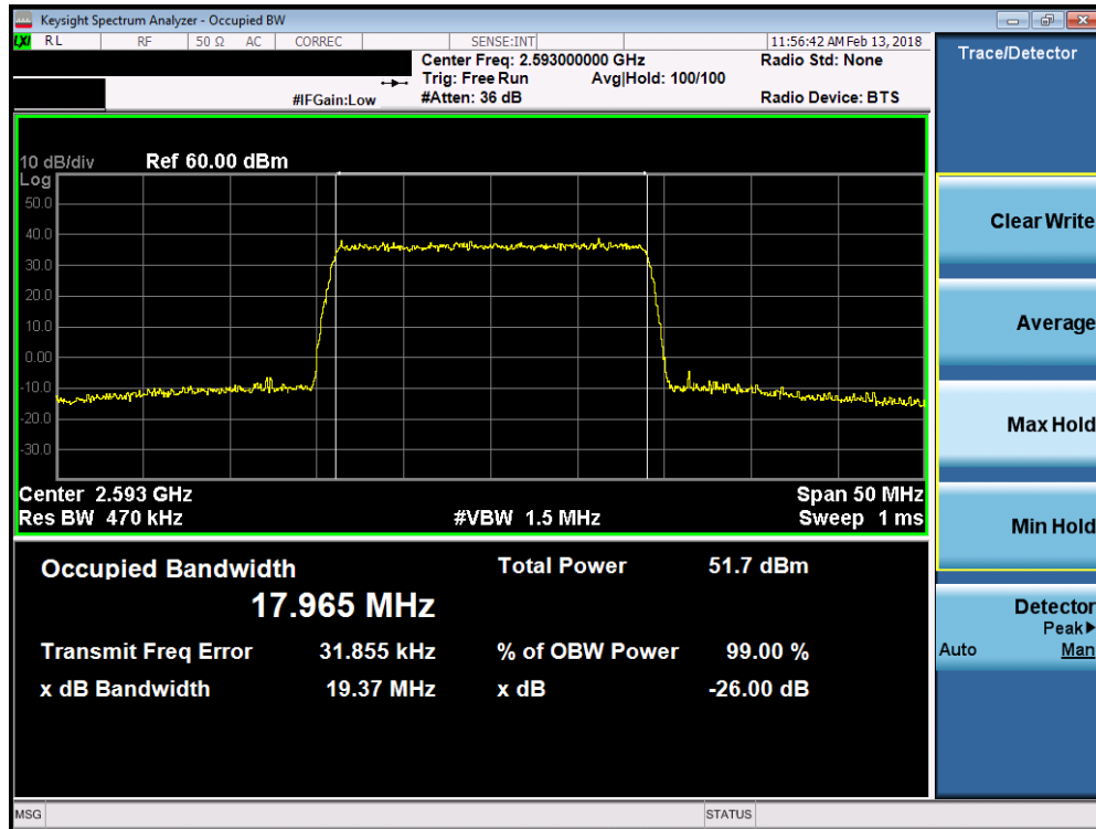
Plot 7-109. Occupied Bandwidth Plot (Band 41 - 20.0MHz QPSK)
