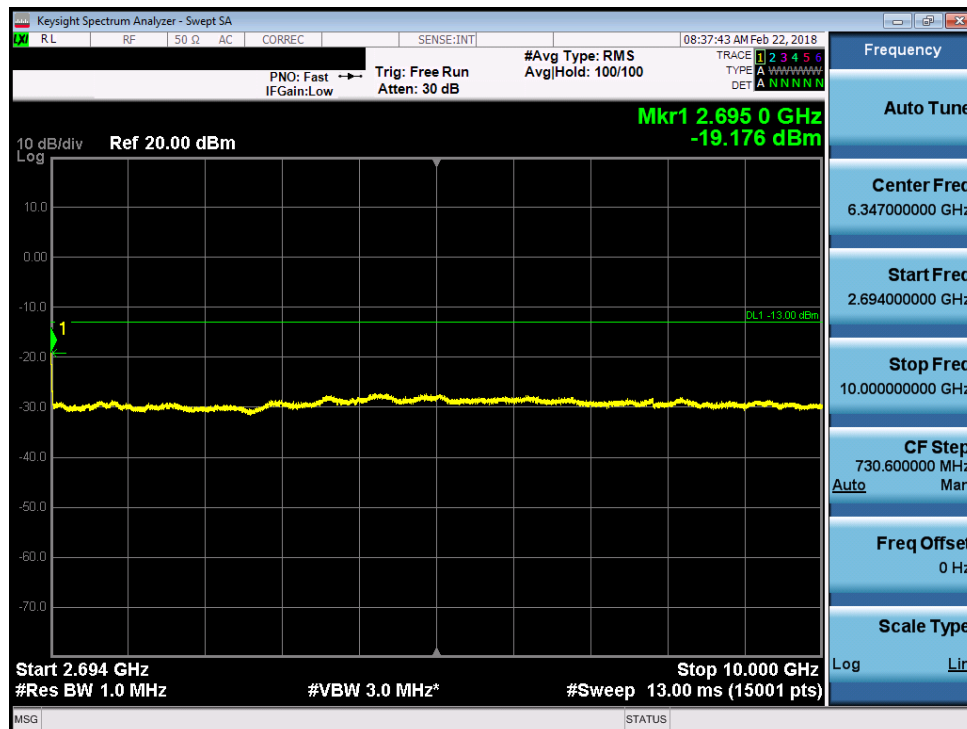
Plot 7-145. Conducted Spurious Plot (Band 41 - 5.0MHz QPSK – High Channel)
