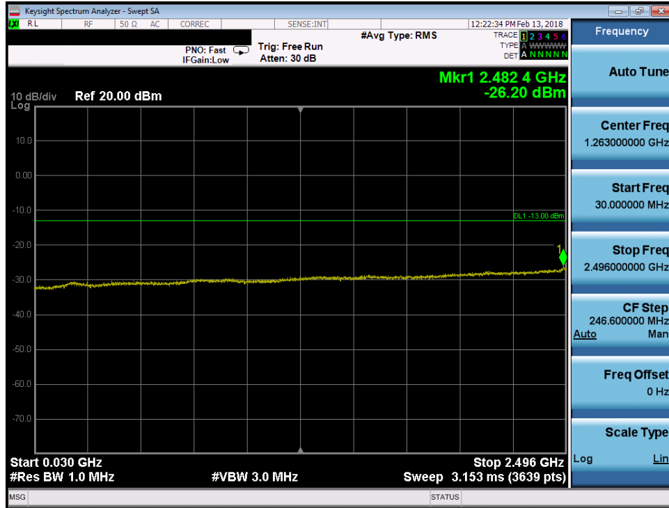
Plot 7-129. Conducted Spurious Plot (Band 41 - 5.0MHz QPSK – Low Channel)
