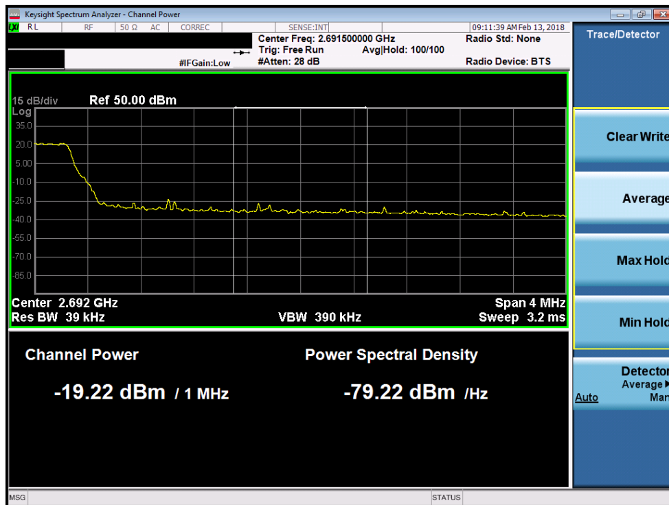
Plot 7-162. Upper Extended Band Edge Plot (Band 41 - 5.0MHz 256-QAM)
