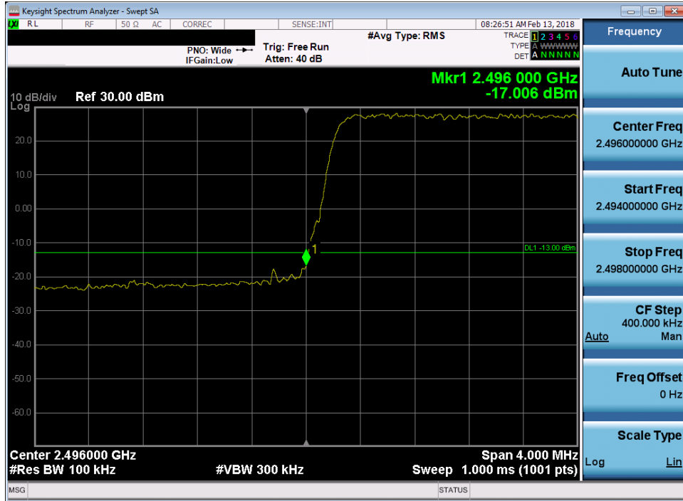
Plot 7-147. Lower Band Edge Plot (Band 41 - 5.0MHz QPSK)
