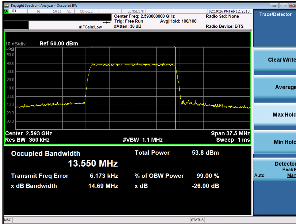
Plot 7-121. Occupied Bandwidth Plot (Band 41 - 15.0MHz QPSK)
