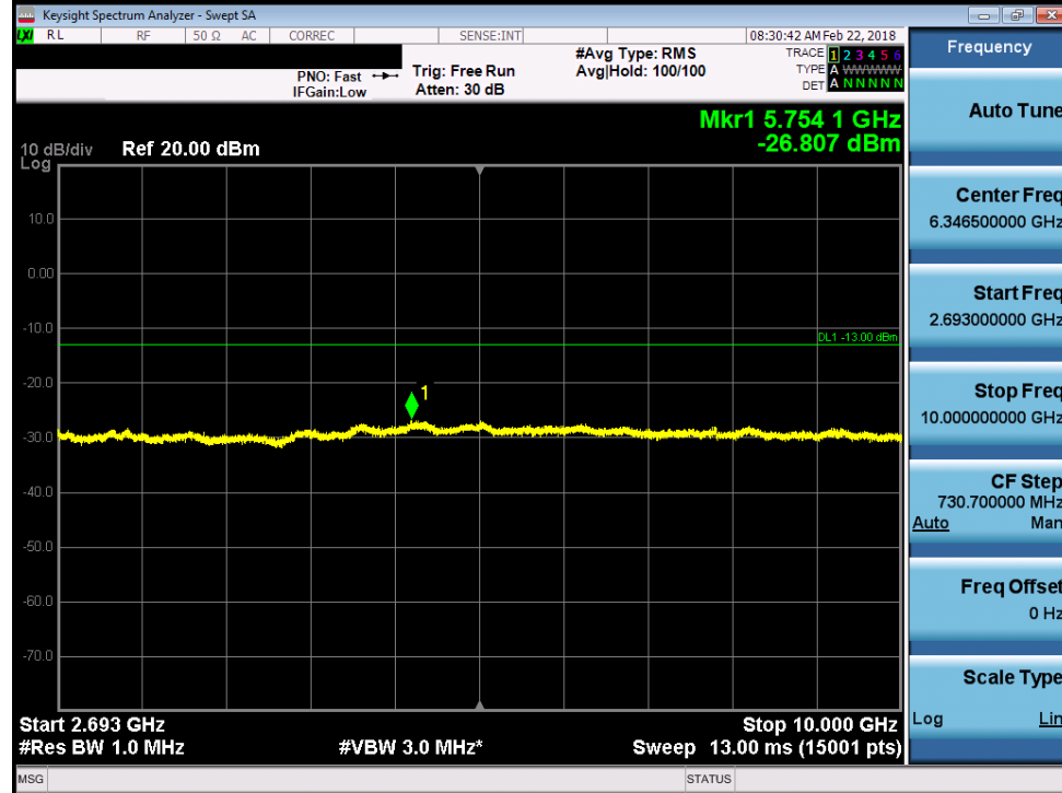
Plot 7-139. Conducted Spurious Plot (Band 41 - 5.0MHz QPSK – Low Channel)
