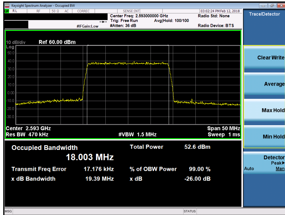
Plot 7-128. Occupied Bandwidth Plot (Band 41 - 20.0MHz 256-QAM)
