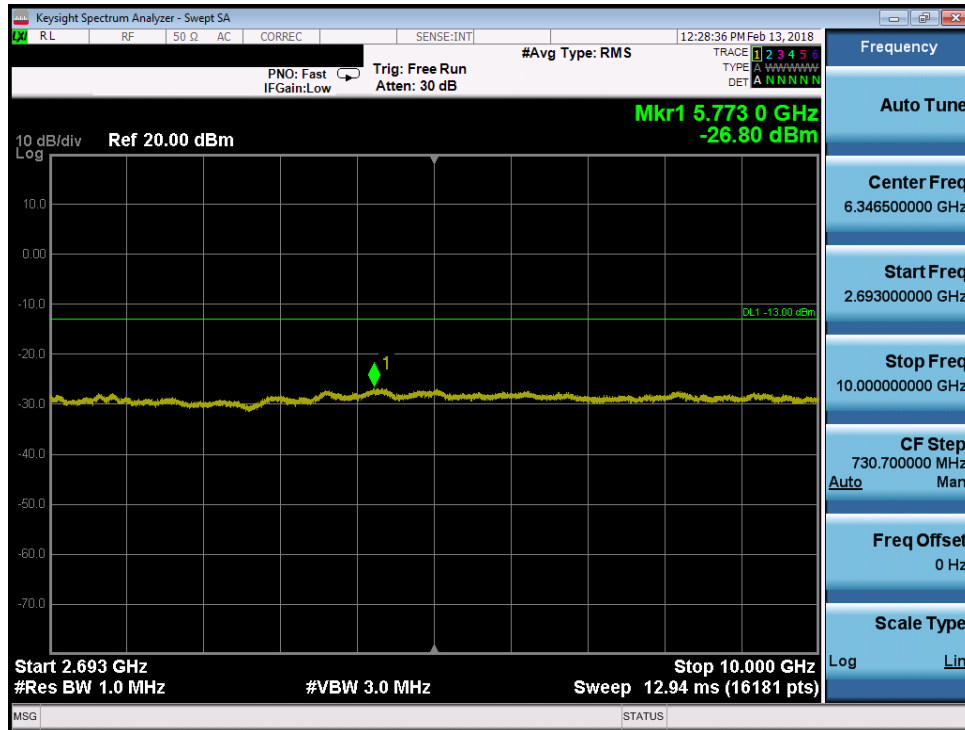
Plot 7-133. Conducted Spurious Plot (Band 41 - 5.0MHz QPSK – Mid Channel)
