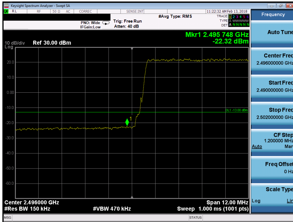
Plot 7-179. Lower Band Edge Plot (Band 41 - 15.0MHz QPSK)
