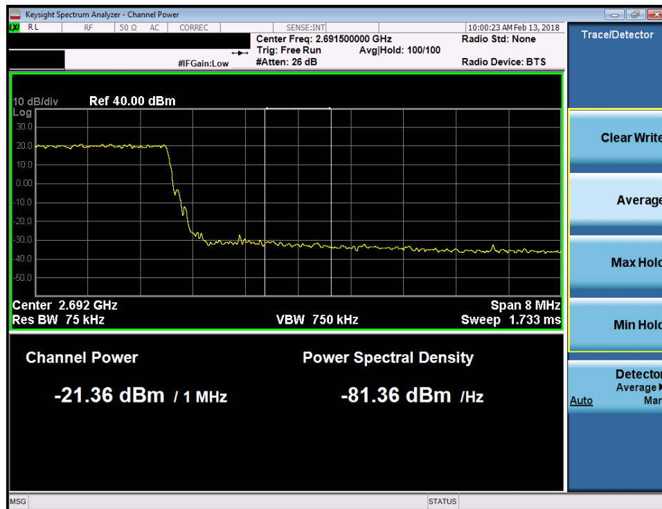
Plot 7-166. Upper Extended Band Edge Plot (Band 41 - 10.0MHz QPSK)
