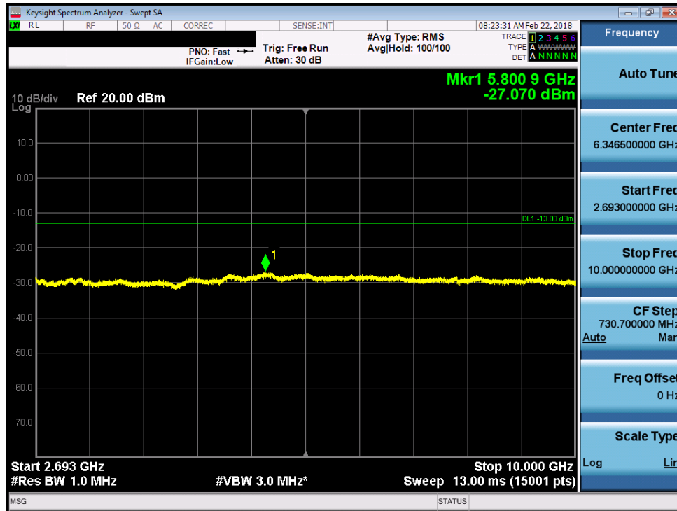
Plot 7-142. Conducted Spurious Plot (Band 41 - 5.0MHz QPSK – Mid Channel)
