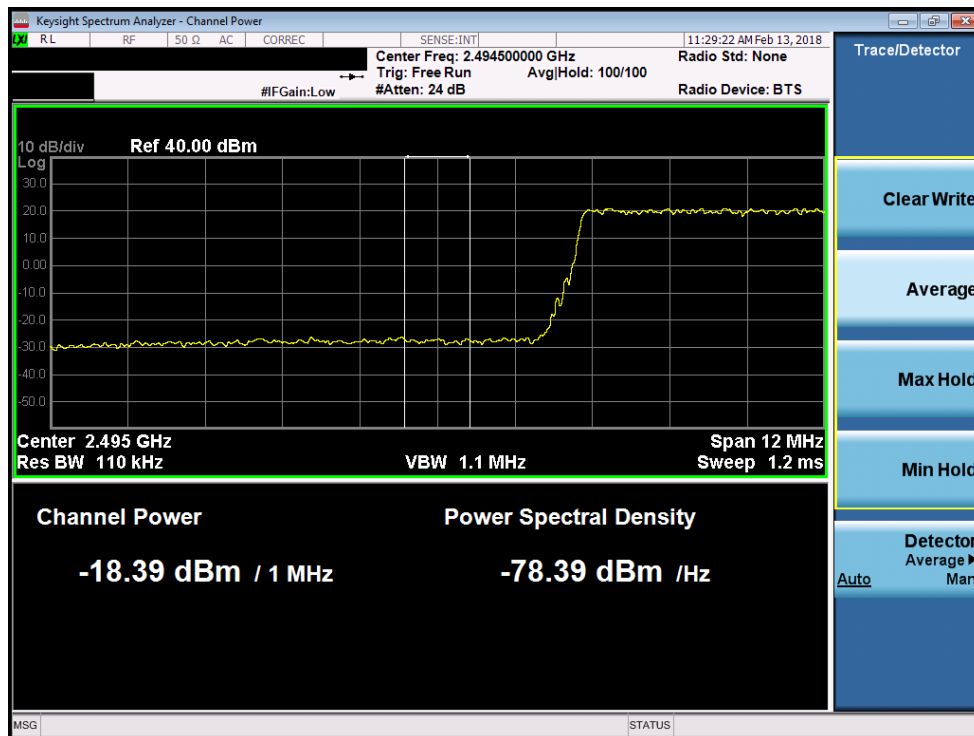
Plot 7-188. Lower Extended Band Edge Plot (Band 41 - 15.0MHz 64-QAM)
