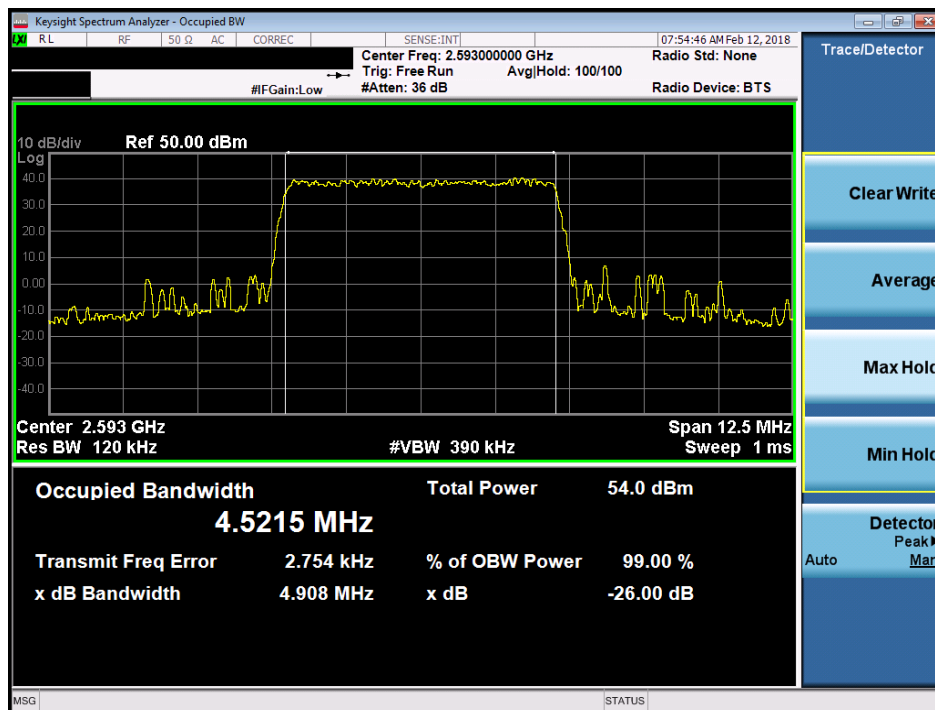
Plot 7-114. Occupied Bandwidth Plot (Band 41 - 5.0MHz 16-QAM)
