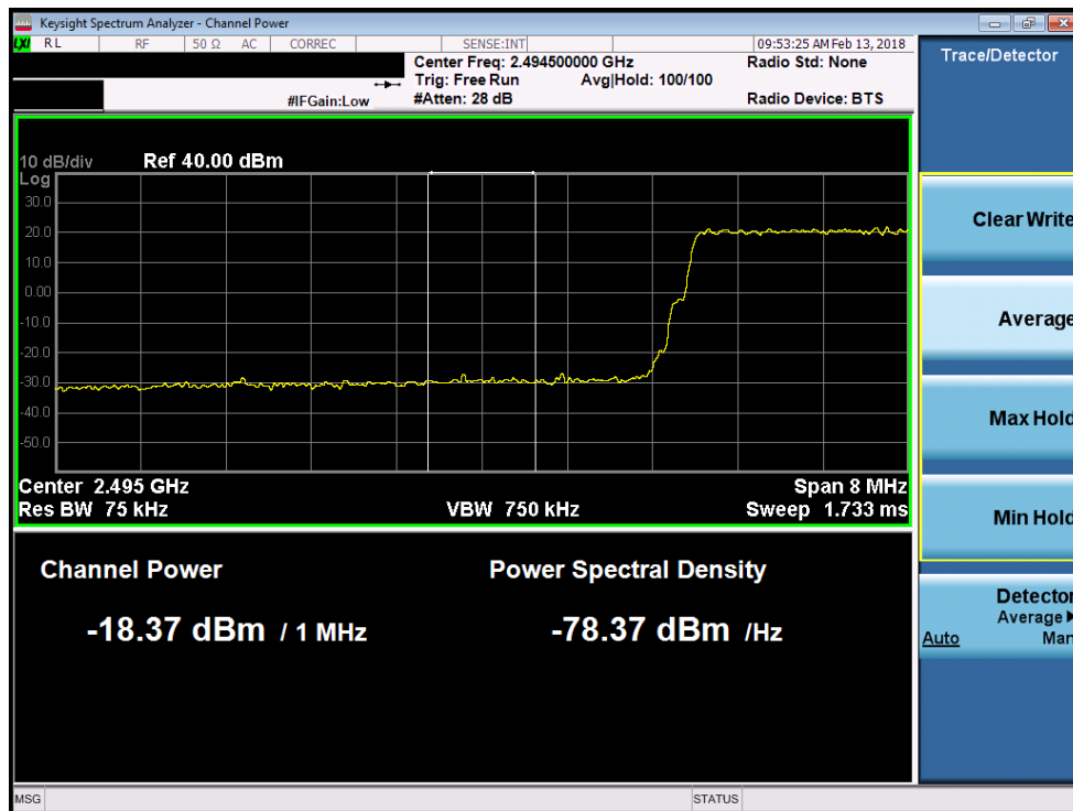
Plot 7-168. Lower Extended Band Edge Plot (Band 41 - 10.0MHz 16-QAM)
