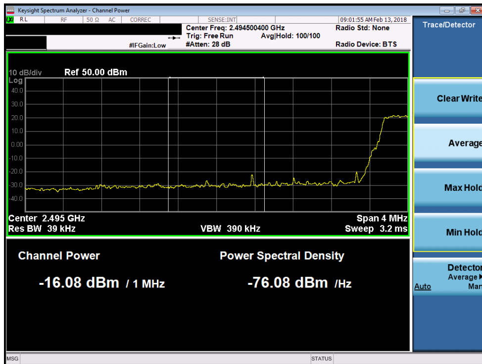
Plot 7-152. Lower Extended Band Edge Plot (Band 41 - 5.0MHz 16-QAM)
