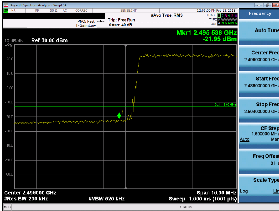
Plot 7-195. Lower Band Edge Plot (Band 41 - 20.0MHz QPSK)
