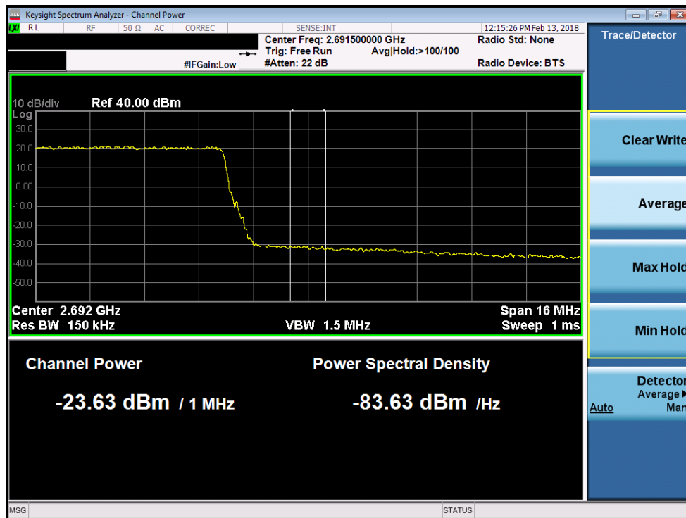
Plot 7-202. Upper Extended Band Edge Plot (Band 41 - 20.0MHz 16-QAM)
