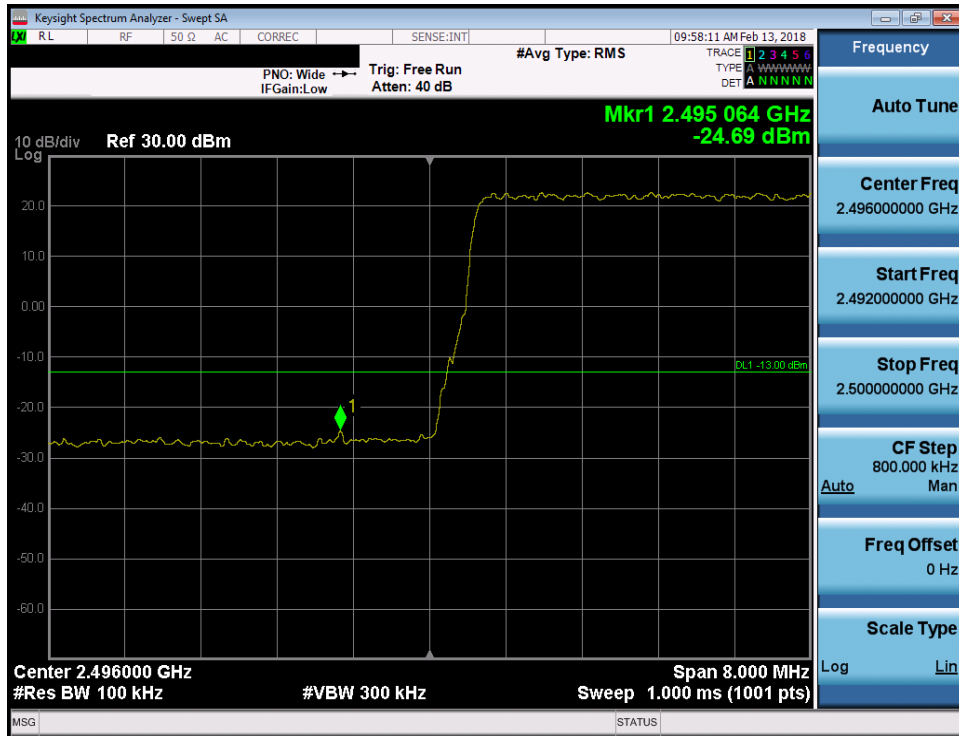
Plot 7-175. Lower Band Edge Plot (Band 41 - 10.0MHz 256-QAM)
