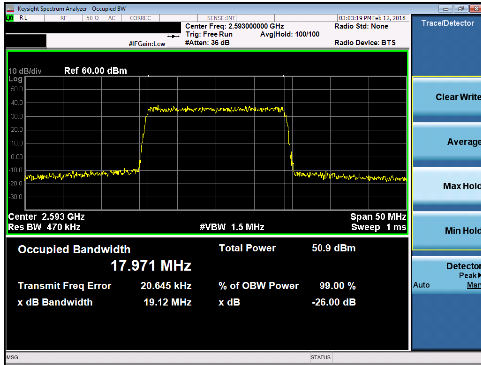
Plot 7-127. Occupied Bandwidth Plot (Band 41 - 20.0MHz 64-QAM)
