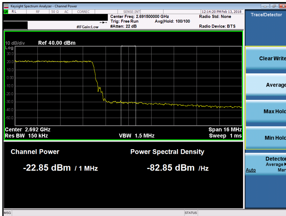
Plot 7-198. Upper Extended Band Edge Plot (Band 41 - 20.0MHz QPSK)
