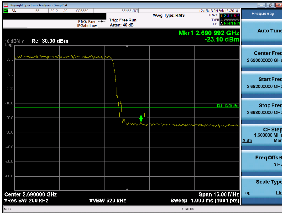
Plot 7-201. Upper Band Edge Plot (Band 41 - 20.0MHz 16-QAM)
