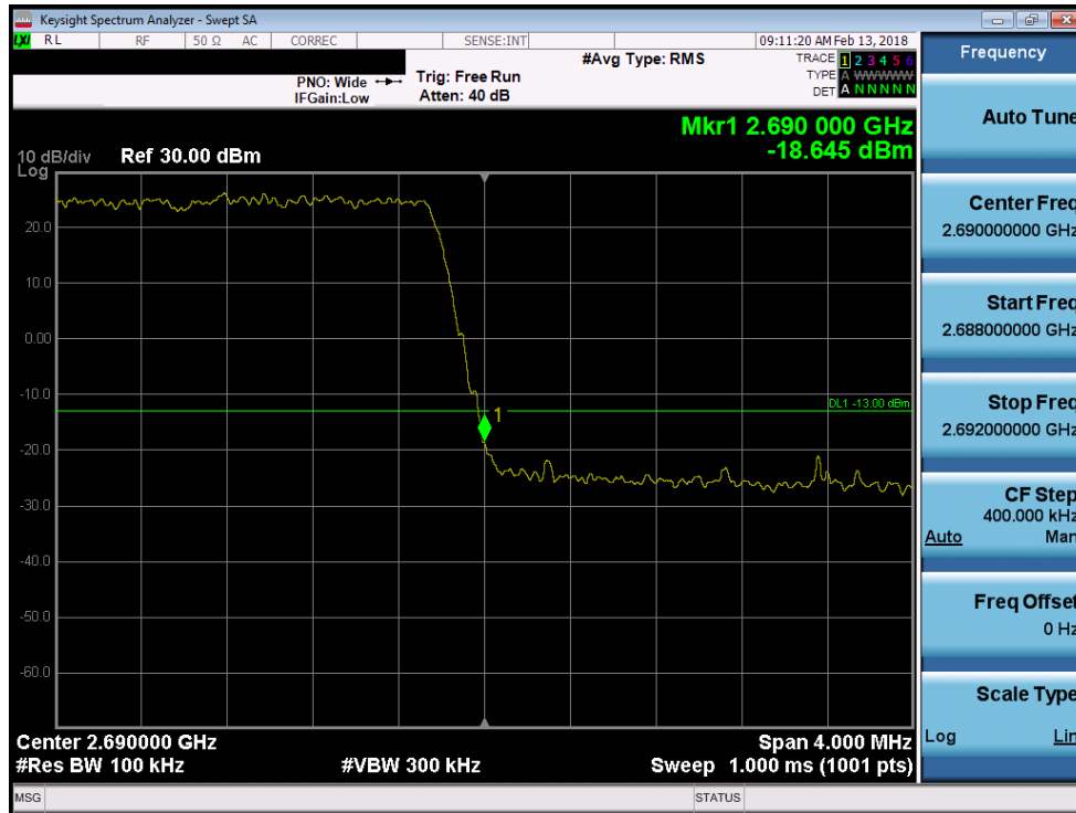
Plot 7-161. Upper Band Edge Plot (Band 41 - 5.0MHz 256-QAM)
