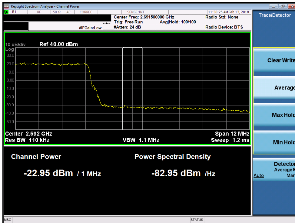
Plot 7-186. Upper Extended Band Edge Plot (Band 41 - 15.0MHz 16-QAM)
