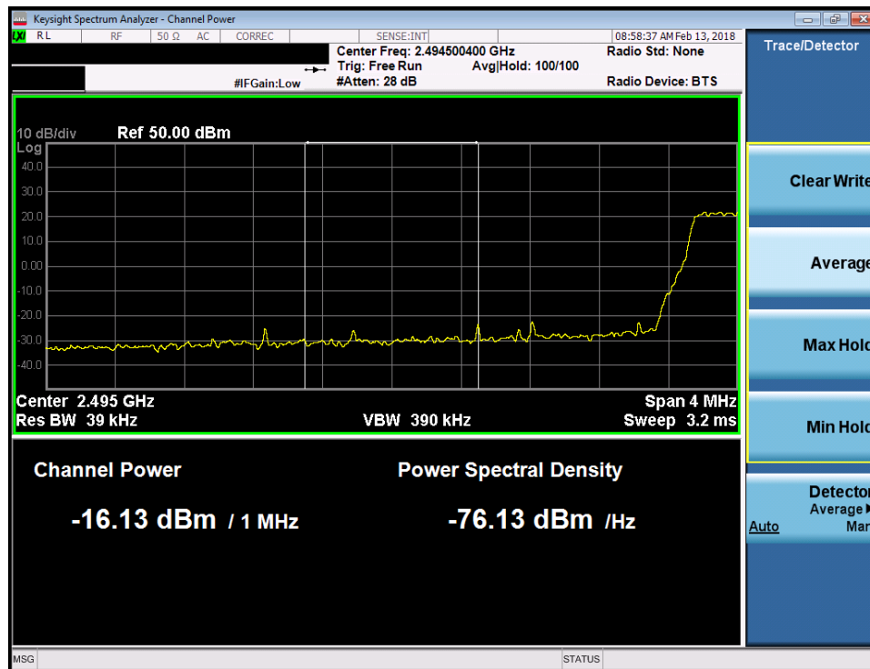
Plot 7-156. Lower Extended Band Edge Plot (Band 41 - 5.0MHz 64-QAM)
