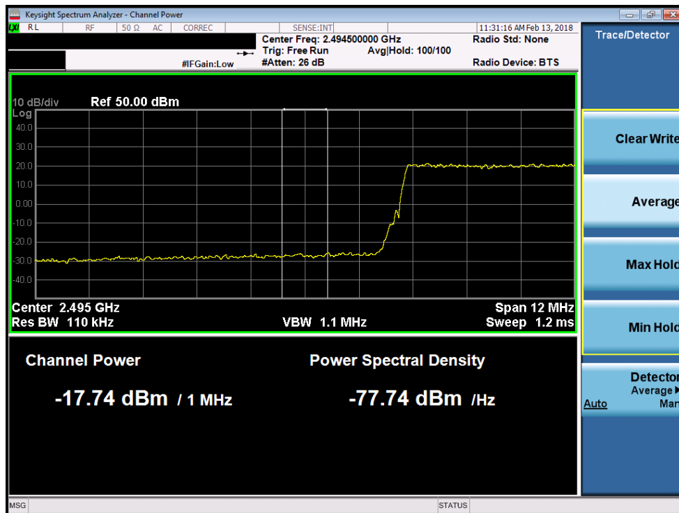
Plot 7-192. Lower Extended Band Edge Plot (Band 41 - 15.0MHz 256-QAM)
