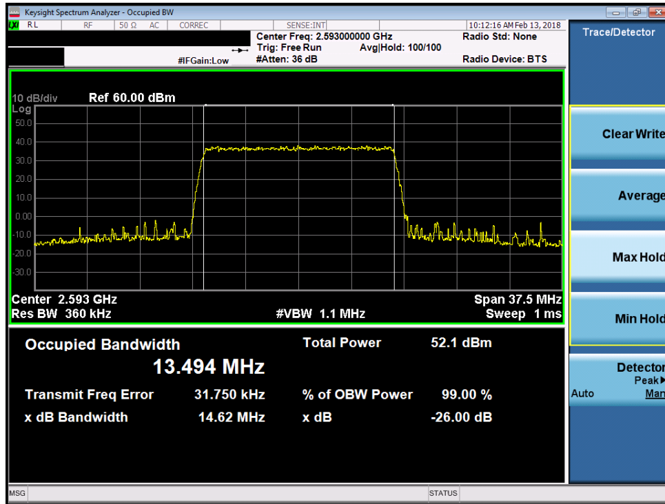
Plot 7-107. Occupied Bandwidth Plot (Band 41 - 15.0MHz 64-QAM)
