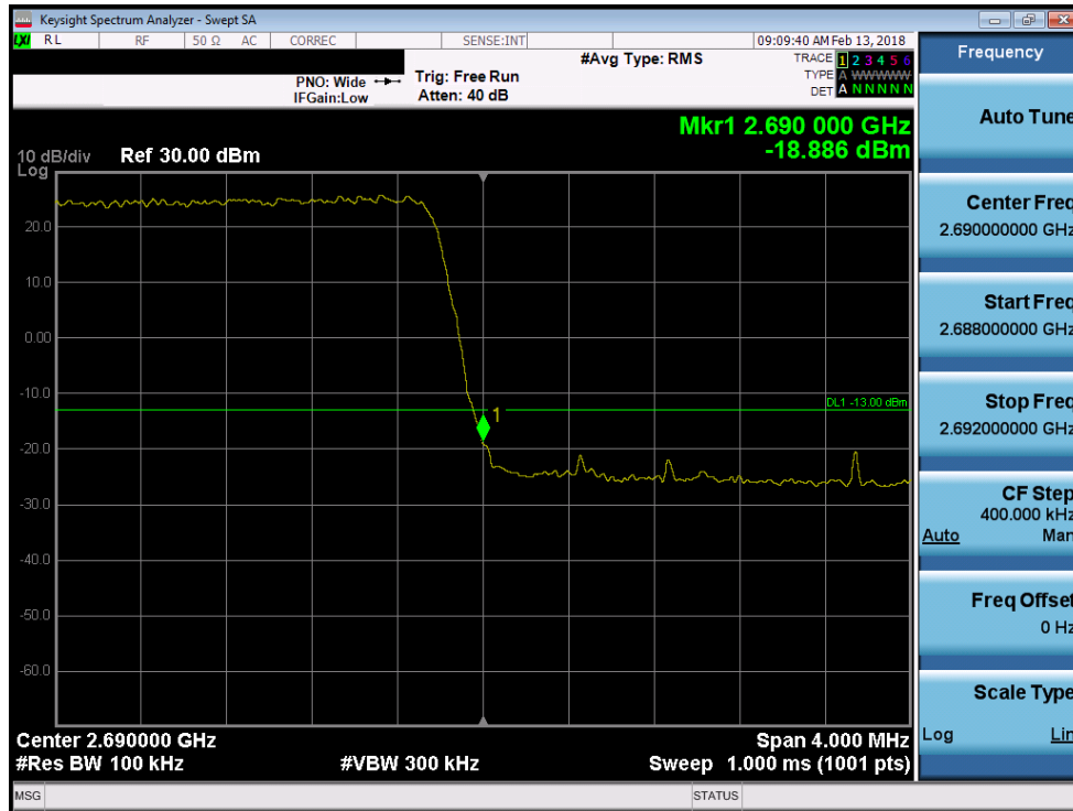
Plot 7-157. Upper Band Edge Plot (Band 41 - 5.0MHz 64-QAM)
