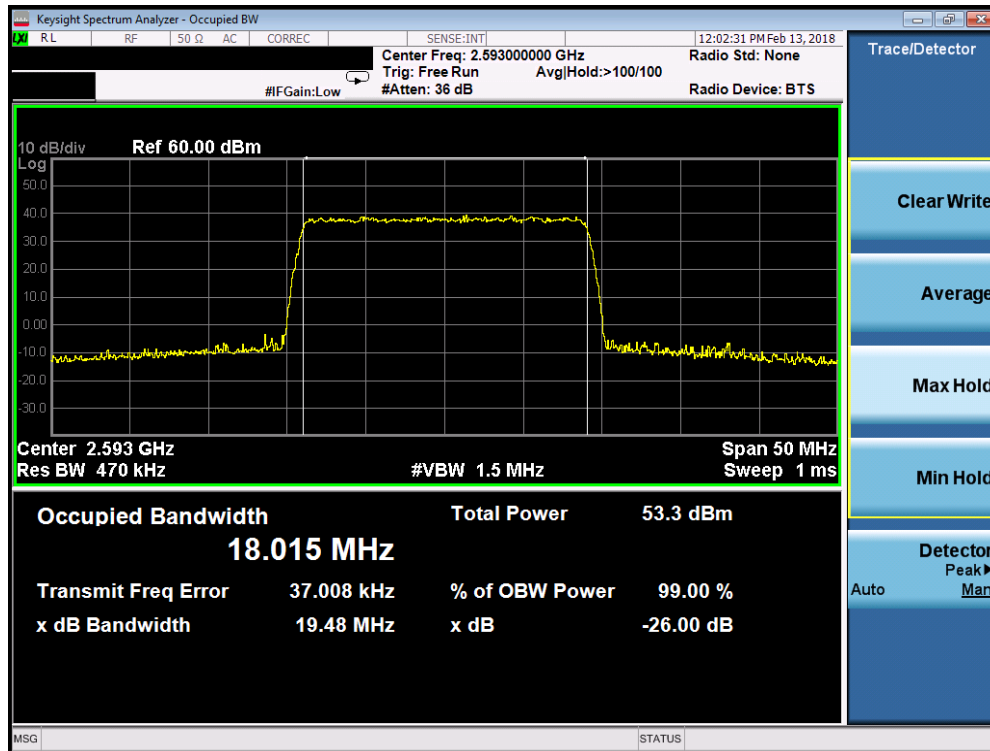
Plot 7-112. Occupied Bandwidth Plot (Band 41 - 20.0MHz 256-QAM)
