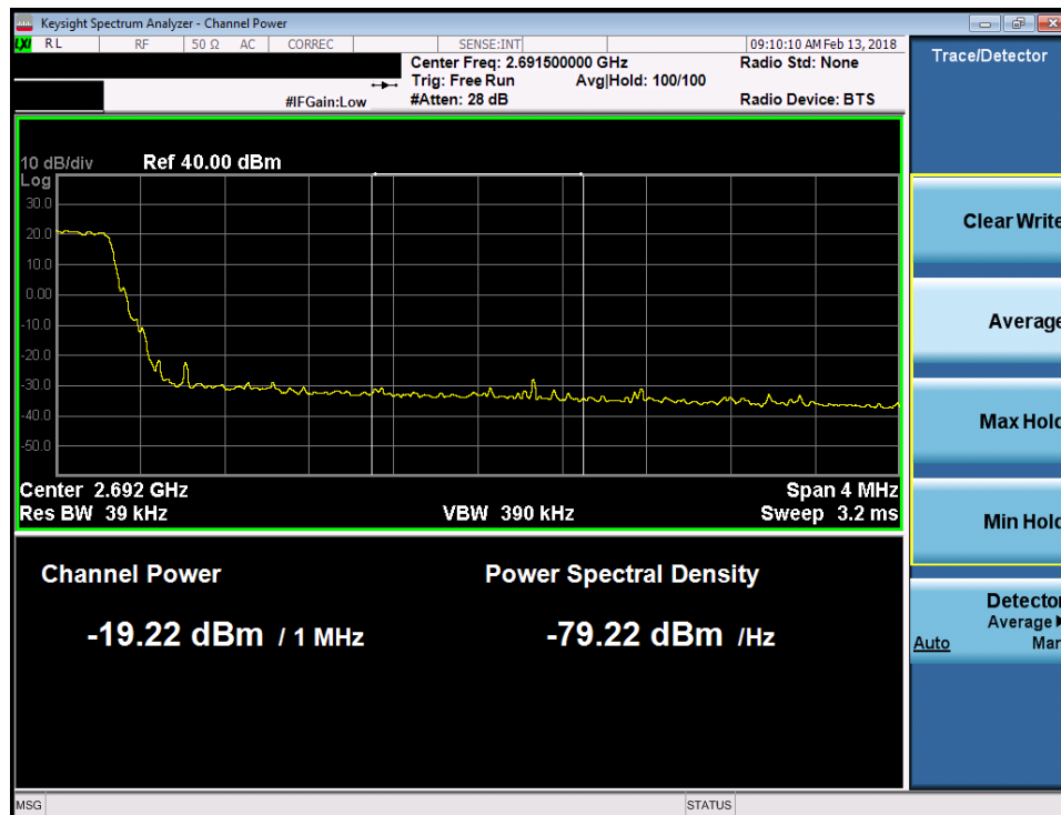
Plot 7-158. Upper Extended Band Edge Plot (Band 41 - 5.0MHz 64-QAM)
