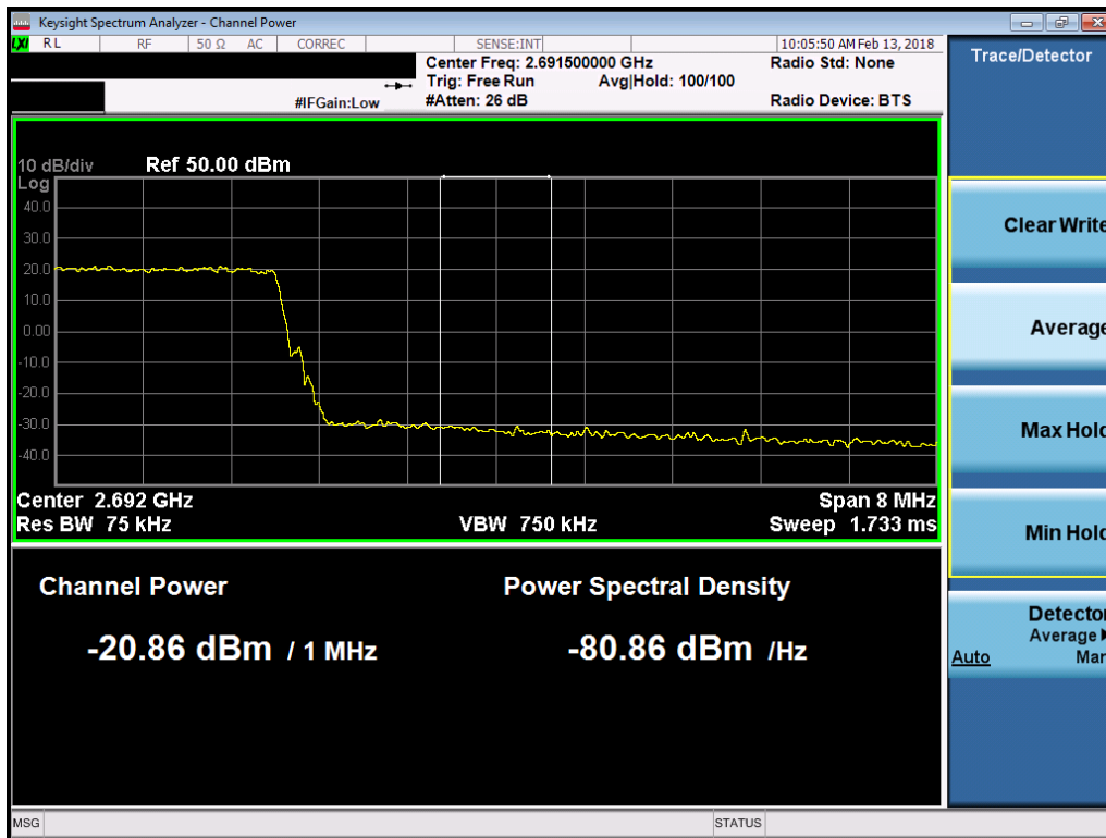
Plot 7-178. Upper Extended Band Edge Plot (Band 41 - 10.0MHz 256-QAM)
