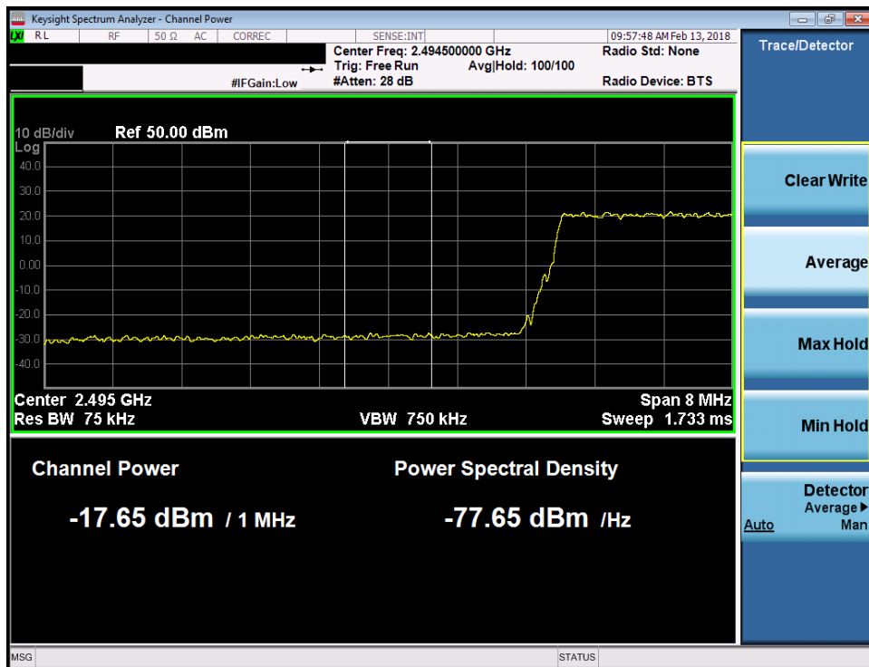
Plot 7-176. Lower Extended Band Edge Plot (Band 41 - 10.0MHz 256-QAM)
