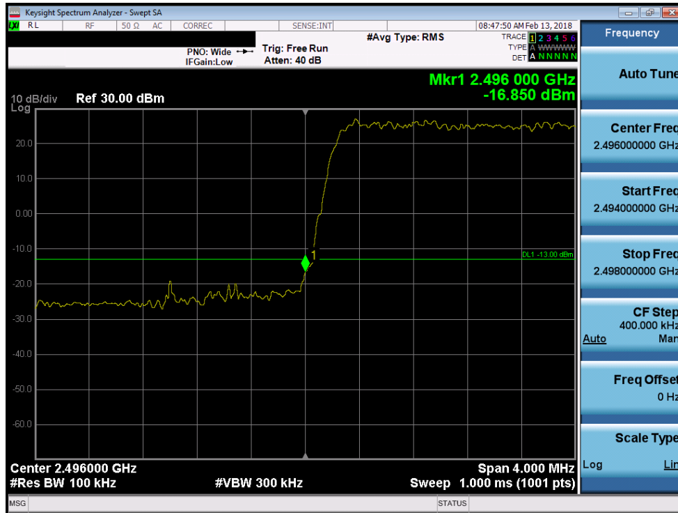
Plot 7-159. Lower Band Edge Plot (Band 41 - 5.0MHz 256-QAM)
