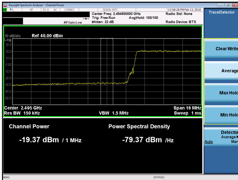
Plot 7-200. Lower Extended Band Edge Plot (Band 41 - 20.0MHz 16-QAM)
