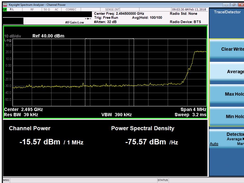
Plot 7-148. Lower Extended Band Edge Plot (Band 41 - 5.0MHz QPSK)
