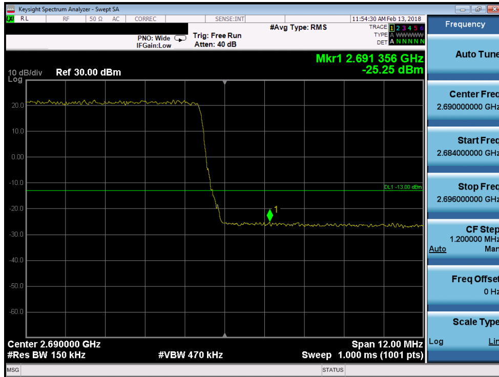
Plot 7-193. Upper Band Edge Plot (Band 41 - 15.0MHz 256-QAM)
