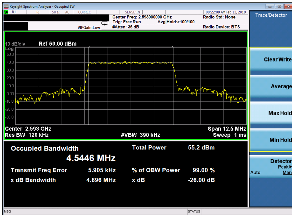
Plot 7-100. Occupied Bandwidth Plot (Band 41 - 5.0MHz 256-QAM)
