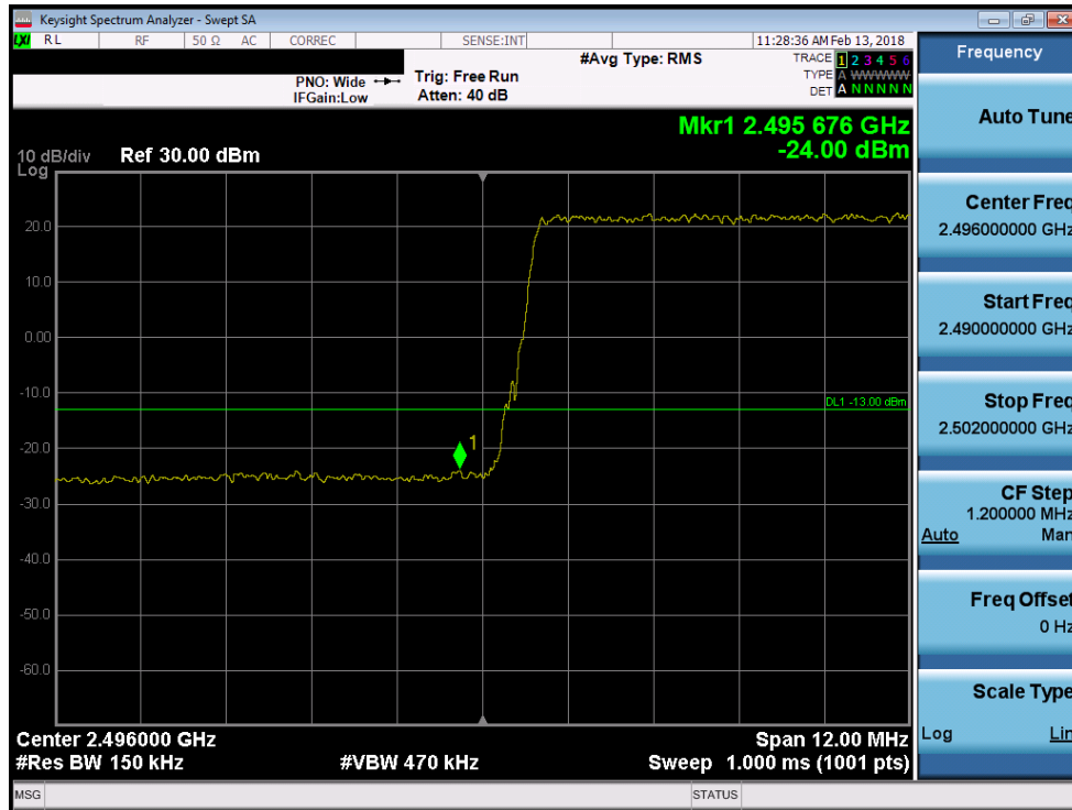
Plot 7-187. Lower Band Edge Plot (Band 41 - 15.0MHz 64-QAM)
