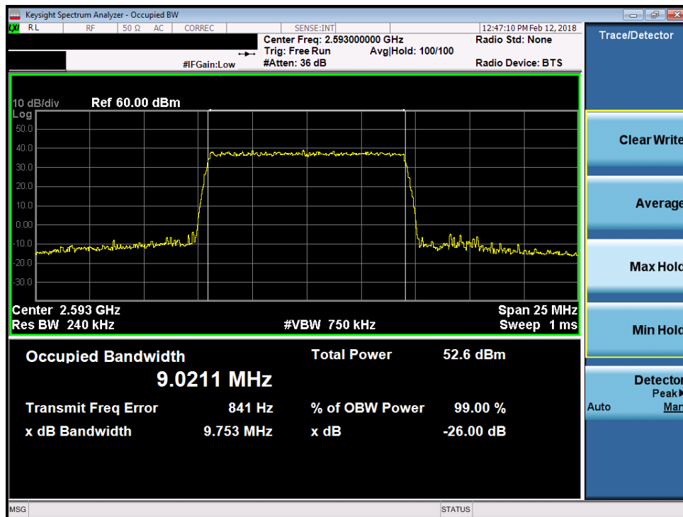
Plot 7-118. Occupied Bandwidth Plot (Band 41 - 10.0MHz 16-QAM)
