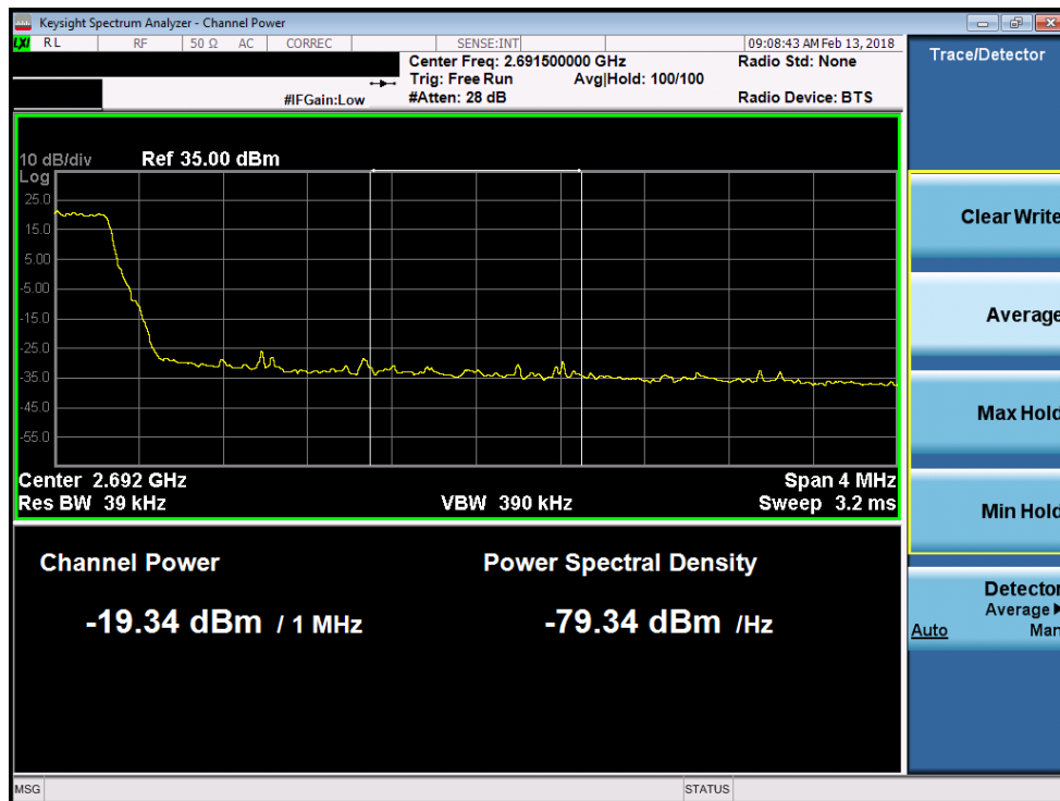
Plot 7-154. Upper Extended Band Edge Plot (Band 41 - 5.0MHz 16-QAM)
