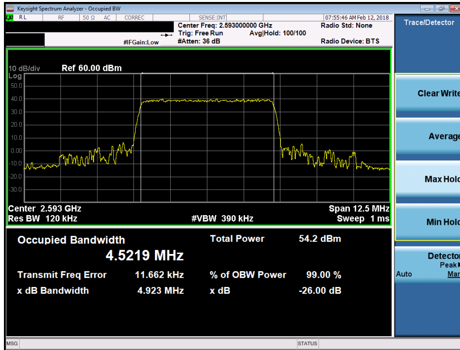
Plot 7-113. Occupied Bandwidth Plot (Band 41 - 5.0MHz QPSK)
