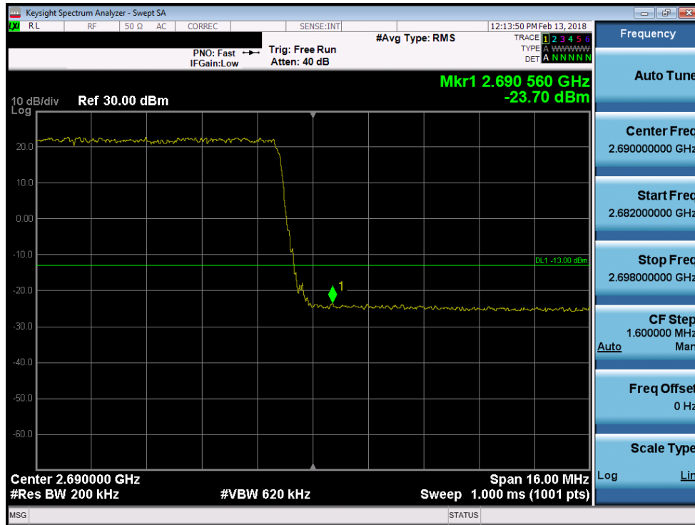
Plot 7-197. Upper Band Edge Plot (Band 41 - 20.0MHz QPSK)
