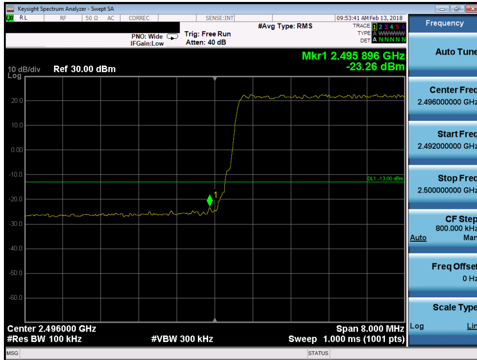
Plot 7-167. Lower Band Edge Plot (Band 41 - 10.0MHz 16-QAM)
