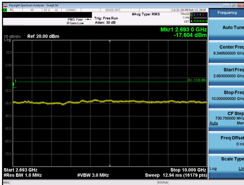
Plot 7-136. Conducted Spurious Plot (Band 41 - 5.0MHz QPSK – High Channel)
