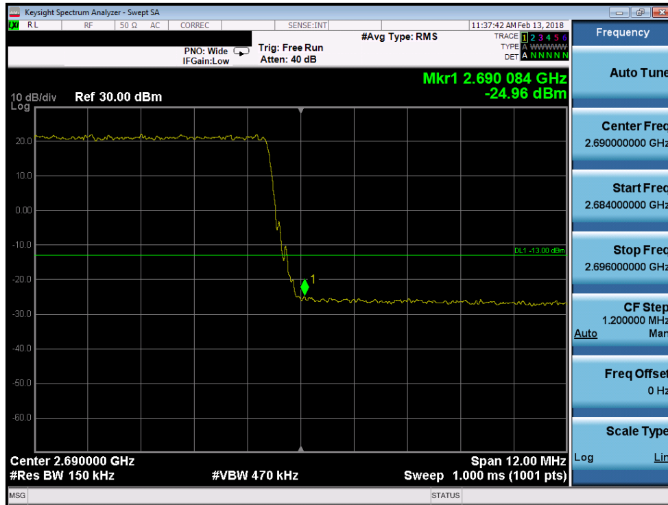
Plot 7-185. Upper Band Edge Plot (Band 41 - 15.0MHz 16-QAM)
