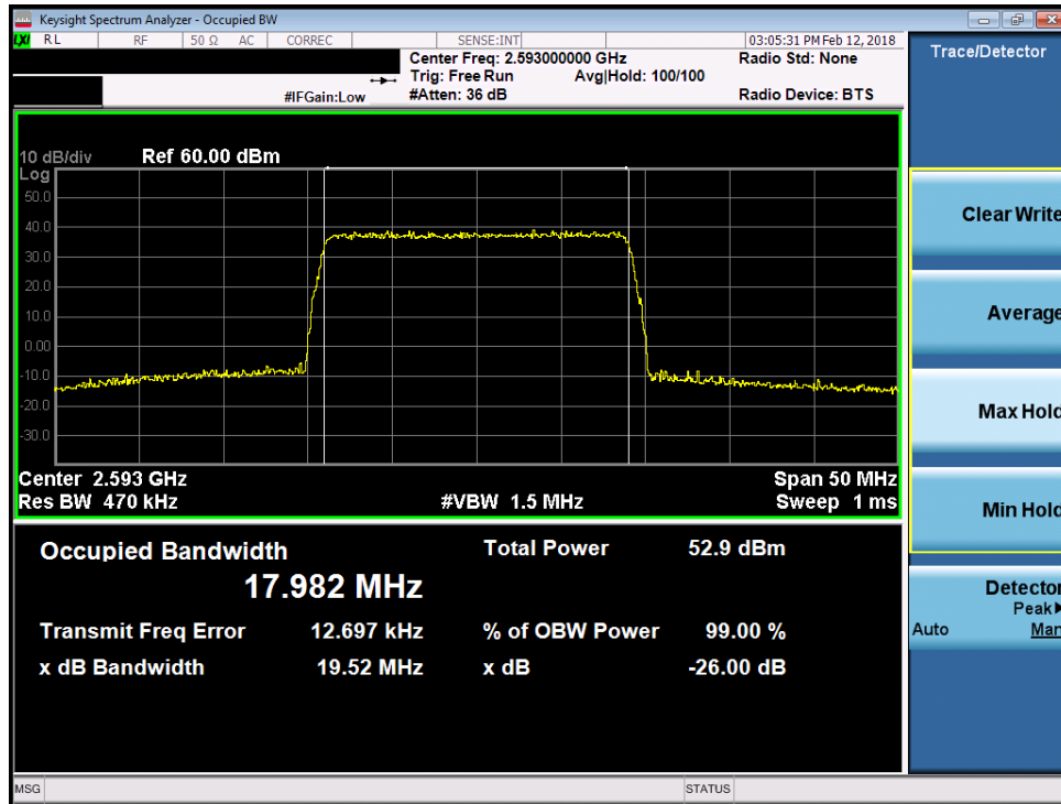
Plot 7-125. Occupied Bandwidth Plot (Band 41 - 20.0MHz QPSK)
