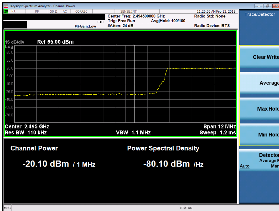
Plot 7-184. Lower Extended Band Edge Plot (Band 41 - 15.0MHz 16-QAM)
