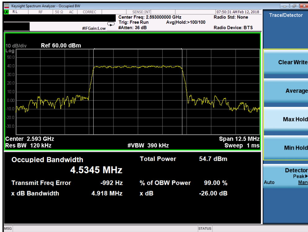
Plot 7-116. Occupied Bandwidth Plot (Band 41 - 5.0MHz 256-QAM)
