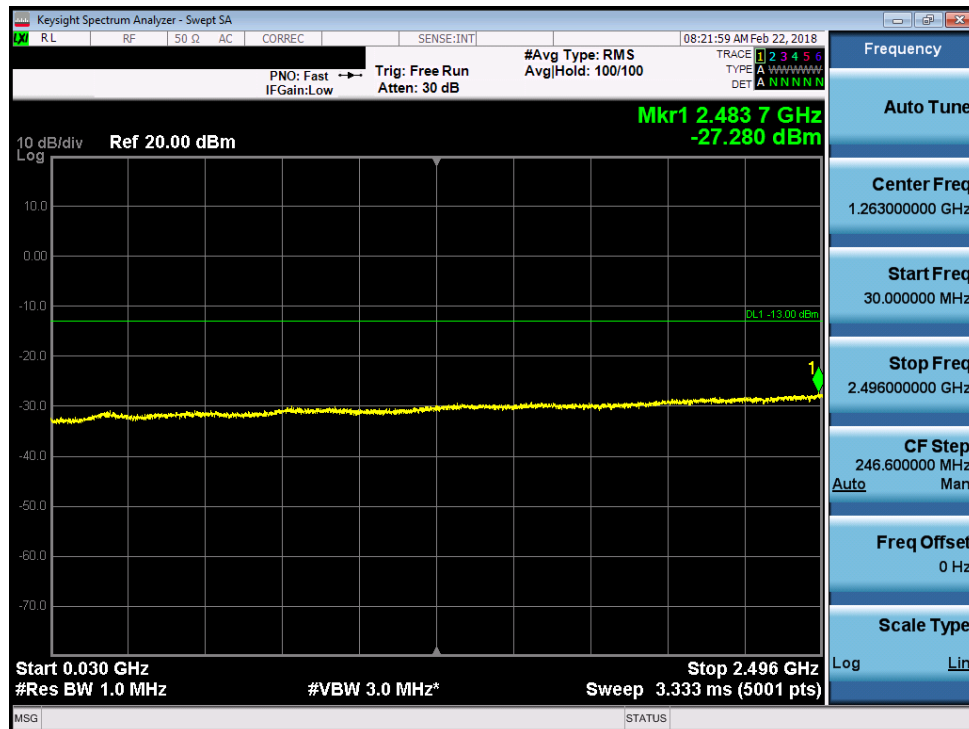
Plot 7-141. Conducted Spurious Plot (Band 41 - 5.0MHz QPSK – Mid Channel)
