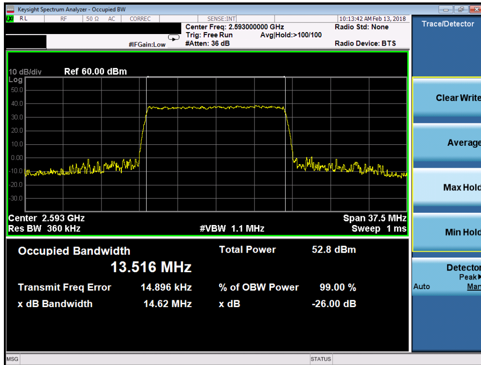
Plot 7-108. Occupied Bandwidth Plot (Band 41 - 15.0MHz 256-QAM)
