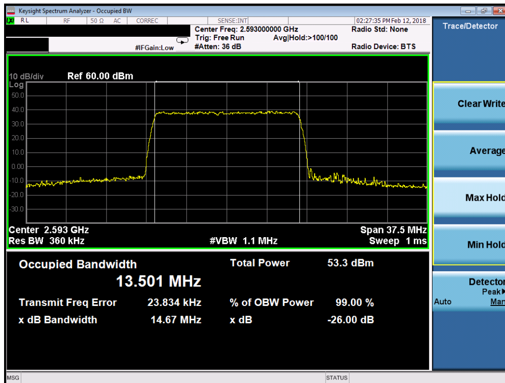
Plot 7-124. Occupied Bandwidth Plot (Band 41 - 15.0MHz 256-QAM)
