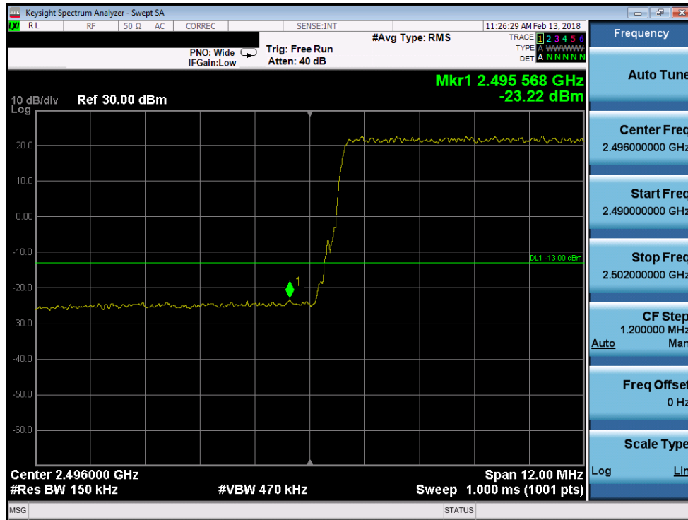
Plot 7-183. Lower Band Edge Plot (Band 41 - 15.0MHz 16-QAM)
