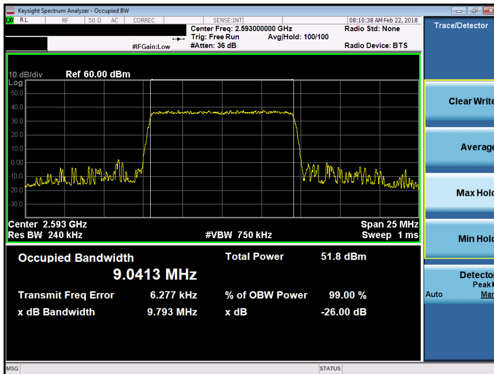
Plot 7-102. Occupied Bandwidth Plot (Band 41 - 10.0MHz 16-QAM)
