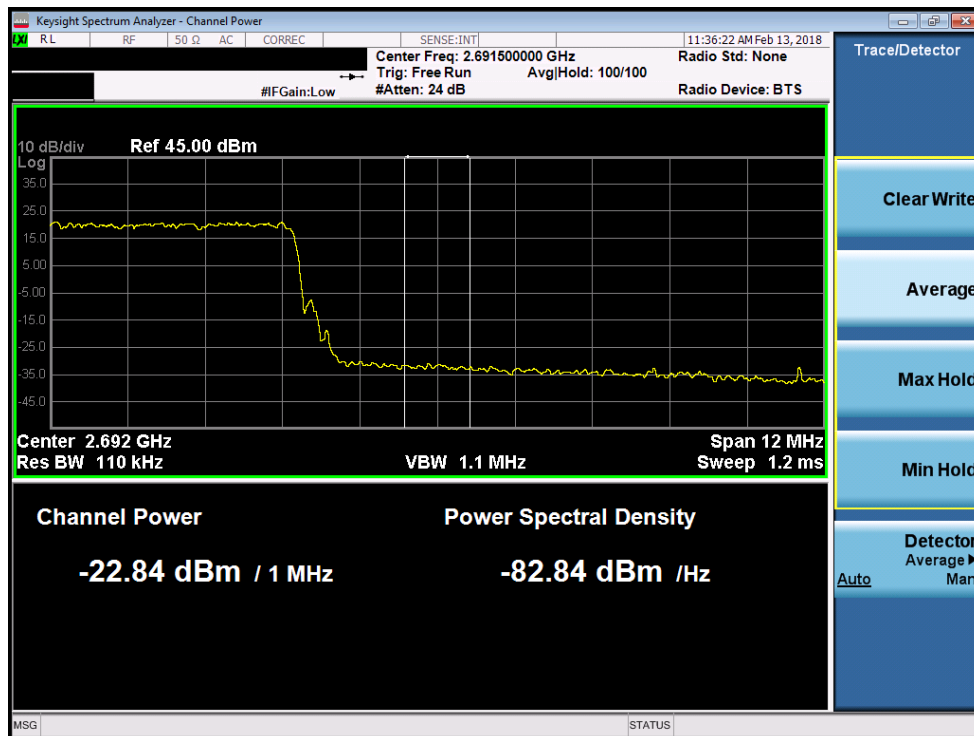
Plot 7-182. Upper Extended Band Edge Plot (Band 41 - 15.0MHz QPSK)
