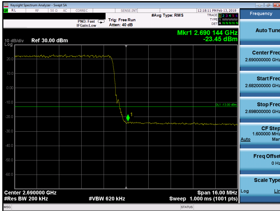
Plot 7-209. Upper Band Edge Plot (Band 41 - 20.0MHz 256-QAM)
