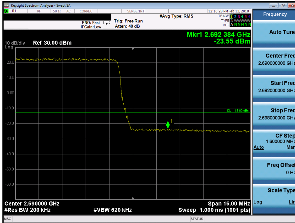
Plot 7-205. Upper Band Edge Plot (Band 41 - 20.0MHz 64-QAM)
