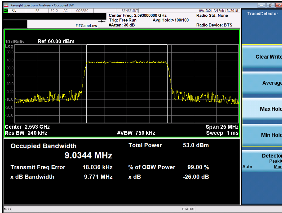
Plot 7-101. Occupied Bandwidth Plot (Band 41 - 10.0MHz QPSK)
