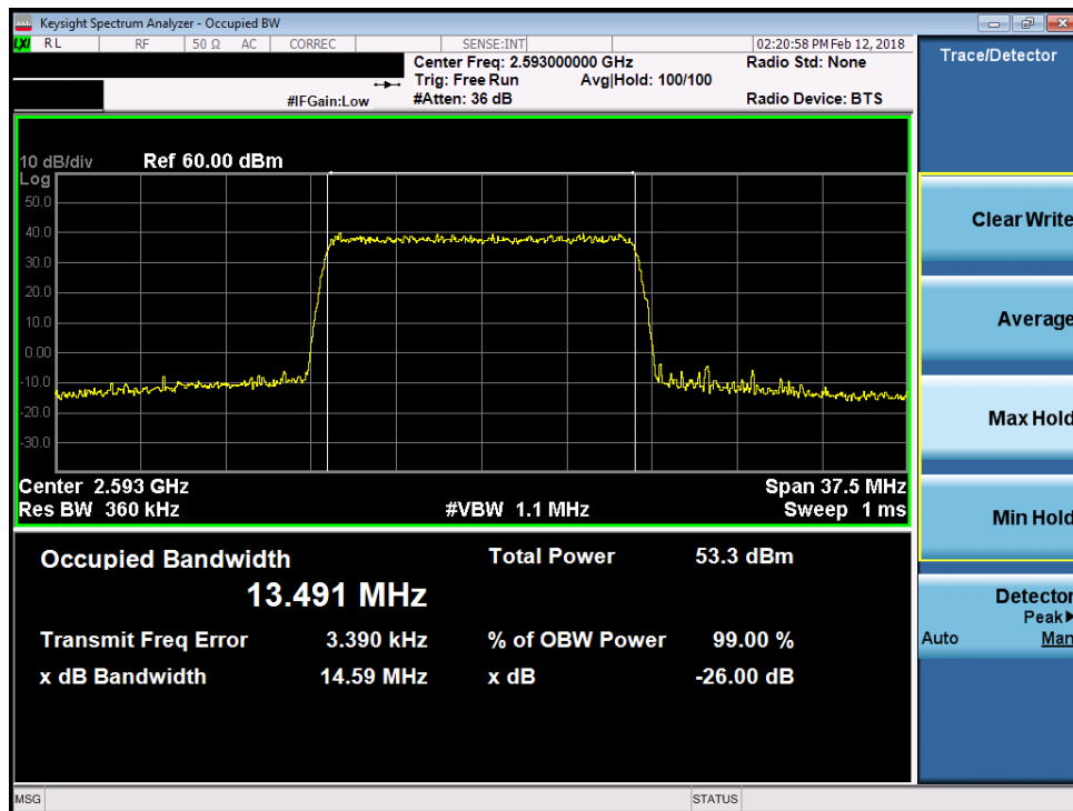
Plot 7-122. Occupied Bandwidth Plot (Band 41 - 15.0MHz 16-QAM)
