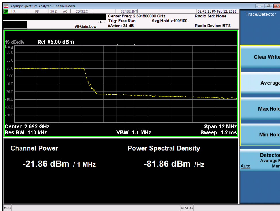
Plot 7-250. Upper Extended Band Edge Plot (Band 41 - 15.0MHz 16-QAM)
