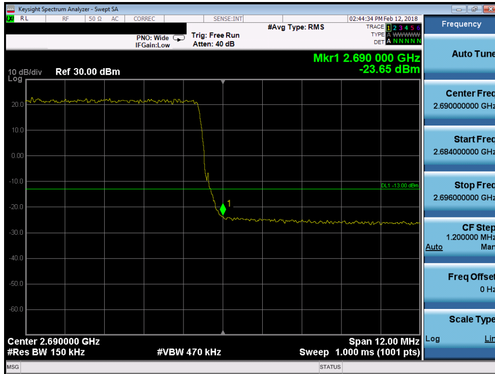
Plot 7-253. Upper Band Edge Plot (Band 41 - 15.0MHz 64-QAM)
