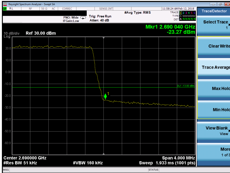
Plot 7-213. Upper Band Edge Plot (Band 41 - 5.0MHz QPSK)
