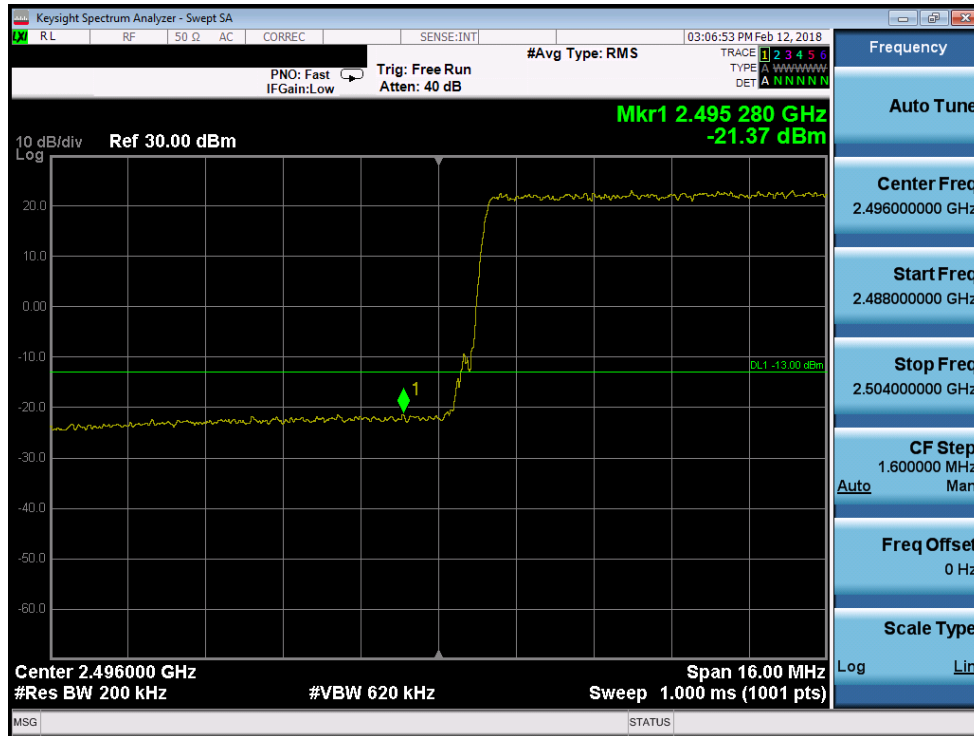
Plot 7-259. Lower Band Edge Plot (Band 41 - 20.0MHz QPSK)
