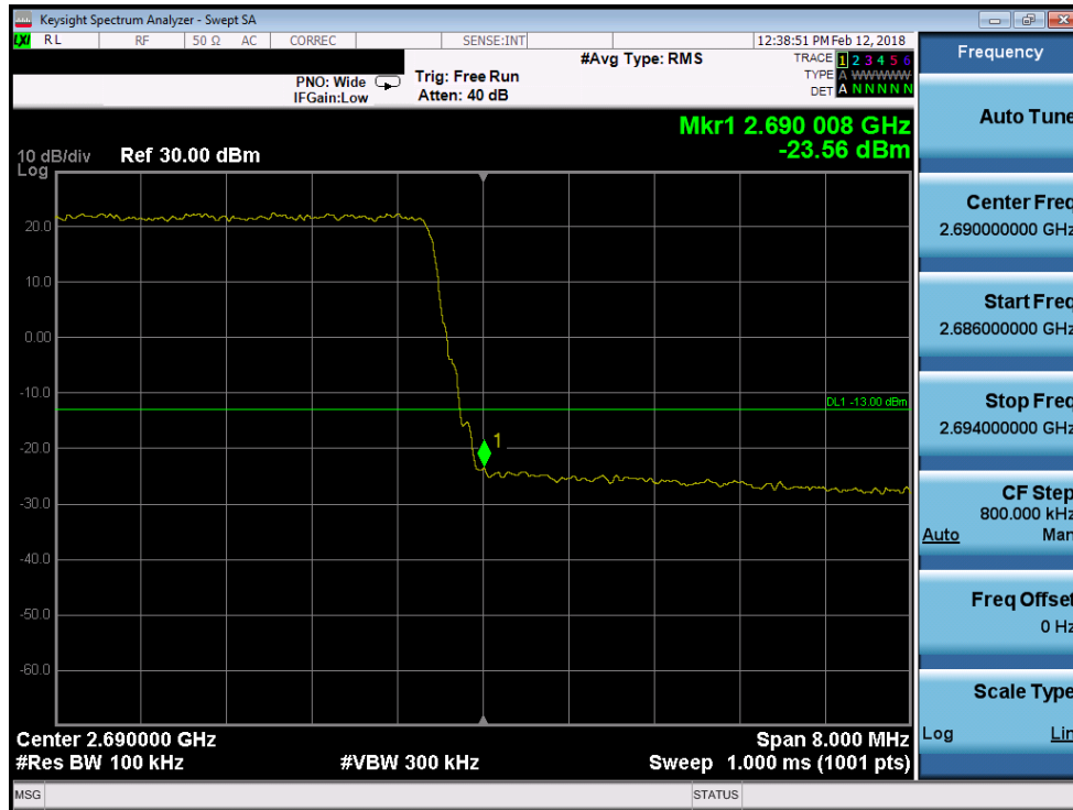
Plot 7-233. Upper Band Edge Plot (Band 41 - 10.0MHz 16-QAM)
