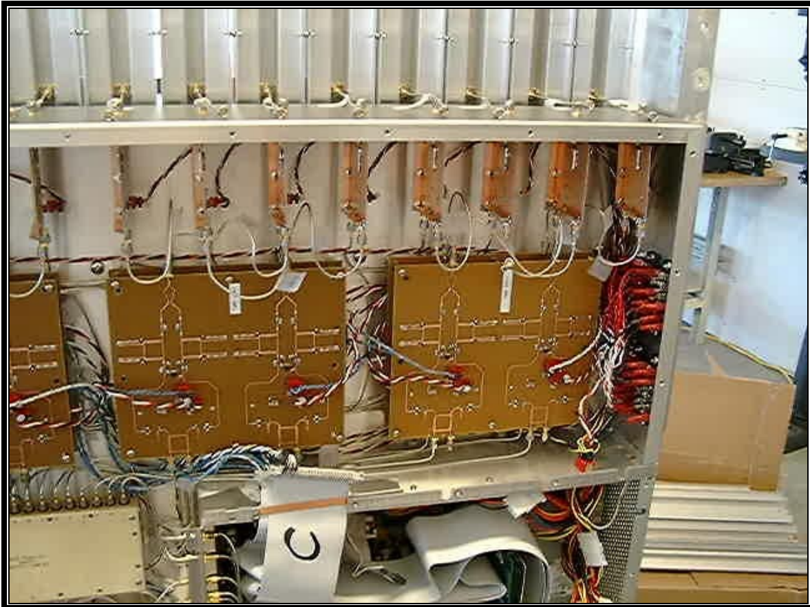
PHOTOGRAPH 14: INSIDE THE BOX – RIGHT SIDE
