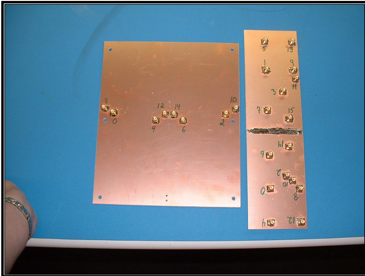
PHOTOGRAPH 26: BUTLER MATRIX BACK
