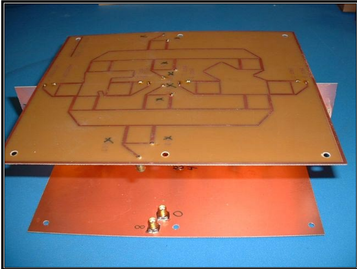
PHOTOGRAPH 27: BUTLER MATRIX ASSEMBLED
