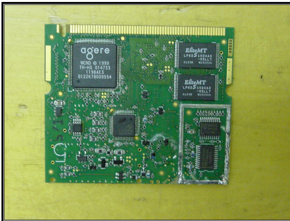
PHOTOGRAPH 22: AGERE MINIPCI RADIO BOTTOM WITHOUT SHIELD
