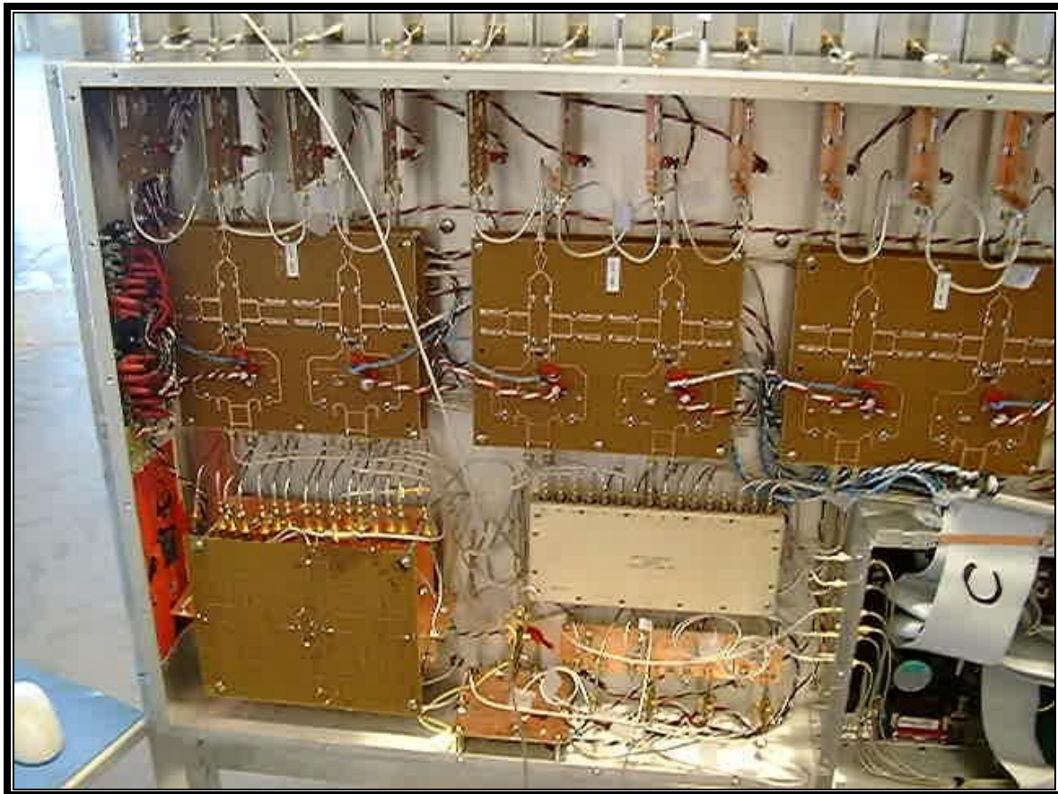
PHOTOGRAPH 13: INSIDE THE BOX – LEFT SIDE
