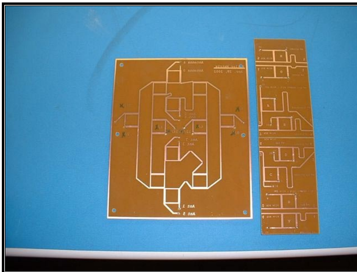
PHOTOGRAPH 25: BUTLER MATRIX FRONT
