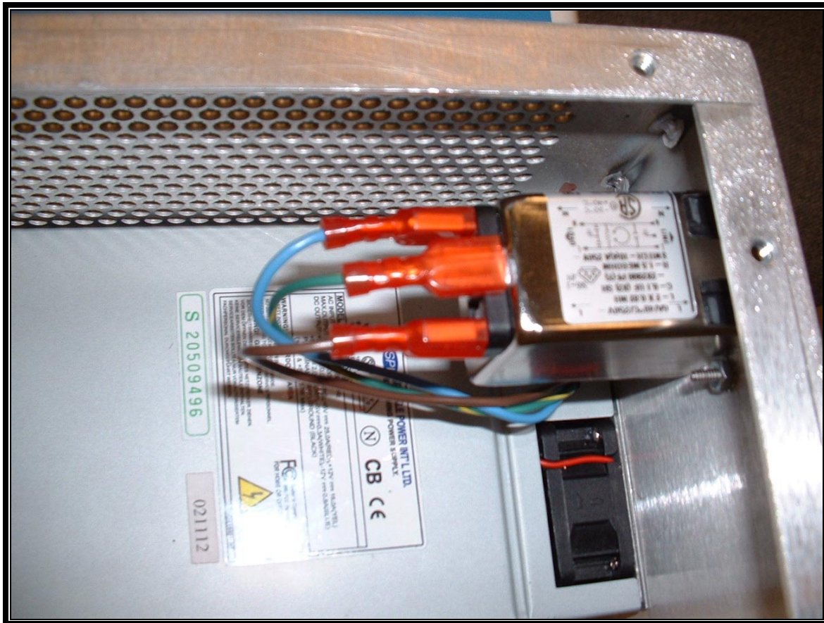
PHOTOGRAPH 16: AC LINE FILTER IMPLEMENTATION #2
