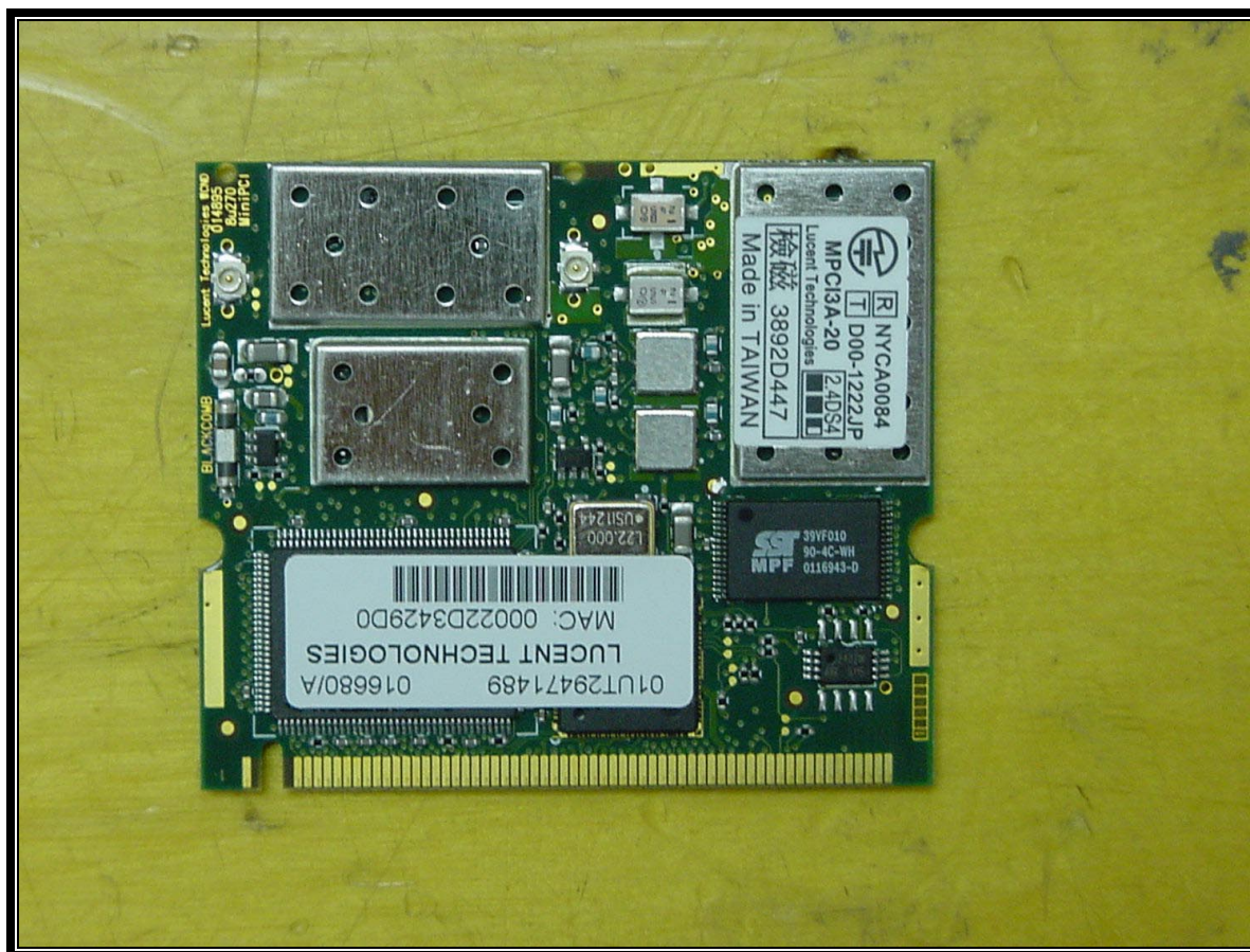
PHOTOGRAPH 19: AGERE MINIPCI RADIO TOP WITH SHIELDS
