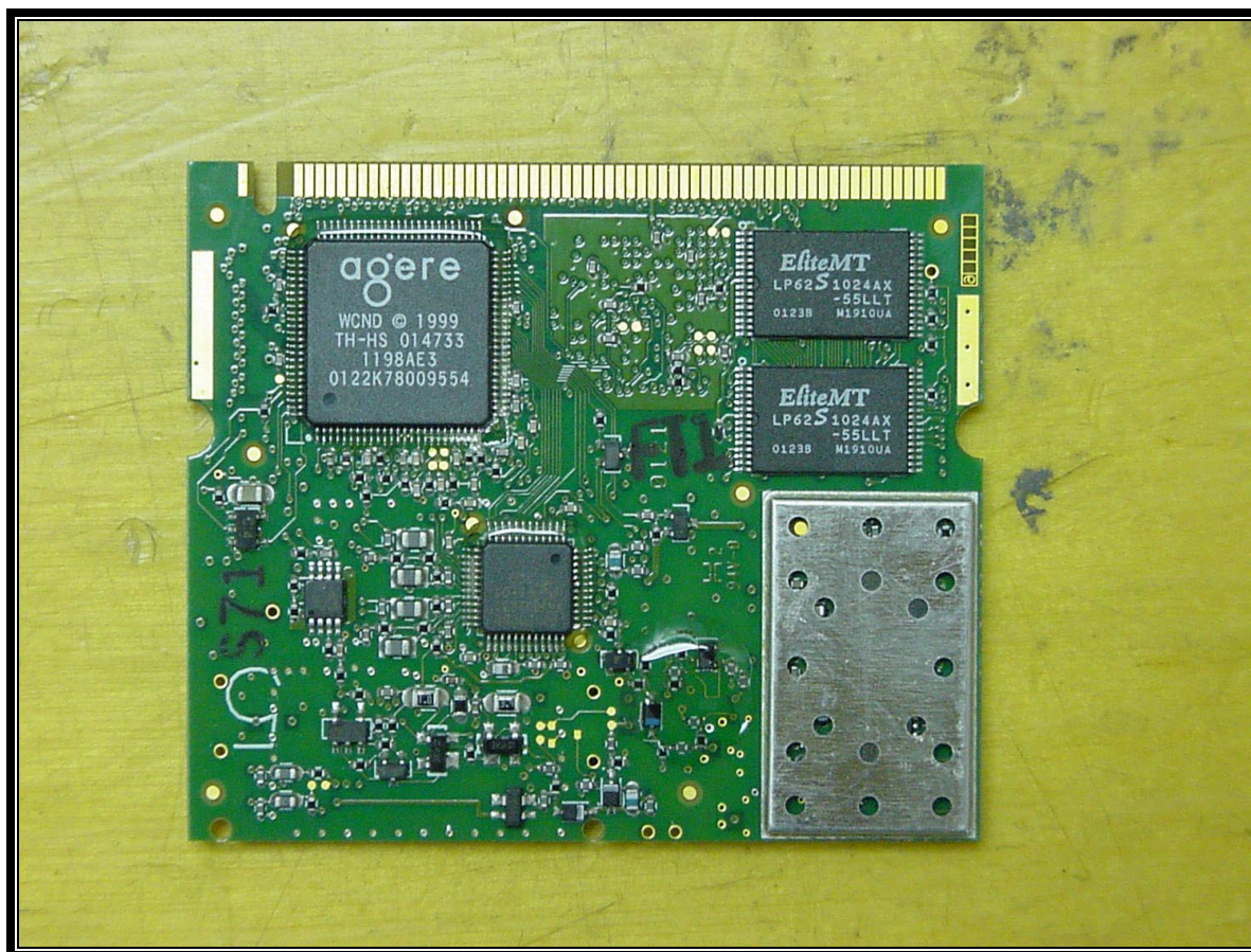
PHOTOGRAPH 20: AGERE MINIPCI RADIO BOTTOM WITH SHIELD
