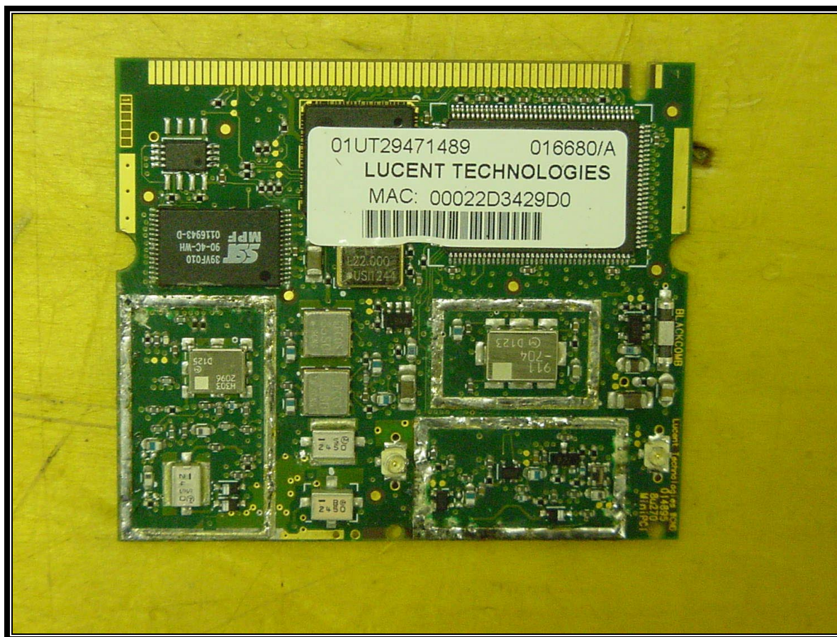
PHOTOGRAPH 21: AGERE MINIPCI RADIO TOP WITHOUT SHIELDS
