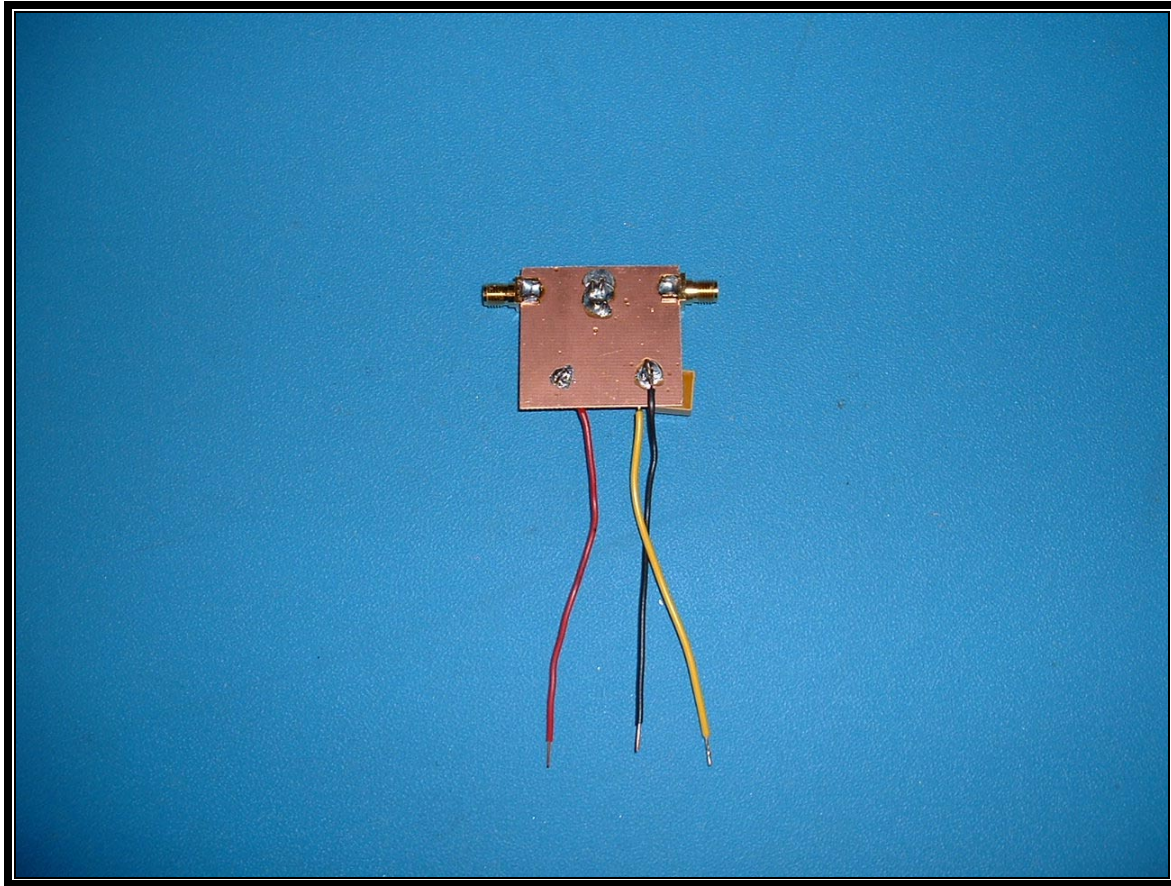
PHOTOGRAPH 38: LNA BOTTOM
