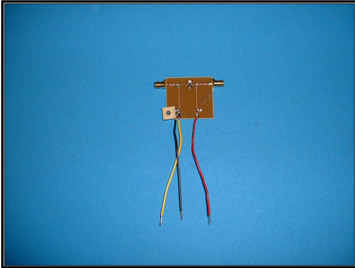
PHOTOGRAPH 37: LNA TOP
