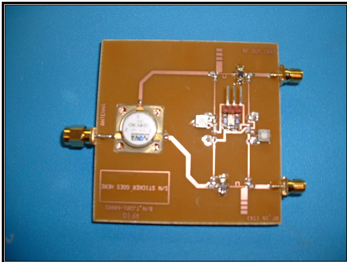
PHOTOGRAPH 46: RFIO TOP
