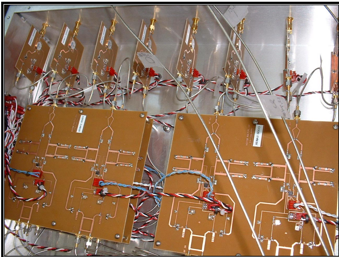
PHOTOGRAPH 55: VM'S AND RFIO'S INSTALLED
