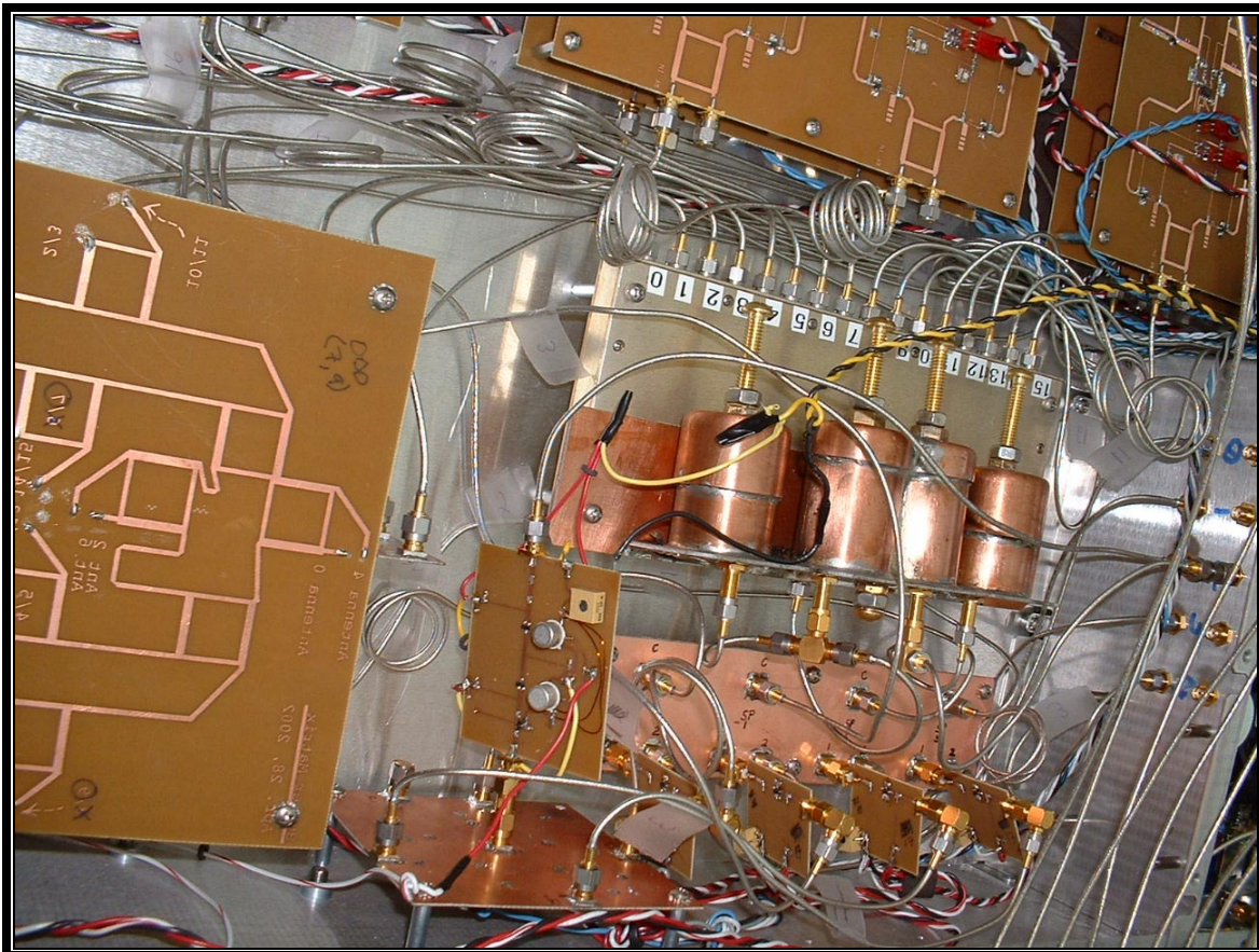
PHOTOGRAPH 45: RX ASSEMBLY WITH PIN DIODE ATTENUATOR
