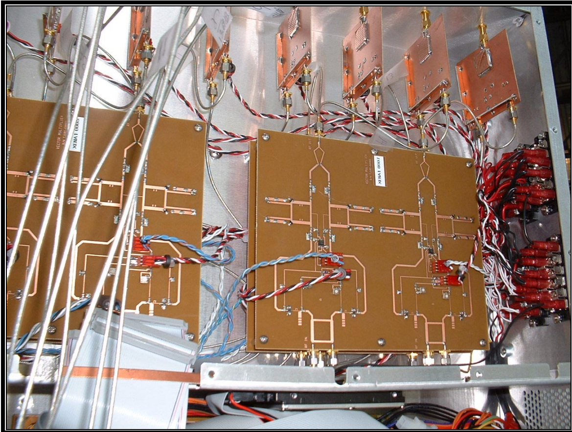
PHOTOGRAPH 56: VM'S AND DC POWER CONNECTIONS
