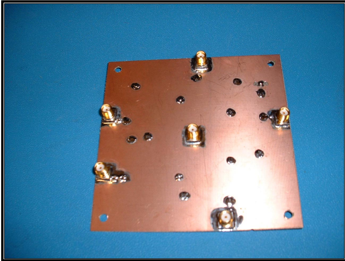
PHOTOGRAPH 44: PIN DIODE SWITCH BOTTOM
