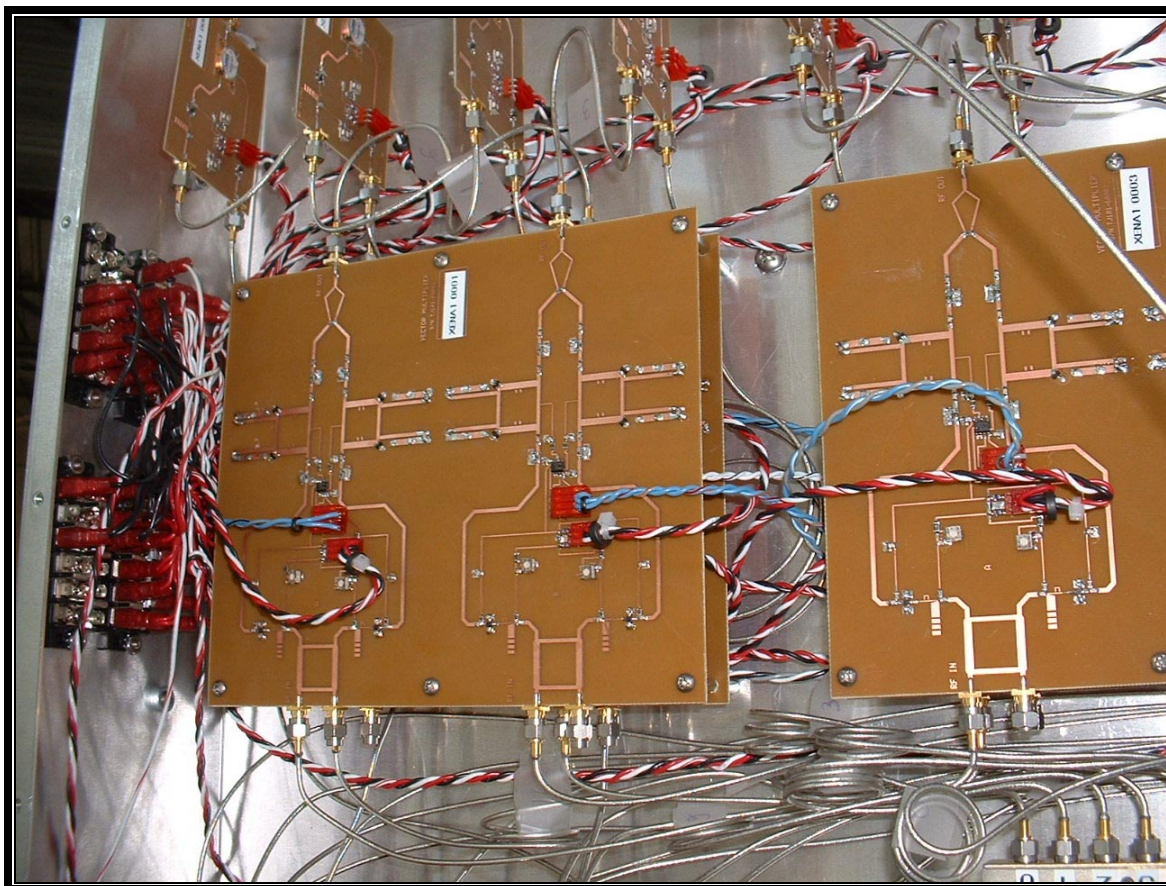
PHOTOGRAPH 52: VECTOR MULTIPLIER INSTALLED
