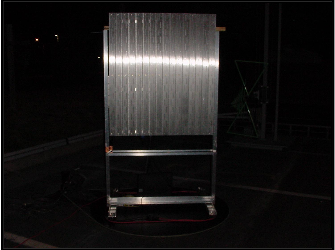
PHOTOGRAPH 3: RADIATED EMISSION FRONT VIEW WORST-CASE CONFIGURATION
