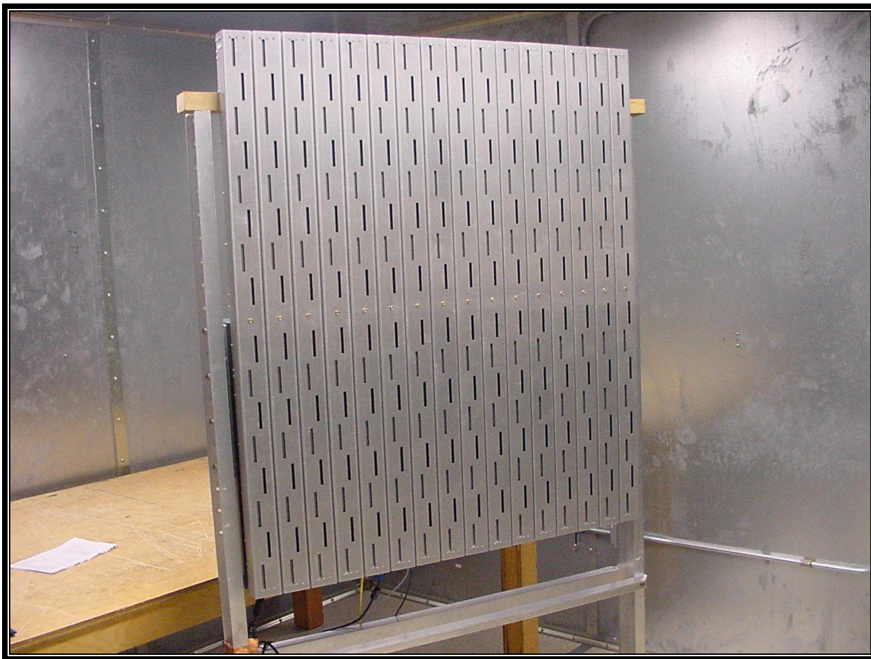
PHOTOGRAPH 5: CONDUCTED EMISSION FRONT VIEW WORST-CASE CONFIGURATION
