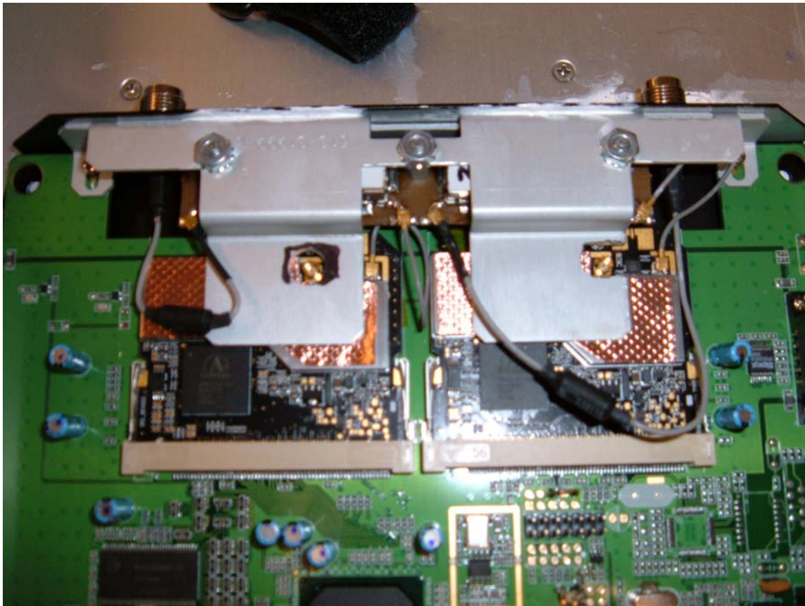
Figure 5 - Digital Board with Radios, Heat Sink, & Filters
