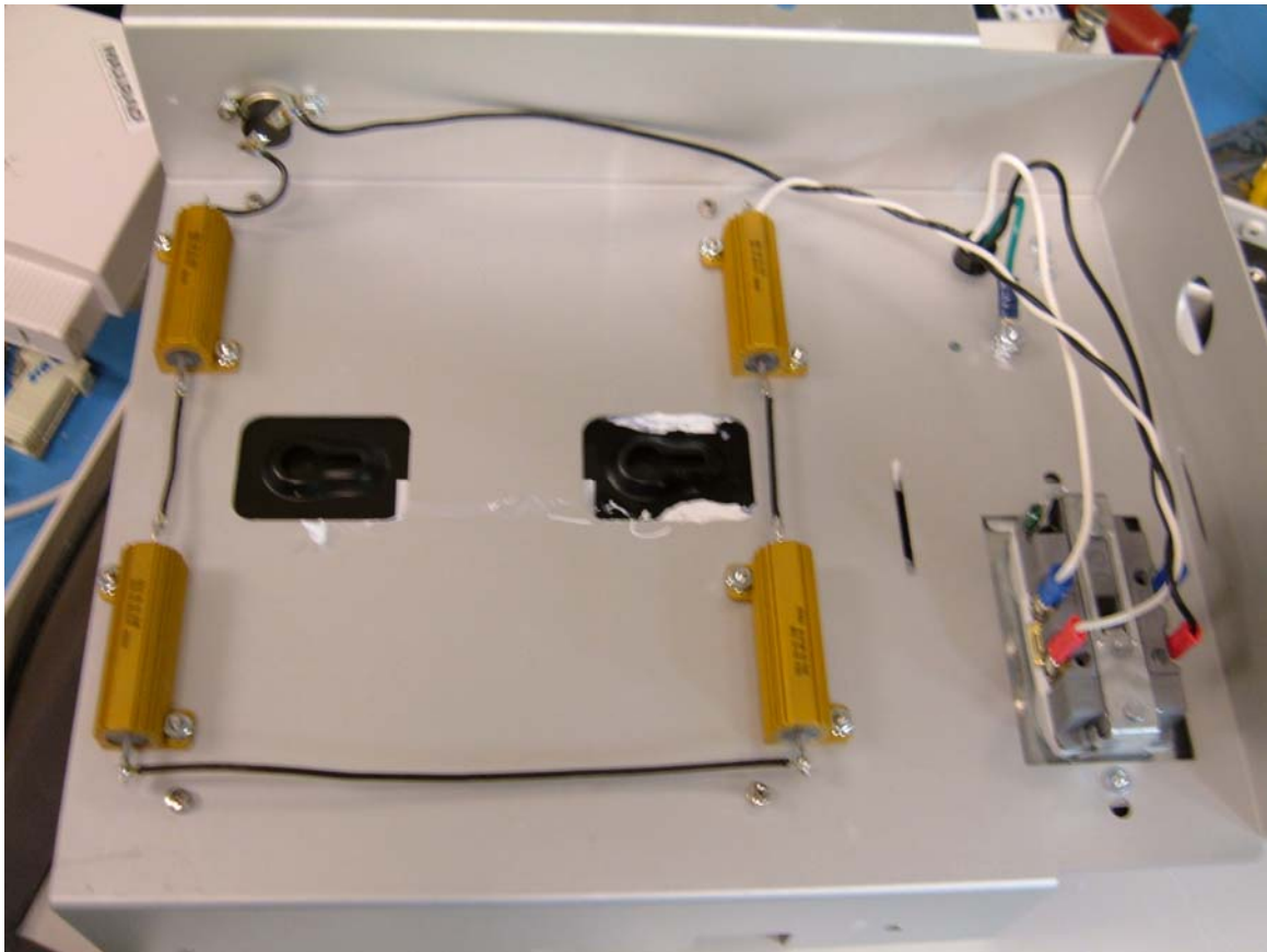
Figure 8 - Heater Resistors
