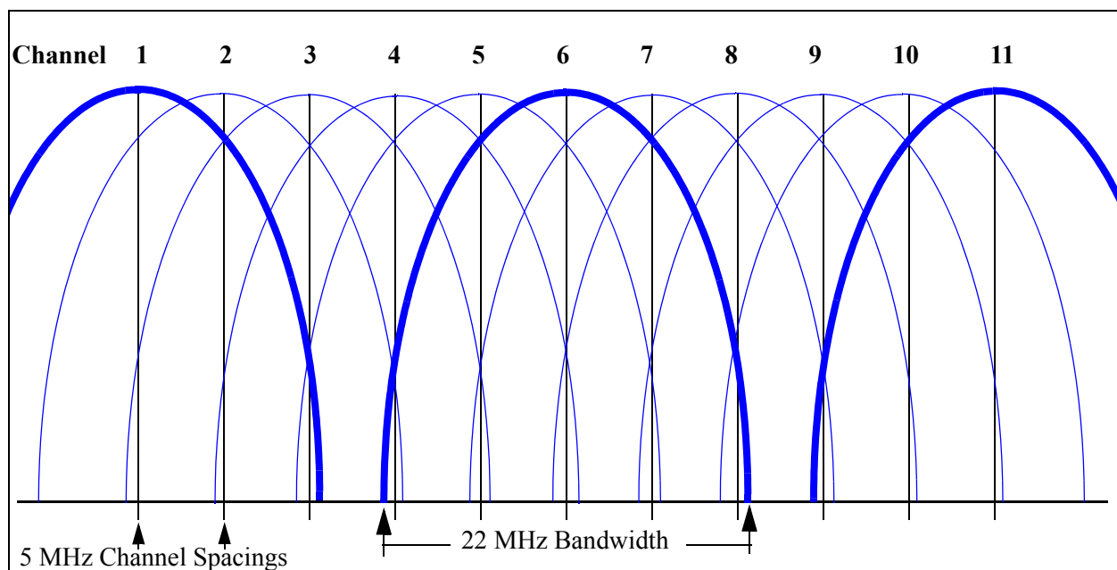
Figure 10—ISM Band Channel Spacings for Channels 1 to 11
