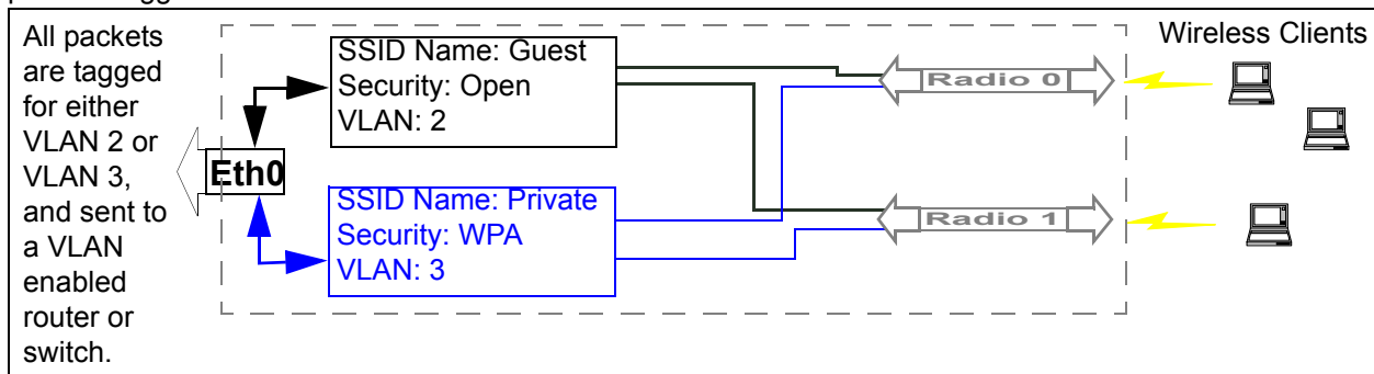
Figure 5 Creating Two Separate Networks Using VLANs
