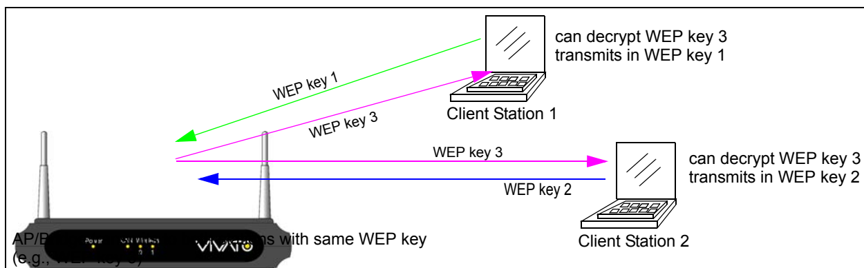
Figure 8 Example of Using Multiple WEP Keys and Transfer Key Index on Client Stations
