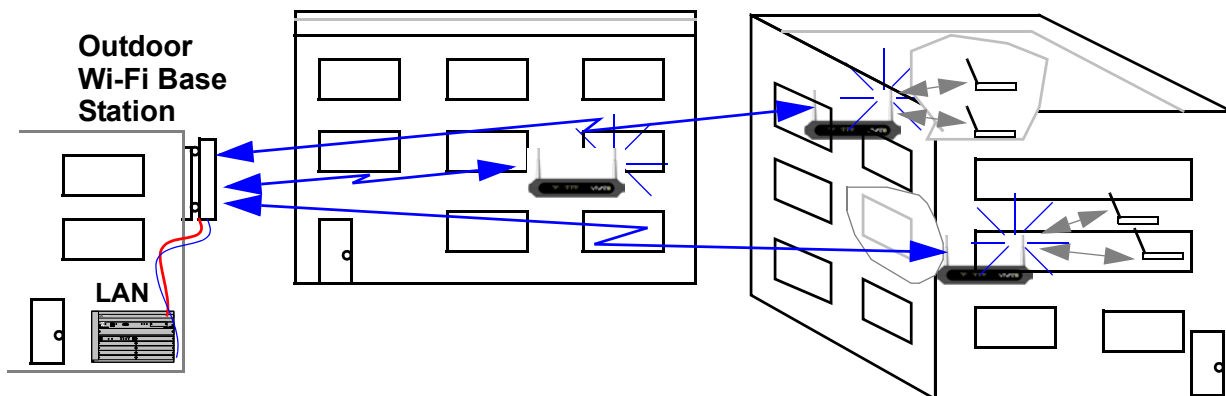
Figure 4—Wireless Backhaul to AP/Bridge Example
