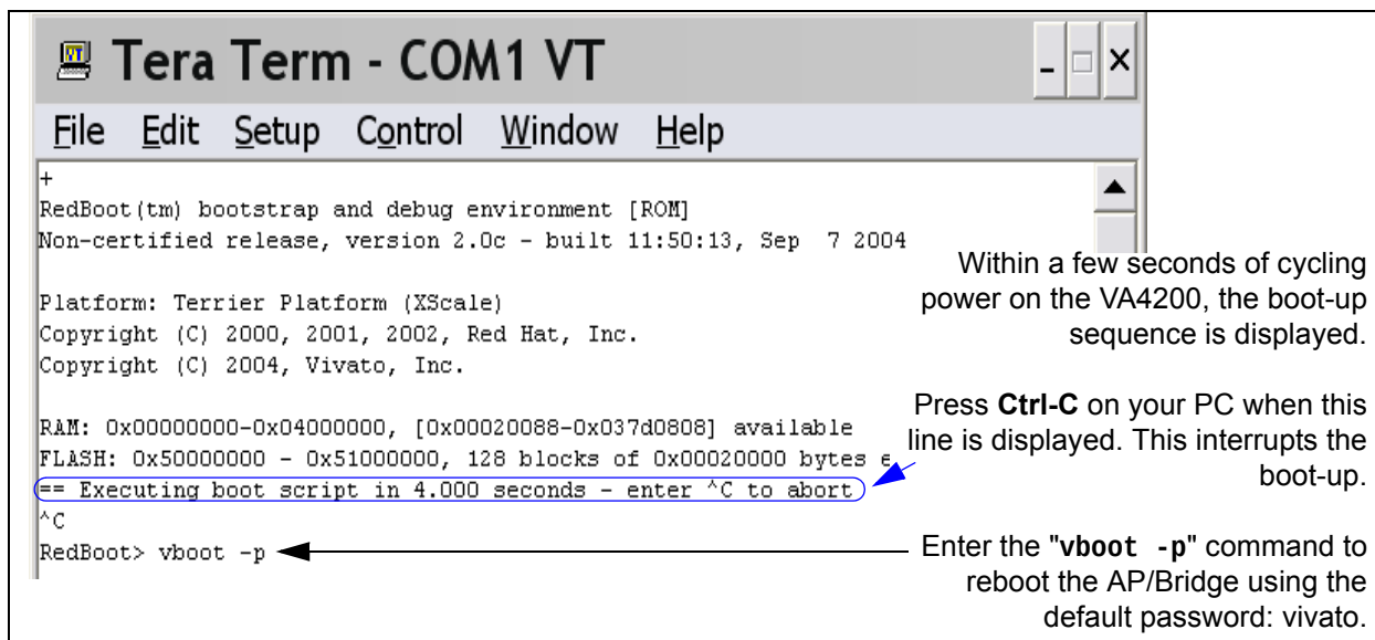
Figure 9—Accessing the Bootloader by Interrupting the Boot Sequence
