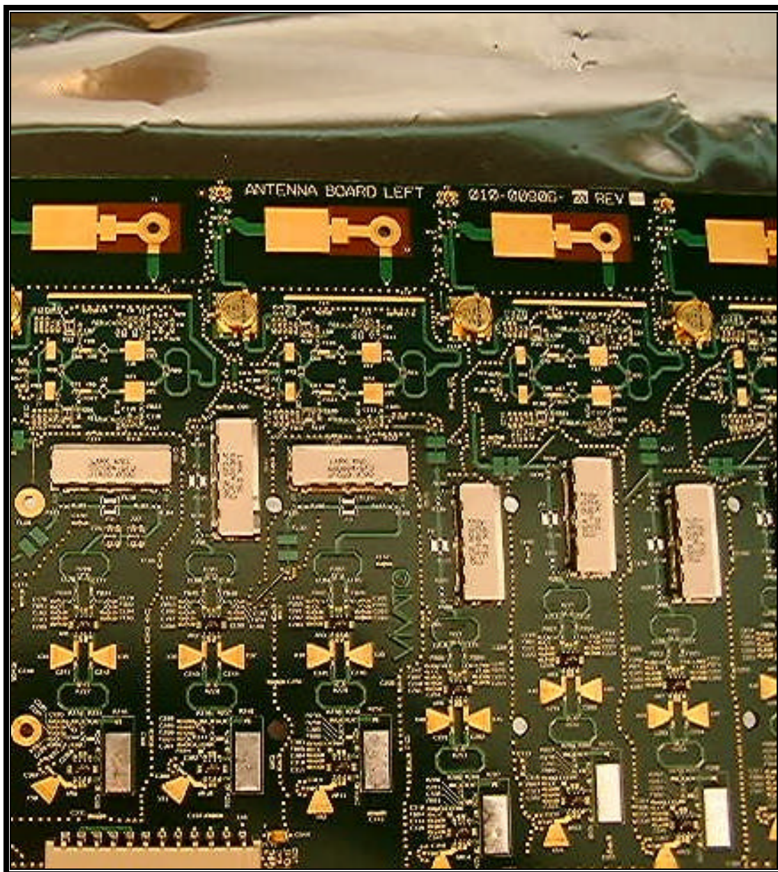
PHOTOGRAPH 33: LEFT ANTENNA BOARD TOP VIEW LEFT HALF
