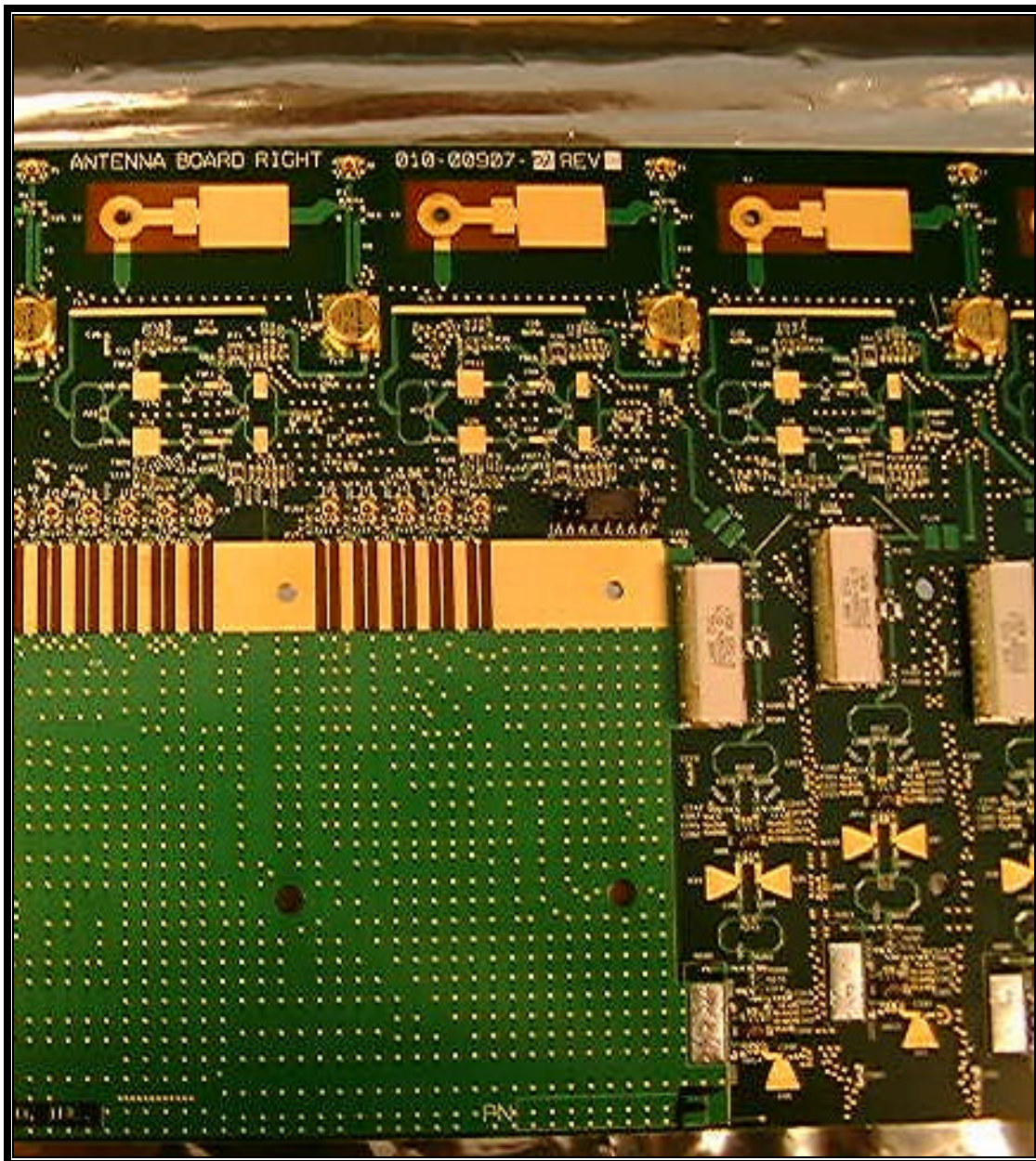
PHOTOGRAPH 35: RIGHT ANTENNA BOARD-LEFT HALF
