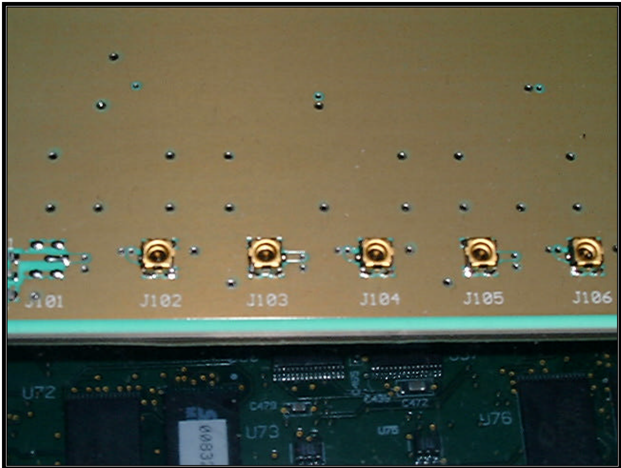
PHOTOGRAPH 22: ALFRED BOARD CONNECTORS
