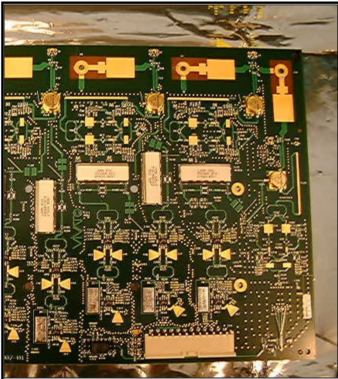
PHOTOGRAPH 36: RIGHT ANTENNA BOARD-RIGHT HALF
