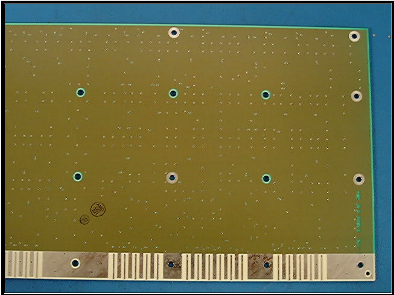
PHOTOGRAPH 18: ALFRED BOARD REAR VIEW RIGHT HALF
