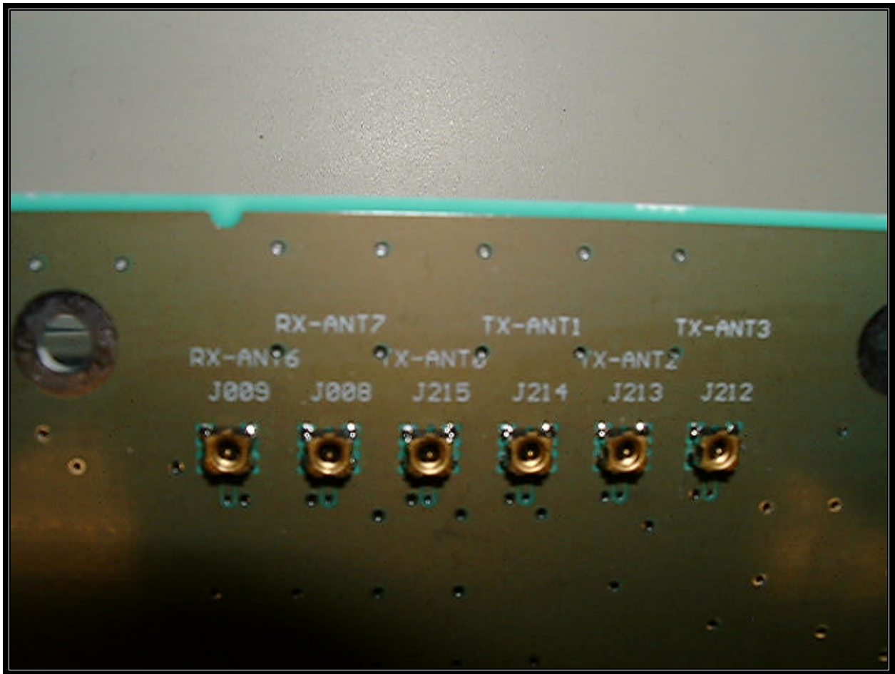
PHOTOGRAPH 28: ALFRED BOARD CONNECTORS
