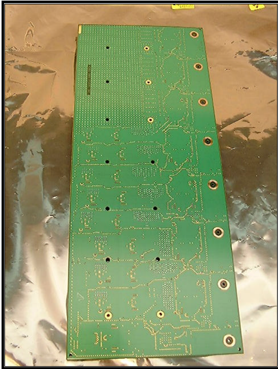
PHOTOGRAPH 31: LEFT ANTENNA BOARD-BOTTOM VIEW
