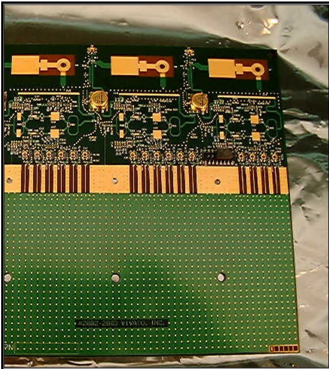
PHOTOGRAPH 34: LEFT ANTENNA BOARD-TOP VIEW RIGHT HALF
