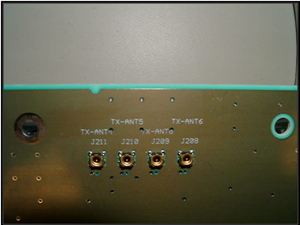
PHOTOGRAPH 30: ALFRED BOARD CONNECTORS
