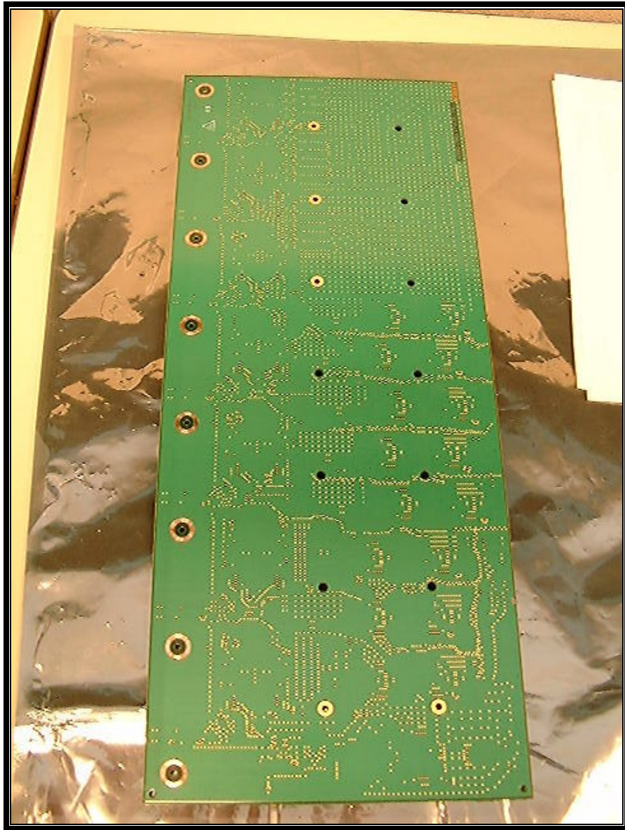
PHOTOGRAPH 32: RIGHT ANTENNA BOARD-BOTTOM VIEW
