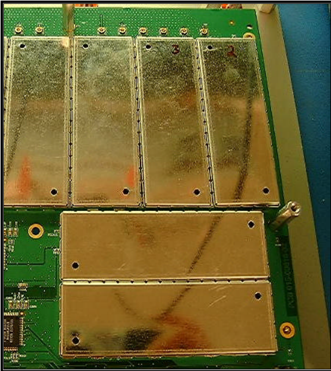
PHOTOGRAPH 48: SIGNAL PROCESSING BOARD-TOP VIEW RIGHT HALF WITH SHIELDS
