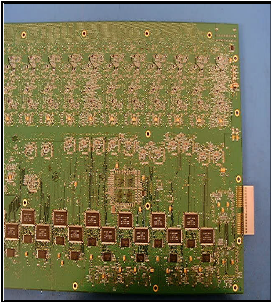
PHOTOGRAPH 44: SIGNAL PROCESSING BOARD-REAR VIEW RIGHT HALF
