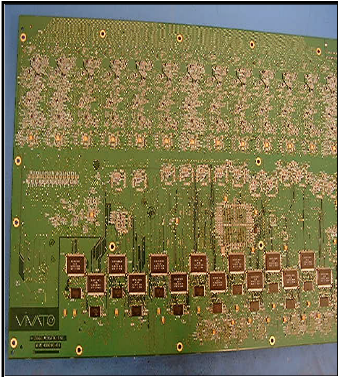
PHOTOGRAPH 43: SIGNAL PROCESSING BOARD-REAR VIEW LEFT HALF
