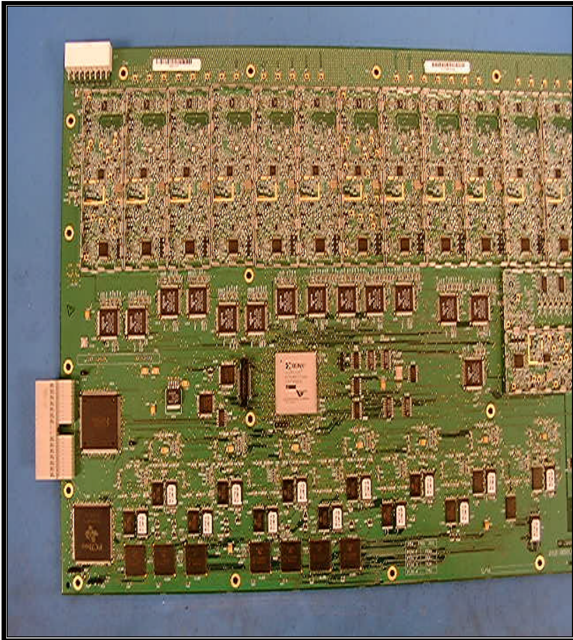
PHOTOGRAPH 45: SIGNAL PROCESSING BOARD-TOP VIEW LEFT HALF WITHOUT SHIELDS
