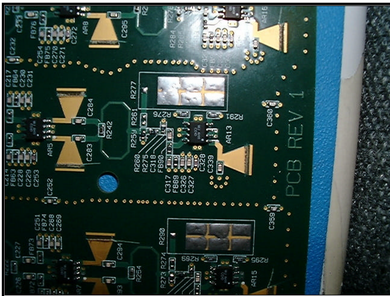
PHOTOGRAPH 38: ANTENNA BOARD PA
