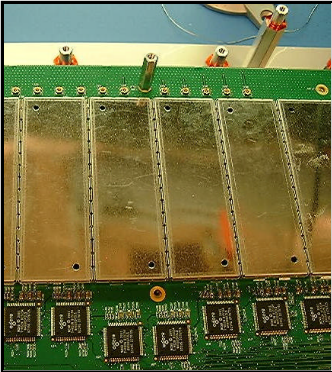
PHOTOGRAPH 47: SIGNAL PROCESSING BOARD-TOP VIEW LEFT HALF WITH SHIELDS
