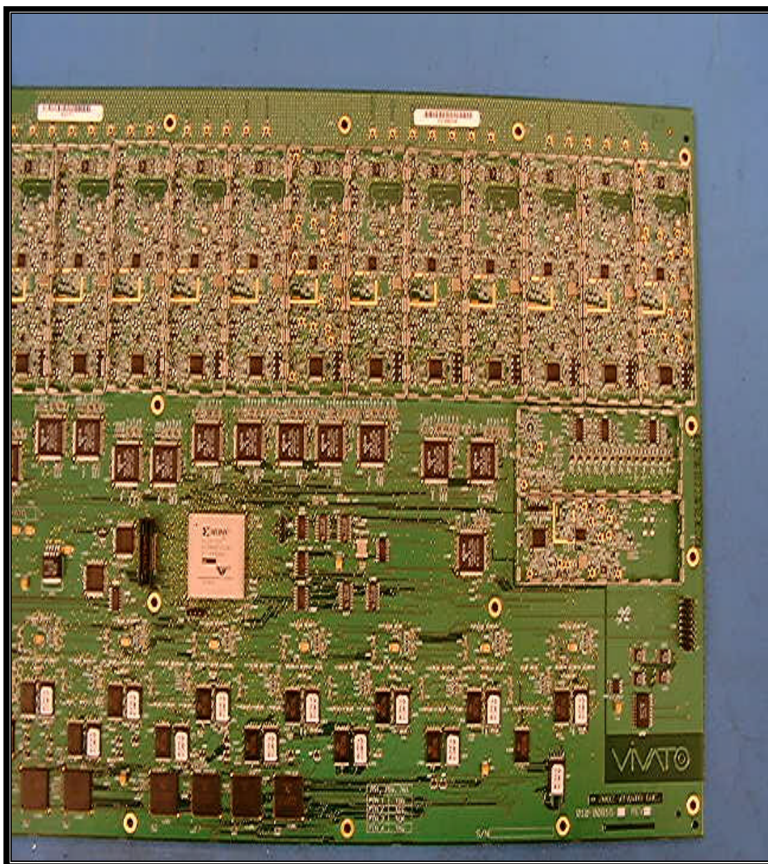
PHOTOGRAPH 46: SIGNAL PROCESSING BOARD-TOP VIEW RIGHT HALF WITHOUT SHIELDS
