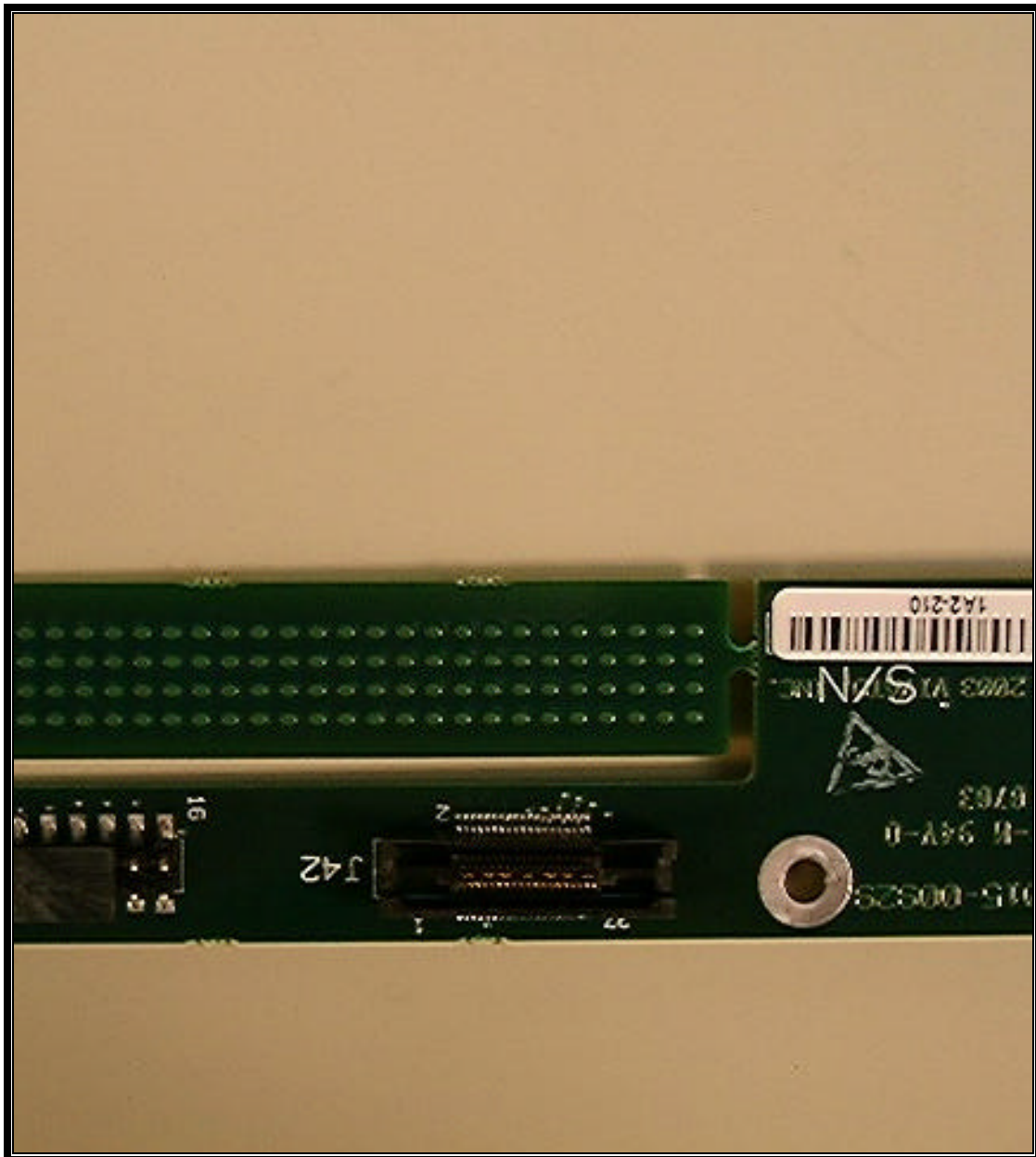
PHOTOGRAPH 41: SOSA BOARD-SIDE 2 LEFT HALF
