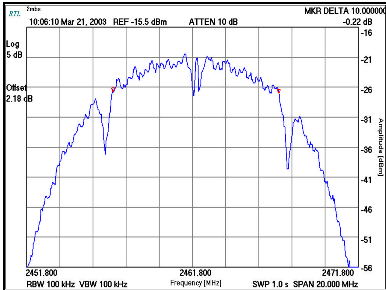
PLOT 7.7-8: 6 DB BANDWIDTH: CHANNEL 11 SET FOR 2 MBPS
