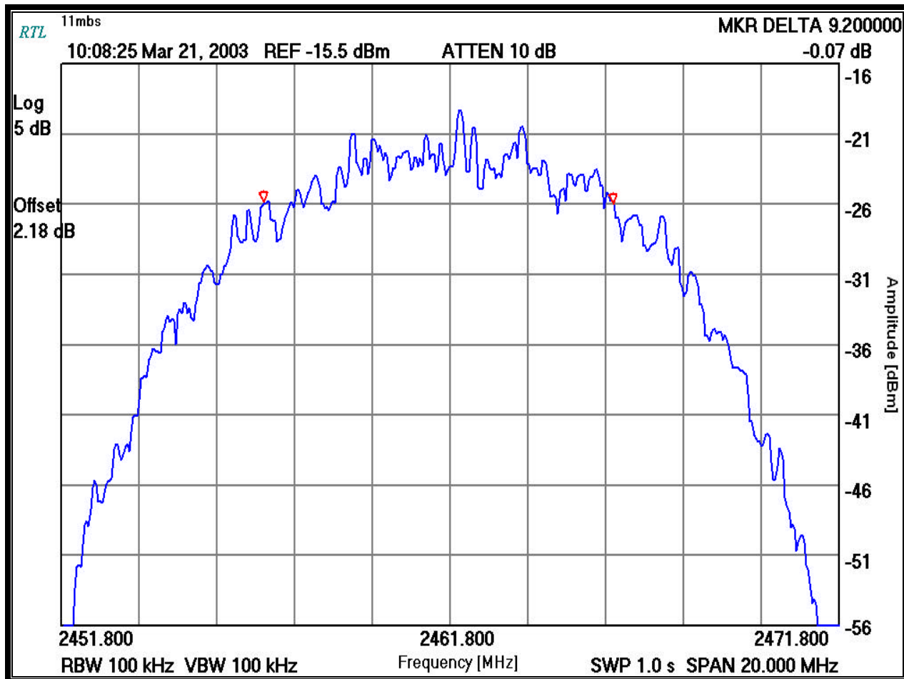
PLOT 7.7-9: 6 DB BANDWIDTH: CHANNEL 11 SET FOR 11 MBPS
