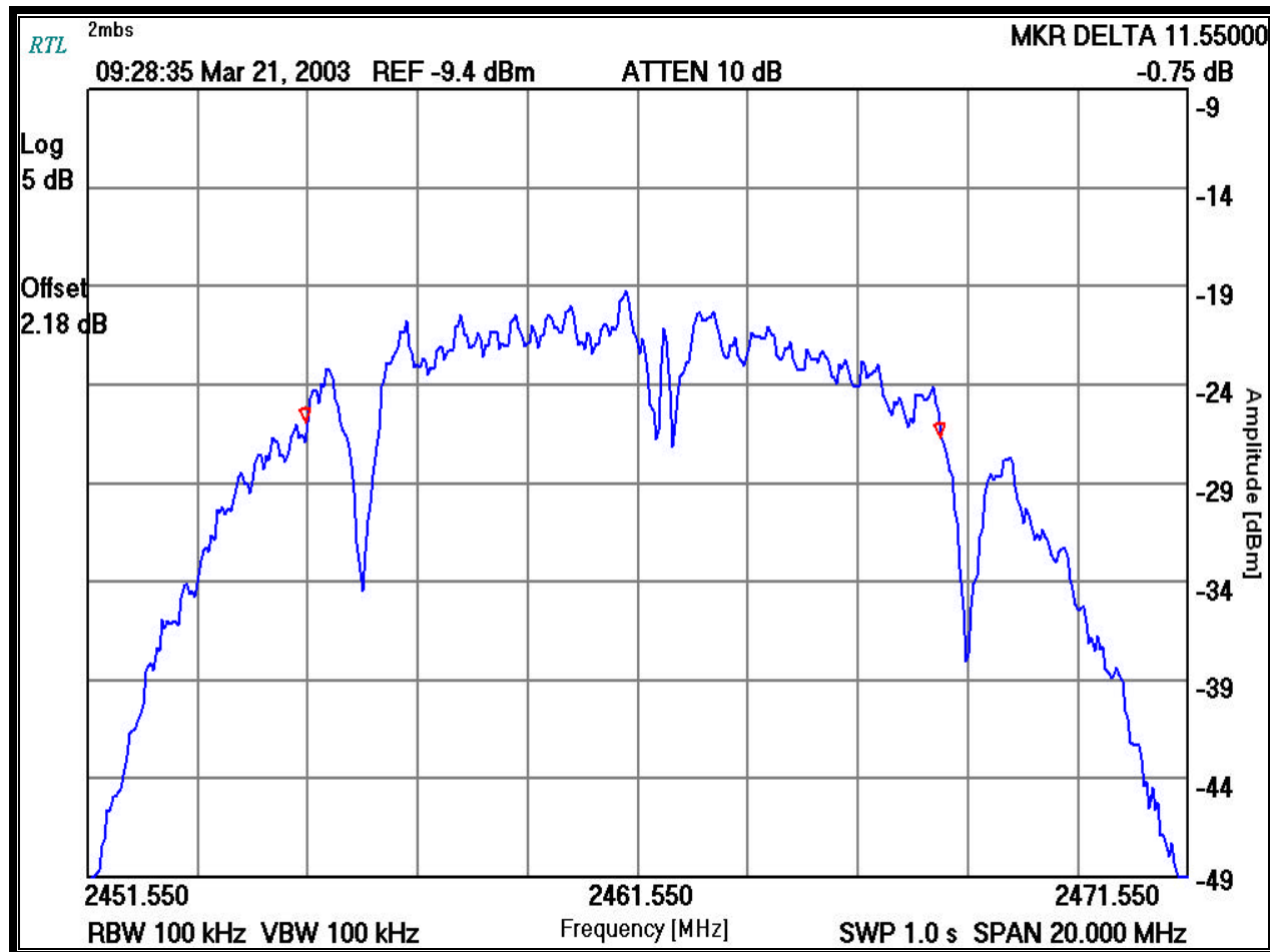
PLOT 7.5-8: 6 DB BANDWIDTH: CHANNEL 11 SET FOR 2 MBPS
