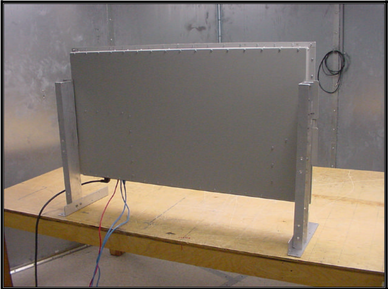
PHOTOGRAPH 2: CONDUCTED EMISSIONS REAR VIEW WORST CASE CONFIGURATION
