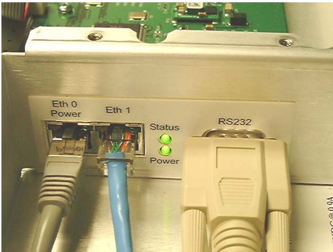
Figure 4 IO Ports
