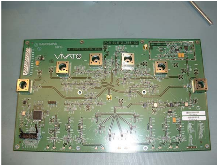
Figure 7 RF Board Top
