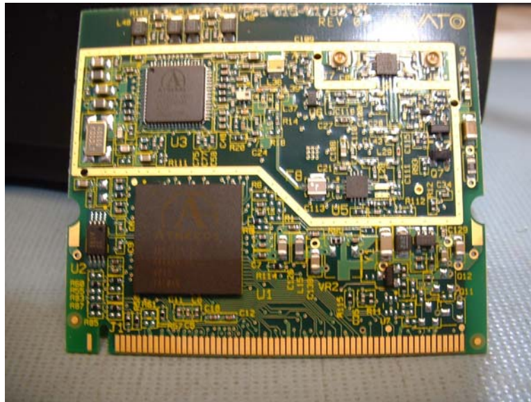
Figure 3 Mini-PCI Card Top without shield
