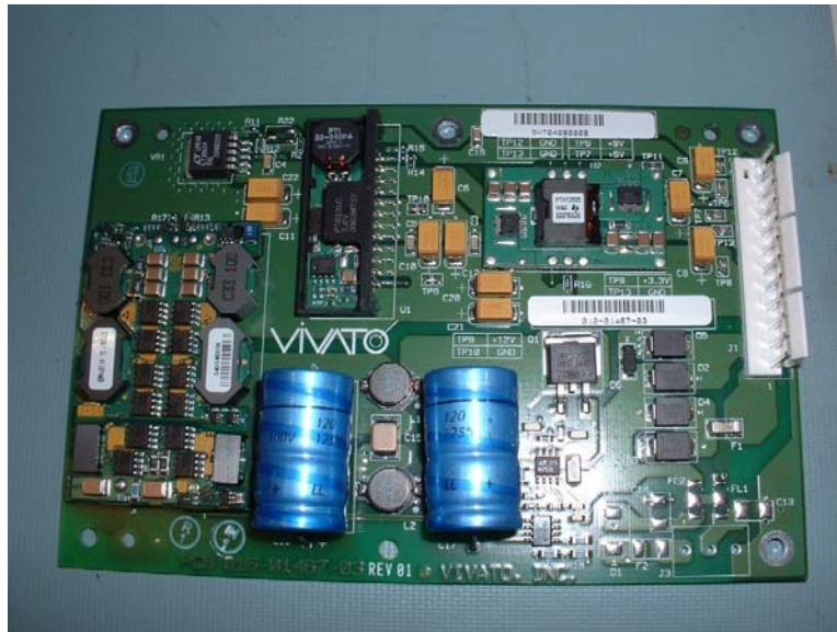
Figure 5 Power Supply Board Top
