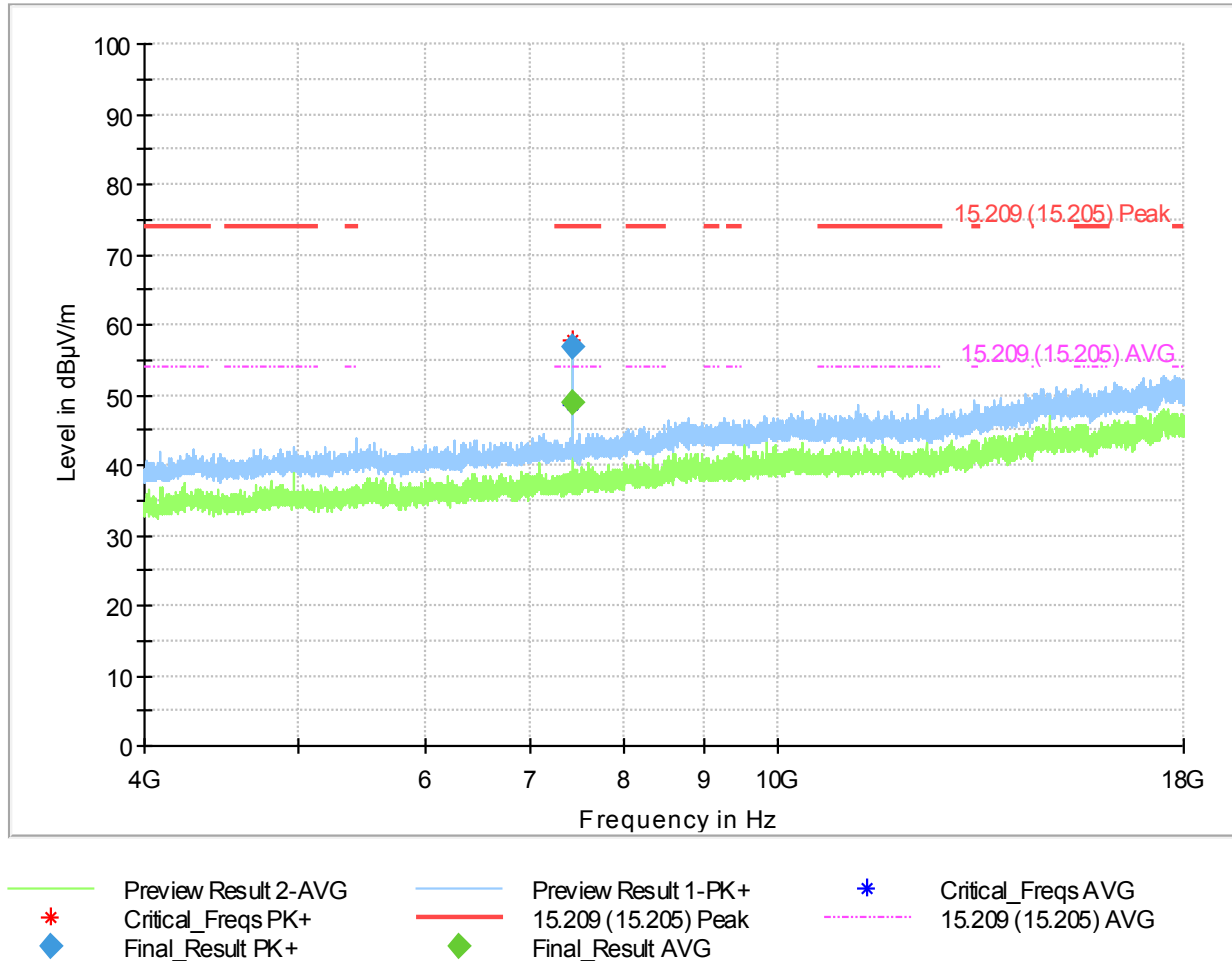
Plot 13: Mode 1, RSE 4 GHz – 18 GHz, high channel, horizontal / vertical polarisation
