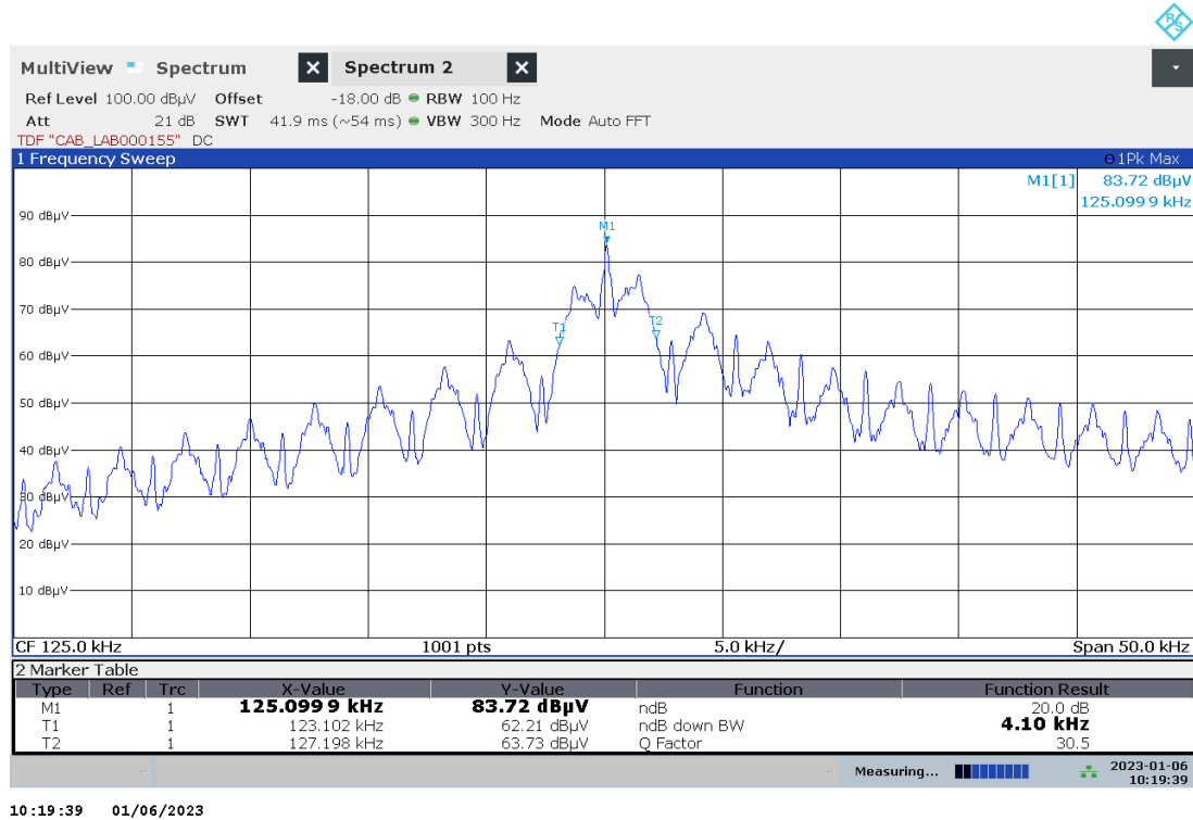
Plot No. 5: 20 dB Bandwidth
