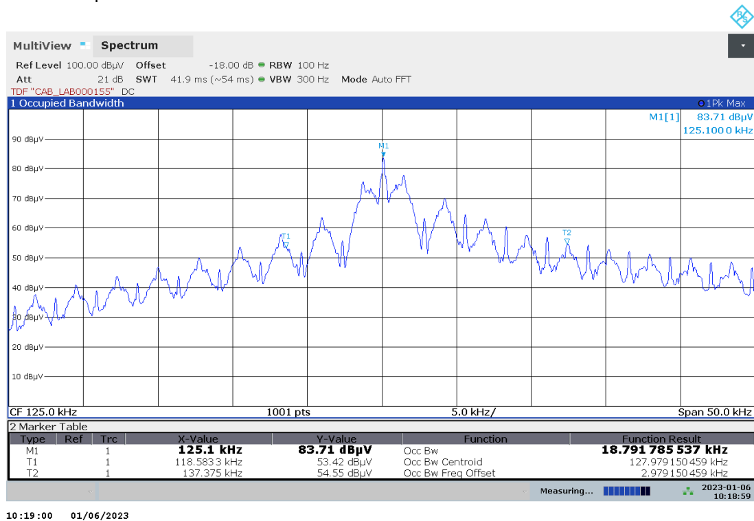
Plot No. 6: 99% Occupied Bandwidth
