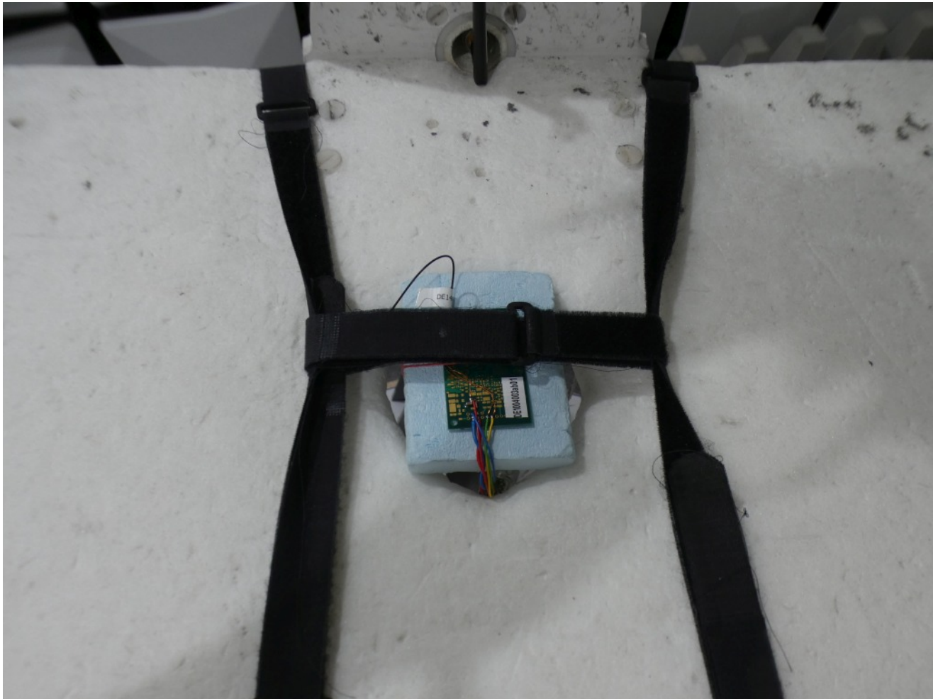
Photo 4: Test setup for radiated measurements, detailed view (stand alone setup, 1 GHz – 24 GHz; FCC 15c247)
