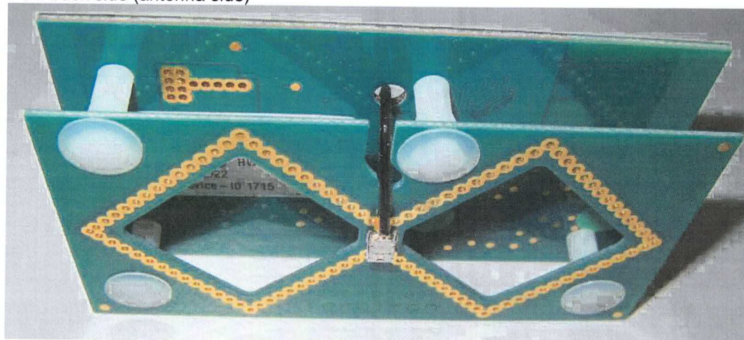
PCB back side (antenna side)
