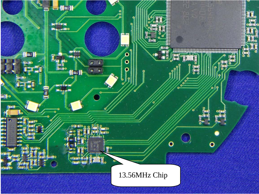
(22) EUT Photo
