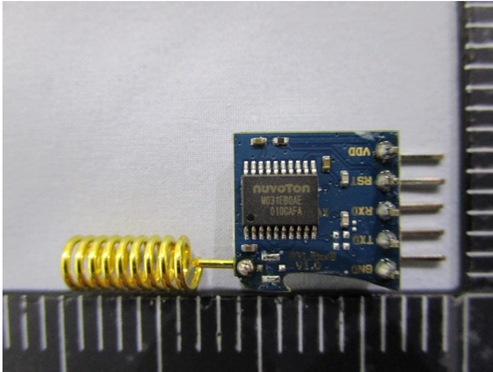
Outview: RYLR998 Pic 7
