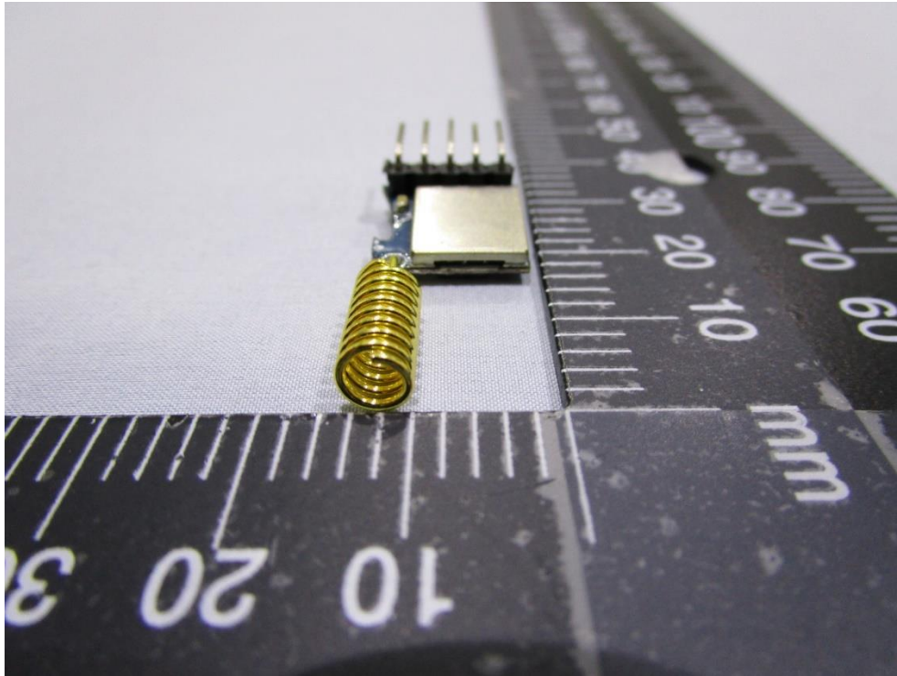
Outview: RYLR998 Pic 5
