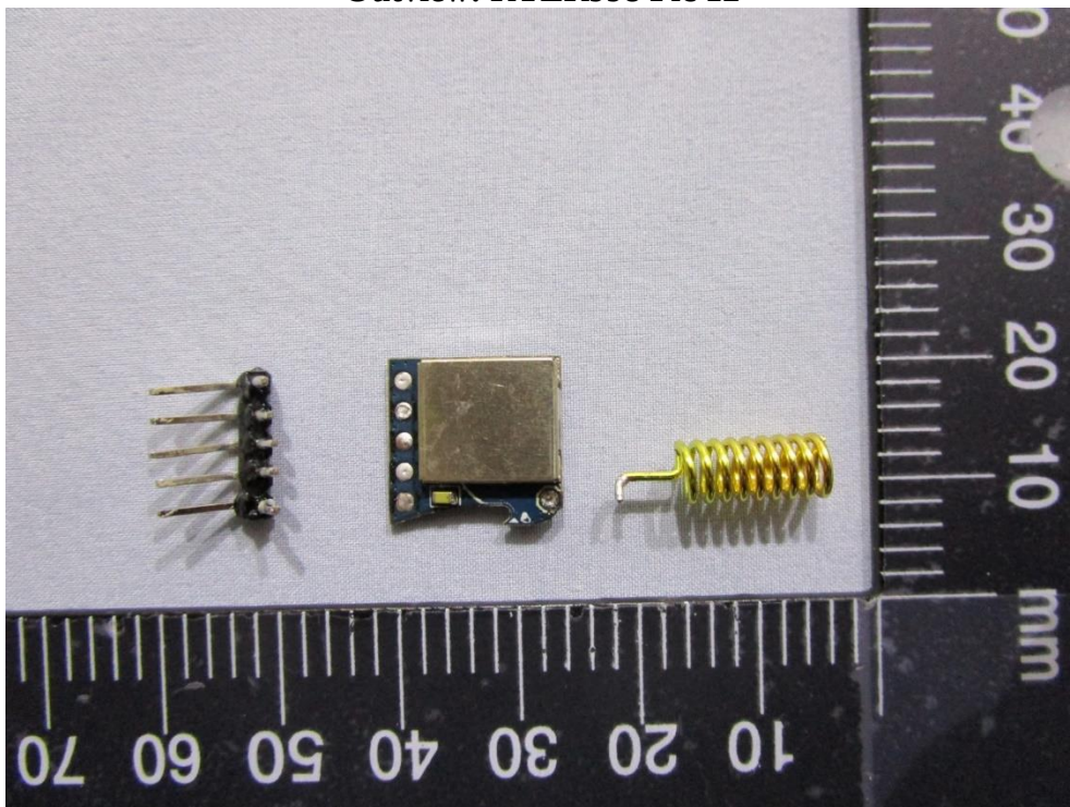
Outview: RYLR998 Pic 12
