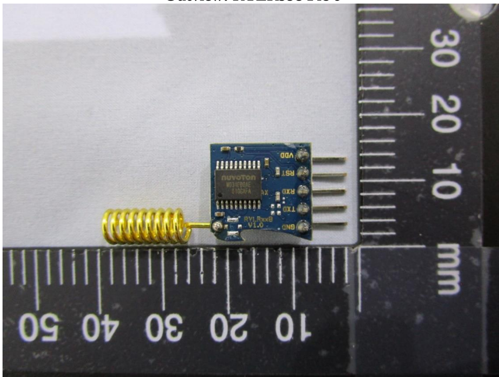
Outview: RYLR998 Pic 6
