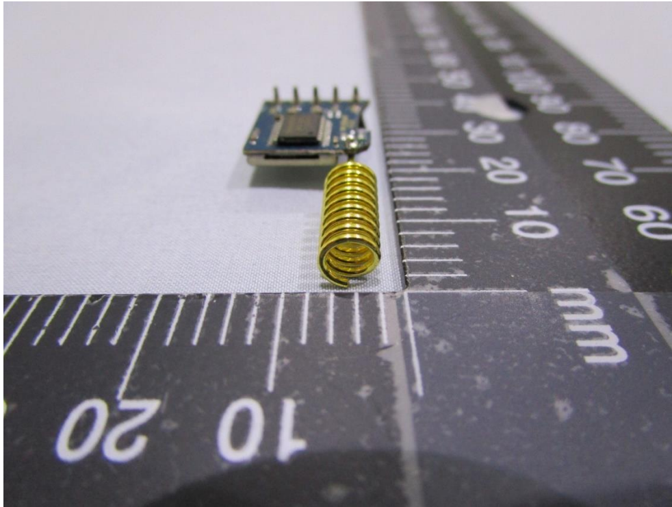
Outview: RYLR998 Pic 11
