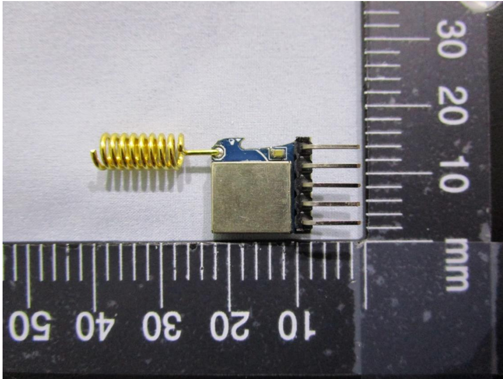
Outview: RYLR998 Pic 1
