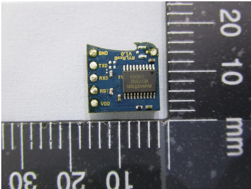
Outview: RYLR998 Pic 18
