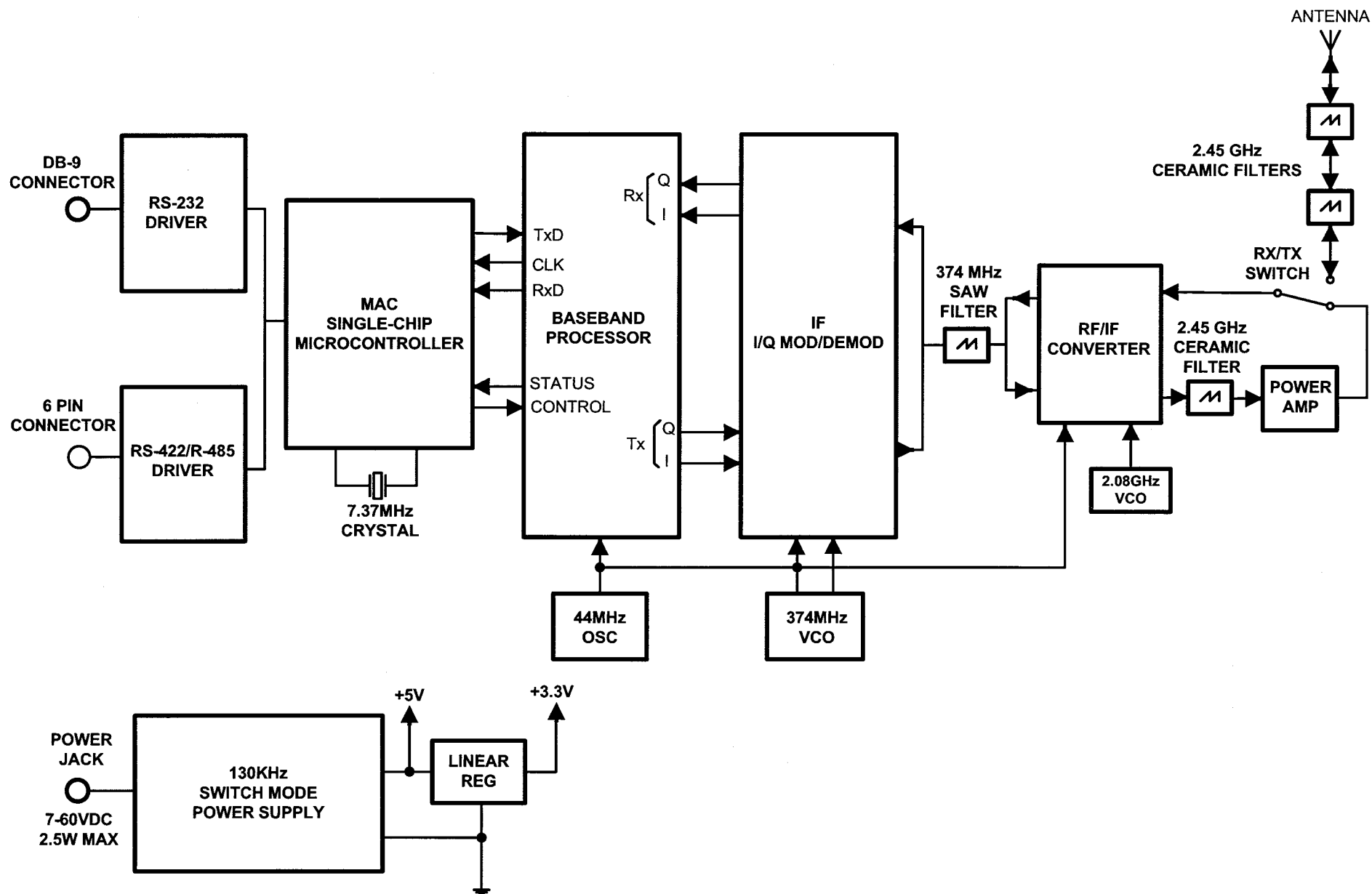
M-2911 BLOCK DIAGRAM
