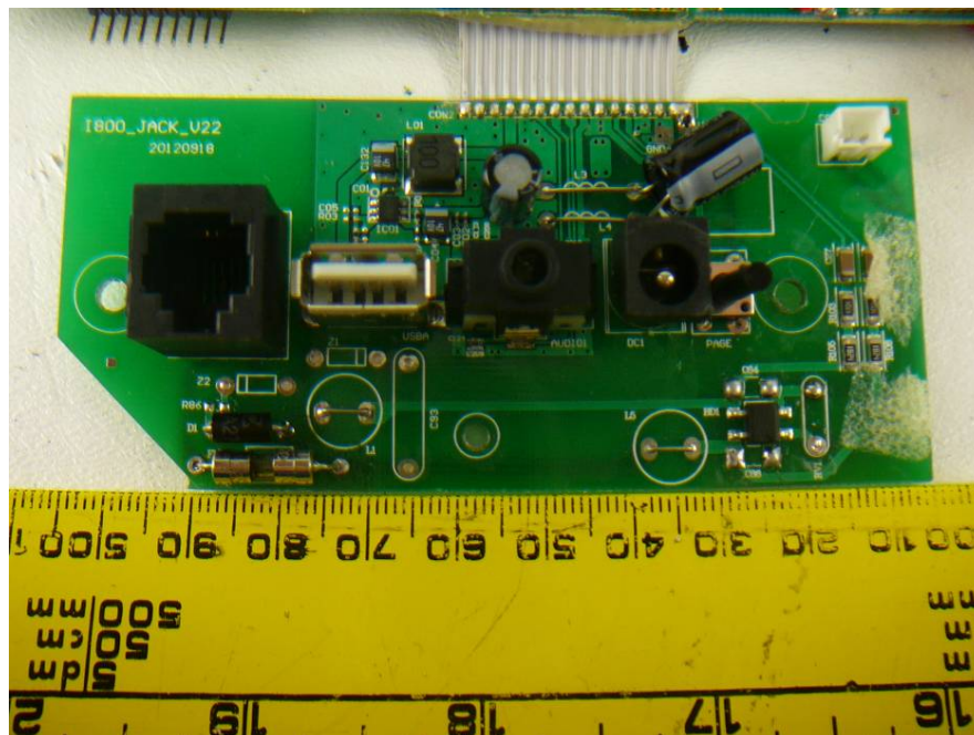
EUT (Base) – I800_JACK_V22 Board Top View
