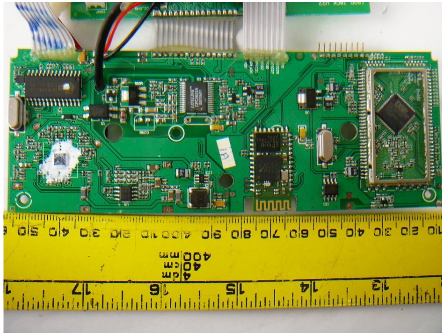
EUT (Base) – Main Board Top Shielding off View
