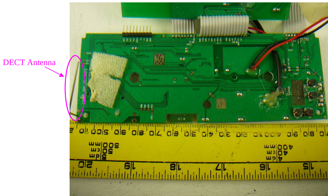
EUT (Base) – Main Board Bottom View
