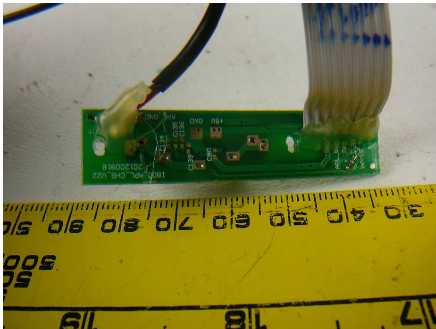
EUT (Base) – I800_APL_CHG_V22 Board Bottom View
