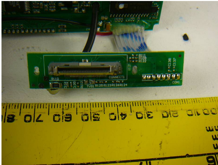
EUT (Base) – I800_APL_CHG_V22 Board Top View
