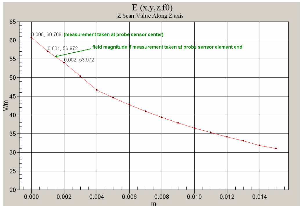
Figure 6 Z-axis scan at maximum point above a typical wireless device
