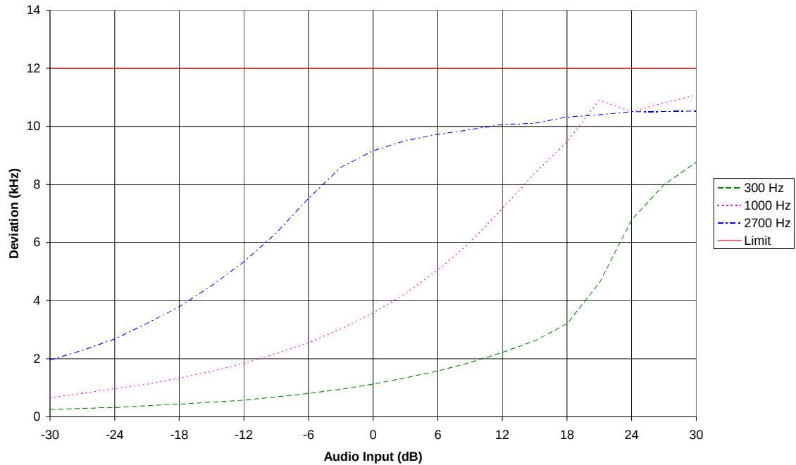
Modulation Limiting - Voice Only, Positive Peaks
