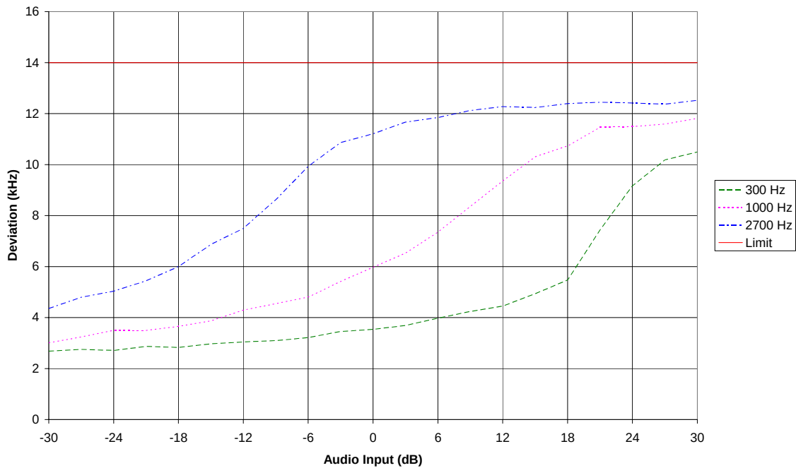
Modulation Limiting - Voice+SAT, Positive Peaks
