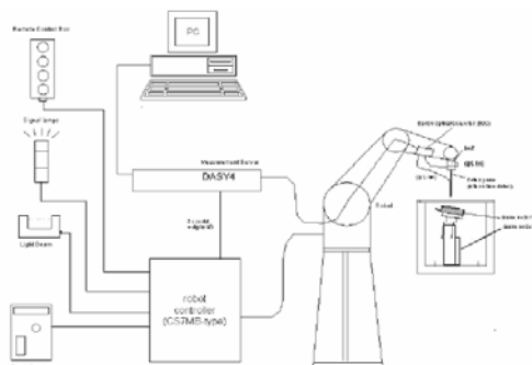
Figure 10 SPEAG Robotic System Diagram
