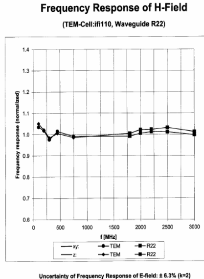
Figure 7 H-Field Probe Frequency Response
