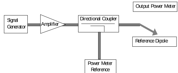
Figure 15 Setup to Dipole
