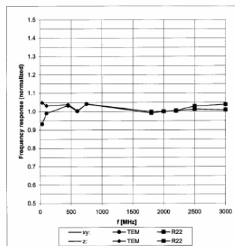
Frequency Response of E-Field (TEM-Cell: R1110 EXX, Waveguide R22)
