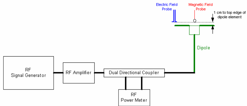
Figure 16 System Check Setup
