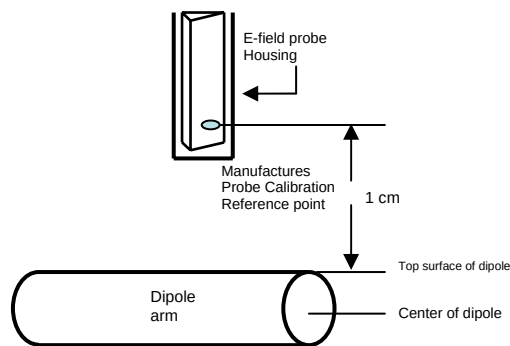
Figure 13 Separation Distance from Dipole to Field Probe
