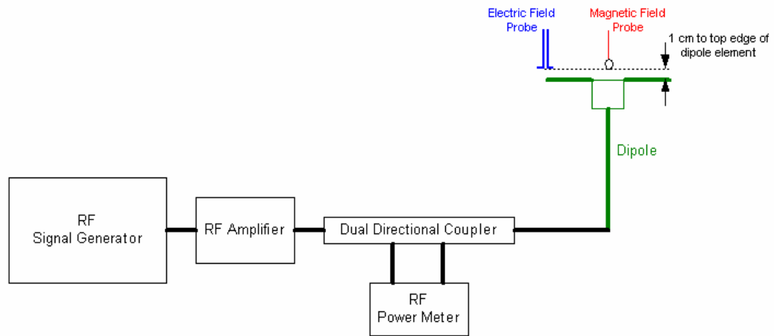
Figure 20 Determining Modulation Factor Probe Setup
