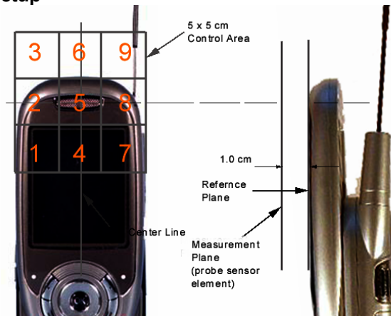
Figure 11 E/H-Field Emissions Test Setup Diagram
