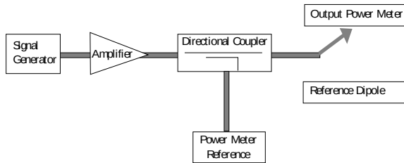
Figure 14 Setup for Desired Output Power to Dipole
