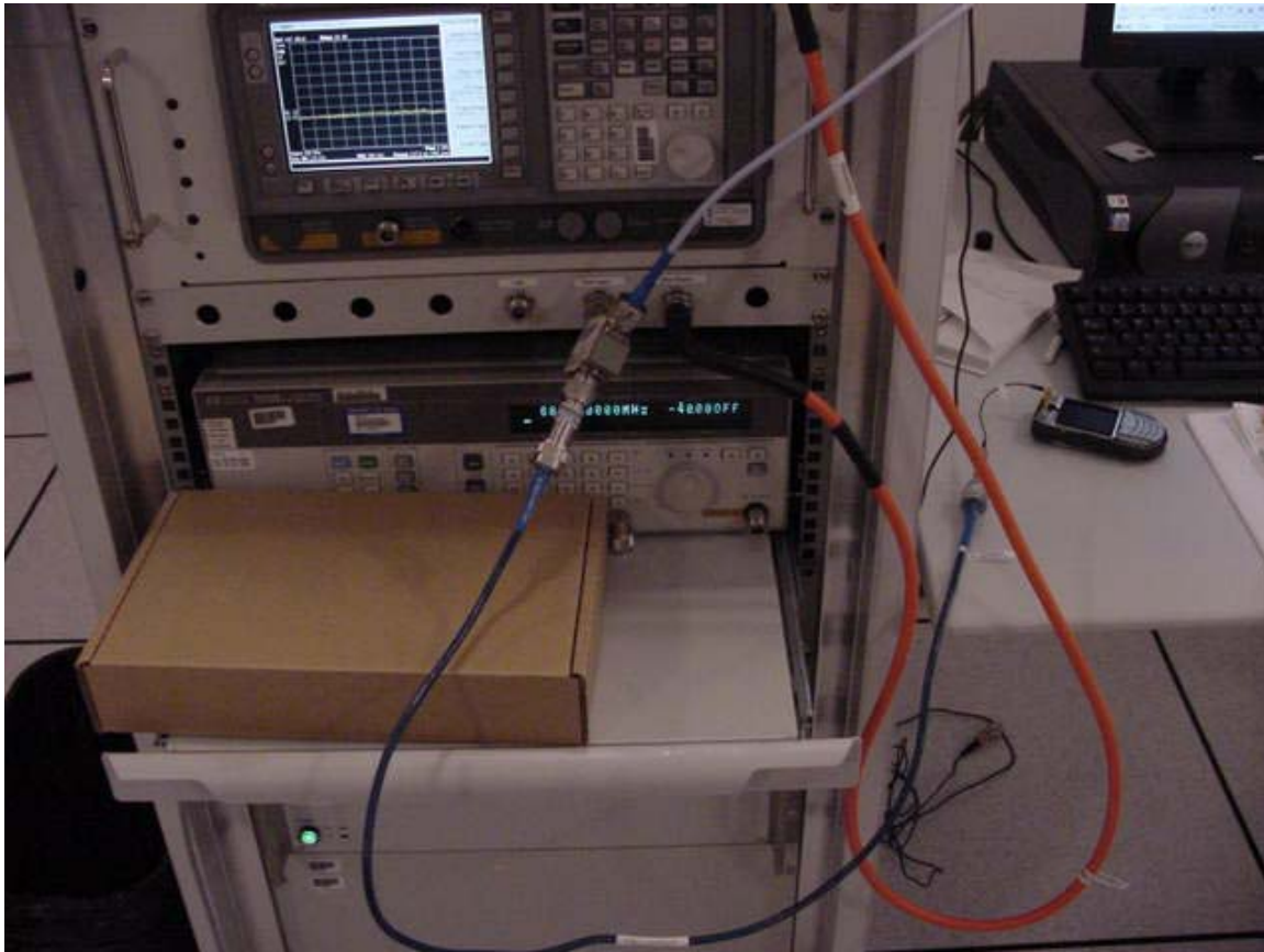
Conducted antenna terminal measurement
