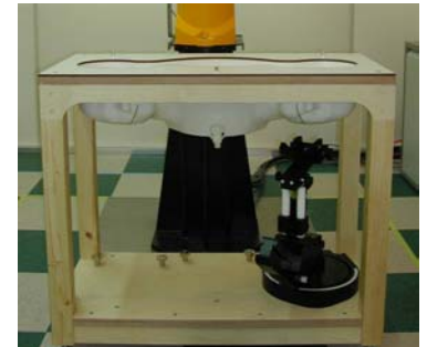
Figure 11. SAM Phantom
