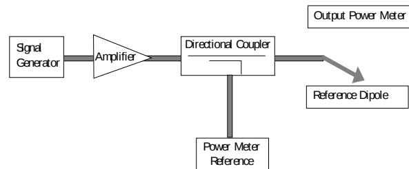
Figure 14 Setup to Dipole
