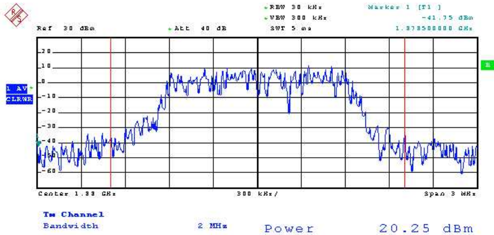
CDMA Signal for 1900MHz band
