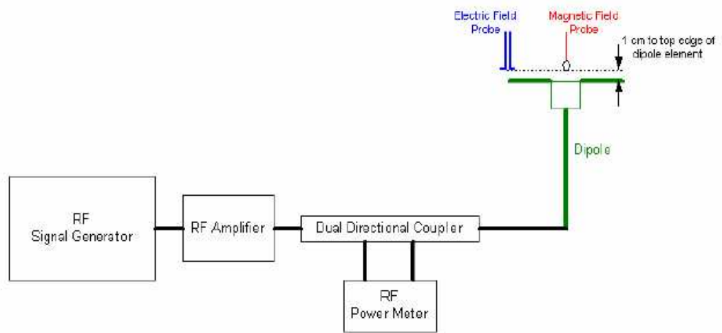
Determining Modulation Factor Probe Setup
