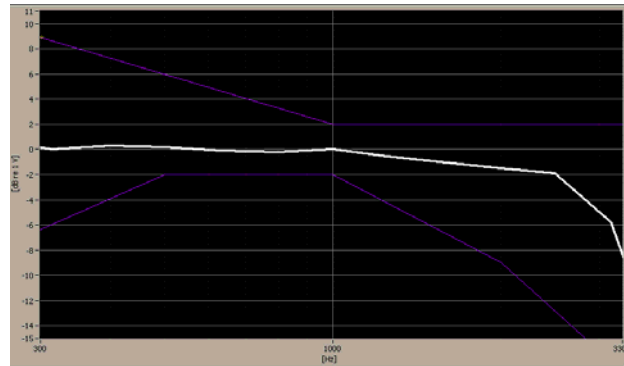
Figure 6-1 Axial Frequency Response
