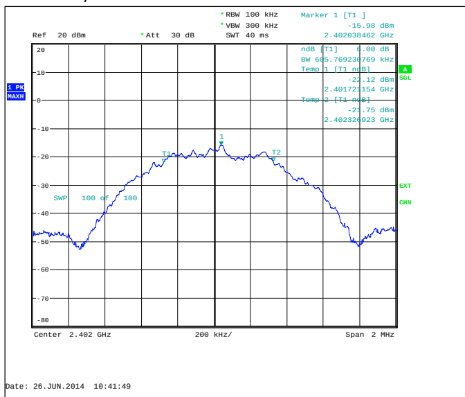
Channel 0 / 2402 MHz
