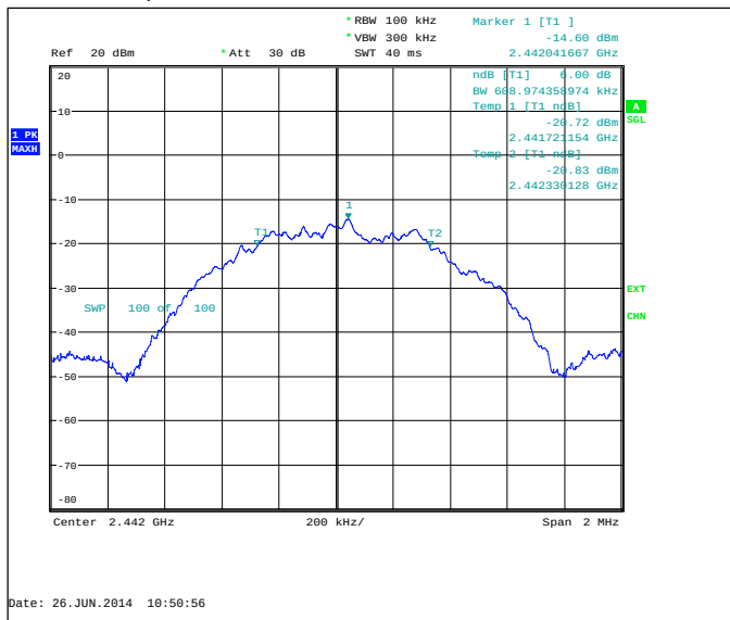
Channel 20 / 2442 MHz
