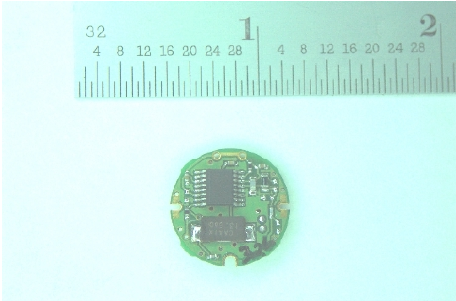
Back Side of the PCB Assembly
