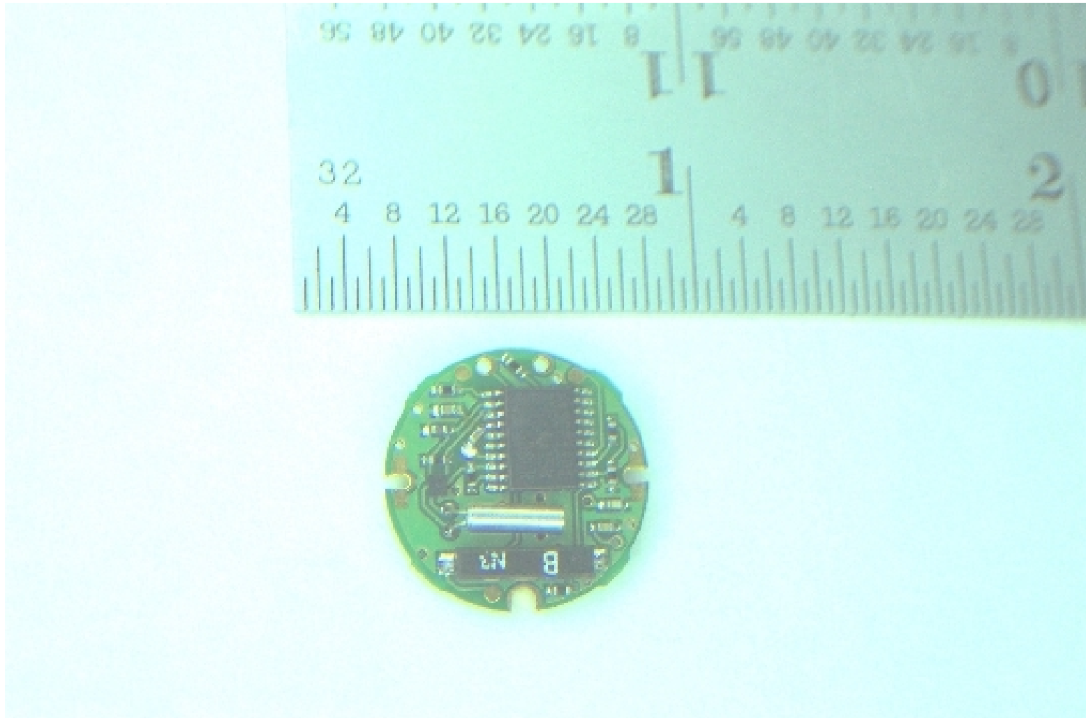
Top Side of the PCB Assembly
