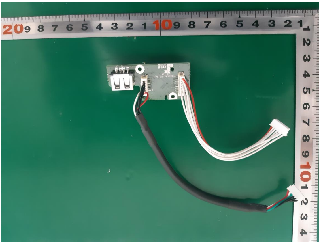
SUB BOARD(BOTTOM)
