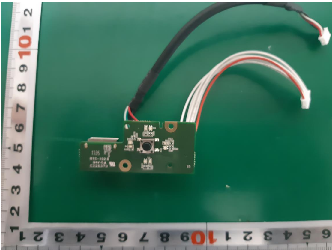
SUB BOARD(BOTTOM)
