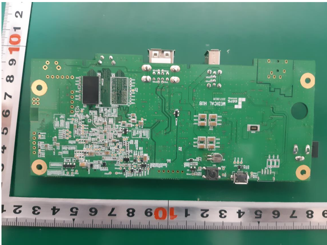
MAIN BOARD(BOTTOM)
