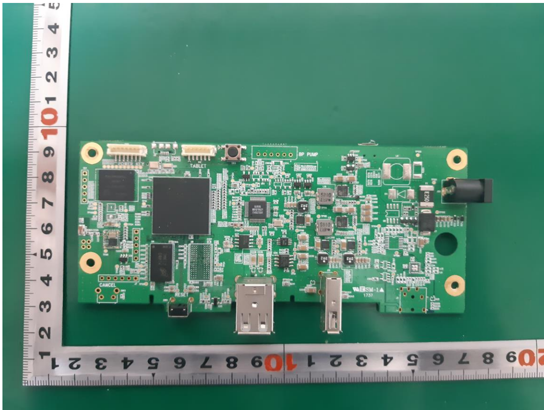
MAIN BOARD(BOTTOM)
