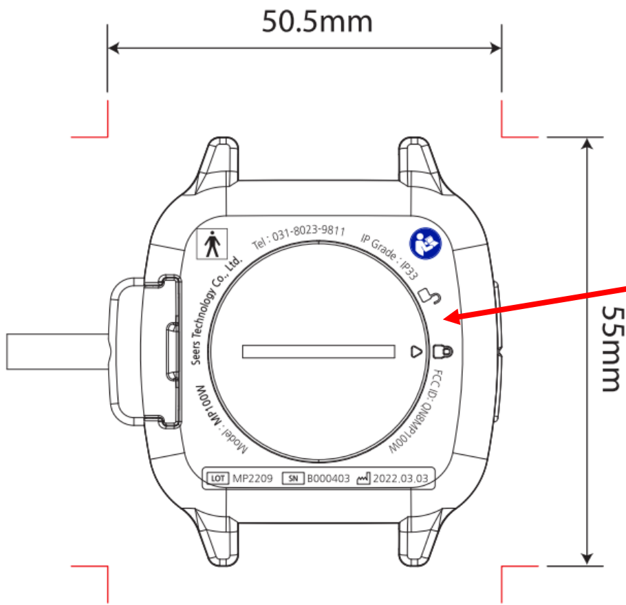
BOTTOM-COVER Part
