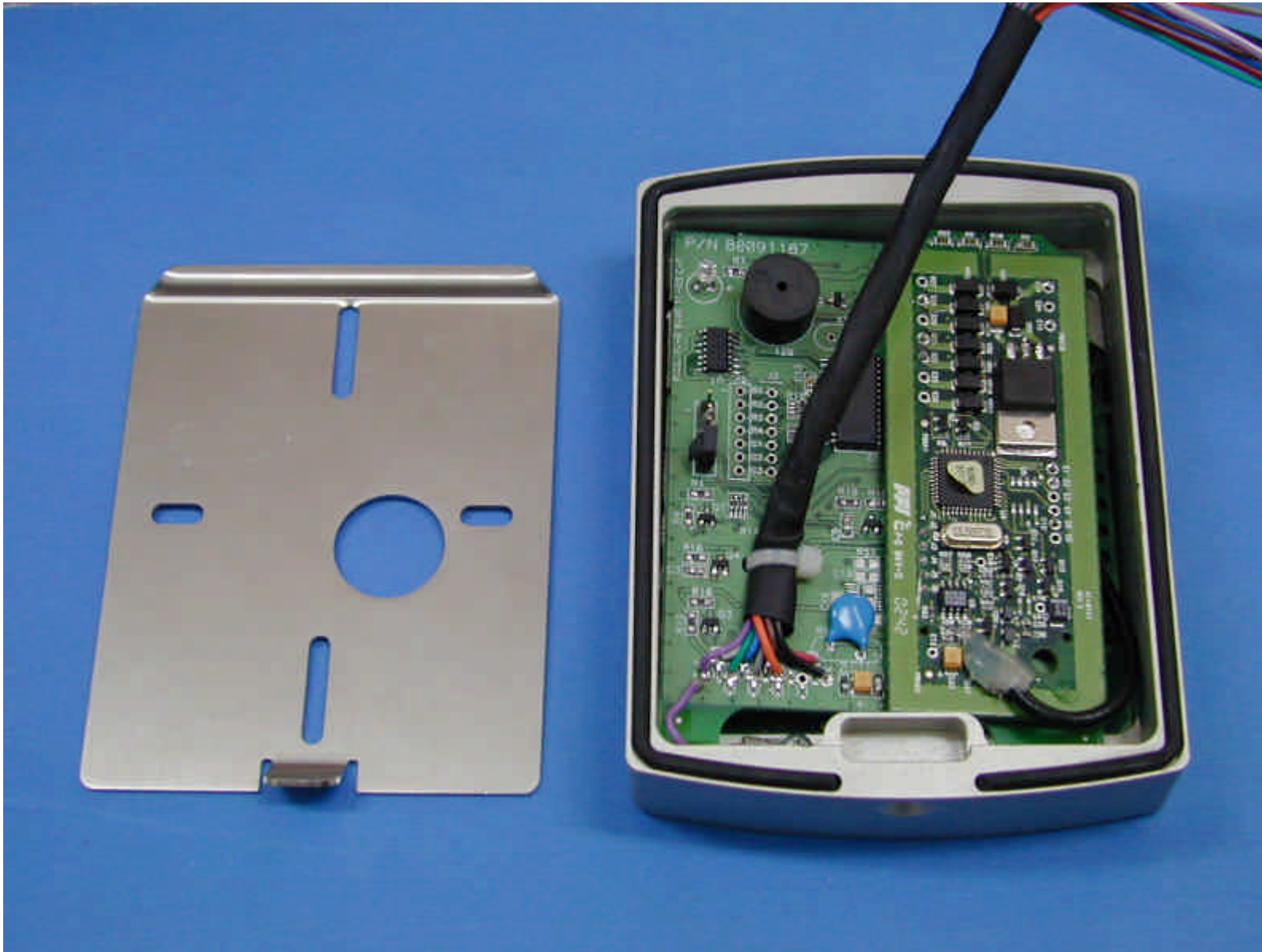
Internal view
