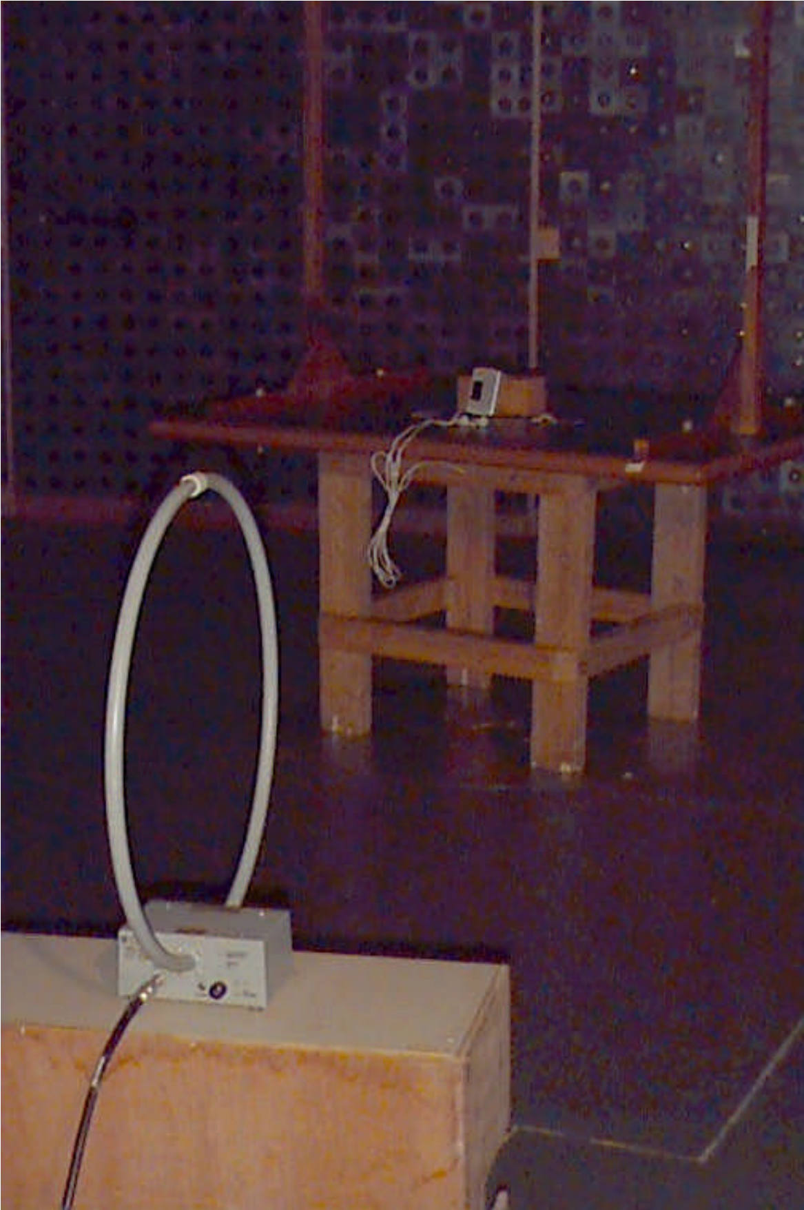
Measurements with loop antenna
