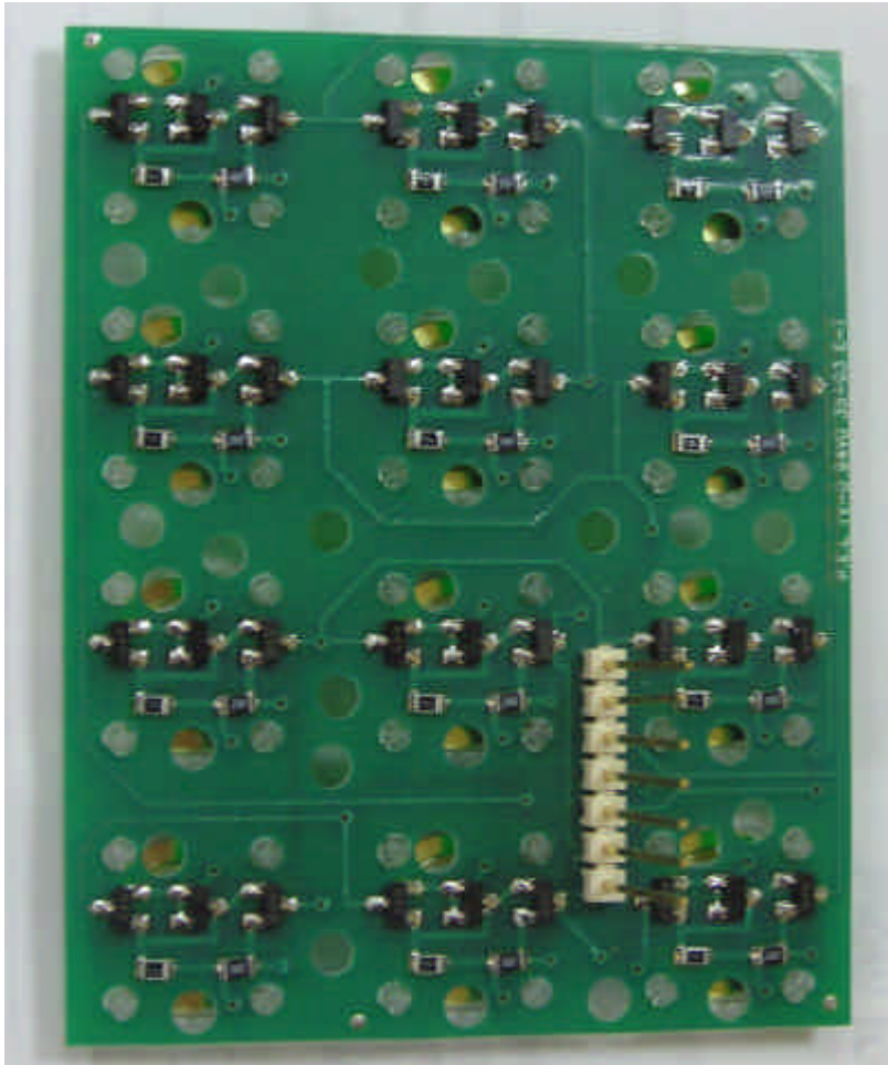
Photograph No.11 Keypad PCB front side
