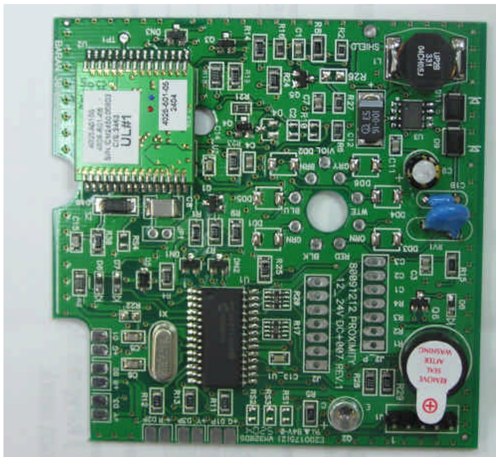
Photograph No.8 Controller PCB front side
