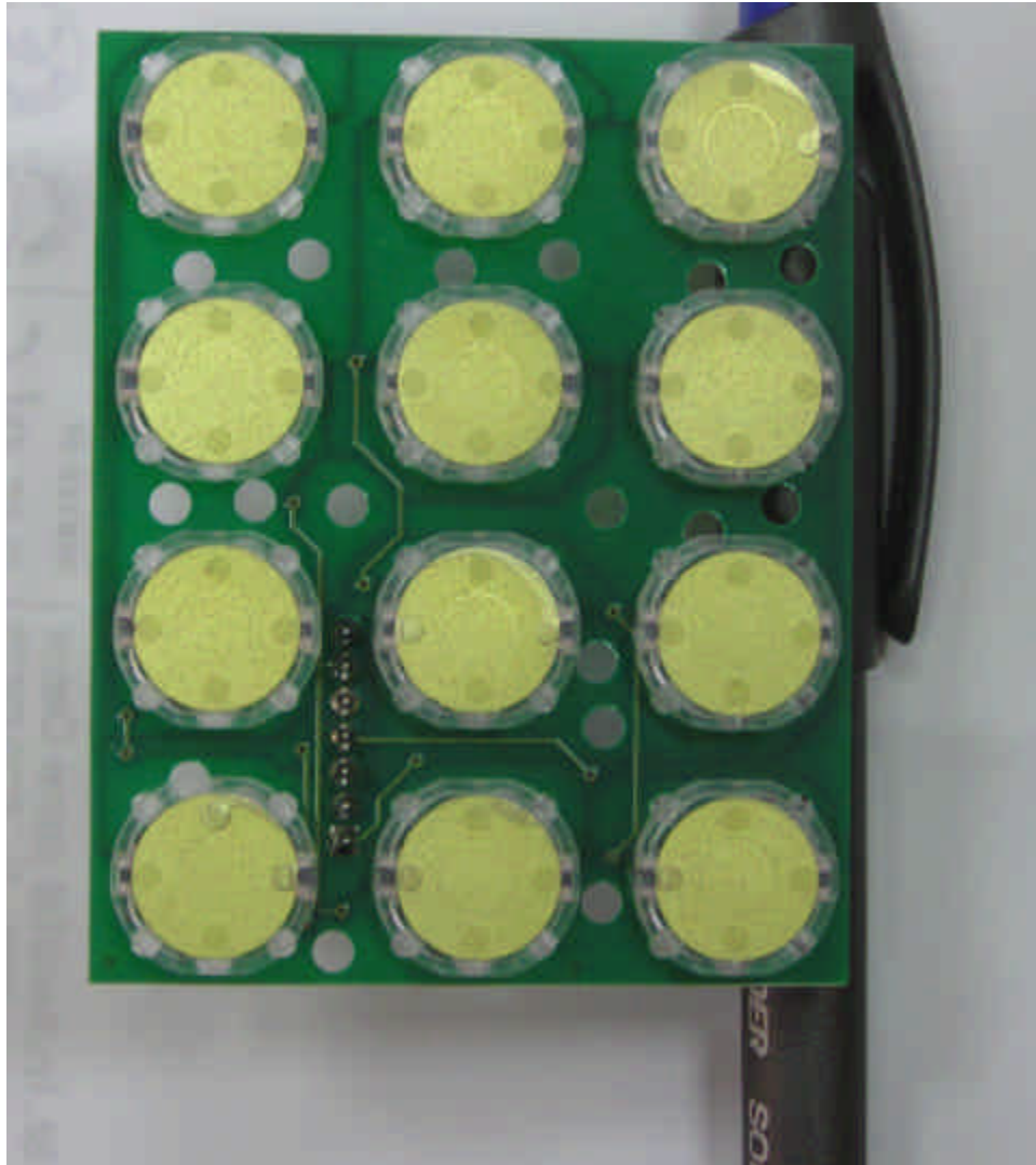
Photograph No.10 Keypad PCB front side
