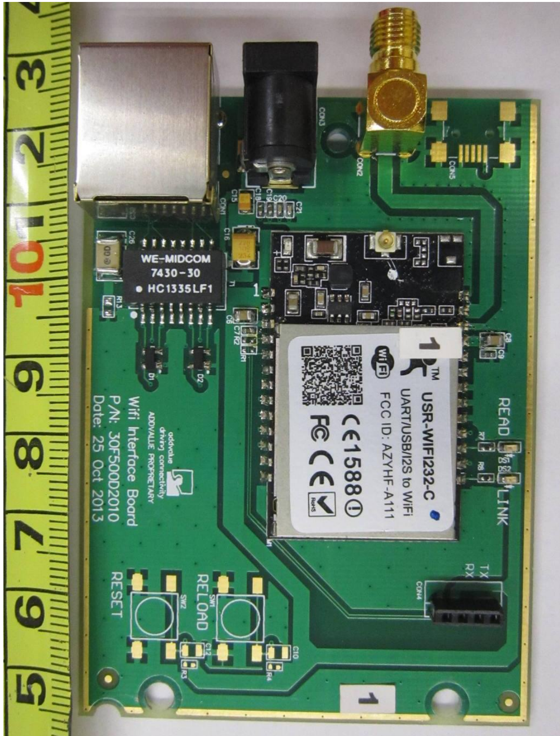
WiFi Interface Board PCB Component Side
