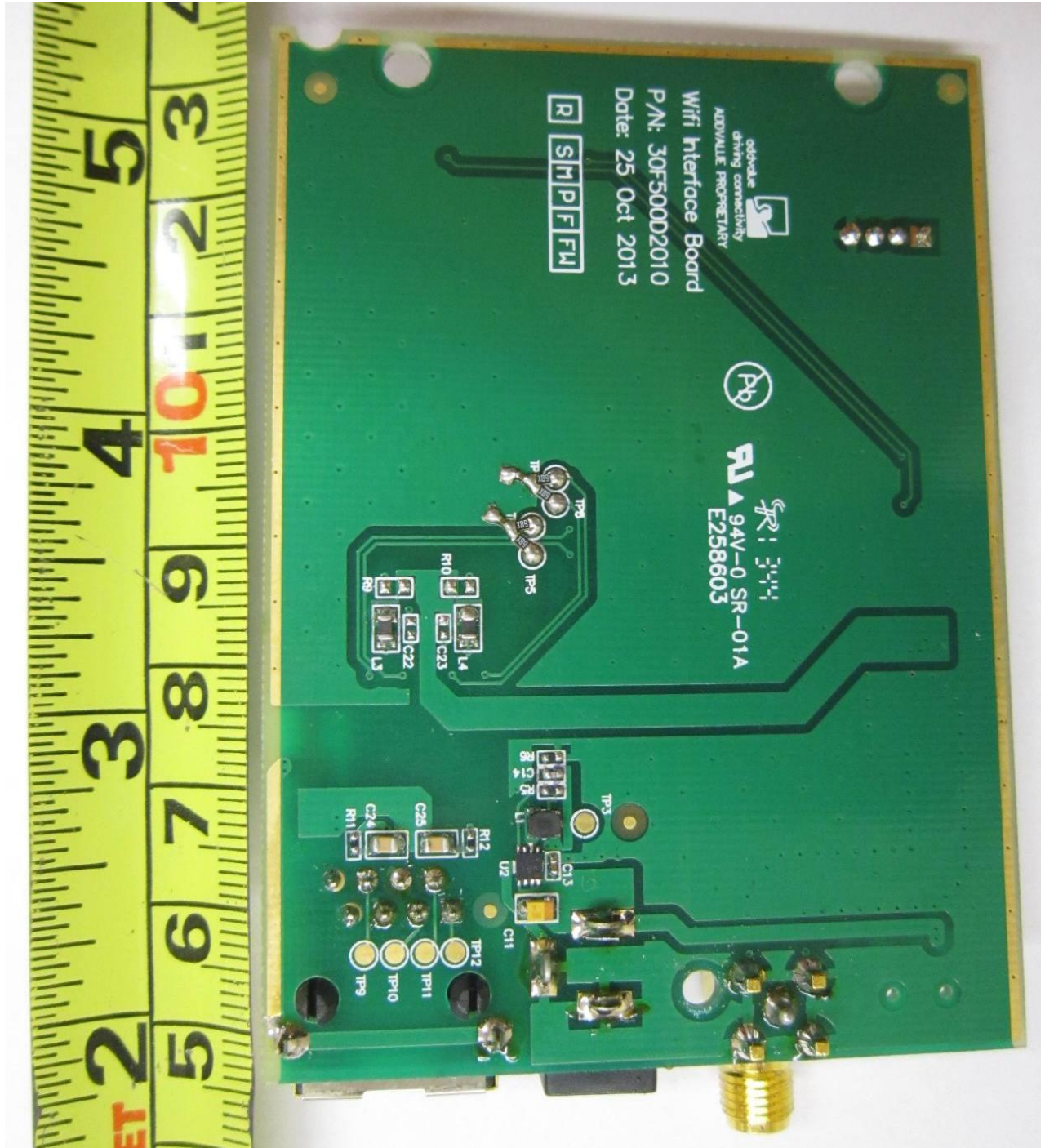
WiFi Interface Board PCB Trace Side
