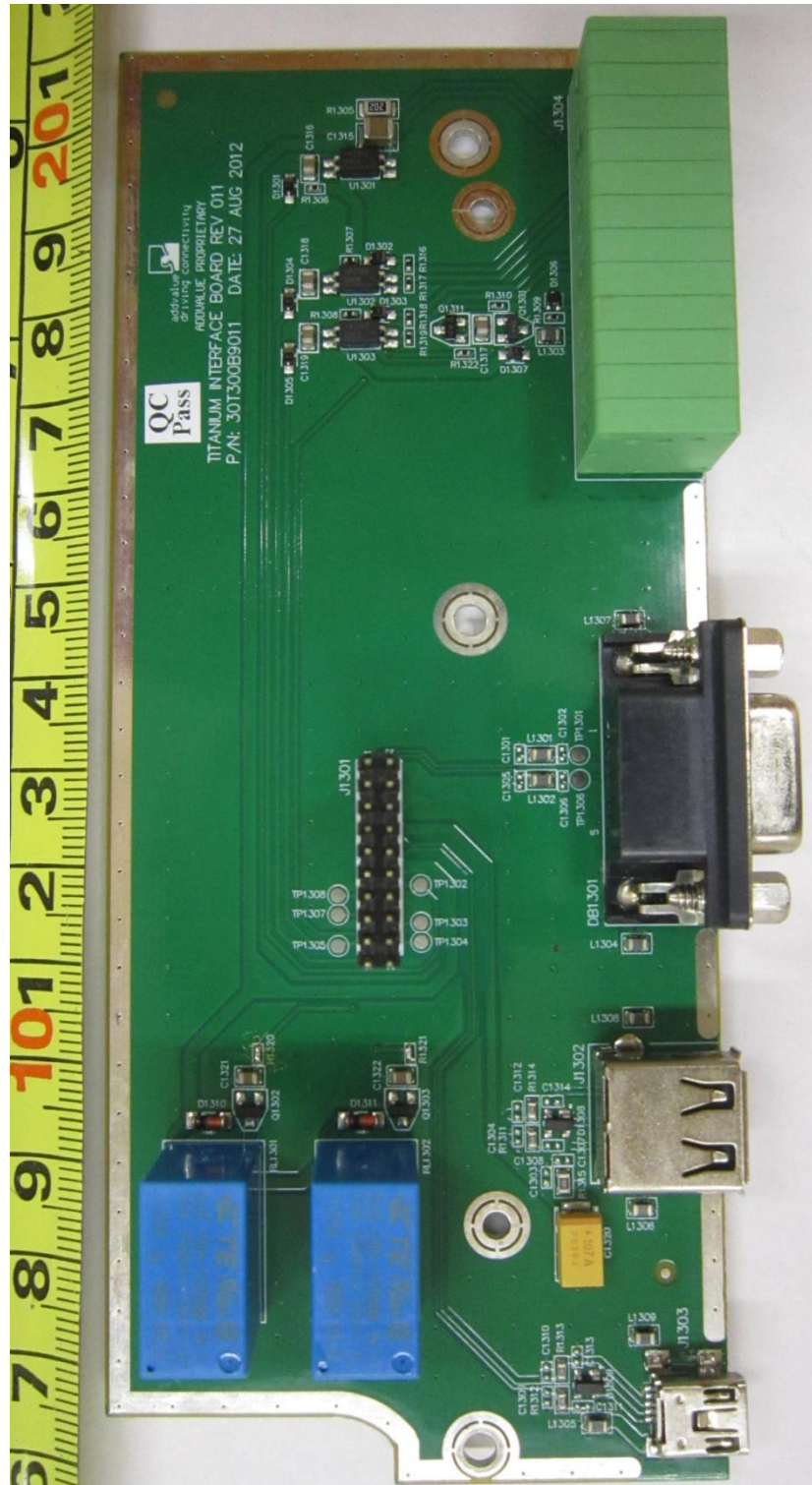
Interface Board PCB Component Side
